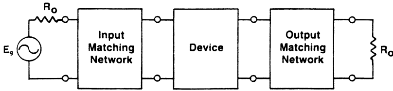
FIGURE 2.30 Two-port matching network ( R_0 = Z_0 ).
