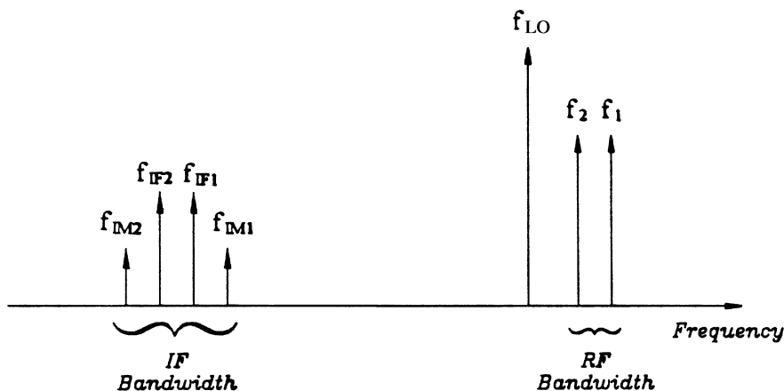
FIGURE 5.11 Intermodulation products.
