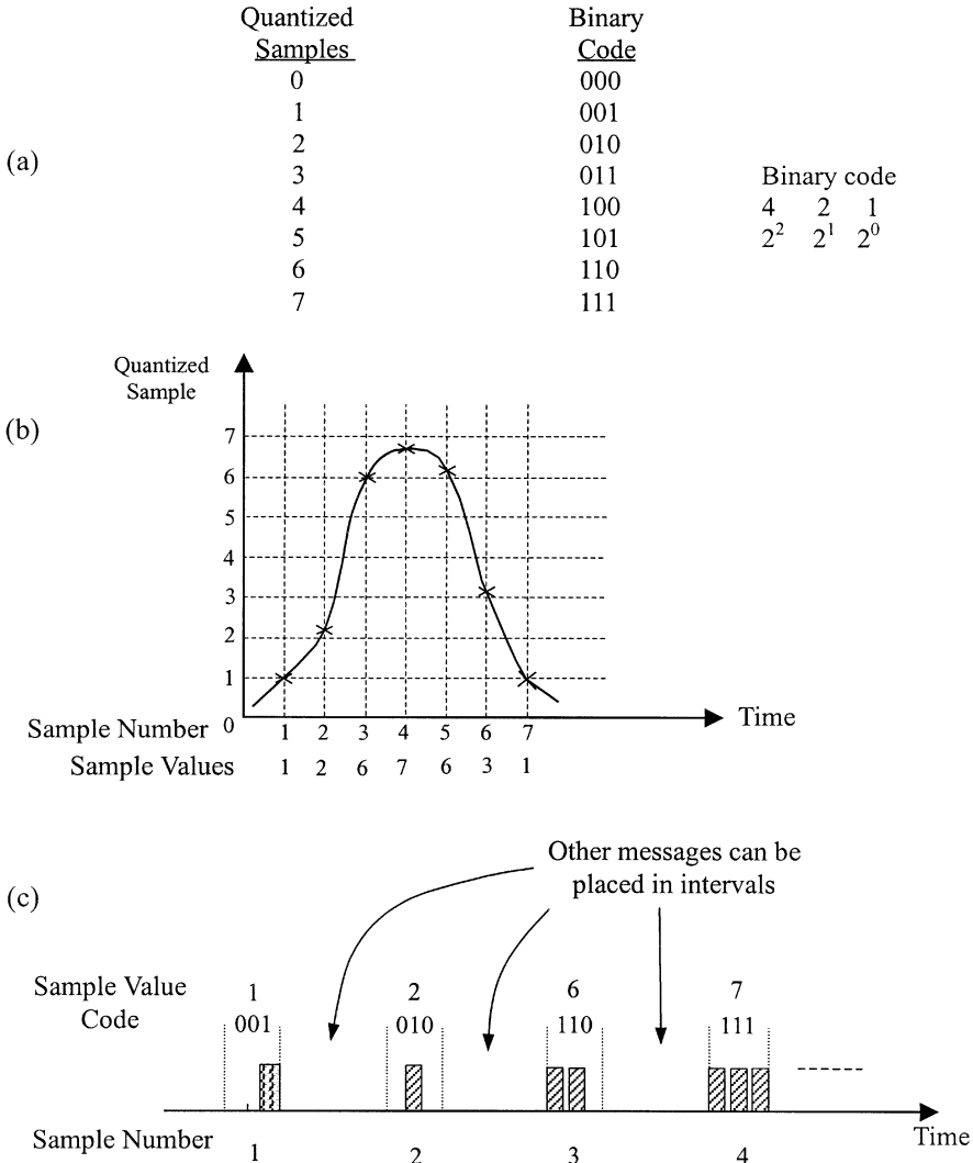
FIGURE 9.17 Sampling and PCM encoding for N = 3 : (a) quantized samples and binary codes; (b) sampling and quantization; (c) PCM codes.
