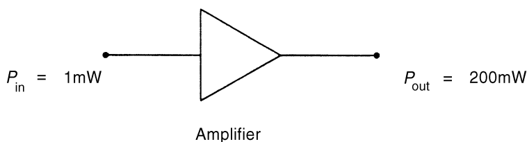
FIGURE 2.12 Amplifier circuit.
