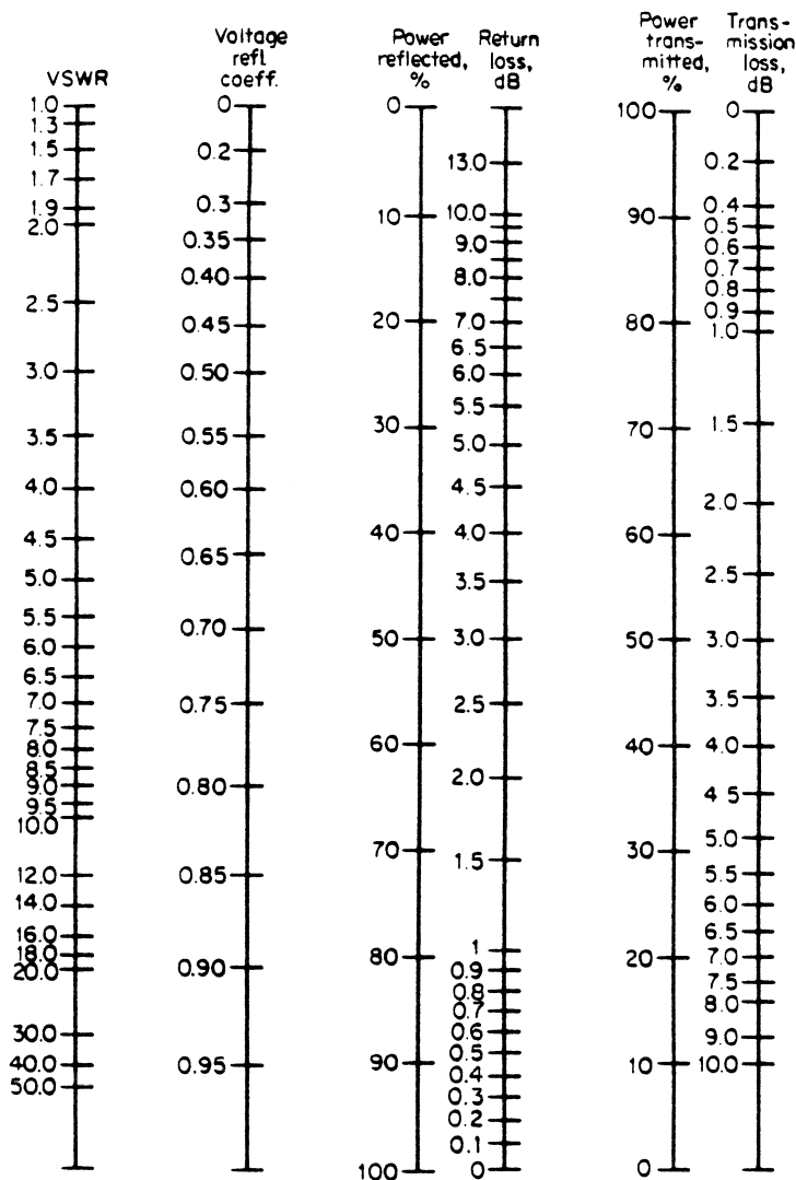
FIGURE 2.9 VSWR nomograph.
