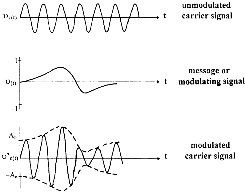
FIGURE 9.2 Signals in AM.
