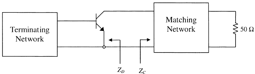
FIGURE 4.36 Transistor oscillator.
