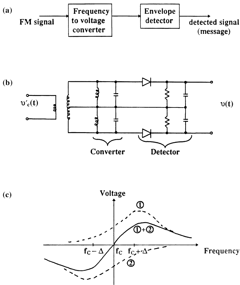
FIGURE 9.5 Balanced frequency discrimination: (a) block diagram; (b) circuit schematic; (c) voltage–frequency characteristics.
