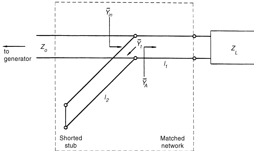
FIGURE 2.31 Matching network using a single stub to match Z_L to Z_0 .
