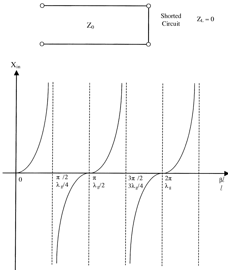
FIGURE 2.10 Transmission line connected to a shorted load.
