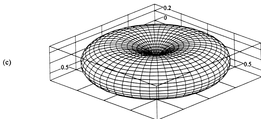
FIGURE 3.14 (a) Thin-wire dipole and monopole antenna. (b) E - and H -plane radiation patterns. (c) Three-dimensional view of the radiation pattern.
