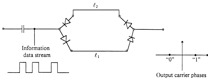
FIGURE 9.8 Biphase switch.
