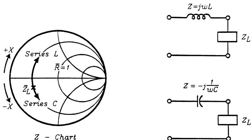
FIGURE 2.35 Adding a series reactance to a load.
