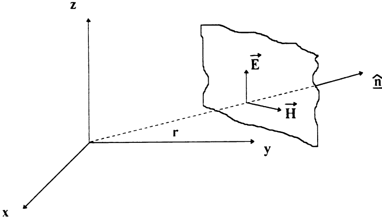
FIGURE 3.5 Plane wave.
