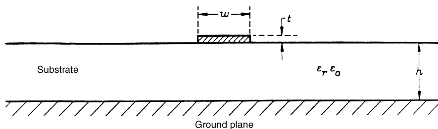
FIGURE 2.23 Microstrip transmission line.
