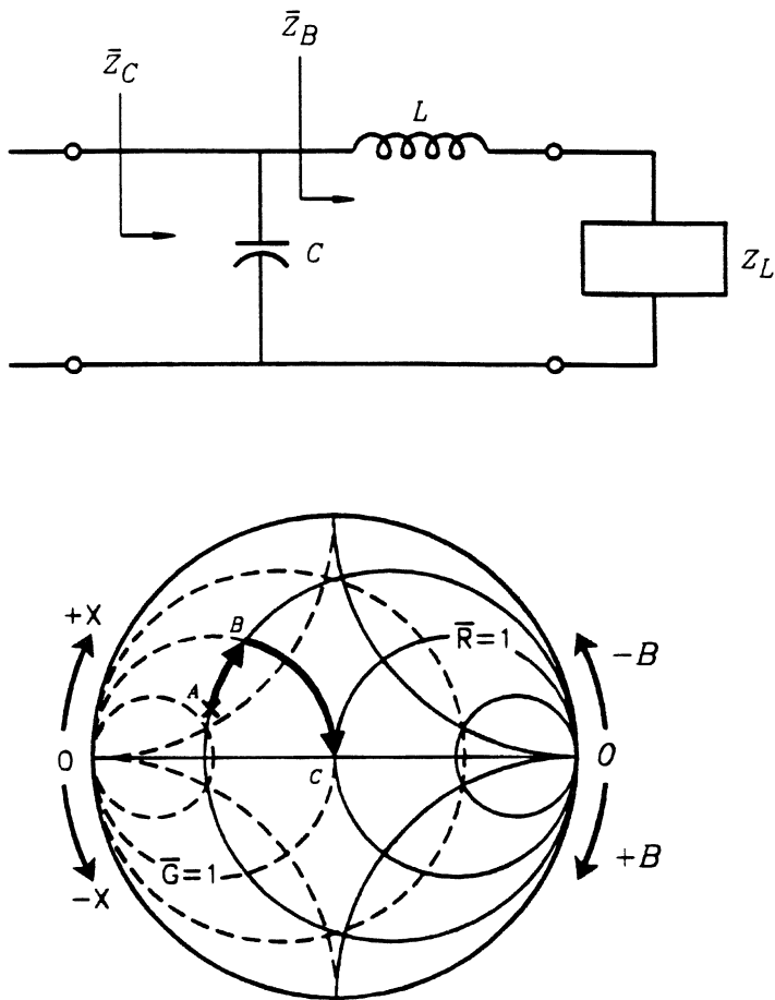
FIGURE 2.37 Using a series L and a shunt C to match Z_L to Z_0 .
