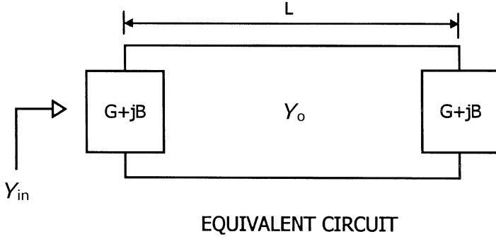
FIGURE 3.26 Transmission line model of a patch antenna.
