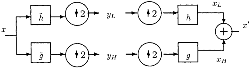
Fig. 4.6 Signal analysis and reconstruction in DWT.
