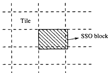
Fig. 10.3 Overlapping tiles.
