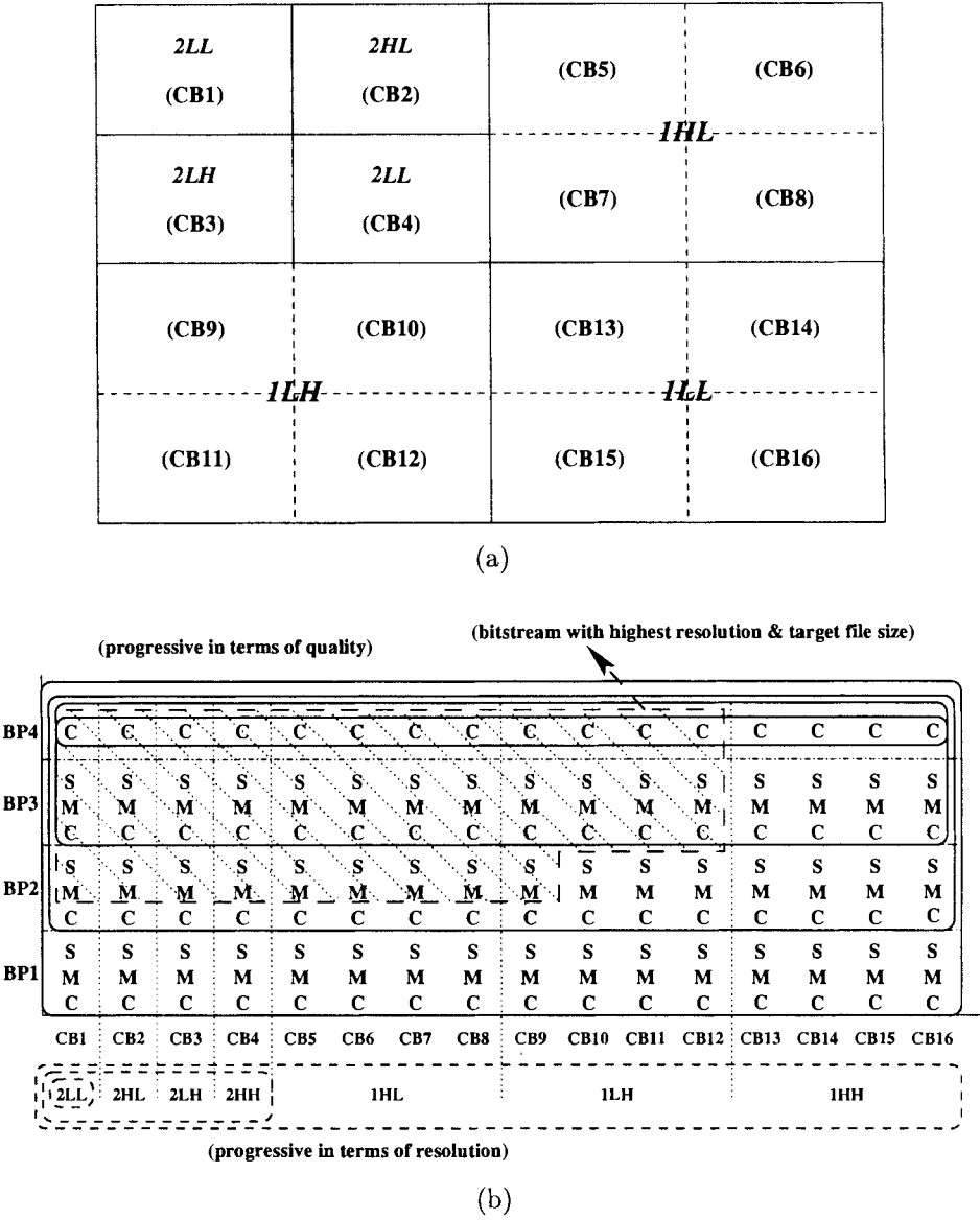
Fig. 7.15 (a) A two-level DWT with 16 code-blocks. (b) Bitstream formations. (Note: the letters S , M , and C in (b) stand for the bitstream generated during significance propagation pass, magnitude refinement pass, and cleanup pass, respectively.)
