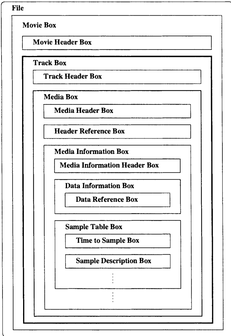
Fig. 10.7 File structure (boxes) of a Motion JPEG2000 movie with one track.
