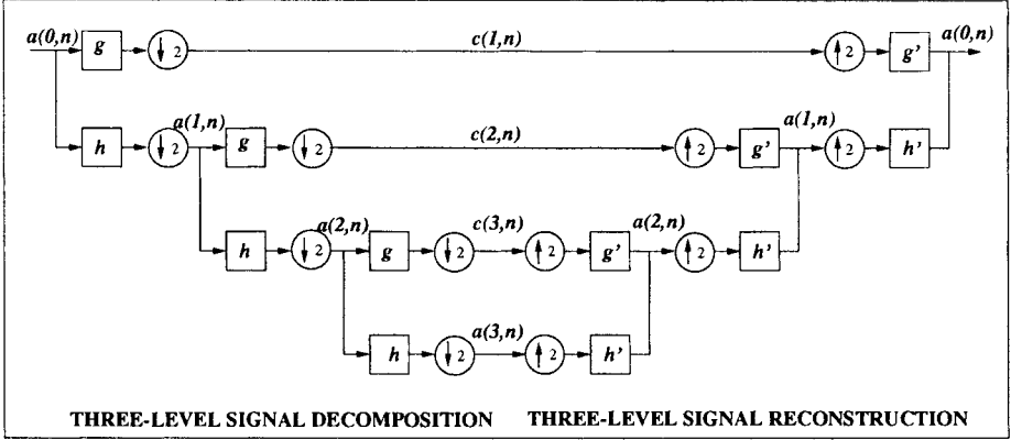
Fig. 4.2 Three-level multiresolution wavelet decomposition and reconstruction of signals using pyramid filter structure.
