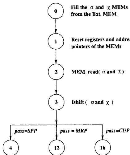
Fig. 9.8 Initial phase for the EBCOT encoder.
