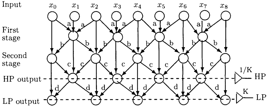
Fig. 5.6 Data dependency diagram of lifting-based DWT with four lifting factors.
