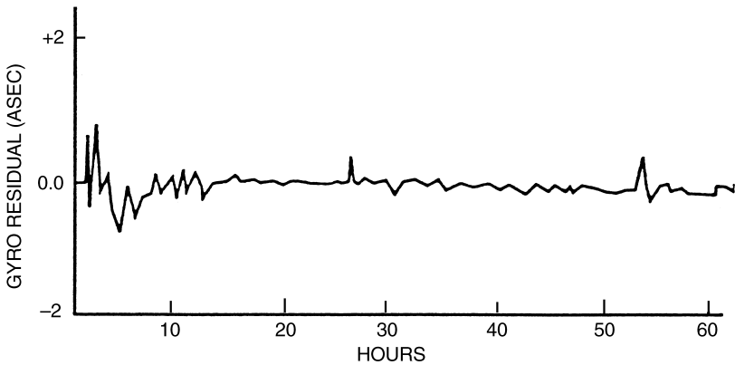
Fig. 5.8 Gyroscope residuals.
