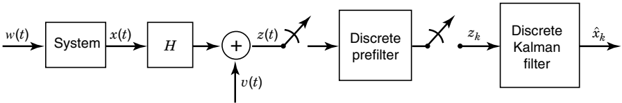
Fig. 7.17 Discrete linear prefilter.
