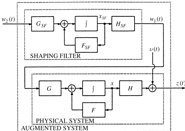
Fig. 3.7 Shaping filter model for nonwhite noise.
