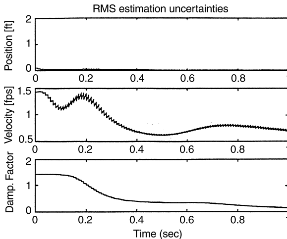
Fig. 5.3 RMS uncertainties in estimates.
