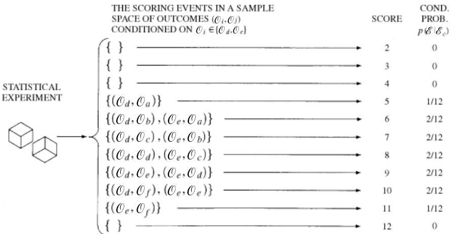
Fig. 3.4 Conditional scoring probabilities for two dice.
