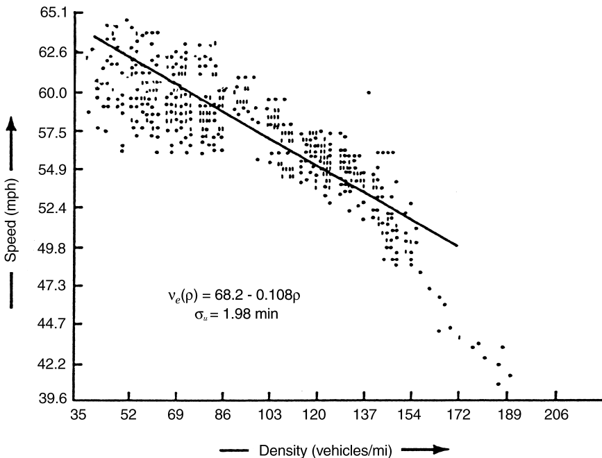
Fig. 5.9 Speed–density relationship.
