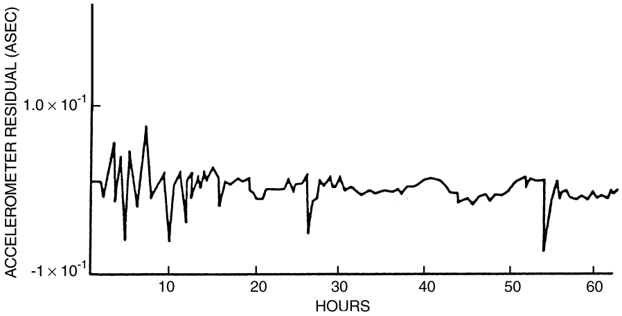
Fig. 5.7 Accelerometer residuals.
