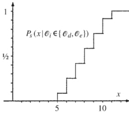
(b) Two dice with conditioning
