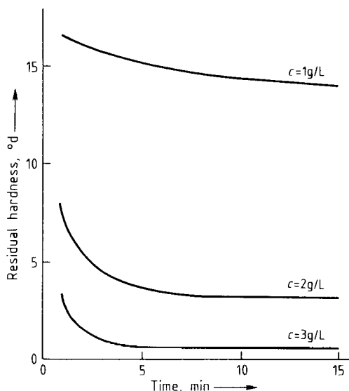
Figure 48. Kinetics of calcium binding to zeolite A [75] Initial hardness: 30 °d (530 ppm \text{CaCO}_3 ); temperature: 25 °C
