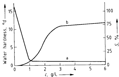
Figure 25. Water softening (a) and soil removal S from cotton soiled with a dust/sebum mixture (b) resulting from a cross-linked water-insoluble polyacrylate at 90 °C [4]
