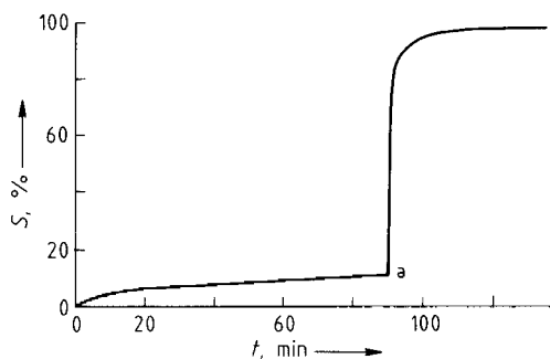
Figure 10. Washing effect S of potassium octanoate (2 wt%) on polyester fibers coated with decanol [19] 0.5 mol/L KCl added after 90 min Prior to a: no formation of liquid-crystalline mixed phase; subsequent to a: formation of liquid-crystalline mixed phase
