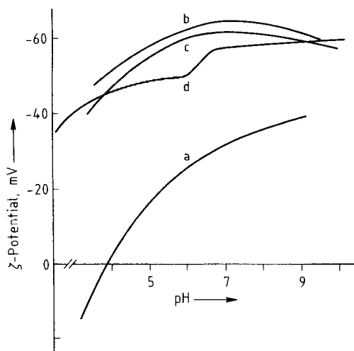
Figure 19. \zeta -Potential of hematite as a function of pH at 25 °C in the presence of sodium chloride (a), sodium triphosphate (b), benzenhexacarboxylic acid (c), and 1-hydroxyethane-1,1-di-phosphonic acid (d) [4] Anion concentration: 2.5 \times 10^{-3} mol/L
