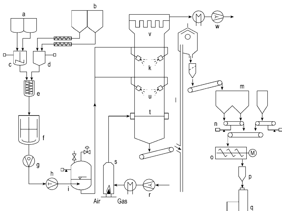
Figure 76. Traditional spray-drying process
