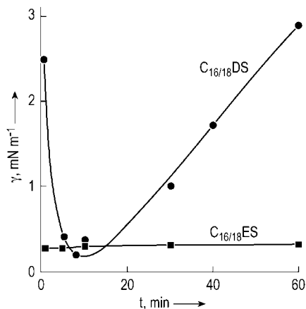
Figure 13. Dynamic interfacial tension \gamma between aqueous phase and mineral oil vs. time t for tallow \alpha -ester sulfonate and tallow di-salt ( T=60^\circ\text{C} ; 0.2 g/l surfactant; 4 g/l \text{Na}_2\text{SO}_4 ) [14]
