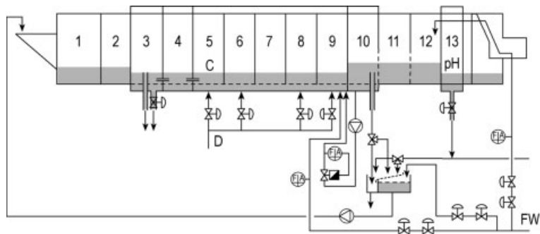
Figure 116. Continuous batch washer
