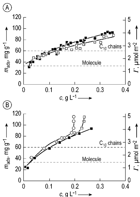
Figure 21. Adsorbed amounts m_{\text{ads}} and surface concentration \Gamma on graphitized carbon black as a function of the surfactant concentration c A) Alkyl monoglycoside (C 10 G 1 ) at 22 °C (■) and 44 °C (□); B) Fatty alcohol ethoxylate (C 10 E 4 ) at 19 °C (■), 30 °C (□), and 45 °C (○)
