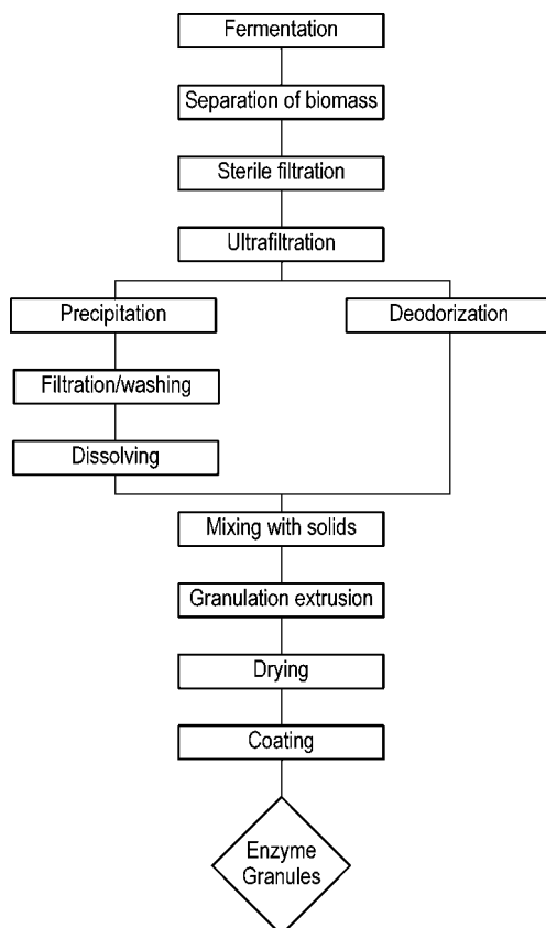
Figure 90. Downstream processing in enzyme production
