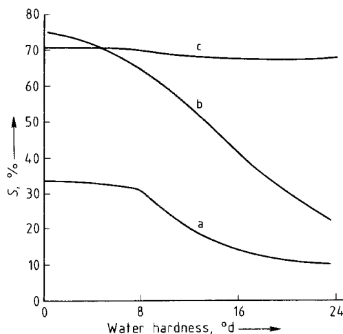
Figure 29. Soil removal S from wool as a function of water hardness at 30 °C [4]
