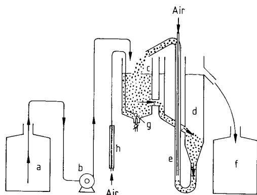
Figure 97. Experimental arrangement for the OECD Confirmatory Test as specified by the German Detergent Law
