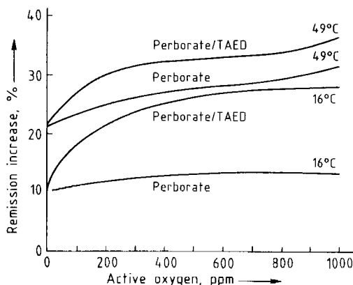
Figure 55. Bleaching effect as a function of bleach concentration [105]
