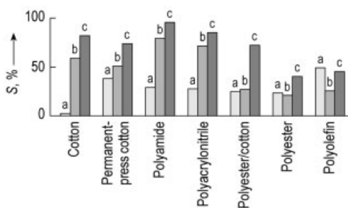
Figure 31. Influence of textile fibers on soil removal S [4]
