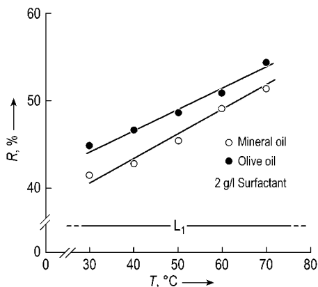
Figure 11. Phase behavior of C_{12}E_9 and detergency
