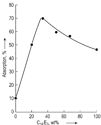
Figure 8. Emulsifying ability (% of absorption) of toluene versus composition of the mixture SDS- C_{16}E_3 (surfactant concentration 0.5 g/L, pH = , T = 298 K)
