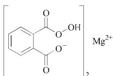
Monoperoxyphthalic acid monomagnesium salt
