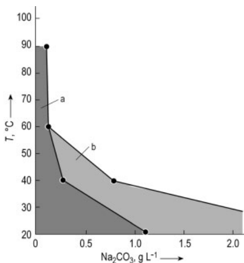
Figure 30. Precipitation inhibition of \text{CaCO}_3 by AC (threshold effect) as a function of temperature and soda ash concentration ( 3.04 \times 10^{-3} \text{ mol/L Ca}^{2+} ) a) 105 mg/L AC; b) 210 mg/L AC
