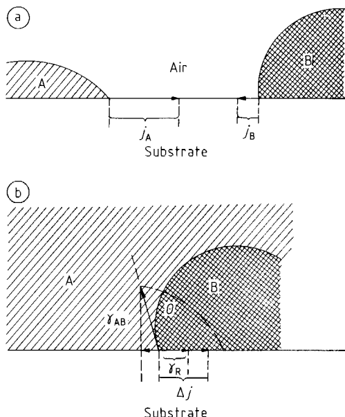
Figure 3. Two liquids on a solid surface
