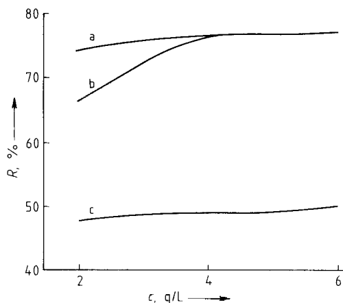
Figure 44. Comparison of soil removal (given as remission R in %) on permanent-press cotton at 0 °C and 90 °C for sodium triphosphate- and sodium carbonate-containing detergents, formulated on the basis of a) 40 % Sodium triphosphate; b) 20 % Sodium triphosphate + 20 % sodium sulfate; c) 40 % Sodium carbonate
