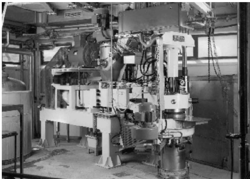
Figure 91. Extrusion process [205]
