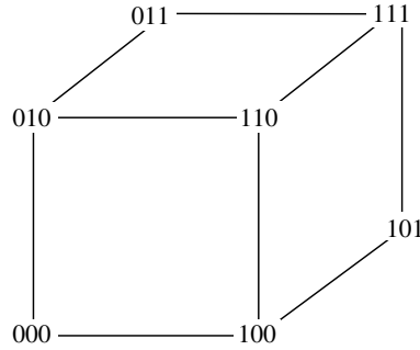
Figure 1.4.1. Three-dimensional binary space.
