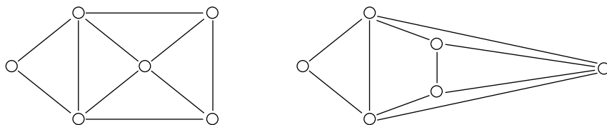
Figure 5.4.9. Isomorphic plane graphs with nonisomorphic duals.
