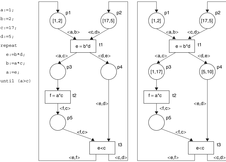
Figure 3.4 Modelling of digital behaviour using Pr/T nets
