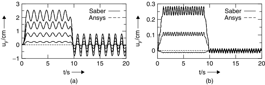
Figure 6.11 Simulation results for the deflection at x = 0.25l, 0.51, 0.75l and 1.0l of a cantilever beam with (a) and without (b) an additional support
