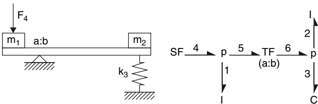
Figure 3.6 Bond graph of a simple mechanical system
