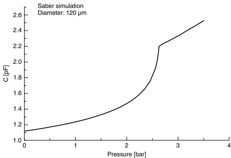
Figure 8.10 Capacitance against pressure for an element diameter of 120 \mu m
