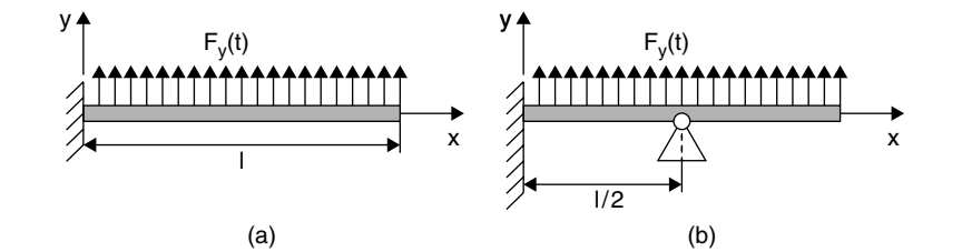
Figure 6.10 Cantilever beam with (a) and without (b) an additional support
