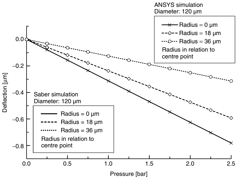
Figure 8.6 Mechanical deflection of the upper plate (diameter 120\text{ }\mu\text{m} ) at various points on the radius. Comparison of the ANSYS FE simulator with the Saber circuit simulation
