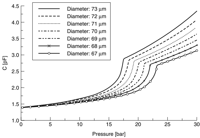
Figure 8.15 Parametric Saber simulations for the variation of the diameter of the pressure element. The plate thickness is fixed at 1.7 \mu\text{m}
