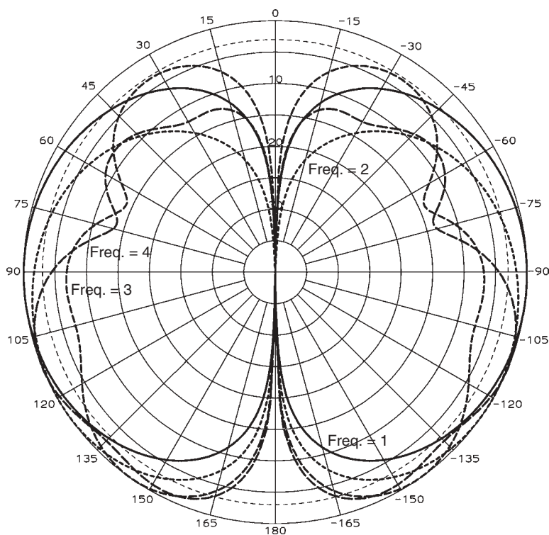
FIGURE 5-33 Elevation pattern of a 60° disccone antenna at normalized frequencies = 1, 2, 3, and 4.
