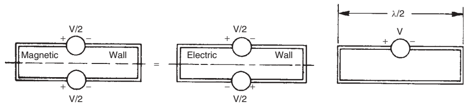
FIGURE 5-30 Folded dipole analysis modes.
