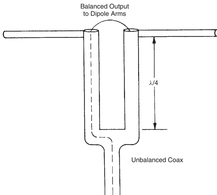
FIGURE 5-36 Folded balun.
