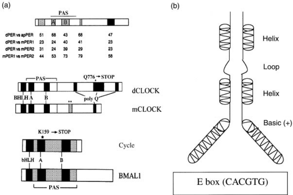
Figure 3.5. Several clock proteins found in both Drosophila and mammals contain PAS domains. (a) Alignment of similar PAS proteins from mammals, fruitflies, and silkworms. The PAS region, which can mediate protein/protein interactions, contains short regions that are almost direct copies of each other [(a) and (b)]. PER also contains other regions that are conserved in mouse (m) and silkworm (ap) PER (% identities shown). CLOCK and CYCLE contain basic helix-loop-helix (bHLH) regions that bind to DNA. CLOCK also contains a polyglutamine-rich (polyQ) C terminus, which is likely to activate RNA polymerase at the promoter to which the CLOCK/CYC heterodimer binds. The mutations in the Drosophila and mouse Clk genes are found in a polyglutamine region, while the Drosophila cyc 0 mutation occurs in the PAS region. [Top, reprinted from Shearman et al. (1997): Two period homologs: circadian expression and photic regulation in the suprachiasmatic nuclei. Neuron 19: 1261–1269, copyright (1997) with permission from Elsevier Science. Middle, reprinted from Allada et al. (1998), copyright (1998) with permission from Elsevier Science. Bottom, reprinted from Rutilla et al. (1998): CYCLE is a second bHLH-PAS clock protein essential for circadian rhythmicity and transcription of Drosophila period and timeless . Cell 93: 805–813, copyright (1998) with permission from Elsevier Science.] (b) bHLH transcription factors generally bind as dimers consisting of two different peptides (e.g., CLK and CYC). The dimers are formed by protein-protein interactions involving the two pairs of alpha helices, while E-box elements in the DNA are bound by the basic regions of the heterodimer.
