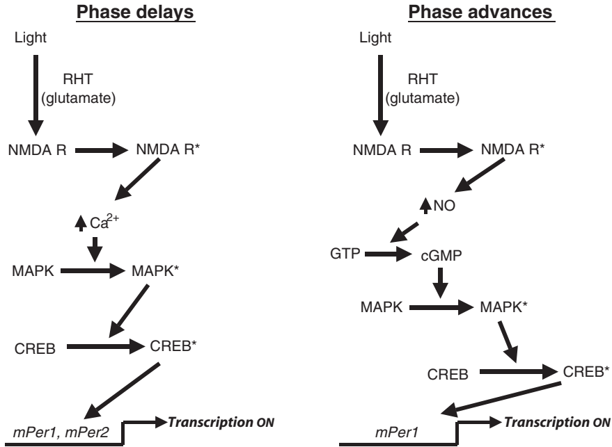
Figure 5.5. Molecular pathway for either phase advances or phase delays in response to a light pulse during the subjective night. During a phase delay, the RHT releases glutamate, which is bound by the NMDA receptor. The activated receptor (indicated by the asterisk) leads to an increase in calcium. Through a series of proteins not shown here, the calcium leads to phosphorylation and activation of MAP kinase (asterisk). Active MAPK leads to activation of the transcription factor CREB by phosphorylation (asterisk). Active CREB then induces transcription of the circadian clock genes, Period-1 and Period-2 . A light pulse given at the latter part of the subjective night also results in activation of the NMDA receptor. In contrast, though, at this time of night, the active NMDA receptor leads to an increase in nitric oxide (NO). NO activates an enzyme, guanylyl cyclase, which converts GTP into cyclic GMP. The rise in cGMP levels also results in activated MAPK and eventually activated CREB. However, transcription of only Period-1 is induced. The reason underlying the dichotomy of responses is not clear, but presumably there are additional factors necessary for transcriptional activation that are available in the early night, but not in the late night.
