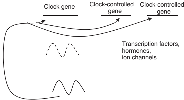
Figure 1.6. Control of downstream genes by the clock. A molecular clock (such as the one shown in Fig. 1.7) can regulate the output pathway by driving cyclic expression of downstream genes. One mechanism by which this occurs is shown here. While regulating its own transcription, the clock protein also regulates the transcription of downstream genes at a specific time of day. This leads to rhythmic expression of those genes.
