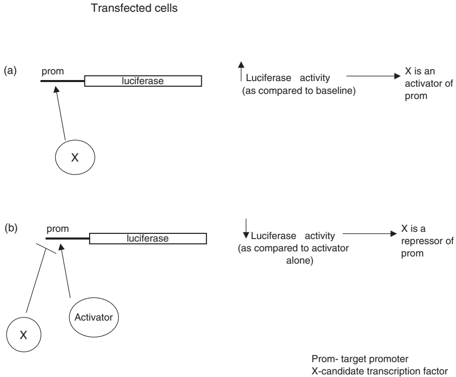
Figure 2.2. Use of cell culture assays to determine the effects of candidate genes on transcription. As described in the text, the promoter of the putative target gene is fused to a reporter and transfected into cultured cells. The reporter shown here is the firefly luciferase protein whose activity can be reliably and easily quantified in a luminometer. Luciferase activity is assayed in cells cotransfected with the candidate transcription factor as well as in control cells (these may be cotransfected with a transcription factor that is not relevant for this process). The level of luciferase activity in control cells serves as a baseline. If the candidate factor is suspected of being a repressor, its effects are best studied under conditions where the target promoter is actively transcribed. Multiple transcription factors may be transfected to determine how the presence of one affects the activity of the other.
