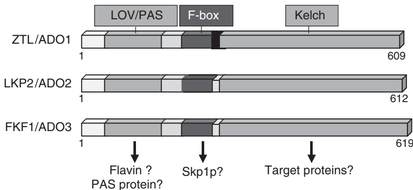
Figure 8.6. Domain structure of the ZTL family of proteins. Schematic alignment of ZTL/ADO1 with paralogs LKP2/ADO2 and FKF1/ADO3 . The PAS-like LOV domain, the F box and six kelch repeats are shown, together with their potential interaction targets.
