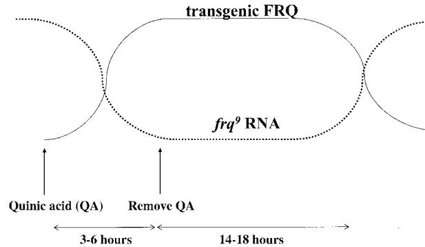
Figure 7.4. Time course of feedback inhibition. frq was expressed under control of a quinic acid-inducible promoter in a frq 9 background. The time course of feedback on frq 9 RNA was examined by inducing expression of transgenic frq with quinic acid and monitoring levels of the endogenous frq 9 transcript (dotted line). As indicated, negative feedback is achieved rapidly and stays in effect for several hours after the quinic acid is removed. The extended period of feedback correlates with the amount of time the transgenic FRQ protein (solid line) stays around. [Adapted from Mellow et al. (1997).]
