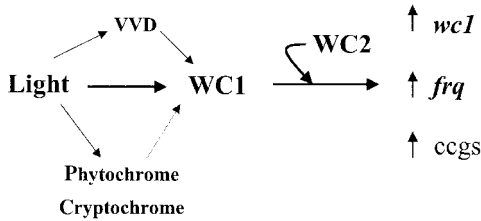
Figure 7.8. Resetting of the clock in response to light. The circadian photoreceptor is the product of the wc-1 gene, although VVD, and possibly phytochrome and cryptochrome, play a modulatory role. WC-1 recruits its partner, WC-2, and activates transcription of frq . [Adapted from Froehlich et al. (2002).] Since WC-1 itself and other clock-controlled genes (ccgs) are also upregulated by light, it is shown to activate transcription of these genes also.
