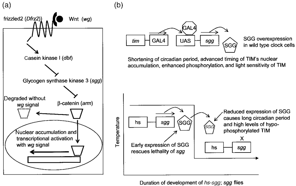
Figure 3.11. The dbt and sgg protein kinases have roles in both the Wnt ( wg ) signaling pathway and the circadian clock. (a) Model for the role of casein kinase I and sgg in the wg pathway. The role for casein kinase I has been shown in Xenopus , while the role for sgg has been shown in many systems (including Drosophila ). Casein kinase I activates the wg pathway by repressing SGG, which otherwise causes \beta -catenin to be degraded. (b) A role for sgg in the Drosophila circadian clock has been demonstrated by overexpressing SGG in tim expressing cells (top), or by lowering SGG protein levels in the adult (bottom). The UAS-GAL4 system was used to overexpress SGG specifically in tim cells. tim is the promoter of the timeless gene, GAL4 is a yeast transcription factor, and UAS is the promoter that GAL4 binds and activates. Bottom, the lethality associated with the sgg mutant was rescued by expressing a sgg transgene, under control of a heat shock promoter, during development. By decreasing the temperature in adults, the effects of reduced sgg expression on circadian rhythms were determined. The heat shock promoter ( hs ) activates sgg at elevated temperatures and is turned off at lower temperatures.
