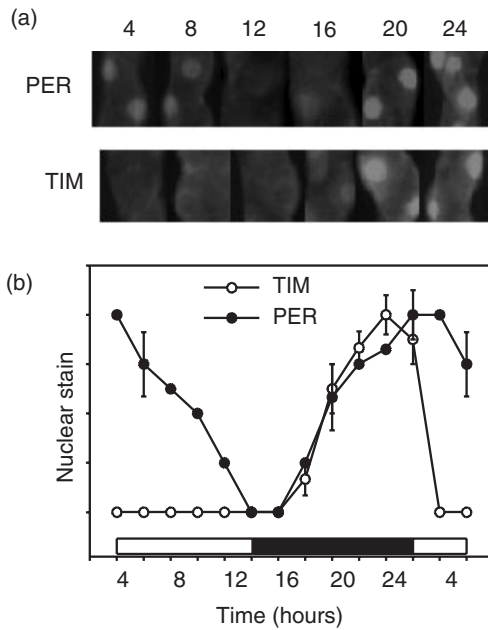
Figure 9.2. Expression of clock proteins PER and TIM in Malpighian (excretory) tubules of D. melanogaster : (a) fragments of tubules showing nuclear location of both proteins; (b) quantification of the intensity of PER and TIM signal [modified from Ivanczenko et al. (2001)].
