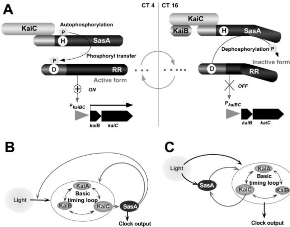
Figure 6.17. Models for SasA function in the circadian system. (a) A model for the function of the SasA-KaiC complex in kaiBC expression. In the early morning, when total KaiC abundance is low, KaiC may bind SasA, stimulating its autophosphorylation and thereby activating its cognate response regulator (RR) through phosphoryl transfer from His (H) to Asp (D). Activated RR is proposed to directly or indirectly activate expression of kaiBC genes from P_{kaiBC} (left). As the KaiBC concentration rises in the evening, the KaiC-SasA complex may bind additional KaiC or KaiB to form a larger complex(es), which reduces SasA autophosphorylation. SasA may then act as a phosphoryl protein phosphatase, inhibiting RR-mediated stimulation of P_{kaiBC} activity (right). (b,c) SasA may function as the first output of the clock to regulate downstream clock-controlled processes (b) or as an element of redundant input pathways (c). In both models, SasA and clock protein KaiC form an outer feedback loop to amplify the KaiABC-based basic timing process by modulating kai gene expression as depicted in (a). In model (b), KaiC-SasA complex controls its cognate response regulator and thereby directly controls downstream gene expression. In model (c), SasA controls the robustness of the circadian oscillation in a light-dependent manner, although SasA is not essential to entrain the clock. SasA may sense light signals directly or indirectly, and the binding of SasA to KaiC would alter SasA's enzymatic activity. [Reprinted from Iwasaki et al. (2000) with permission from Elsevier Science.]
