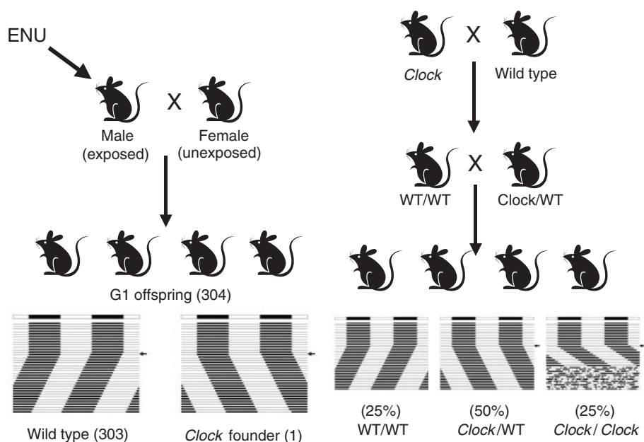
Figure 5.7. Mutation strategy used to generate Clock mutant mice. Male mice were exposed to the mutagen, ENU. These mice were then bred to unexposed female mice, and the offspring (G1) were screened for disorders of circadian locomotor activity rhythms. The vast majority of mice had a normal period length of 23.7 hours, but one mouse had a period of approximately 25 hours. Schematics of the locomotor activity records are shown. The arrow indicates the point where the mice are moved from a light–dark cycle to constant darkness. The long-period mouse was bred to wild-type females and the offspring were screened for locomotor periods. Approximately half of these offspring had wild-type periods, and half had the long-period phenotype, indicating that the mutation was a single-gene autosomal dominant. The long-period phenotype animals were interbred to generate homozygous animals. The offspring fell into three groups phenotypically with respect to locomotor activity period: wild type (25%), parental (50%), and an even longer period of approximately 28 hours (25%). These represented homozygous wild type, heterozygotes, and homozygous Clock mutation, respectively. Such data indicates that the Clock gene is a single, semidominant gene. Notably, the homozygous Clock mutant animals degenerate into arrhythmicity after ~2 weeks in constant darkness.
