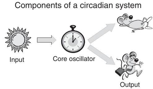
Figure 5.1. Schematic of the three-part model of a circadian system. At the heart of the system is the central oscillator. This is the main timekeeper of the system. The central oscillator is under the influence of input factors. Input is often from environmental factors, such as the light–dark cycle. The central oscillator imposes a rhythm on various aspects of physiology via output pathways. Output can represent both direct neuronal connections and secreted factors.
