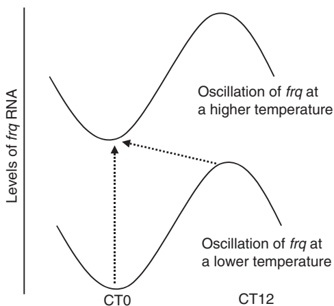
Figure 7.10. Resetting of the circadian clock by temperature. At higher temperature FRQ oscillates around a higher level, such that even the trough levels at 28°C are higher than peak levels at 21°C. It follows then that a temperature shift up at all times of day resets the clock to the trough timepoint (CT0). A temperature shift down (not shown) always resets to the peak timepoint (CT12). [Adapted from Loros and Dunlap (2001).]
