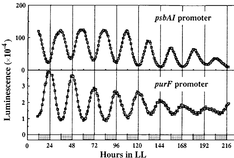
Figure 6.6. Promoter activity of class 1 and class 2 genes as assayed with the luxAB luminescent reporter. The upper trace is from the class 1 gene psbAI ; the bottom trace is from the class 2 gene purF . Data were recorded in constant light (LL), but the times of expected or subjective night are shown by the gray bars along the abscissa. [Reprinted from Johnson and Golden (1999) with permission from the Annual Review of Microbiology , Volume 53. © 1999 by Annual Reviews, www.annualreviews.org.]
