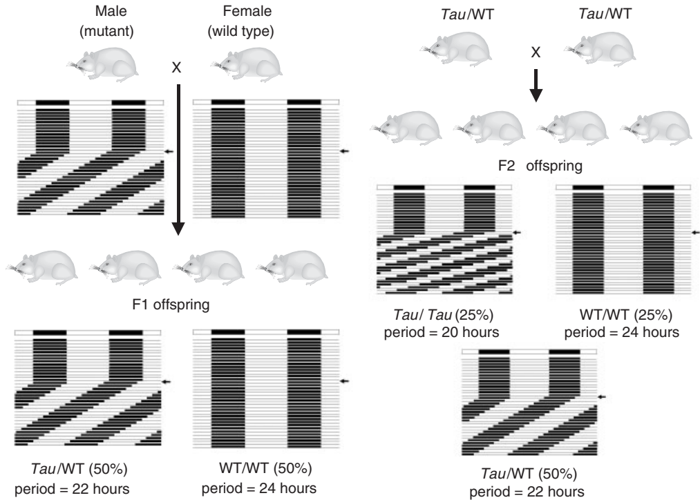
Figure 5.10. Isolation of the tau mutant hamster line. One male with a locomotor period of 22 hours was isolated as a spontaneously generated mutant in a group of Syrian golden hamsters. Note that the normal period for hamsters is 24 hours, so that the period stays the same even in constant darkness. Mating of this mutant hamster male, called tau , to wild-type females yielded a 50:50 ratio of short and wild-type period phenotypes, irregardless of sex. Such a result indicates that the tau mutation represents a single, dominant, autosomal gene. Mating of two heterozygote animals generated three phenotypes with respect to locomotor periods: 20, 22, and 24 hours. These were in a ratio of 1:2:1 indicative of classic Mendelian inheritance of a single semidominant gene.
