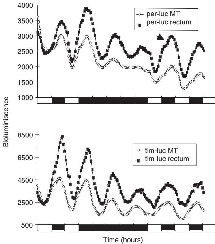
Figure 9.3. Real-time expression of per-luc and tim-luc reporter genes in individual body tissues. Bioluminescence emanating from individual Malpighian tubules (MT) or rectal tissues (rectum) was recorded hourly. The upper panel shows the average plot of per-luc expressing tissues, the lower panel shows the average plot of tim-luc expressing tissues. Black and white bars indicate 12-hour periods when the lights were on and off, respectively; shaded bars indicate dark periods, when the lights would be on in LD. An increase in the amplitude of cycling on reexposure of tissues to LD (arrow) indicates that the two peripheral oscillators are directly light-responsive. [Reprinted from Current Biology 10, Giebultowicz et al., Transplanted Drosophila excretory tubules maintain circadian clock cycling out of phase with the host, pp 107–110, [copyright (2000) with permission from Elsevier Science.]
