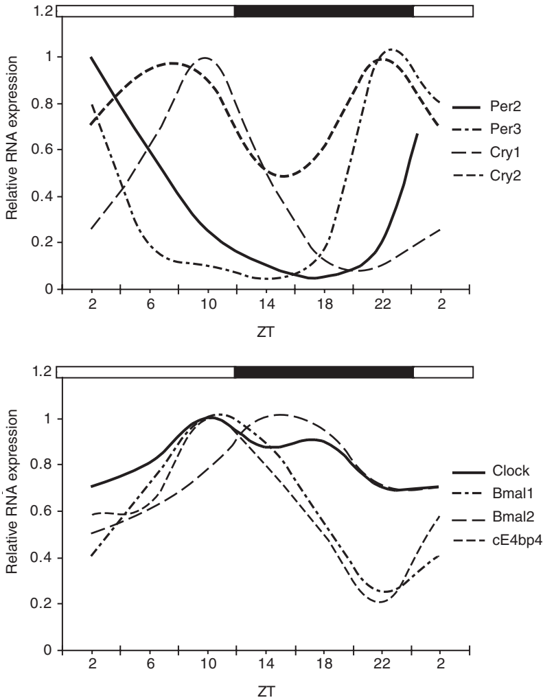
Figure 4.2. Summary of cycling clock genes in the chicken. mRNA levels for each gene are plotted versus time of day [Zeitgeber time (ZT)] in an L:D cycle of 12:12. Open bars at the top represent daytime, starting at ZT0 (lights on); and dark bars represent nighttime, starting at ZT12 (lights off). Levels of RNA do not reflect relative expression of the clock genes to each other, but rather how they change during the day.
