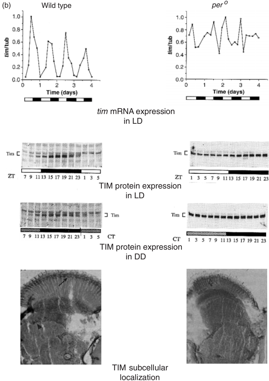
Figure 3.6. Continued. (b) tim expression in wild-type (left) and per 0 mutant (right) heads. Detection was accomplished as in (a). The per 0 mutation eliminates the circadian oscillations of tim gene products and the nuclear accumulation of TIM, but it does not eliminate LD-driven cycles of TIM protein or generally depress TIM protein levels. [Top, reprinted with permission from Sehgal et al. (1995): Rhythmic expression of timeless : A basis for promoting circadian cycles in period gene autoregulation. Science 270 : 808–810, copyright (1995) American Association for the Advancement of Science. Middle, reprinted by permission from Zeng et al. (1996): A light-entrainment mechanism for the Drosophila circadian clock. Nature 380 : 129–135, copyright (1996) Macmillan Publishers Ltd. Bottom, reprinted from Myers et al. (1996): Light-induced degradation of TIMELESS and entrainment of the Drosophila circadian clock. Science 271 : 1736–1740, copyright (1996) American Association for the Advancement of Science.]
