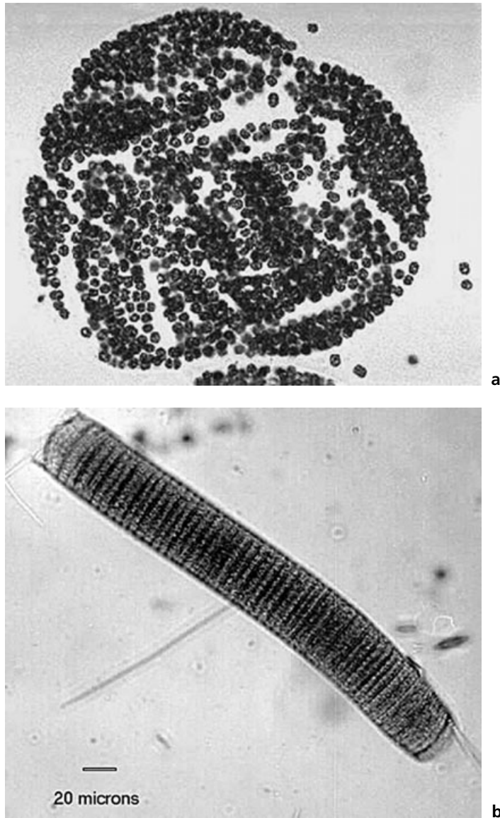
Figure 6.2. (a) Colony of Microcystis sp. Cyanobacteria are quite small and usually unicellular, although they often grow in colonies large enough to see. [Picture courtesy of Isao Inouye (University of Tsukuba), Mark Schneegurt (Wichita State University), and Cyanosite ( www.cyanosite.bio.purdue.edu ).] (b) Oscillatoria filament. Many cyanobacterial species are filamentous. [Pictures courtesy of Roger Burks (University of California at Riverside), Mark Schneegurt (Wichita State University), and Cyanosite ( www.cyanosite.bio.purdue.edu ).]
