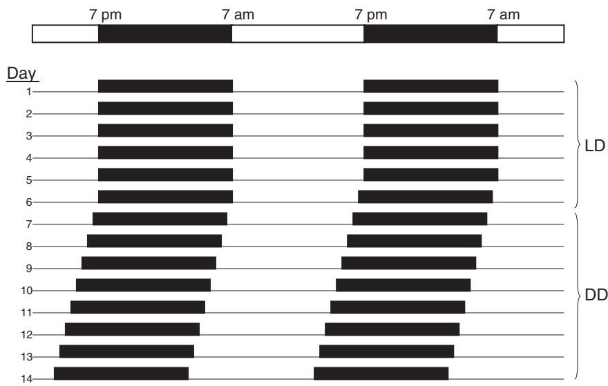
Figure 5.2. Schematic of activity rhythms of a mouse as measured by running on a wheel. The bar at the top shows when lights are on (light bar) and off (dark bar). As indicated, the lights come on at 7 am and turn off at 7 pm. This is a standard 12-hour light–dark (LD) cycle. Activity of the mouse is indicated by the dark bars for each day. Note that the data are double-plotted; that is, day 1 is shown on the first line, followed by day 2. The second line starts with day 2 and ends with day 3. This allows a comparison of days both horizontally and vertically. At the end of day 6, the animal is shifted from an LD cycle to constant darkness (DD). This is called freerunning conditions . Note that the periods of activity shift slightly in constant darkness. This is due to the fact that the endogenous periodicity of most mouse strains is slightly shorter than 24 hours.
