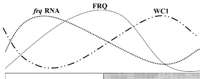
Figure 7.6. Molecular oscillations of frq and WC. WC-1 and frq are the two known oscillating components of the Neurospora clock. While frq RNA as well as protein cycle, WC-1 cycles only at the level of the protein with a phase different from that of FRQ. The oscillations are shown relative to the light-dark cycle (depicted by the bars at the bottom).
