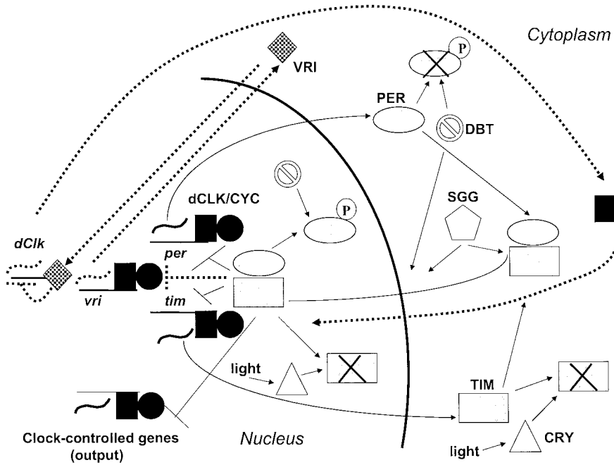
Figure 3.18. A molecular model for the circadian clock in Drosophila . The rhythmic accumulation of PER and TIM proteins results in the formation of a PER/TIM complex, which negatively regulates two feedback loops involving dCLK/CYC. In one of these loops (solid lines) dCLK/CYC positively regulate per and tim transcription, and in the other loop (dotted lines) dCLK/CYC negatively regulates dClk mRNA by activating vri expression. Light, CRY, and SGG regulate a lag in nuclear feedback by PER/TIM through their effects on TIM, and light entrains the oscillator through CRY-mediated degradation of TIM. DBT regulates the initiation and termination of nuclear feedback through its effects on PER. In addition to driving transcription of per and tim , dCLK/CYC is thought to activate transcription of numerous clock-controlled genes, which translate the rhythm of the circadian oscillator into circadian outputs of biochemistry and cell physiology.
