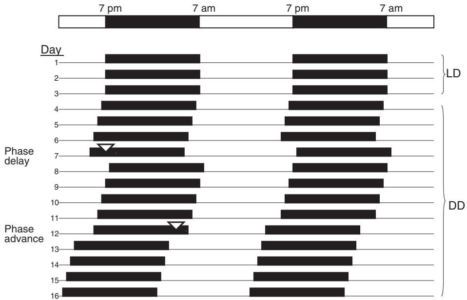
Figure 5.4. Schematic of activity rhythms of a mouse showing effects of a light pulse to generate either a phase delay or a phase advance. The mouse is first entrained to a LD cycle and then allowed to freerun in constant darkness. When a light pulse (indicated by the upside-down triangle) is administered at the beginning of the night, a phase delay occurs as indicated by the delay in the active period during the next night. The overall period stays the same, however. Similarly, a light pulse administered late in the subjective night results in a phase advance as indicated by the earlier onset of activity. Again, note that the overall period stays the same. Often at the onset of a phase change, there is a transient period of near arrhythmicity, which is not illustrated here. Presumably, this occurs while the clock is being “reset.”
