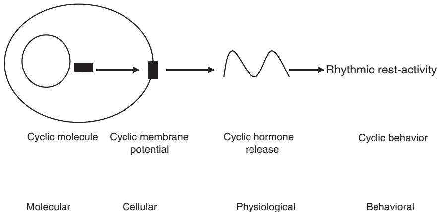
Figure 1.7. Control of an overt, behavioral rhythm by the clock. A simple model is shown in which the clock drives rhythmic expression of a gene that regulates membrane potential. Cycling membrane potential results in rhythmic release of a secreted factor that has an effect on levels of rest and activity.
