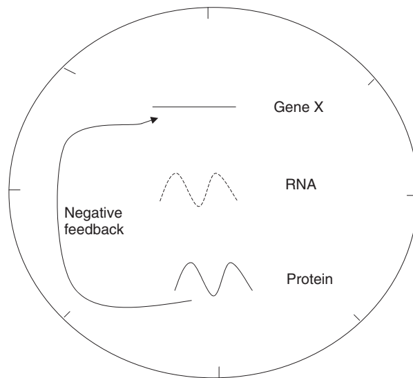
Figure 1.5. The basic model for a 24-hour oscillator. The model is based on work done in many different species ranging from cyanobacteria to mammals and consists of an autoregulatory feedback loop in which a clock gene encodes cycling RNA and protein, and the protein negatively regulates synthesis of its own mRNA. The loop takes ~24 hours to complete (shown within a 24-hour clock).
