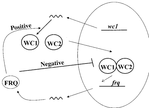
Figure 7.7. The molecular clock in Neurospora . FRQ negatively regulates its transcription by blocking activity of the WC complex in the nucleus. At the same time it positively regulates expression of the WC-1 protein, resulting in an interlocked loop. [Adapted from Lee et al. (2000).]
