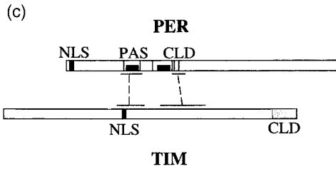
Figure 3.6. Continued. (c) The mutual regulation of per and tim involves protein/protein interactions between PER and TIM. Both proteins contain putative nuclear localization signals (NLSs) thought to mediate nuclear import. In addition, both proteins contain cytoplasmic localization domains (CLDs), which retain PER (or TIM) in the cytoplasm unless the other is coexpressed. PER also contains the previously described PAS region [black bars denote (a) and (b) repeats]. Interactions between PER and TIM occur as shown. [Reprinted from Saez and Young (1996), copyright (1996) with permission from Elsevier Science.]
