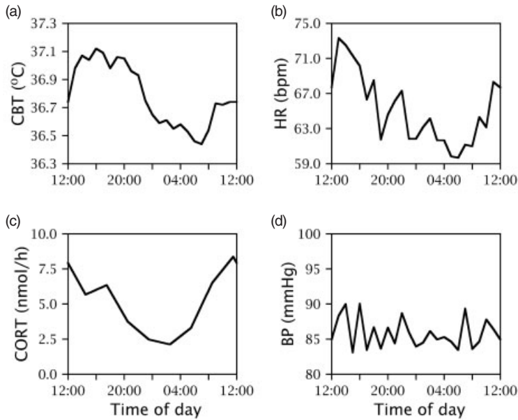
Figure 11.1. Endogenous circadian rhythms. The figure shows endogenous temporal profiles of core body temperature (upper left-hand panel), cortisol excretion (lower left-hand panel), heart rate (upper right-hand panel), and mean arterial blood pressure (lower right-hand panel), recorded during constant routine (averaged over n = 6 healthy subjects). Body temperature (CBT) was measured every 2 minutes by means of a rectal probe [hourly averages are plotted in panel (a)]; cortisol excretion (CORT) was derived from urine samples taken every 3 hours; heart rate (HR) and blood pressure (BP) were measured hourly with an oscillometric monitor; and mean arterial pressure (MAP) was calculated as diastolic BP plus one-third of the difference between diastolic and systolic BP. Endogenous circadian rhythmicity is clear in CBT, CORT, and HR. There are fluctuations over time also in BP, which may or may not reflect ultradian rhythms, but there is no endogenous circadian rhythmicity in BP.
