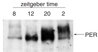
Figure 2.4. Temporal analysis of protein expression by western blot analysis. The data shown are for the Drosophila period protein (PER). Adult Drosophila were entrained to a light–dark cycle for several days, after which they were collected at the timepoints indicated [in zeitgeber time (ZT)]. Heads were isolated and homogenized to prepare protein extracts. The extracts were run on SDS polyacrylamide gels, which separate denatured proteins based on their size. The proteins were then transferred to membranes (“western-blotted”) and probed with an anti-PER antibody. The antibody binds to the membrane only where PER antigen is present, and the presence of the bound antibody is detected indirectly by coupling an enzyme, which emits a luminescent signal assayed through autoradiography. As evident from the figure, levels of PER cycle over the course of the day. The phosphorylation state of PER also cycles. The high-molecular-weight bands seen at ZT2 represent phosphorylated forms of PER.
