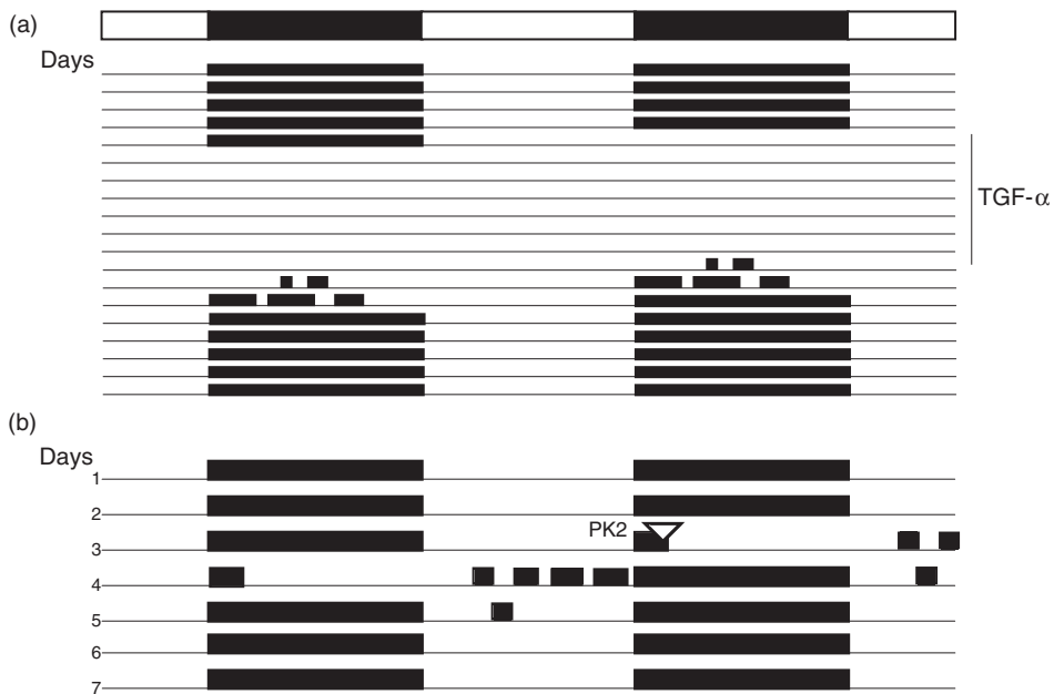
Figure 5.13. TGF \alpha and prokineticin 2 both suppress locomotor activity. (a) Hamsters were entrained to a 14–10 light:dark cycle for two weeks and then moved to constant darkness. At the indicated time, TGF \alpha was constantly infused into the third ventricle through an intraventricular cannula. Locomotor activity almost immediately stopped, and very little activity occurred while infusion was being carried out. When the infusion was stopped, the animals were active again. (b) Similarly, rats subjected to recombinant human PK2 injection into the ventricular system almost immediately stop running on wheels. Interestingly, there is abnormal activity observed the day after the PK2 injection.
