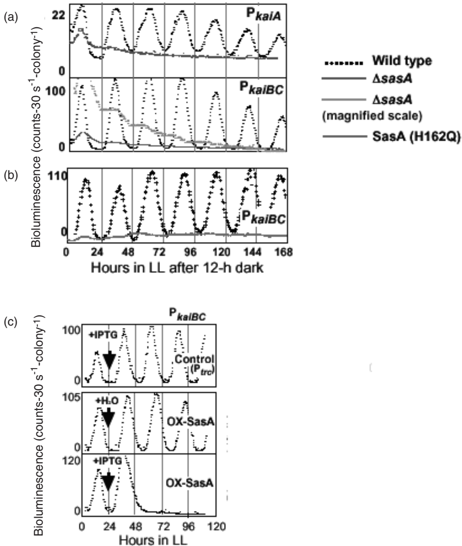
Figure 6.14. Disruption and overexpression of sasA affects circadian kai gene expression. (a) Low amplitude bioluminescence rhythms seen in the absence of sasA . Bioluminescence rhythms of the PkaiA and PkaiBC reporters, in both wild type and sasA lacking backgrounds, are shown. For clarity, the bioluminescence profile of the PkaiBC reporter in the strain lacking sasA is also shown in magnified scale (both solid lines in this panel correspond to the profile in a sasA null). (b) The kaiBC expression profile in the H162Q mutant, in which the putative autophosphorylation residue in sasA was substituted with Gln. Bioluminescence from wild-type (....) and mutant lines (solid line) was monitored in LL. (c) Continuous overexpression of sasA disrupts circadian rhythms. Bioluminescence of a PkaiBC reporter in a Ptrc vector or a Ptrc::sasA (for overexpression of SasA ) construct was monitored. Cells were grown on agar plates in LL, exposed to darkness to synchronize their clocks, returned to LL and treated with IPTG or water at hour 24 after dark exposure (arrows indicate addition of water or IPTG).
