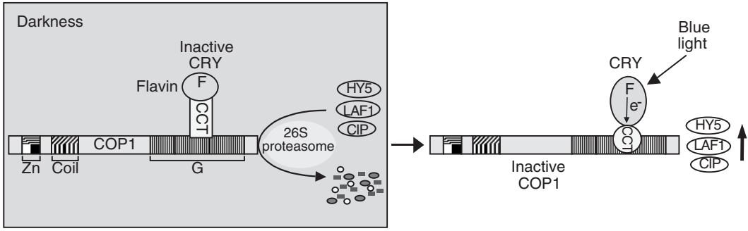
Figure 8.4. A hypothetical model of cryptochrome signaling. Arabidopsis cryptochromes contain a conserved N -terminal flavin-binding domain and a distinct C-terminal extension (CCT). The CCT interacts with the C-terminal WD-40 repeat domain of COP1. In darkness, COP1 is active and promotes the degradation of different interacting proteins via a 26S proteasome-mediated process. CRY blue-light activation may cause a change in the redox state and/or the conformation of the CCT. The activated CCT interacts with COP1, abrogating the COP1 degradation of different substrates (HY5, LAF1, CIP).
