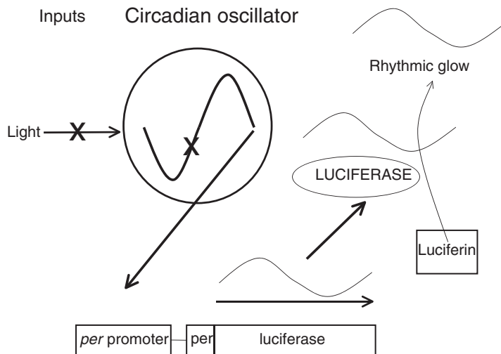
Figure 3.13. Design of a genetic screen for mutants that affect the circadian oscillation of per transcription. Circadian oscillations of luciferase transcription are driven by the per promoter, which responds to clock-driven alterations of dCLK/CYC-dependent activation. The resulting circadian oscillations of luciferase activity produce a rhythmic glow in flies fed luciferin (the substrate for luciferase). The glow can be measured and analyzed in single flies, just as locomotor activity can be (Fig. 3.1). A mutation (X) that affects the input pathway or the oscillator mechanism is predicted to alter the circadian glow rhythm.
