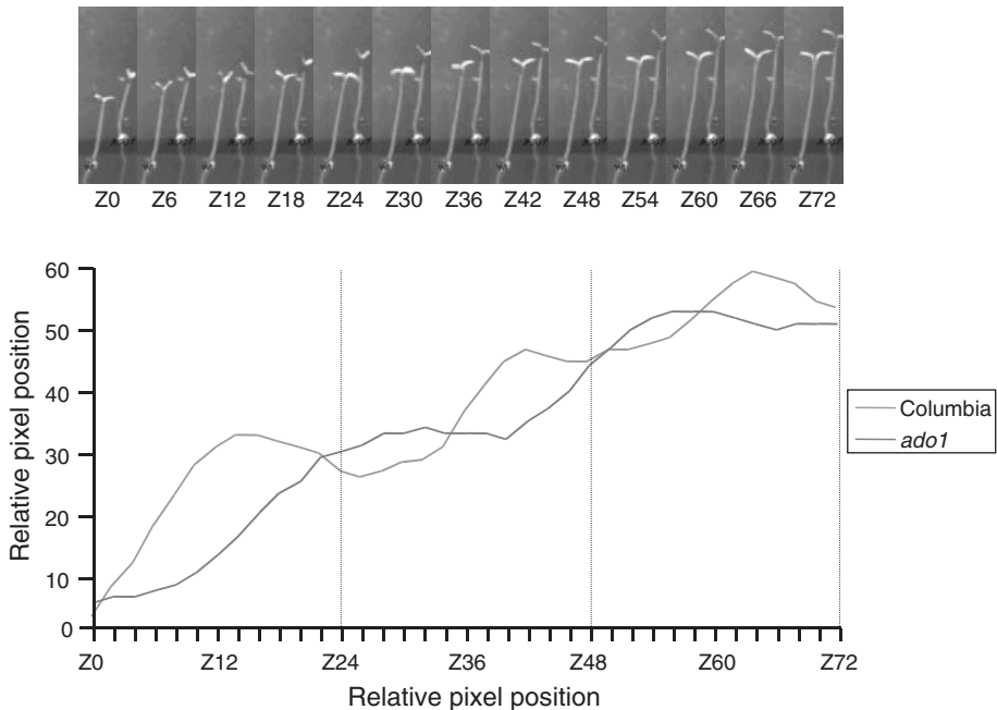
Figure 8.5. Cotyledon tip movement in the ado1 mutant. Cotyledon movement was recorded for wild-type (Columbia) (left part of each panel) and mutant ( ado1 ) (right part of each panel) seedlings grown under a 12-hour photoperiod and then transferred to constant white light. The position in pixels of one cotyledon tip per seedling for 72 hours was recorded. The periodicity of cotyledon movement under continuous white light for the ado1 mutant was about 6 hours longer than that for wild type.
