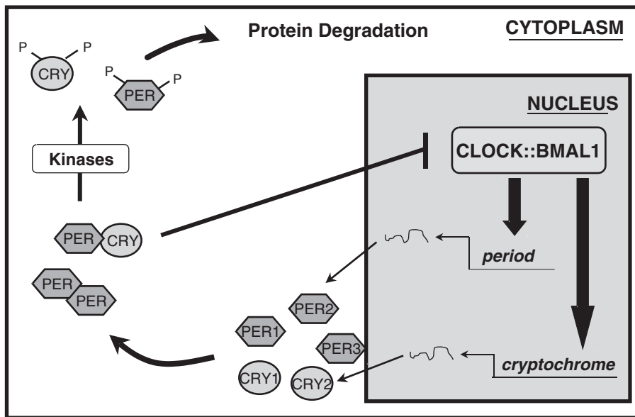
Figure 5.6. Schematic of the feedback loop. The feedback loop consists of four main components: PERIOD (PER), CRYPTOCHROME (CRY), CLOCK, and BMAL1. CLOCK and BMAL1 are positively acting transcription factors. They heterodimerize and activate transcription of the Per and Cry genes. There are actually three isoforms of PER and two isoforms of CRY as indicated in the figure. The PERs form both homodimers and heterodimers and also heterodimerize with the CRYs. On dimerization, PER and CRY translocate to the nucleus and inhibit the activity of the CLOCK:BMAL1 heterodimer. Evidence suggests that CRY is the dominant repressor. Suppression of CLOCK:BMAL1 activity causes transcription of Per and Cry to be shut off. The feedback loop is not permanently disrupted, however, because the PER and CRY proteins are targeted for degradation. The targeting signal is probably phosphorylation. The PERs are phosphorylated by casein kinase I \epsilon . The CRYs are also phosphorylated, although currently the kinase responsible for this is unknown. On degradation of PER and CRY, transcriptional repression is relieved and the cycle begins anew. The end result of the feedback loop is daily oscillation of both mRNA and protein levels of the core components. The exception is CLOCK, which is expressed at the same level throughout the day.
