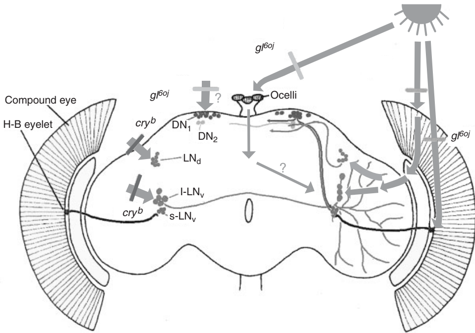
Figure 3.17. Redundant entrainment pathways for the lateral neurons as revealed by the effects of various mutations on entrainment. The cry b mutation disrupts the Drosophila cryptochrome photoreceptor. The gl mutation prevents development of all the cells that express PER in the adult head except the lateral neurons. Therefore, a gl ; cry double mutant has no entrainment pathways. [Reprinted from Helfrich-Forster et al. (2001): The circadian clock of fruit flies is blind after elimination of all known photoreceptors. Neuron 30: 249–261, copyright (2001) with permission from Elsevier Science.] The cells that are potentially circadian photoreceptors include the dorsal and ventral (large and small) lateral neurons (LN d , I LN v , s LN v ), the compound eye, the ocelli (three light-sensing organs on top of the head), the H-B eyelet (a cluster of photoreceptors between the retina and the optic lobe), and a cluster of dorsal neurons (DN). The pathways blocked by each of the two mutations, gl 60j , and cry b , are indicated by the bars on the arrows.
