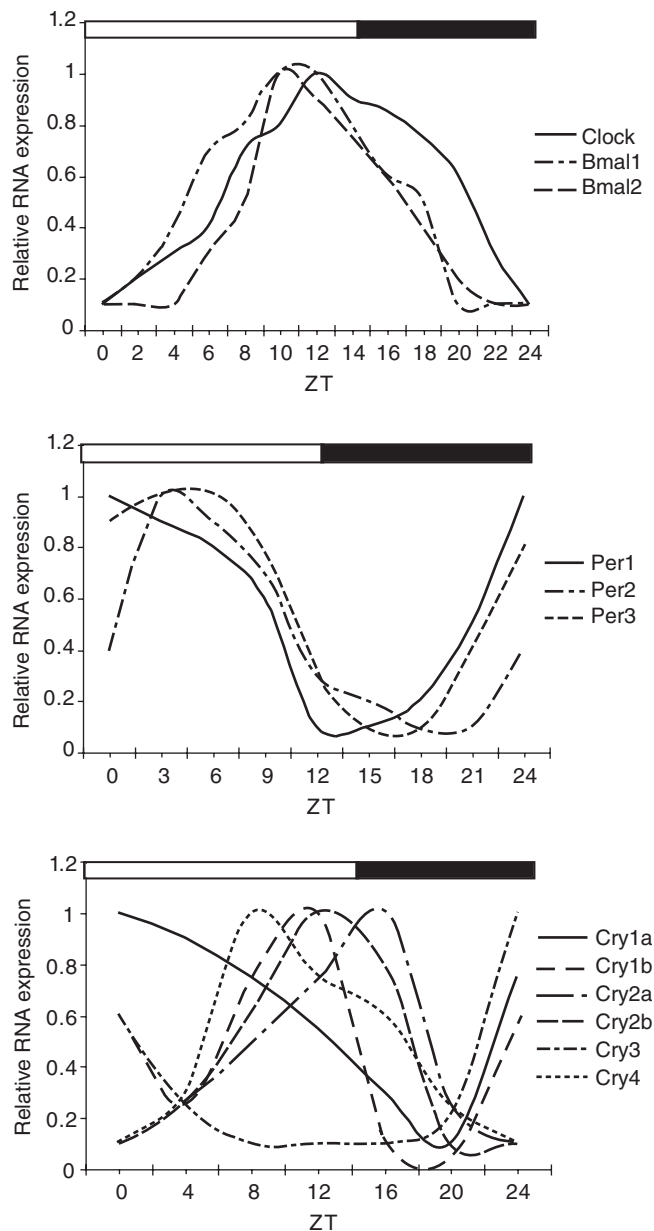
Figure 4.5. Summary of cycling clock genes in zebrafish. mRNA levels for each gene are plotted as described in Figure 4.2. Top panel is mRNA collected from zebrafish eye in a 14:10 light:dark cycle. Middle panel is mRNA collected from cultured Z3 cells (see text) in a 12:12 L:D cycle. Bottom panel is mRNA collected from zebrafish eye and whole body in a 14:10 L:D cycle.
