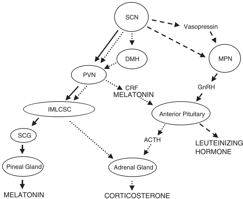
Figure 5.12. Output pathways of the SCN that regulate hormonal rhythms. The three most widely described hormonal outputs of the circadian system are melatonin, corticosterone, and leuteinizing hormone production. The melatonin pathway is shown connected by solid arrows. The SCN connects to the paraventricular nucleus (PVN), which in turn connects to the interomediolateral column of the spinal cord (IMLCSC). The IMLCSC connects to the pineal gland via the supracervical ganglion (SCG). The corticosterone pathway is shown by dotted arrows. There are multiple pathways controlling the corticosterone rhythm: (1) similar to the melatonin pathway, the SCN connects to the PVN, which in turn connects to the IMLCSC—however, the IMLCSC connects directly to the adrenal glands; (2) the PVN also regulates corticosterone release by producing corticotroph releasing factor (CRF), which stimulates the anterior pituitary to release adrenocorticotrophic hormone (ACTH, which stimulates the adrenals); and (3) the SCN also connects to the CRF, producing neurons of the PVN indirectly via the dorsal medial nucleus of the hypothalamus. The pathway regulating leuteinizing hormone release is shown by dashed arrows. LH is released by the anterior pituitary in response to gonadotrophin releasing hormone (GnRH) from the medial preoptic nucleus (MPN) of the hypothalamus. The SCN regulates the MPN both directly and indirectly via rhythmic vasopressin production.
