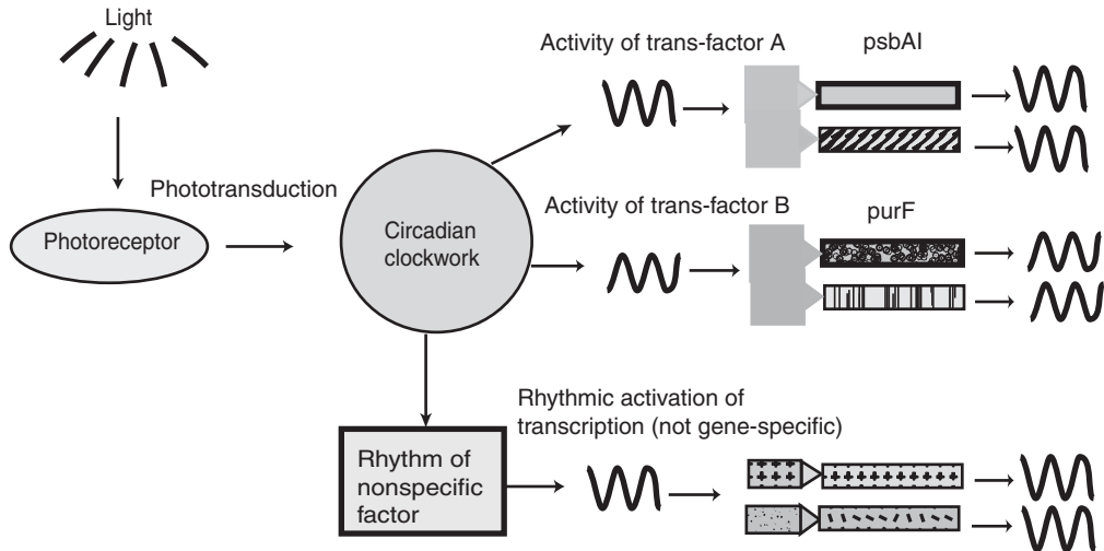
Figure 6.7. Model for global circadian control of gene expression. Coding regions of clock-controlled genes are depicted as rectangles with adjacent promoter regions. Some ensembles of genes may be controlled by rhythmic activity of specific trans factors that coordinately regulate groups of genes. These trans factors could be activated at different phases. Other genes may be regulated by global but nonspecific factors that oscillate. [Modified from Johnson et al. (1996).]
