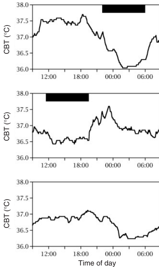
Figure 11.2. Masking of endogenous circadian rhythms by sleep. The figure shows typical circadian profiles of core body temperature (CBT) in humans studied in a laboratory: normal sleep–wake cycle (sleep from 22:00 until 06:00; top panel), displaced sleep–wake cycle (sleep from 11:30 until 19:30; middle panel), and constant routine (no sleep; bottom panel). Sleep periods are indicated with a black bar. The data illustrate that sleep–wake behavior, although under circadian control, can mask endogenous circadian rhythmicity in other variables such as CBT. Therefore, sleep is seldom considered an intrinsic component of endogenous circadian rhythmicity in humans, but is treated as a separate neurophysiological system. The same applies for the expression of (physical) activity during wakefulness. From studies of body temperature profiles obtained under different experimental circumstances, mathematical “purification” procedures have been developed to estimate the endogenous circadian profile of body temperature in the presence of environmental and internal masking factors. Using knowledge of sleep–wake times, activity patterns or light exposure, reasonably accurate estimates of endogenous circadian rhythm parameters can be obtained with such purification methods without the need for laboratory-based constant routine experiments. Note also that even in the constant routine data of individual subjects (bottom panel), recorded under highly controlled laboratory circumstances, there are fluctuations over time that cannot be accounted for by circadian rhythmicity. These fluctuations probably reflect biological or measurement noise, as they are largely averaged out when data for multiple subjects are pooled, leading to a stereotypical sinusoidal profile of CBT circadian rhythmicity.
