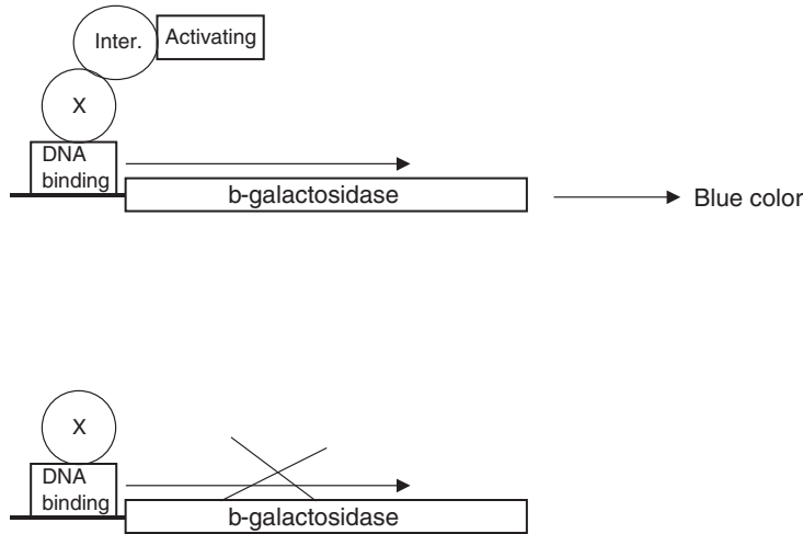
Figure 2.5. Identification of interacting proteins through the yeast two-hybrid assay. The protein of interest (protein X) is fused to the DNA binding domain of a transcription factor. An entire library of cDNA sequences is fused to a domain that is capable of activating transcription ("Activating"). Transcription of the reporter occurs only when the DNA binding and activating domains are brought together through the interaction of protein X with a protein in the library ("Inter."). Transcription of the reporter produces a protein that either allows growth of the yeast on specific media or renders a blue color to the yeast colony. In the example shown here, the reporter is \beta -galactosidase, which confers a blue color.
