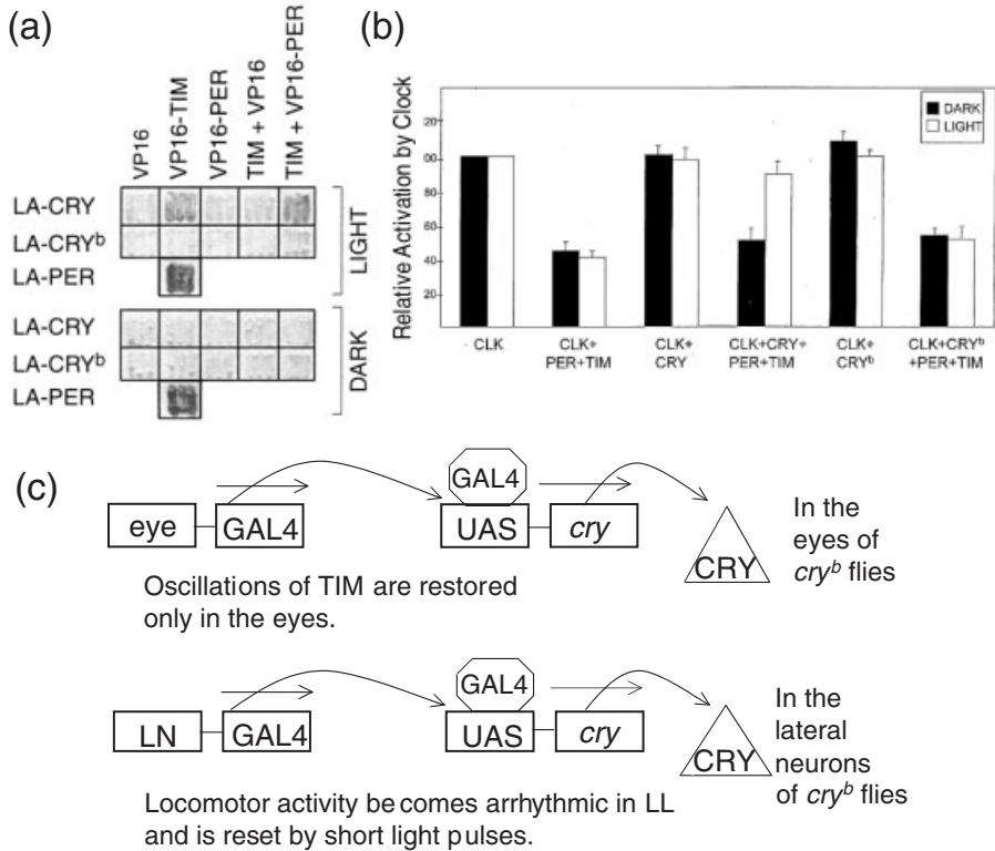
Figure 3.15. CRY undergoes a light-influenced association with TIM and acts intracellularly. (a) The yeast two-hybrid assay (described in Fig. 3.7a) shows that CRY associates with TIM in the light but not the dark. Proteins designated “LA-” are expressed as fusions with the LEXA DNA-binding domain, while those designated “VP16-” are expressed as fusions with the VP16 RNA polymerase-activating domain. CRY could also form a three-component (ternary complex) with PER, if TIM was present to complex with both PER and CRY (hence the interaction detected with LA-CRY, TIM, and VP16-PER; however, as described in the text, subsequent studies also found direct interactions between PER and CRY). CRY b cannot associate with TIM in either light or dark, and PER associates with TIM in either light or dark. (b) CRY disrupts the repression of dCLK by PER/TIM, but only in the presence of light. CRY b does not disrupt PER/TIM function. The cell culture assay is described in Figure 3.7b. [Reprinted with permission from Ceriani et al. (1999), copyright (1999) American Association for the Advancement of Science.] (c) Expression of CRY only in the eyes or only in the lateral neurons rescues the cry mutant phenotype only in the cells where CRY is expressed. The GAL4/UAS expression system is described in Figure 3.11b. The eye-specific (“eye”) promoter is the rhodopsin promoter, and the lateral neuron-specific (“LN”) promoter is the pigment dispersing factor promoter.
