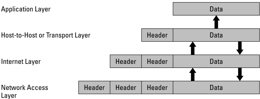
Figure 11-1: TCP/IP Encapsulation.
