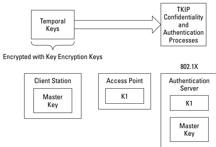
Figure 12-16: Key hierarchy for rekeying
