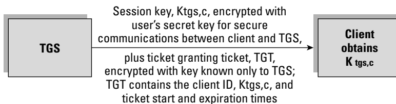
Figure 3-2: TGS and client session key/TGT exchange
