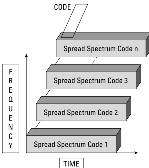
Figure 12-7: CDMA operation
