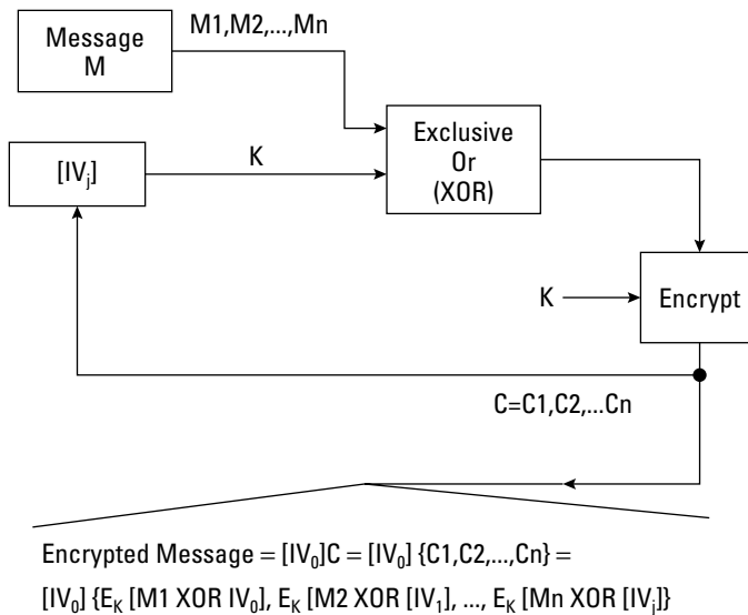
Figure 12-18: AES CBC mode
