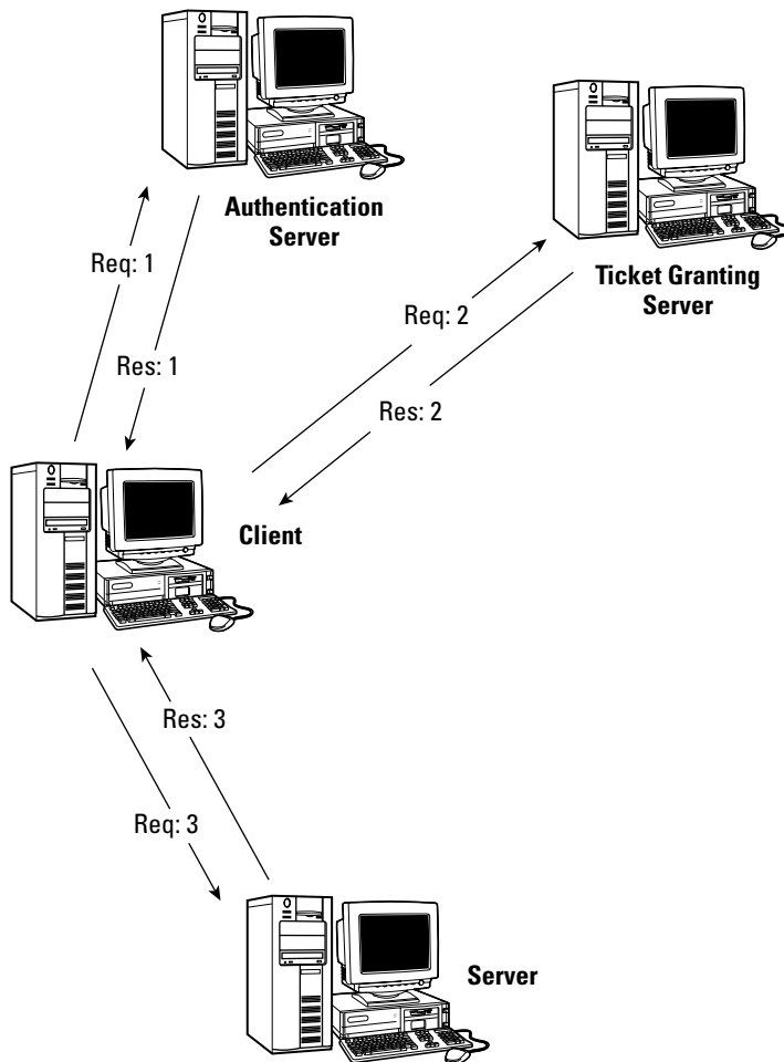
Figure 16-3: Ticket-granting server in the Kerberos Protocol
