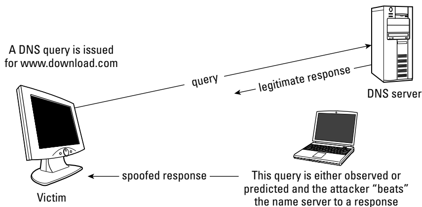
Figure 9-7: Illustration of a simple DNS attack that redirects traffic destined for www.download.com to a malicious site because the DNS query response from the attacker is received before the legitimate response arrives
