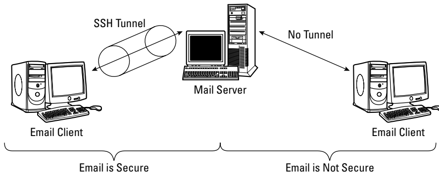
Figure 8-11: An SSH tunnel secures one-half of the e-mail transmission.
