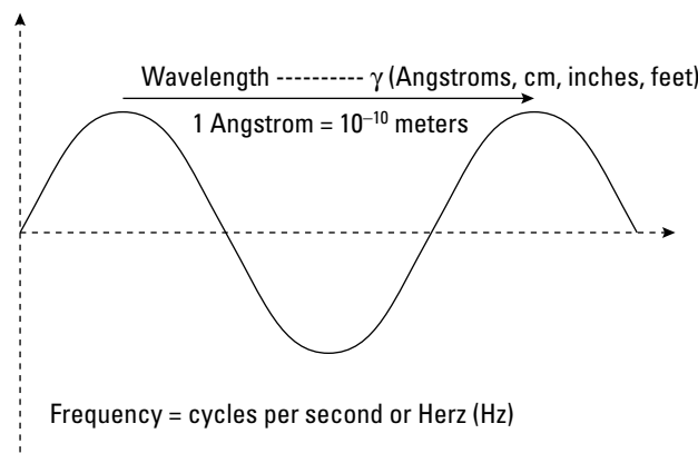
Figure 12-1: Sine wave characteristics
