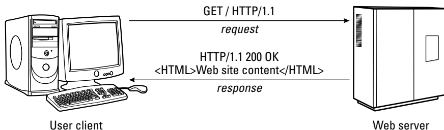
Figure 7-1: The basic request and response model used in an HTTP session
