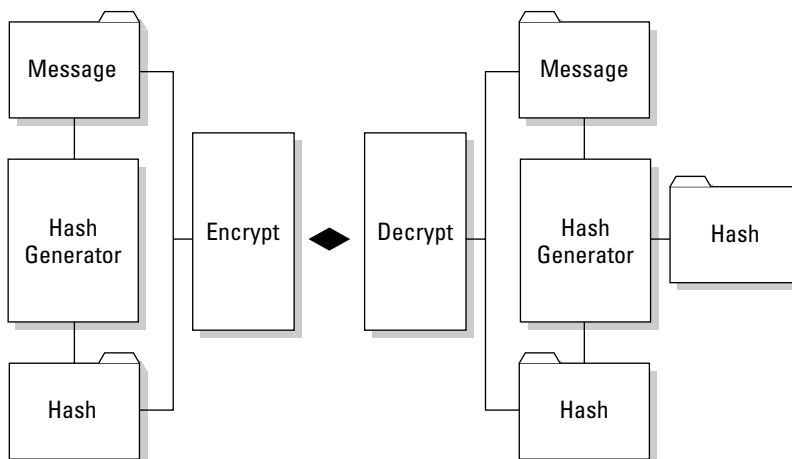
Figure 16-4: Digital signatures in PKI
