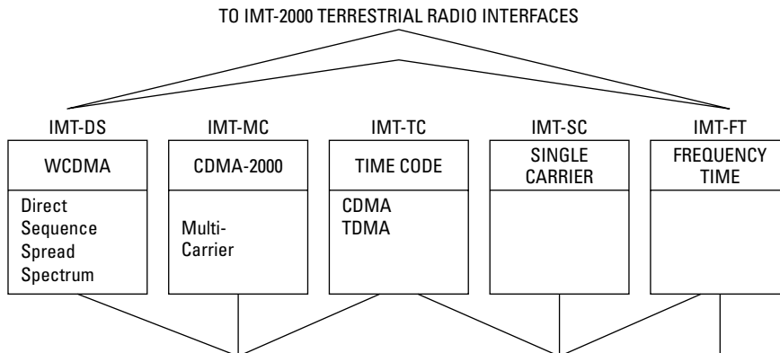
Figure 12-8: IMT-2000
