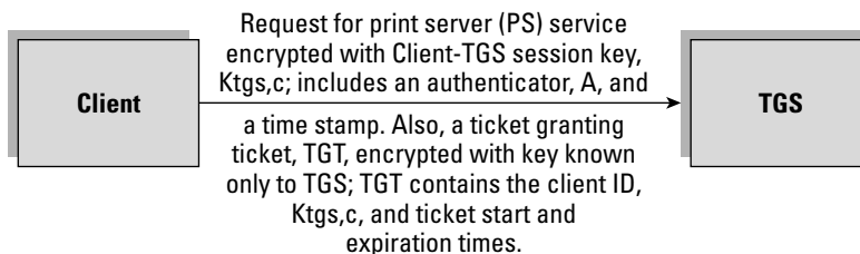
Figure 3-3: Client to TGS request for PS ticket
