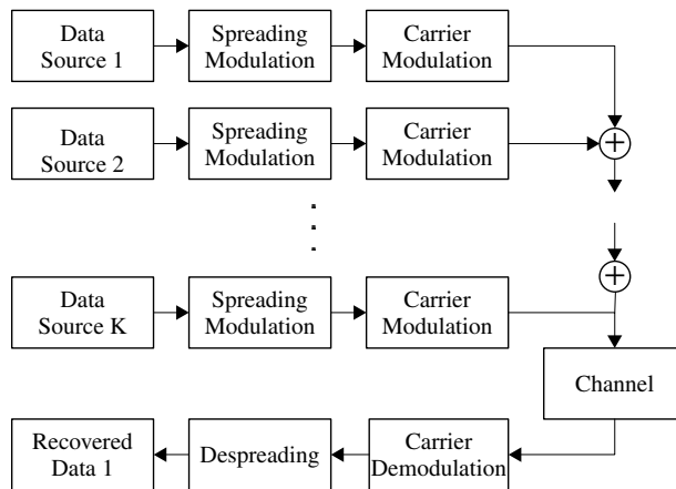
Figure 2.31 A generic K -user DS-CDMA system model, where only uplink channels of the system are concerned.
