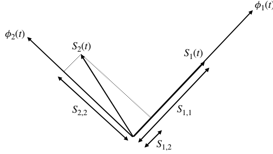
Figure 2.52 Signal space vector representation of two spreading codes and their orthogonal functions in ODFD MUD scheme.
