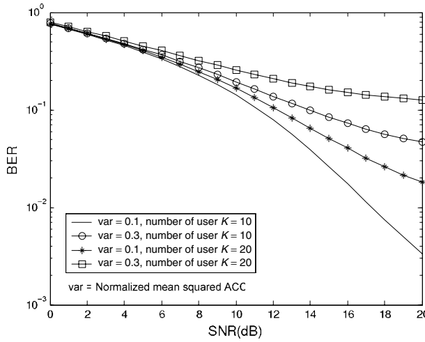
Figure 7.33 Bit error rate versus SNR with number of active users ( K = 10 or 20 ) and normalized mean squared ACF of pulse waveform ( \sigma_{mp\_normal}^2 ) being parameters. The spreading code length is 1024. The first cluster of the first user consists of 10 rays with totally 15 clusters. For all other users' signals, there are five clusters, each of which consists of 10 rays. A modified S-V channel model is considered, in which the arrival rates for the clusters and rays are 1/11 (1/ns) and 1/0.35 (1/ns), respectively. \sigma = 4.8 dB. The mean attenuation power of the first ray \Omega_1 = 1 , and all other rays decay exponentially with its decay factor \Gamma being 16. \gamma = 8.5 .
