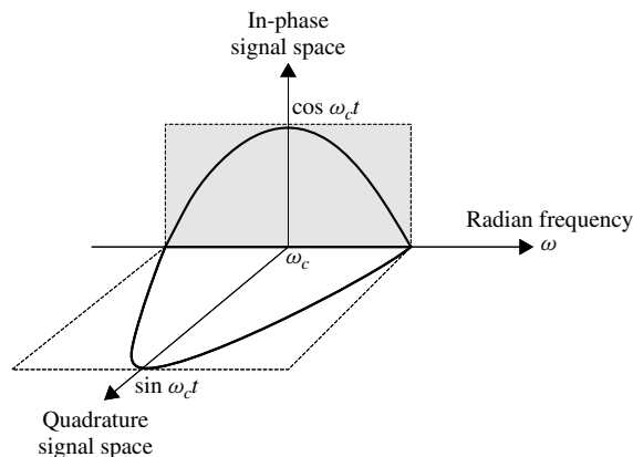
Figure 2.15 Orthogonality of \sin(\omega_c t) and \cos(\omega_c t) carriers in the in-phase and quadrature signal spaces in QPSK digital modulation.
