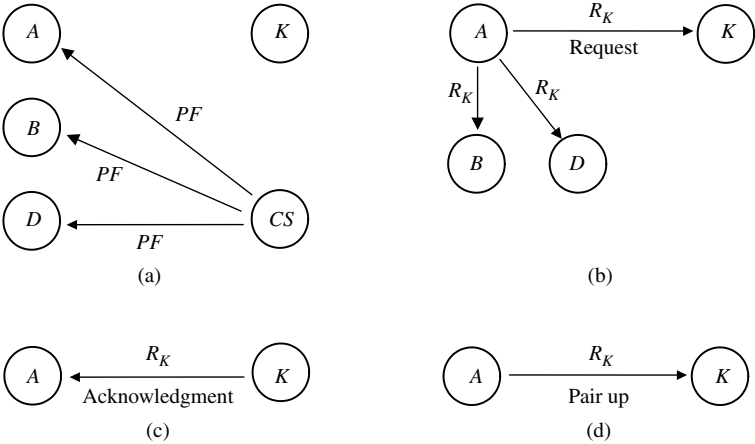
Figure 2.44 Pairing-up procedure between A (a transmitter) and K (a receiver) in the HSS protocol with B and D being contenders. (a) CS broadcasts PF ; (b) A initiates request to K ; (c) K acknowledges to A ; and (d) A pairs up with K .
