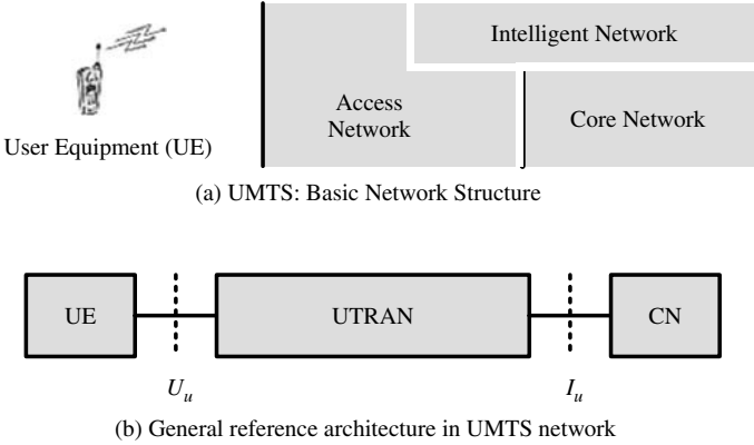
Figure 3.20 (a) UMTS basic network structure, and (b) UMTS general reference architecture.
