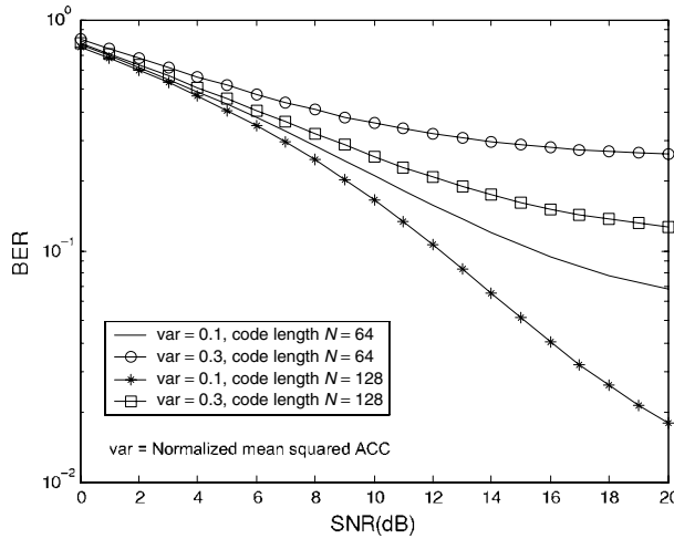
Figure 7.34 Bit error rate versus SNR in modified S-V multipath channel with spreading code length ( N = 64 or 128 ) and normalized mean squared ACF of pulse waveform ( \sigma_{mp\_normal}^2 = 0.1 or 0.3 ) being parameters. The number of active users is equal to 20. The first cluster of the first user consists of 10 rays with a total of 15 clusters. For all other users' signals, there are five clusters, each of which consists of 10 rays. A modified S-V channel model is considered, in which the arrival rates for the clusters and rays are 1/11 (1/ns) and 1/0.35 (1/ns), respectively. Channel parameter \sigma = 4.8 dB. The mean attenuation power of the first ray \Omega_1 = 1 , and all other rays decay exponentially with their decay factor \Gamma being 16. \gamma = 8.5 .
