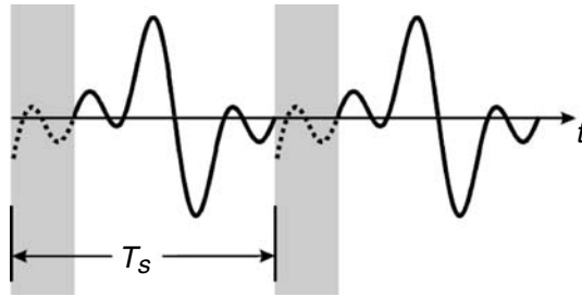
Figure 7.17 The cyclic prefix (shown as the shaded parts) used in an OFDM system as a guard time, which should be longer than the delay spread of the channel. Usually, the CP spans about one fourth of the symbol duration.
