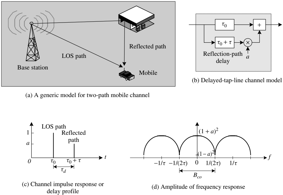
Figure 2.8 A generic two-path multipath channel model (a). Delayed-tap-line channel model (b). The delay spread of the channel is shown in (c). The frequency-selectivity and thus the coherent bandwidth of the channel can be seen from the amplitude of frequency response shown in (d).
