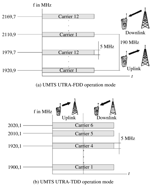
Figure 3.22 (a) UMTS UTRA-FDD operation mode, and (b) UMTS UTRA-TDD operation mode.
