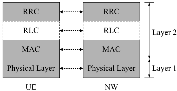
Figure 10.8 The E-UTRAN control-plane protocol stack.
