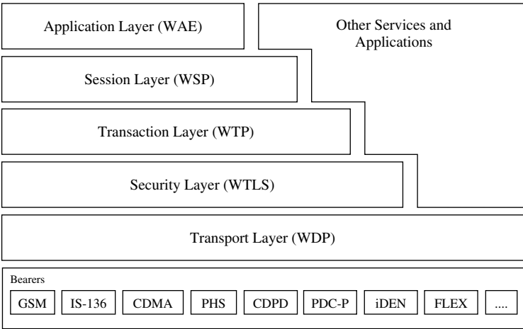
Figure 5.3 WAP architecture and reference model [508].
