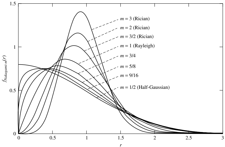
Figure 2.2 The probability density function of Nakagami- m random variable with m being its parameter. It can be seen that the Nakagami- m distribution will become Rician, Rayleigh, half-Gaussian when the parameter m takes \frac{3}{2} \sim 3 , 1 and \frac{1}{2} , respectively.
