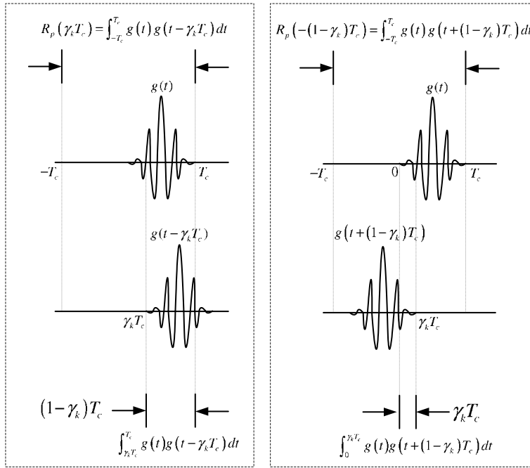
Figure 7.27 This figure illustrates how to calculate chip-wise pulse autocorrelation functions R_p(\gamma_k T_c) and R_p(-(1 - \gamma_k) T_c) .
