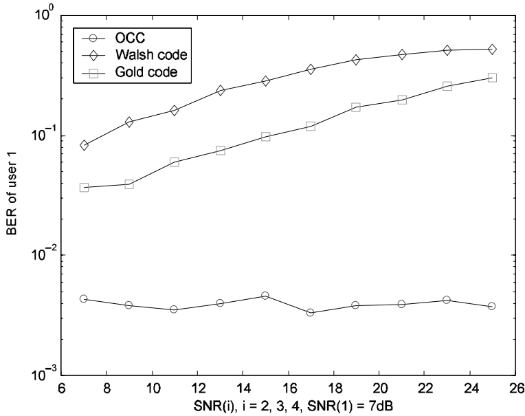
Figure 7.7 Illustration of inherent near-far resistance for an OC code-based CDMA system, where the performance of a conventional DS-SS-CDMA system based on Gold and Walsh-Hadamard codes under the near-far effect is also plotted. Four users are present in the system and the signal of interest is from user 1. An up link asynchronous multipath channel with its path gain being [0.8557, 0.5134, 0.0642] is considered. Interpath and interuser delays are one and three chips, respectively. The parameters of the OC code are K = M = 4 , N = 4 , and thus the PG is MN = 16 . The length of the Gold and Walsh-Hadamard codes is 15 and 16, respectively.
