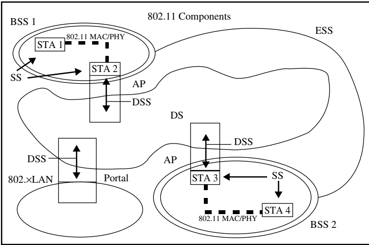
Figure 4.2 802.11 WLAN components [452].
