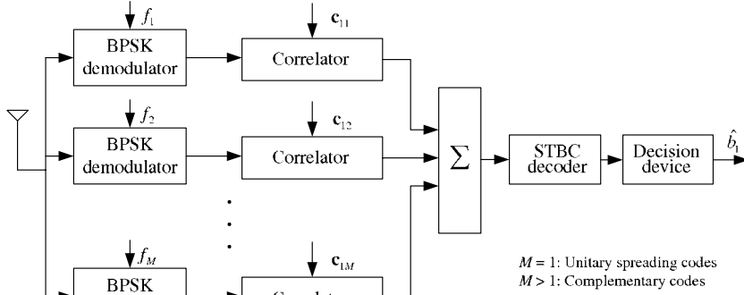
Figure 8.9 The block diagram for a generic STBC-CDMA receiver whose signal of interest is the k -th user ( k = 1 is assumed here), where M BPSK demodulators are tuned to different carriers, f_1, f_2, \dots, f_M . M element codes should undergo individual matched filtering and then be summed up to form a variable prior to STBC decoding. If M = 1 , the model represents an STBC-CDMA system based on unitary codes; otherwise it will be a model for an STBC-CDMA system using complementary codes.
