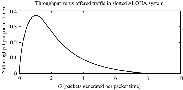
Figure 2.42 Throughput of a slotted ALOHA system, where the capacity peak ( S = \frac{1}{e} \simeq 0.3678 ) happens when the offered traffic is G = 1 .
