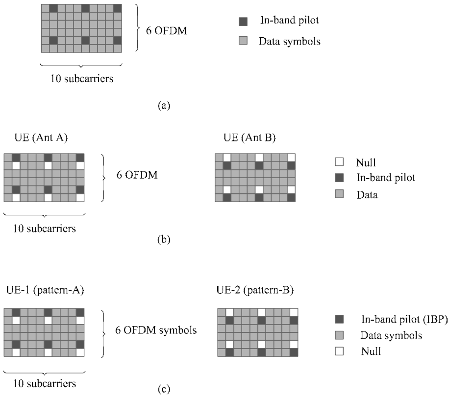
Figure 10.12 (a) Exemplifies the case of a single UE transmitting on a single antenna for which no orthogonal pilot is used. (b) Exemplifies the case of a UE transmitting on multiple antennae for which orthogonal pilot patterns are transmitted from multiple antennae. (c) Exemplifies the case of multiple UEs, each of which transmits on a single antenna, and shares the same time and frequency resource. Each UE transmits one orthogonal pilot pattern (virtual MIMO case).
