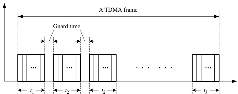
Figure 2.28 Illustration of a time frame structure in a TDMA scheme, where K users share a TDMA frame for their transmissions in their individual time slots, and a guard time (GT) is inserted in between every two consecutive time slots to prevent possible interference caused by transceiver time jitter or synchronization errors, and so on.
