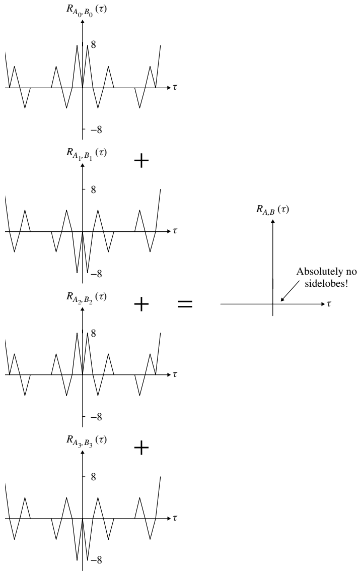
Figure 2.34 Cross-correlation function of an orthogonal complementary code with its element code length being 16 and PG\ 16 \times 4 = 64 . A detailed information of this particular CC code is given in Table 2.5 where R_{A_0, B_0}(\tau) is the CCF of element codes A_0 and B_0 , R_{A_1, B_1}(\tau) is the CCF of element codes A_1 and B_1 , R_{A_2, B_2}(\tau) is the CCF of element codes A_2 and B_2 , R_{A_3, B_3}(\tau) is the CCF of element codes A_3 and B_3 , and R_{A, B}(\tau) is the sum of R_{A_0, B_0}(\tau) , R_{A_1, B_1}(\tau) , R_{A_2, B_2}(\tau) , and R_{A_3, B_3}(\tau) .
