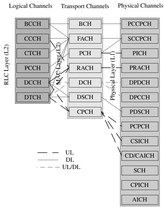
Figure 3.26 Physical, transport, and logical channels in the UMTS standard and their mapping relation among them.
