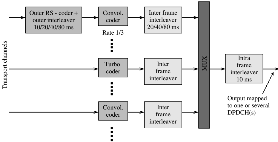
Figure 3.29 Mapping from transport channels to physical channels using deferent coding and multiplexing schemes in the UTRA-FDD.
