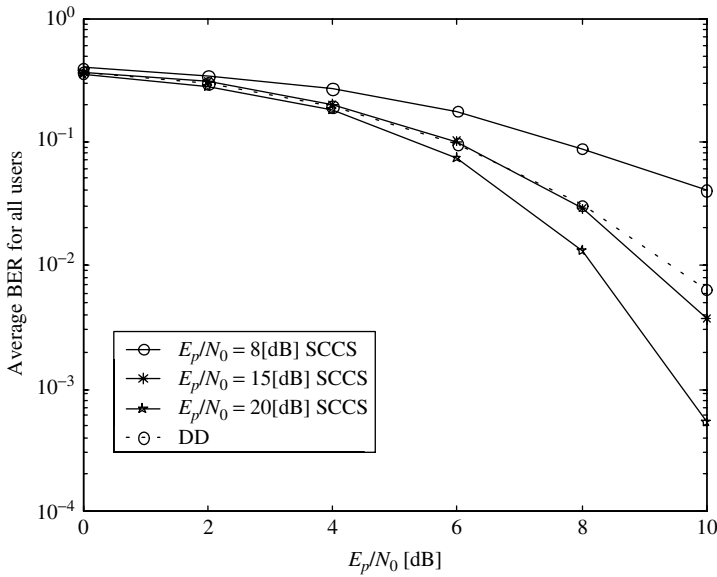
Figure 2.60 The average BER over all users versus pilot channel SNR E_p/N_0 for DD and SCCS detectors in a synchronous CDMA system. Multipath number is L = 3 , multipath pattern is [1, 0.6, 0.6/8] , interpath delay is five chips, the local code is c_1(t) , the length of Gold codes is N = 31 with the generating polynomials and initial loadings being p_1 = [1, 1, 0, 1, 1, 1] ; p_2 = [1, 0, 0, 1, 0, 1] , v_1 = [0, 0, 0, 0, 0, 1] ; v_2 = [0, 0, 0, 0, 0, 1] .
