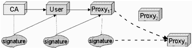
Figure 6.9 Proxies.
