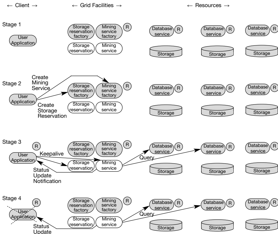
Figure 5.9 Workflow example.
