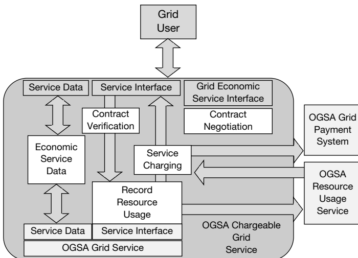
Figure 7.2 Computational grid service being sold as a Chargeable Grid Service (CGS).
