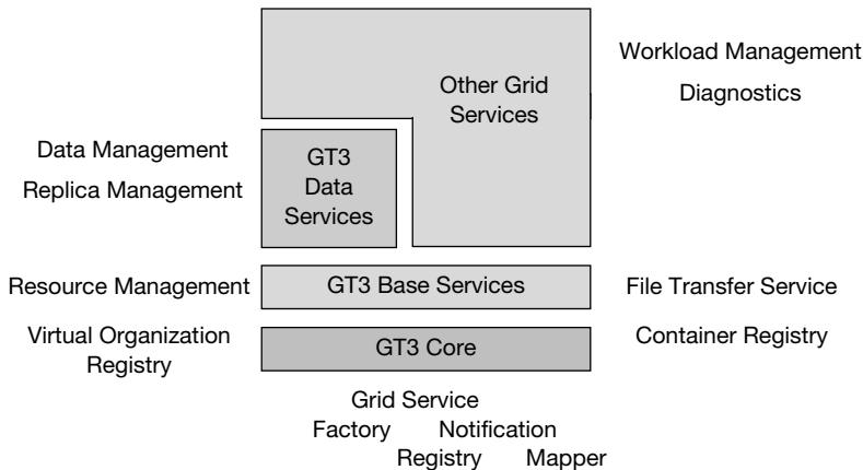
Figure 6.4 GT3 architecture.
