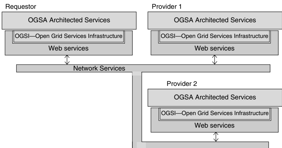
Figure 4.1 Networking role.
