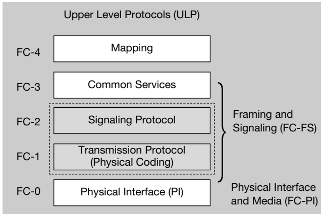
Figure 8.2 FC layers.
