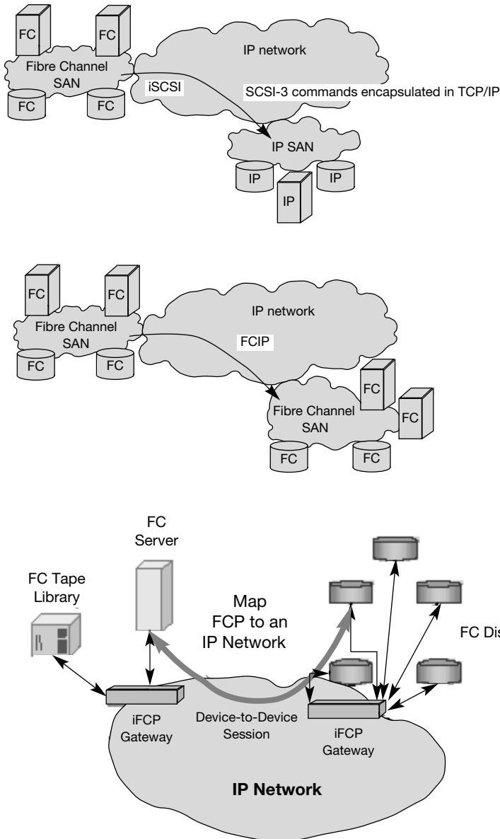
Figure 8.9 Tunneling arrangements. Top: iSCSI permits SCSI-3 commands to tunneled and delivered reliably over IP networks. Middle: FCIP permits multiple local FC SANs to be interconnected over an IP network backbone. Bottom: iFCP permits FC SANs to be interconnected via IP networks of any length, using traditional IP network elements (e.g., routers).
