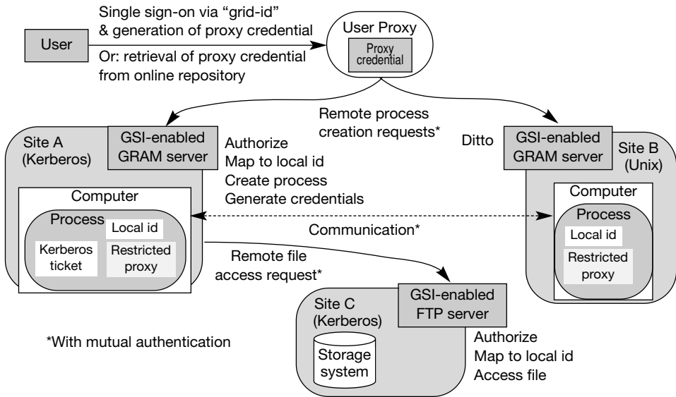
Figure 6.2 GSI in action "Create processes at A and B that communicate and access files at C." Copyright © 2002 University of Chicago and The University of Southern California. All Rights Reserved.
