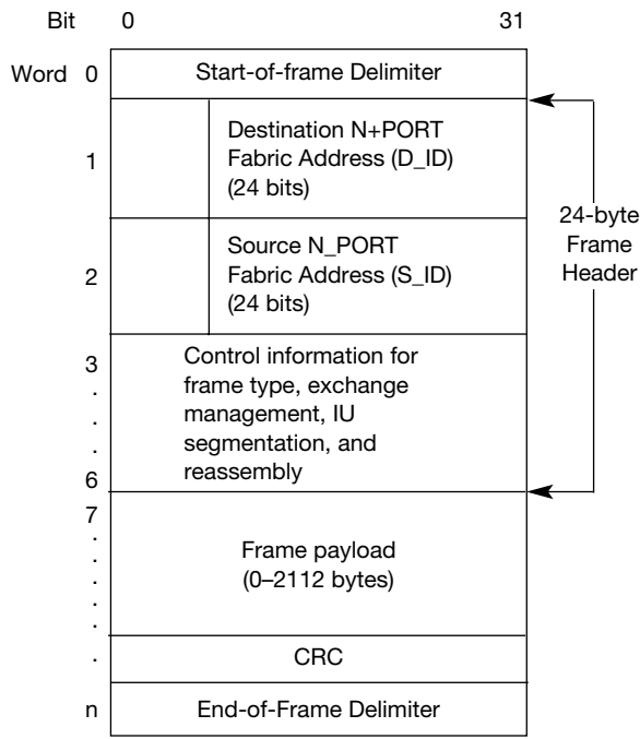
Figure 8.7 Fibre channel frame format.
