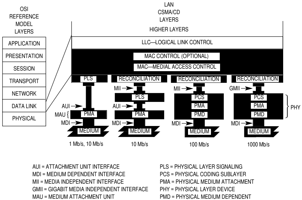
Figure 8.11 LAN standard relationship to the ISO/IEC Open Systems Interconnection (OSI) reference model.
