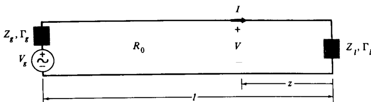
Figure 5.9. Complete two-wire transmission line system.
