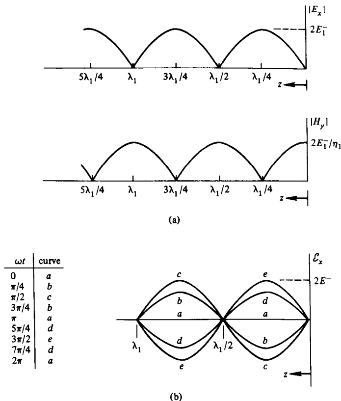
Figure 4.10. Pure standing waves, \text{SWR} \rightarrow \infty . (a) |E_x| and |H_y| versus z , dielectric-perfect conductor interface. (b) \mathcal{E}_x versus z for various values of t , \mathcal{E}_x(z, t) = -2E^- \sin(\omega t) \sin(k_1 z) .
