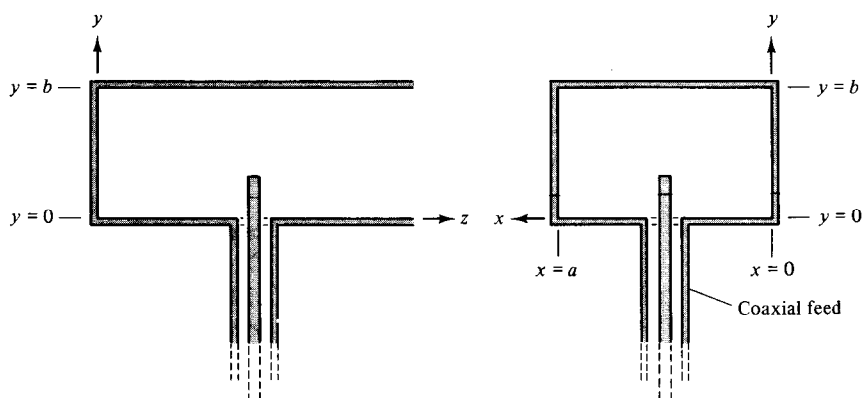
Figure 6.6. Monopole coupling into a waveguide from a coaxial cable.
