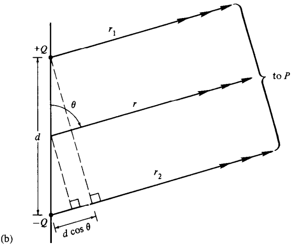
Figure 2.8. (a) Electric dipole centered on the z axis (b) Simplifications for calculating \Phi at a remote point P .
