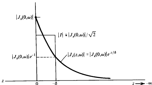
Figure 4.6. Actual distribution of |J_x(z, \omega)| and the equivalent uniform current density (skin effect).
