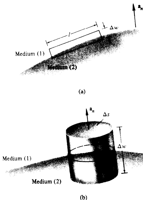
Figure 3.10. (a) Rectangular path for evaluating \oint \mathcal{E} \cdot d\mathbf{l} or \oint \mathcal{H} \cdot d\mathbf{l} . (b) Cylindrical surface for evaluating \oint \mathcal{B} \cdot d\mathbf{s} or \oint \mathcal{A} \cdot d\mathbf{s} .
