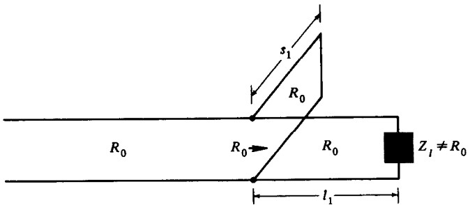
Figure 5.31. Single stub matching system.
