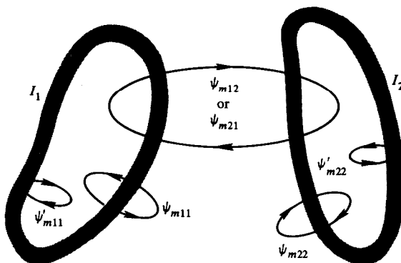
Figure 2.41. Magnetically coupled circuits showing the various flux linkages.
