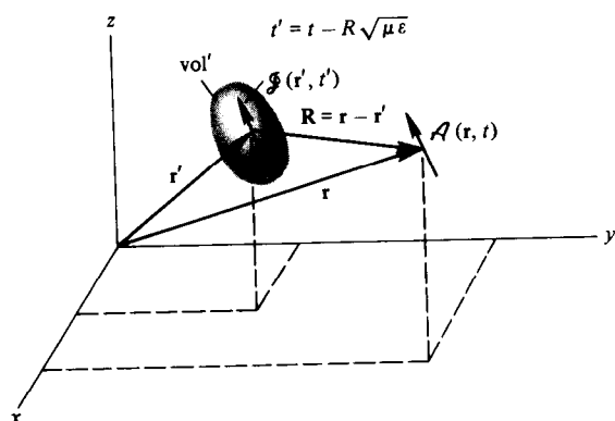
Figure 3.9. Geometry for the calculation of \mathcal{A}(\mathbf{r}, t) due to \mathbf{J}(\mathbf{r}', t') .
