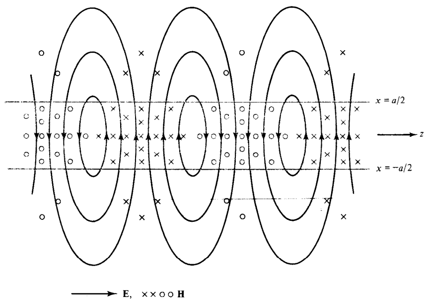
Figure 6.14. \text{TM}_0^0 dielectric slab field distribution.
