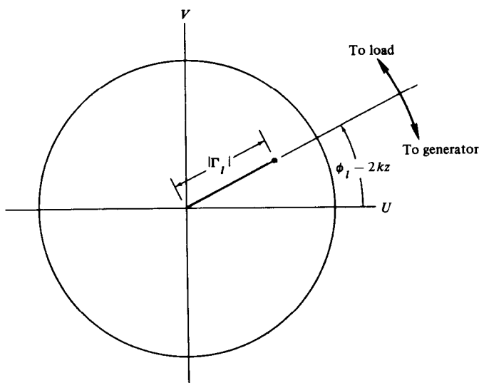
Figure 5.22. |\Gamma_I| \phi_I - 2kz in the U, V plane.
