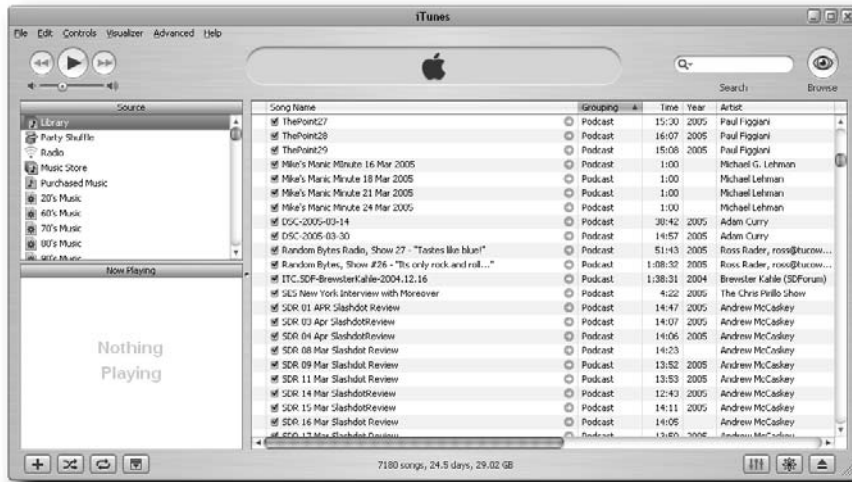
FIGURE 3-27: iTunes Library.
