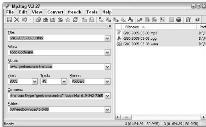
FIGURE 9-18: Mp3Tag v. 2.27.
