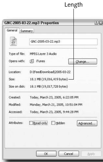
FIGURE 12-4: File properties.
