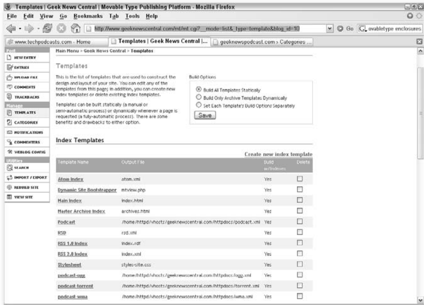
FIGURE 11-4: Template menu.
