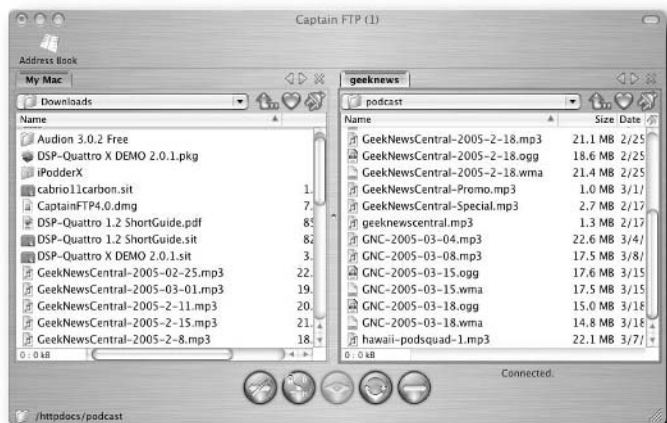
FIGURE 5-7: Captain FTP.
