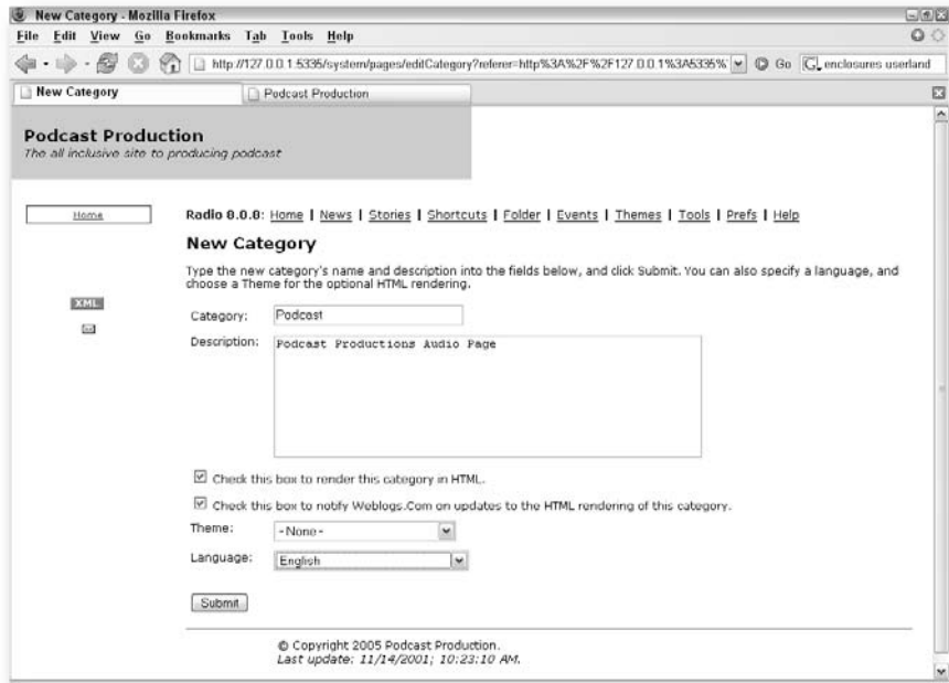
FIGURE 11-8: Category addition.
