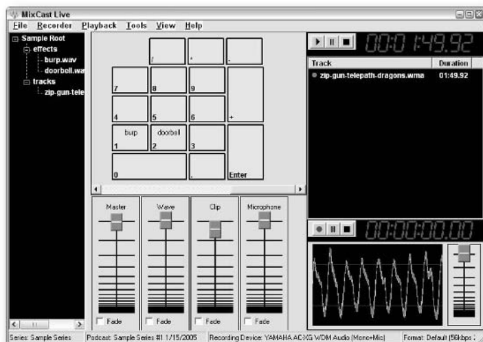
FIGURE 5-5: Mixcast Live.
