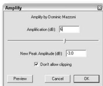
FIGURE 9-8: Amplify window.
