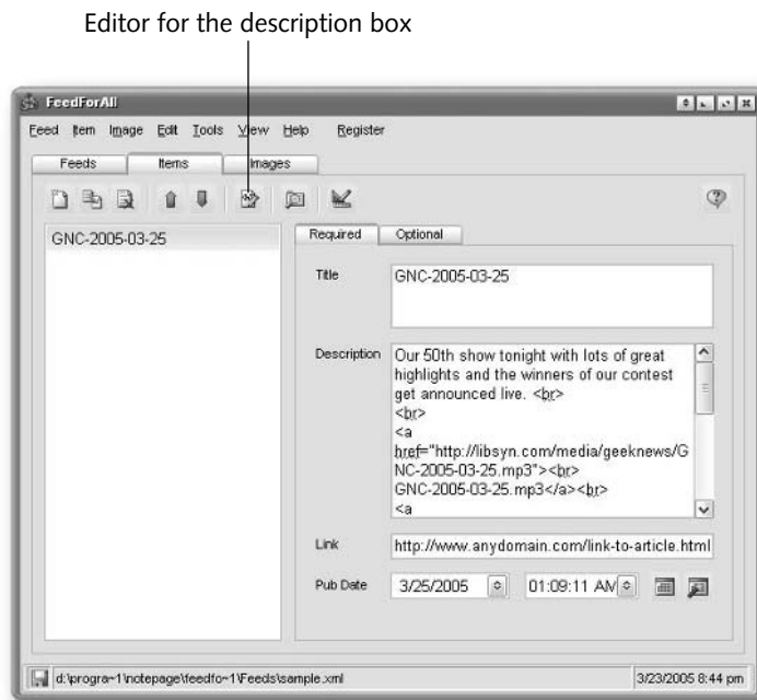
FIGURE 12-2: Items tab.
