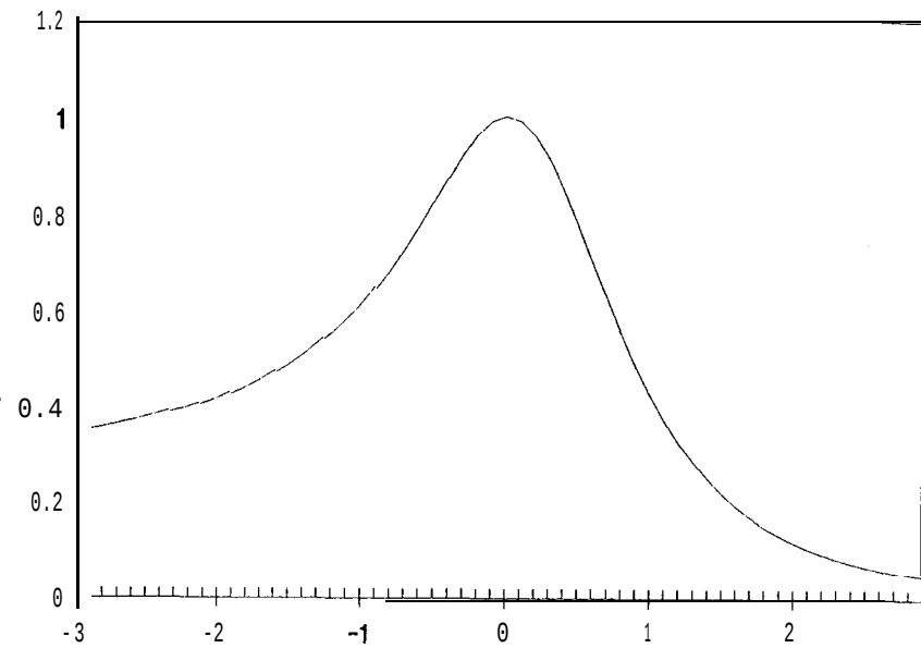
Figure 4-8 LOC = 0 SCALE = 1 SKEW = -0.5 KURT = 2.
