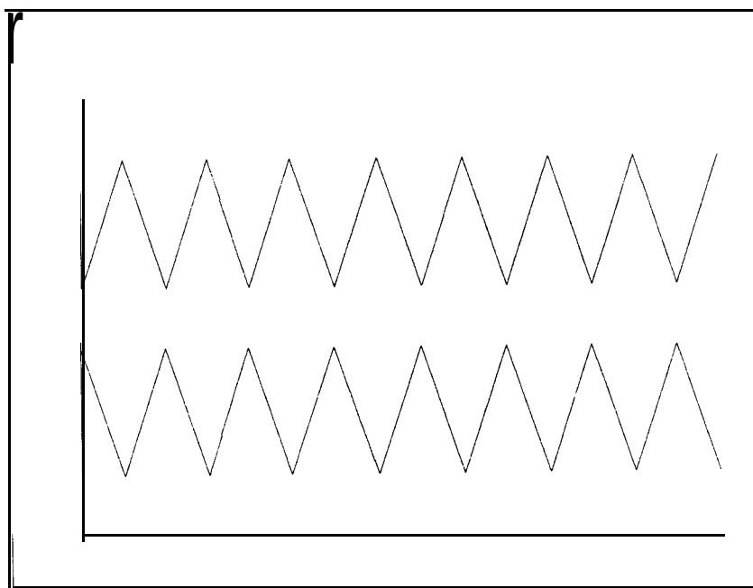
Figure 1-3 Negative correlation ( r = -1.00 ).
