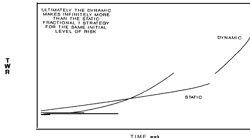
Figure 8-1 Static versus dynamic fractional f .
