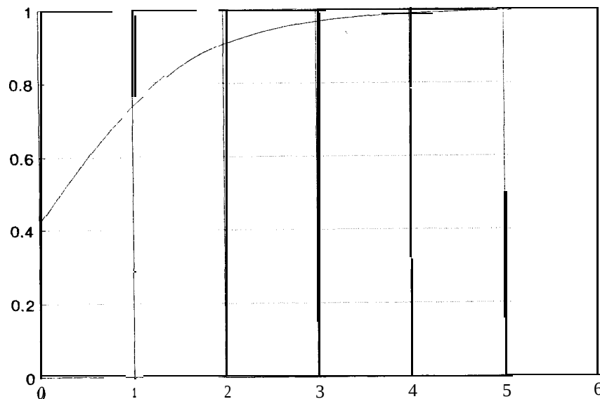
Figure E1.5 Cumulative probability functions for the Exponential Distribution ( A = 1 ).
