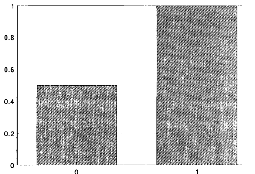
Figure B-4 Cumulative probability functions for the Bernoulli Distribution ( P = .5 ).
