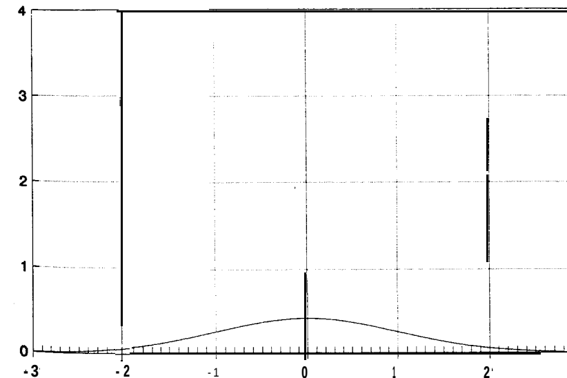
Figure 3-14 The real shape of the Normal Distribution.
