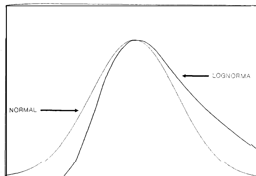
Figure 3-15 The Normal and Lognormal distributions.
