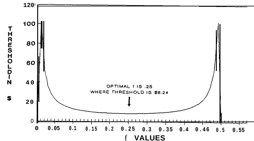
Figure 2-1 Threshold to the geometric for 2:1 coin toss.
