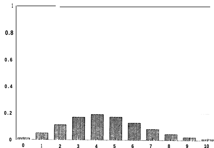
Figure B-i 2 Probability density functions for the Poisson Distribution ( L = 4.5 ).
