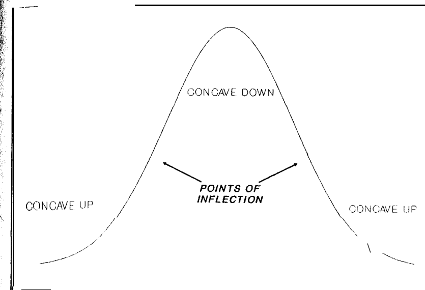
Figure 4-1 1 Points of inflection on a bell-shaped distribution.
