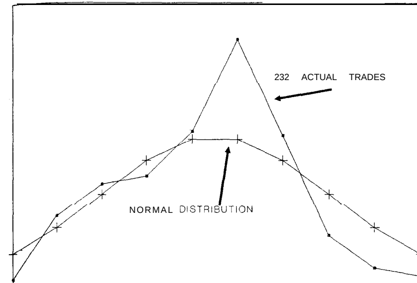
Figure 3-16 232 individual trades in 10 bins from -2 to +2 sigma versus the Normal Distribution.
