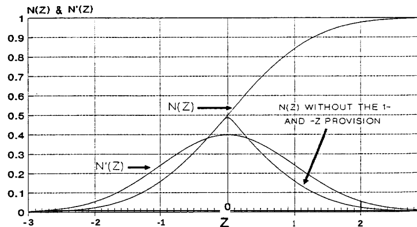
Figure 3-9 Doing away with the 1- and -Z provision in Equation (3.21).
