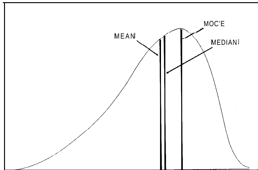
Figure 3-3 Skewness alters location.
