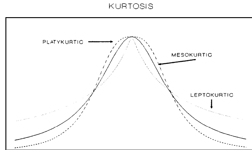
Figure 3-4 Kurtosis.
