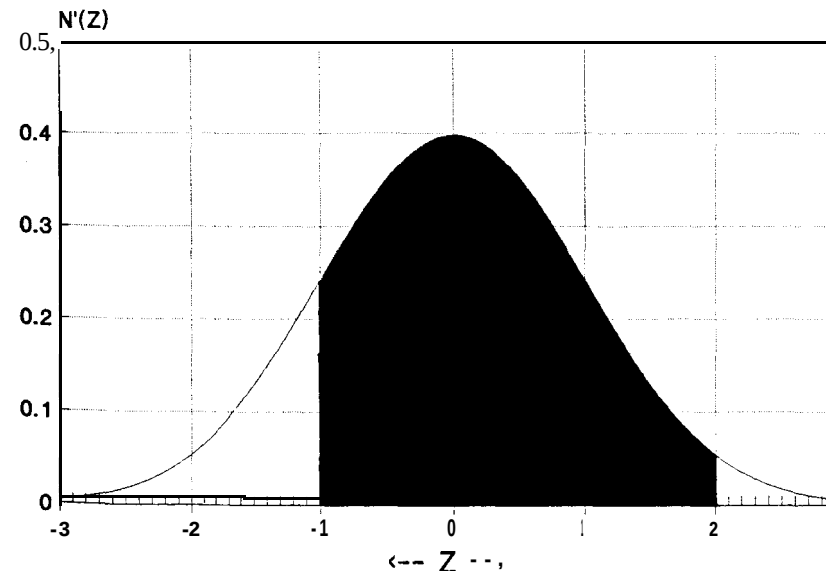
Figure 3-12 The area between -1 and +2 standard units.
