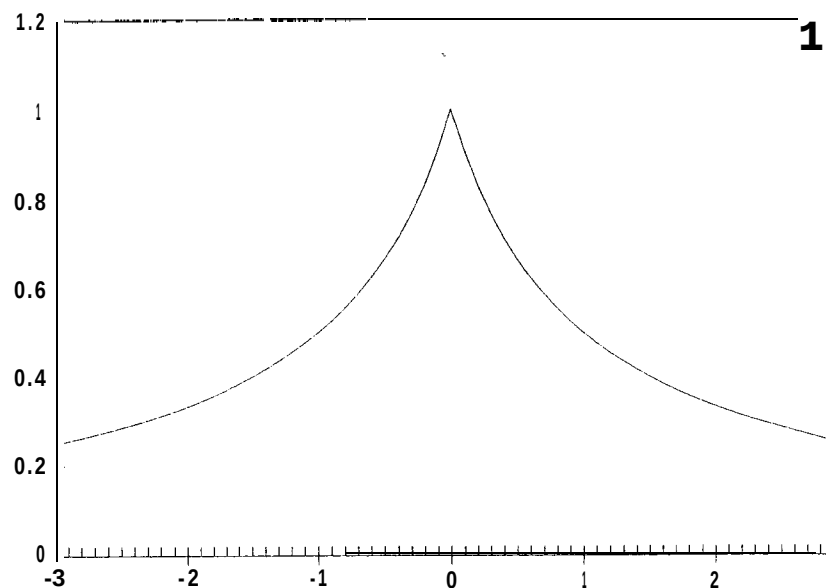
Figure 4-5 LOC = 0 SCALE = 1 SKEW = 0 KURT = 1.
