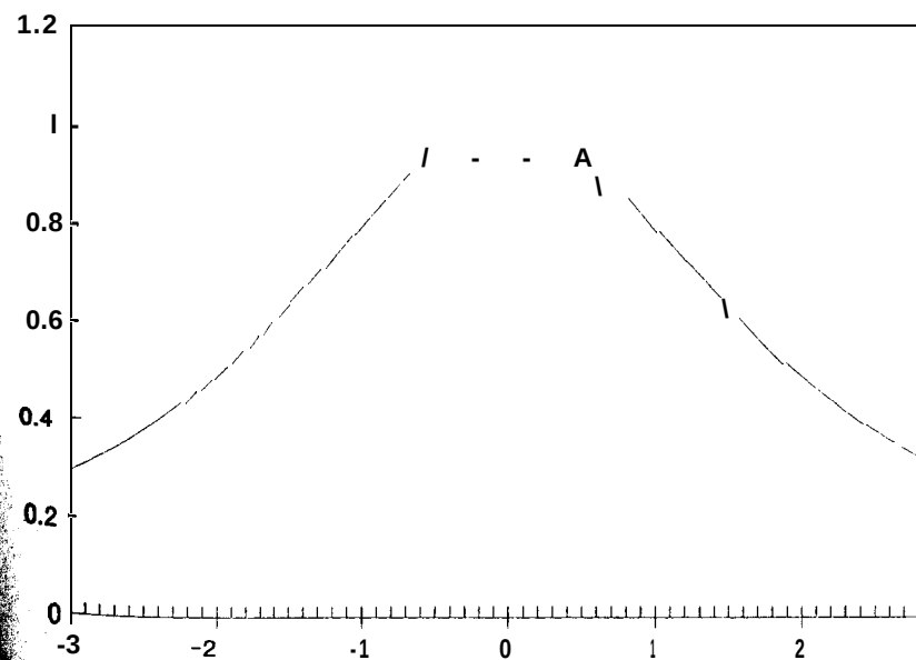
Figure 4-6 LOC = 0 SCALE = .5 SKEW = 0 KURT = 2.
