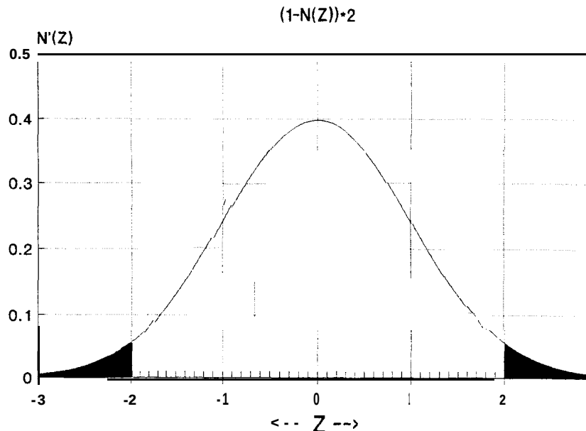
Figure 3-11 Two-tailed probability of an event being beyond 2 sigma.
