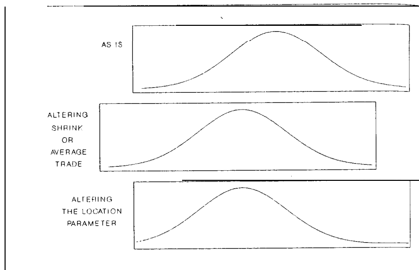
Figure 4-12 Altering location parameters.
