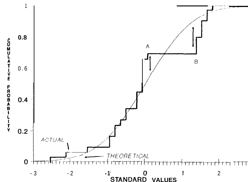
Figure 4-1 The K-S test.
