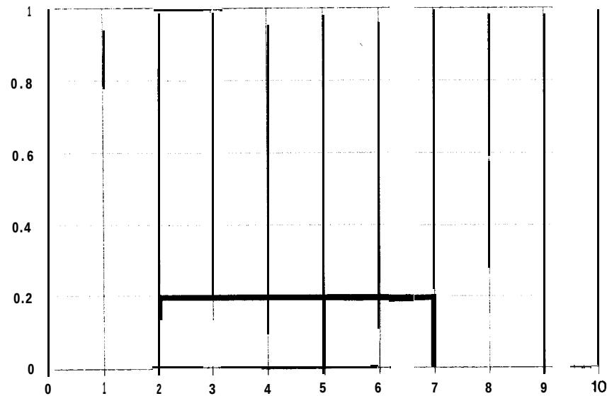
Figure B-1 Probability density functions for the Uniform Distribution ( A = 2 , B = 7 ).
