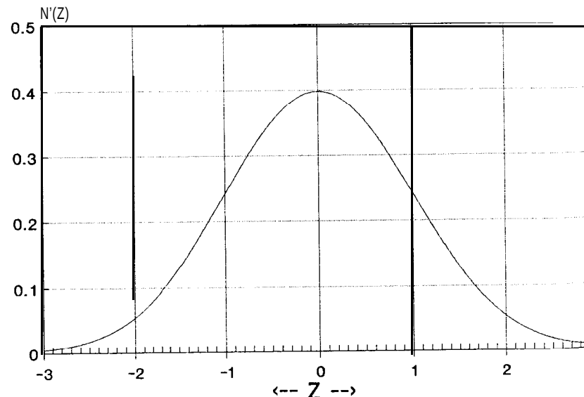
Figure 3-7 The Normal Probability density function.
