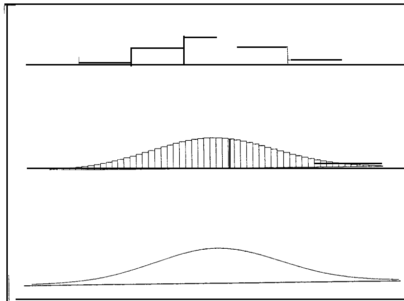
Figure 3-1 A continuous distribution is a series of infinitely thin bins
