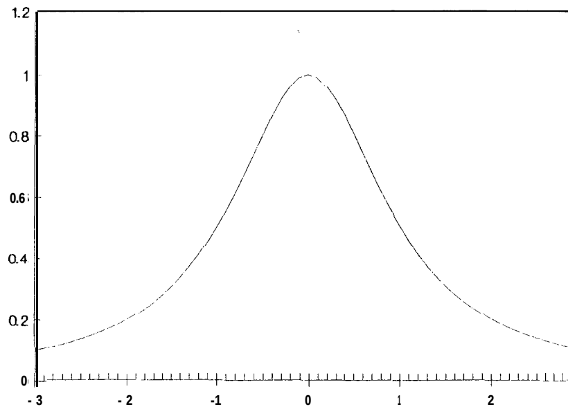
Figure 4-2 LOC = 0 SCALE = 1 SKEW = 0 KURT = 2.
