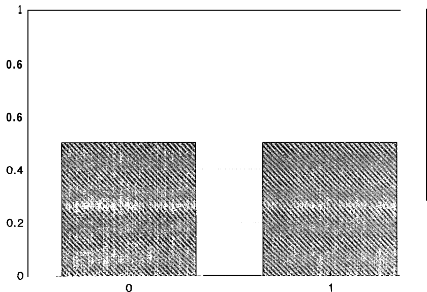
Figure B-3 Probability density functions for the Bernoulli Distribution ( P = .5 ).
