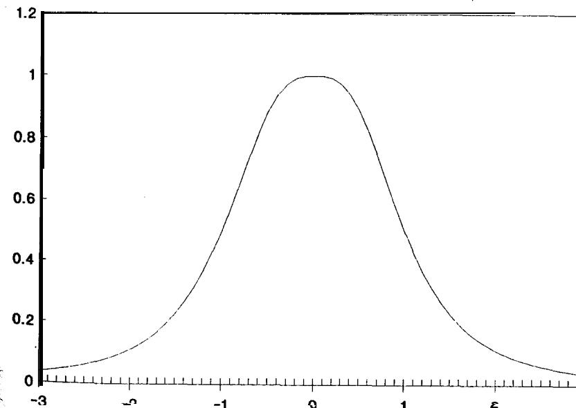
Figure 4-4 LOC = 0 SCALE = 1 SKEW = 0 KURT = 3.
