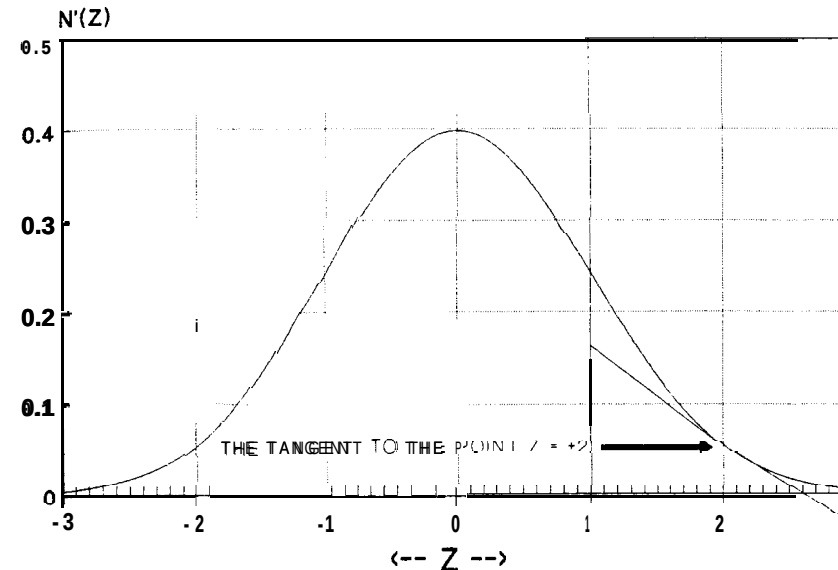
Figure 3-13 N'(Z) giving the slope of the line tangent tangent to N'(Z) at Z = +2 .
