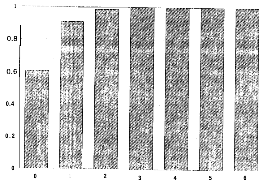
Figure E1-1 Cumulative probability functions for the Poisson Distribution ( L = .5 ).
