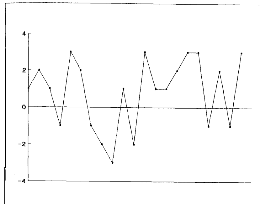
Figure I-4 Individual outcomes of 21 trades.
