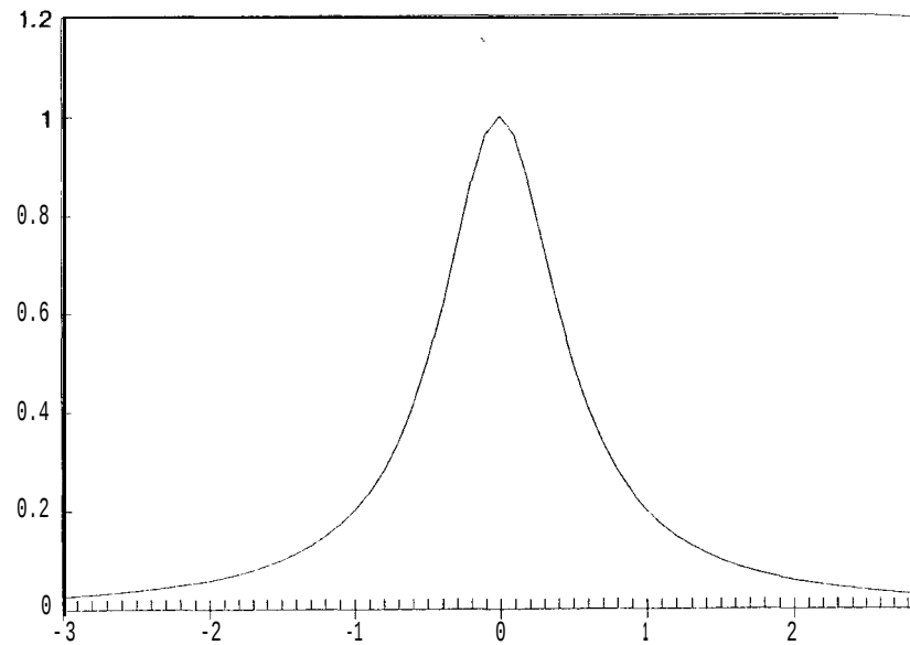
Figure 4-7 LOC = 0 SCALE = 2 SKEW = 0 KURT = 2.
