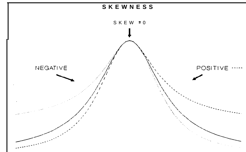
Figure 3-2 Skewness.
