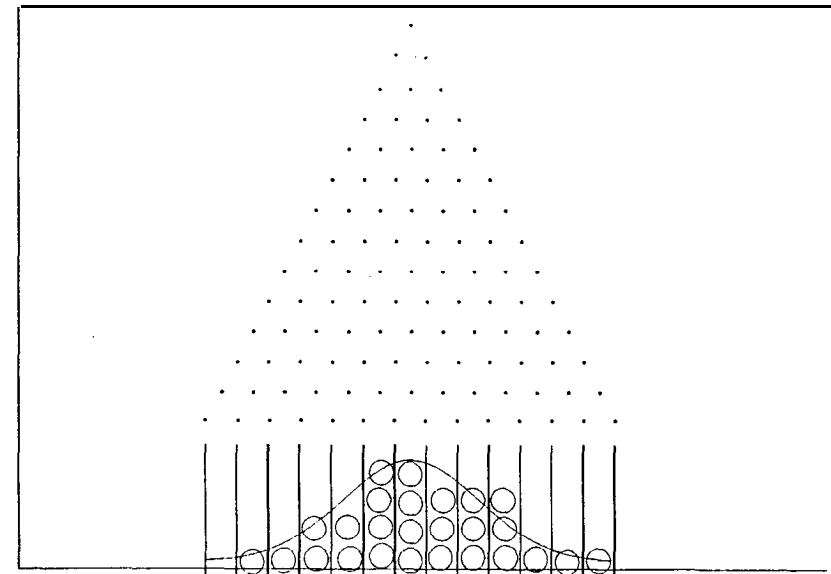
Figure 3-5 Galton's board.
