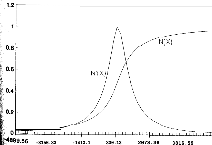
figure 4-10 Adjustable distribution fit to the 232 trades.
