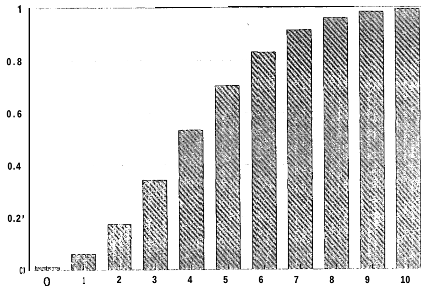
Figure 8-13 Cumulative probability functions for the Poisson Distribution ( L = 4.5 ).
