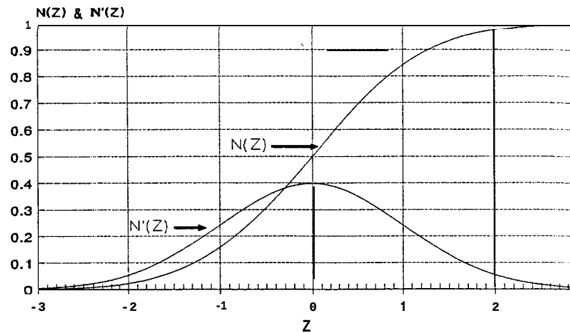
Figure 3-8 Equation (3.21) showing probability with Z = +2 .
