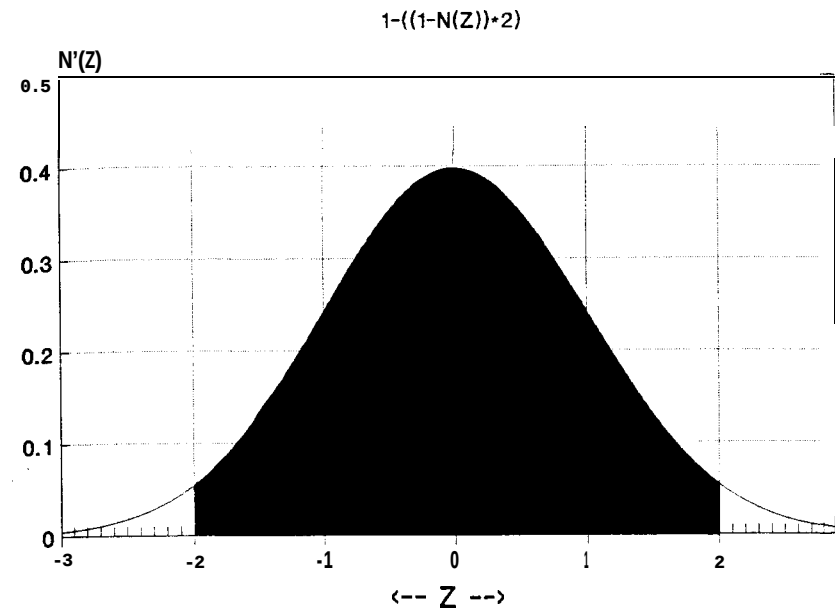
Figure 3-10 A two-tailed probability of an event being + or - 2 sigma.
