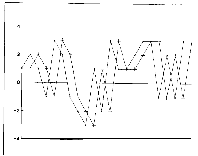
Figure I-5 Individual outcomes of 21 trades skewed by 1 trade.
