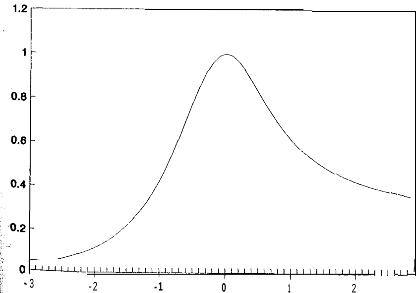
Figure 4-9 LOC = 0 SCALE = 1 SKEW = +0.5 KURT = 2.
