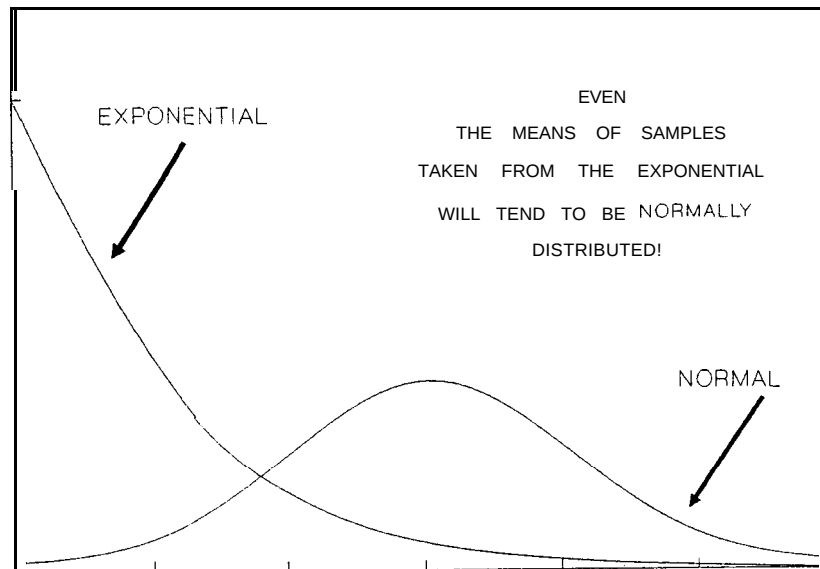
Figure 3-6 The Exponential Distribution and the Normal.
