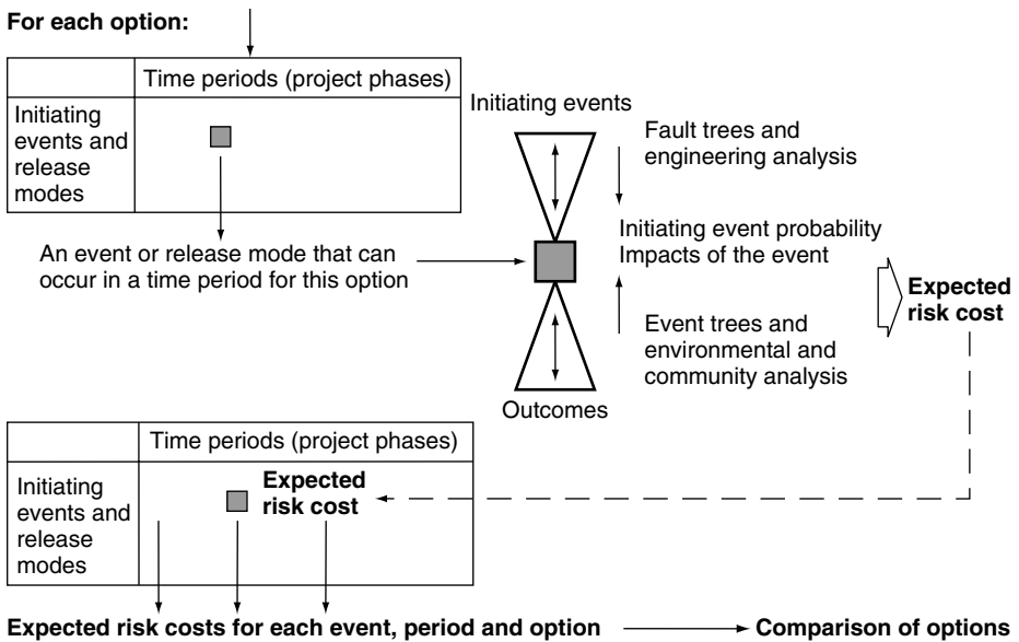
Figure 17.8 —Combining fault tree and event tree analyses
