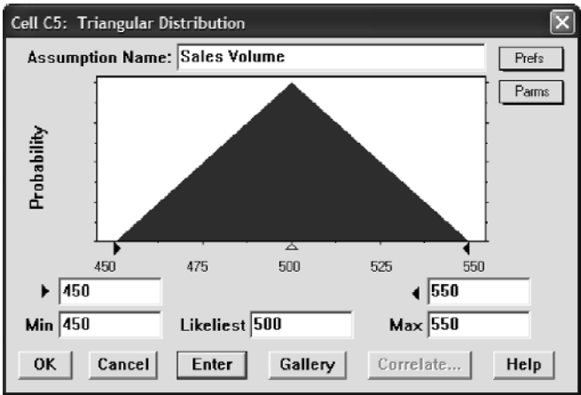
FIGURE 2.7 Triangular distribution for sales volume.
