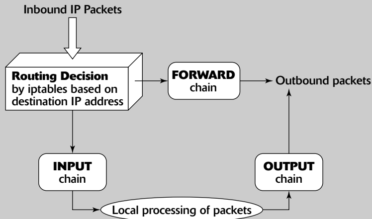
Figure 22-10: Simplified View of the iptables Processing Chains.
