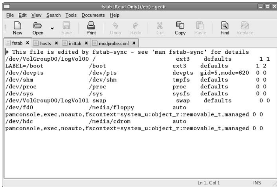
Figure 10-1: Editing Several Files with gedit .
