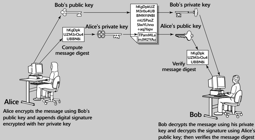
Figure 22-4: Alice Can Digitally Sign Her Message So That Bob Can Tell It's Really from Her.
