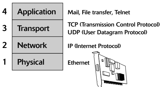
Figure 6-2: A Simplified Four-Layer TCP/IP Networking Model.
