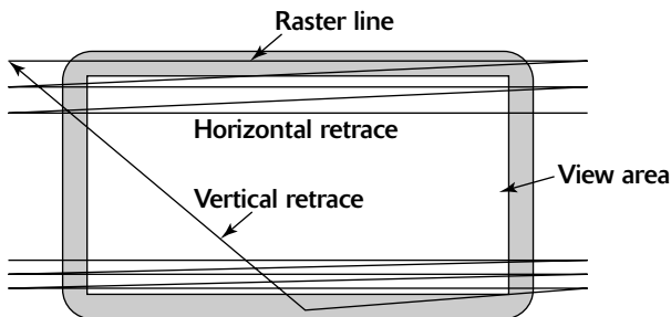
Figure 3-1: A Typical Raster-Scan Display.
