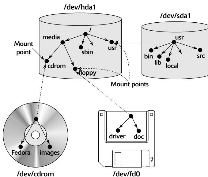
Figure 12-6: Mounting Devices on the Linux File System.
