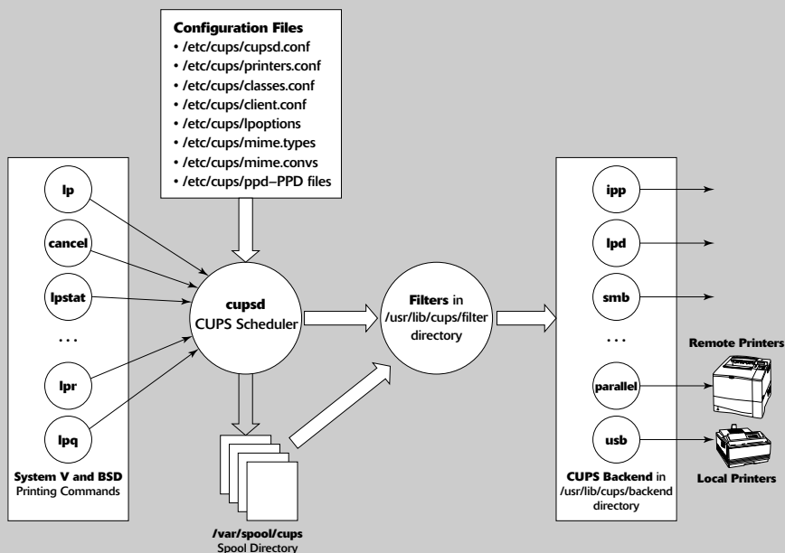
Figure 4-8: The CUPS Architecture.
