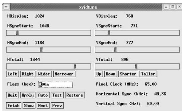
Figure 3-7: Adjust ModeLine Parameters from the Main Window of xvidtune.
