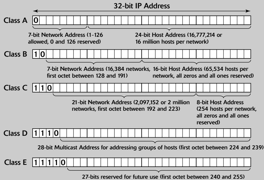
Figure 6-3: Classes of IP Addresses.
