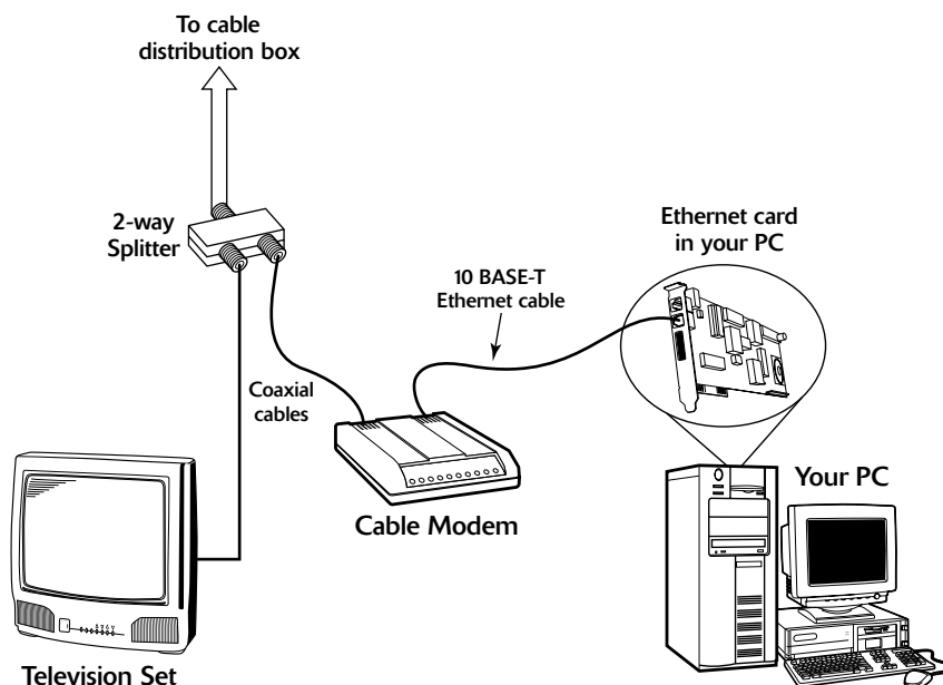
Figure 13-5: Splitting the Cable TV Signal between the TV and the Cable Modem.
