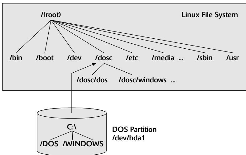
Figure 12-7: Mounting a DOS/Windows FAT Partition on the /dos Directory.
