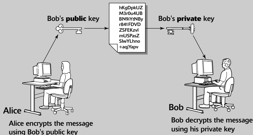
Figure 22-3: Bob and Alice Can Communicate Securely with Public-Key Encryption.
