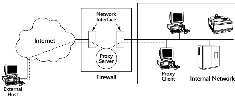
Figure 22-8: A Proxy Server Lets Internal Hosts Access Internet Servers.
