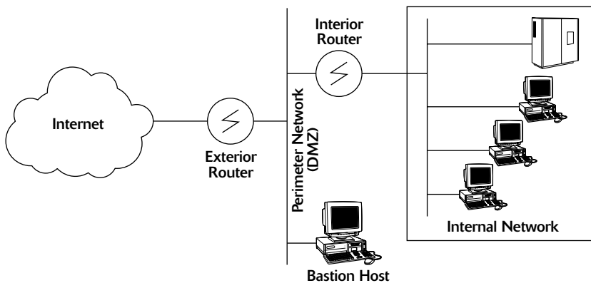
Figure 22-7: A More Complete Internet Firewall Includes a Perimeter Network and Bastion Hosts.
