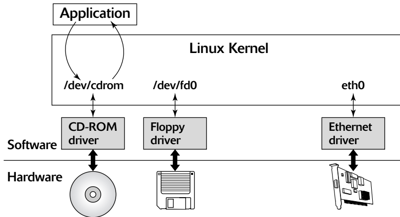
Figure 20-2: Application Accessing Devices through Device Drivers.
