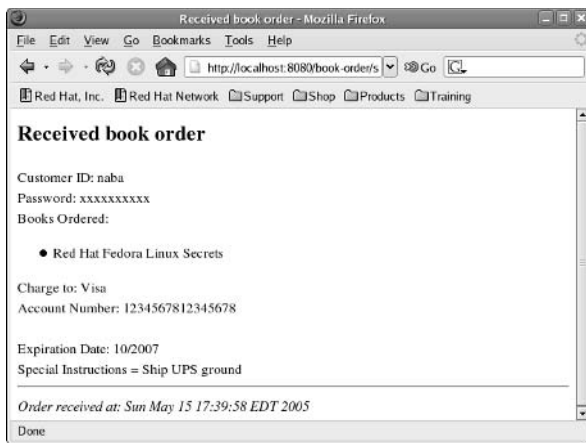
Figure 26-10: The OrderBooks Servlet Displays What the User Entered in the Book Order Form.
