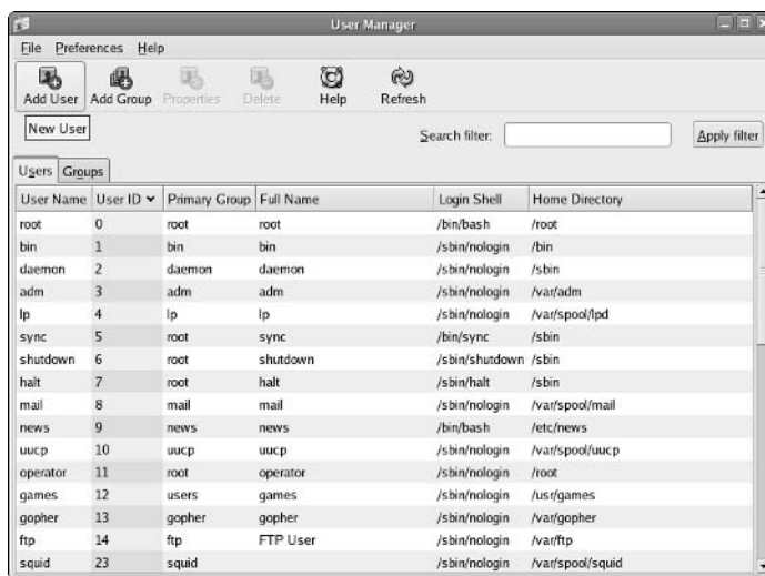
Figure 12-2: User Manager Window.
