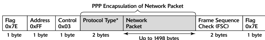
Figure 13-10: The Format of a PPP Frame.
