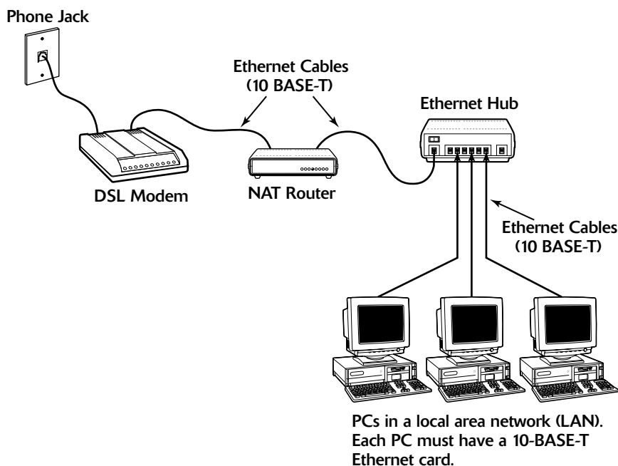
Figure 13-3: Connecting a LAN to the Internet through a NAT Router and DSL Modem.
