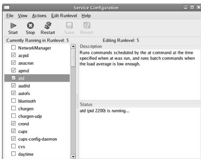
Figure 20-1: Using the Service Configuration Utility to Select the Services You Want to Start Automatically.
