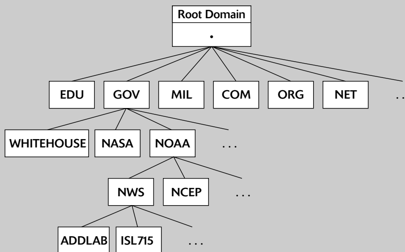
Figure 6-5: Part of the Internet Domain-Name Hierarchy.
