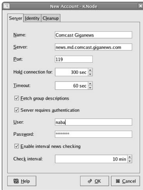
Figure 16-2: Enter Information about the News Server in This Dialog Box.
