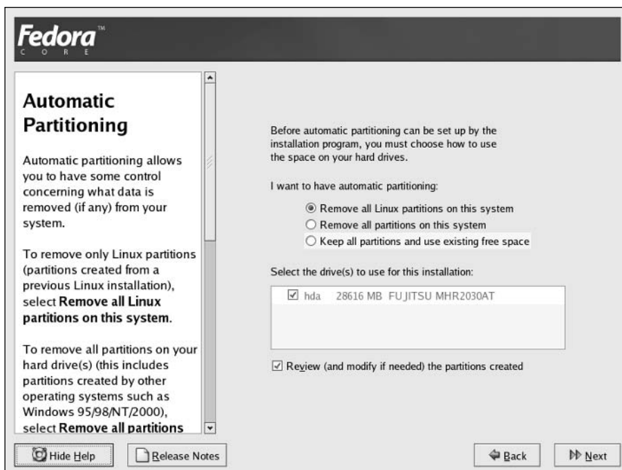
Figure 2-2: Selecting Automatic Partitioning Options during Linux Installation.
