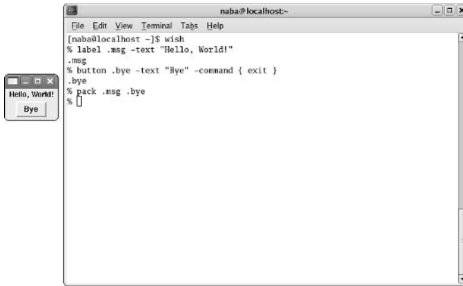
Figure 25-2: Interactively Creating a Label and a Button in wish.
