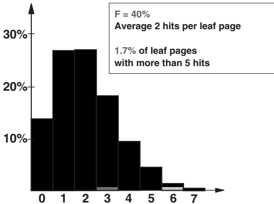
Figure 11.5 Effect of random inserts.
