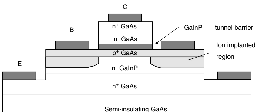
Figure 2.28. Structure of collector-up tunneling-collector HBT designed for low turn-on voltage.
