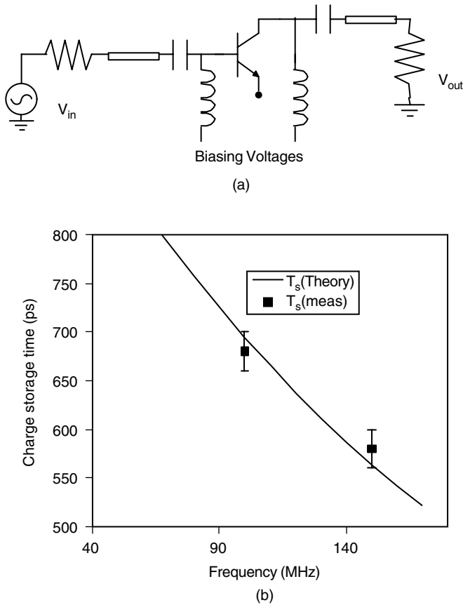
Figure 2.25. (a) Experimental system for the measurement of saturation charge storage in HBTs. (b) Measured saturation charge storage time using various measurement frequencies. The data may be fit with a recombination lifetime value of 1.9 ns.
