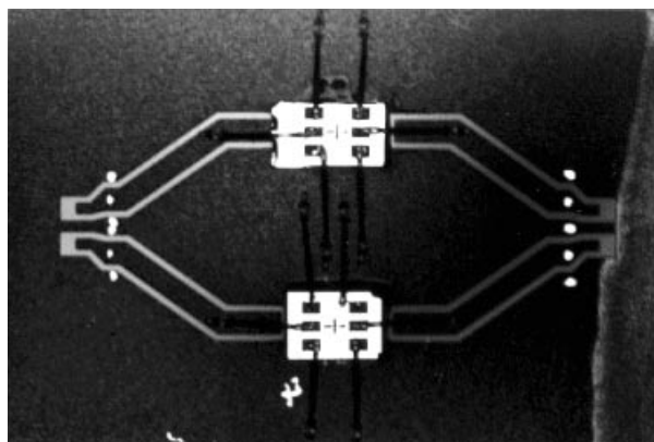
Figure 3.21. Micrograph of fabricated NPN/PPN push-pull common-emitter amplifier.
