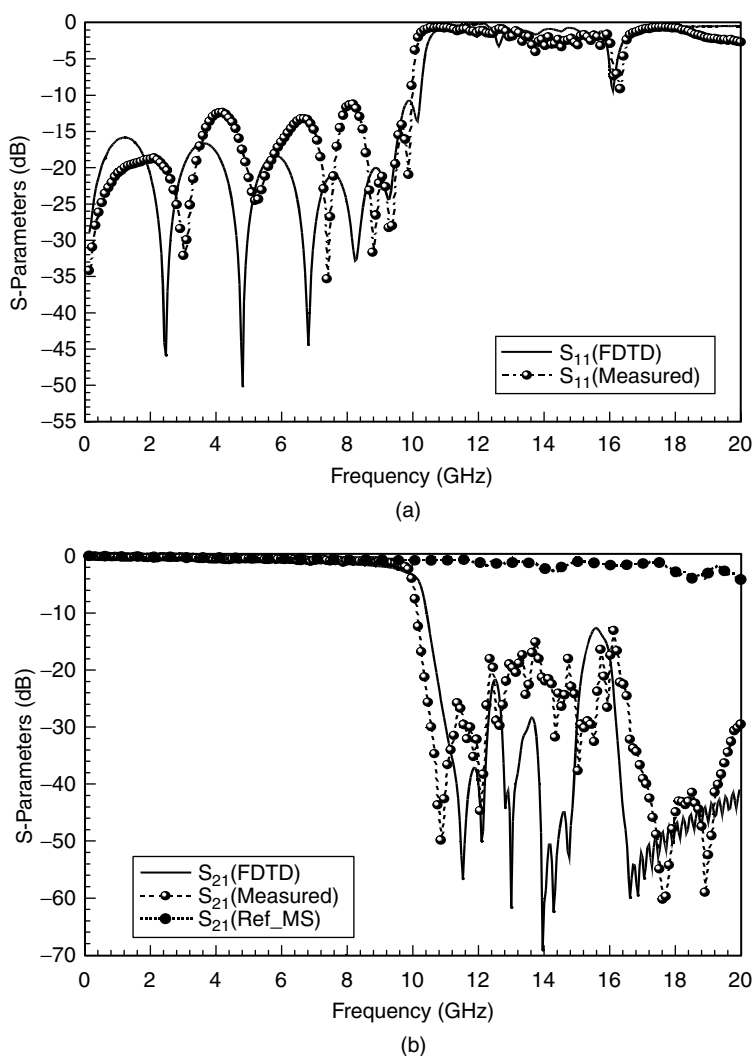
Figure 8.24. Comparison of simulation and measurement results of (a) S_{11} and (b) S_{21} of the microstrip line on the UC-PBG ground plane.
