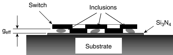
Figure 10.25. Schematic diagram of the effective air gap due to inclusions on the \text{Si}_3\text{N}_4 layer.
