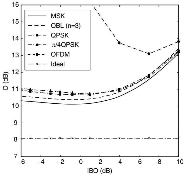
Figure 7.8. Figure of merit for various modulation schemes ( W'/R_b = 1.35 and \text{BER} = 10^{-3} ).
