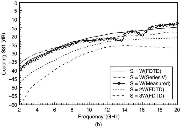
Figure 8.4. Simulation and measurement results of coupling between two 50\,\Omega microstrip lines with various line spacings.
