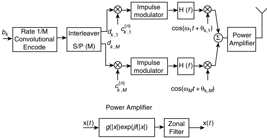
Figure 1.18. Transmitter block diagram for user k .
