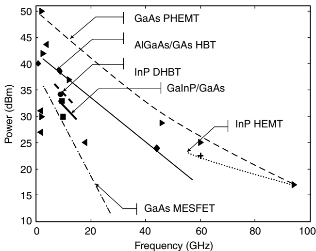
Figure 3.14. Power performance of HEMTs, MESFETs, and HBTs as a function of frequency.
