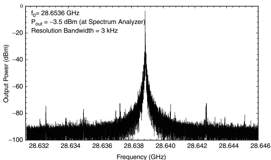
Figure 11.19. Measured micromachined oscillator spectrum. The power is defined at the spectrum analyzer port.
