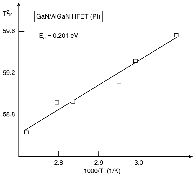
Figure 5.16. Results of DLTS measurements shown for GaN HFET grown on SiC substate. The time constant for this measurement was t_p = 100 \mu\text{s} .
