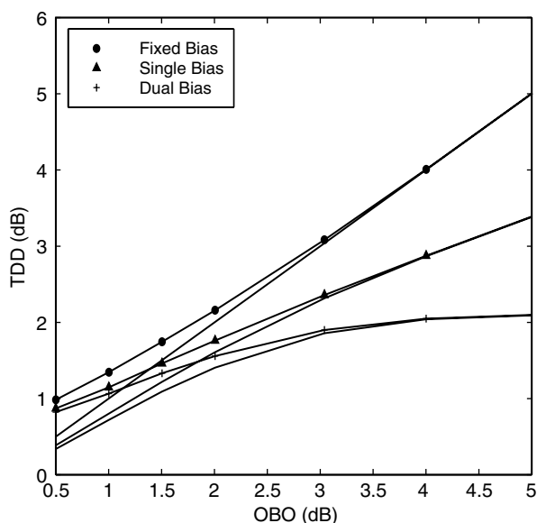
Figure 7.12. Total dc power degradation as a function of output backoff for QPSK.
