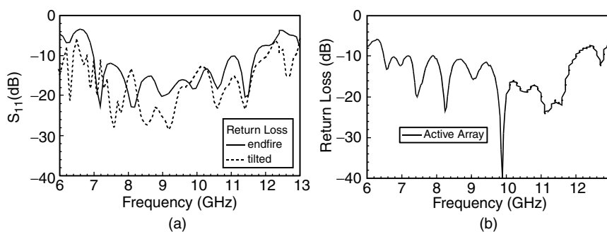
Figure 9.22. Measured input return loss of (a) passive eight-element arrays and (b) active eight-element array.
