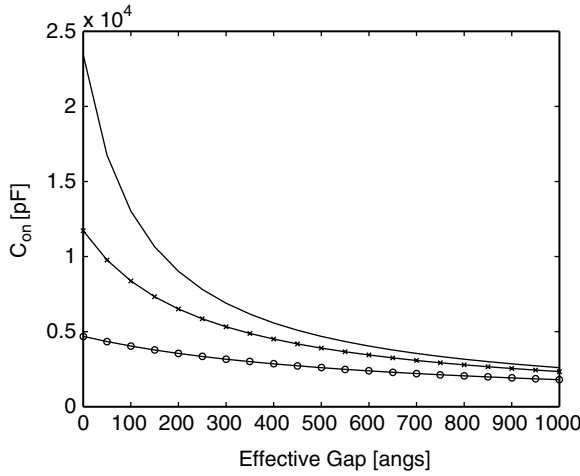
Figure 10.26. Plot of C_{\text{on}} versus g_{\text{eff}} for \text{Si}_3\text{N}_4 thicknesses of 500 Å (—), 1000 Å (×), and 2500 Å (○).
