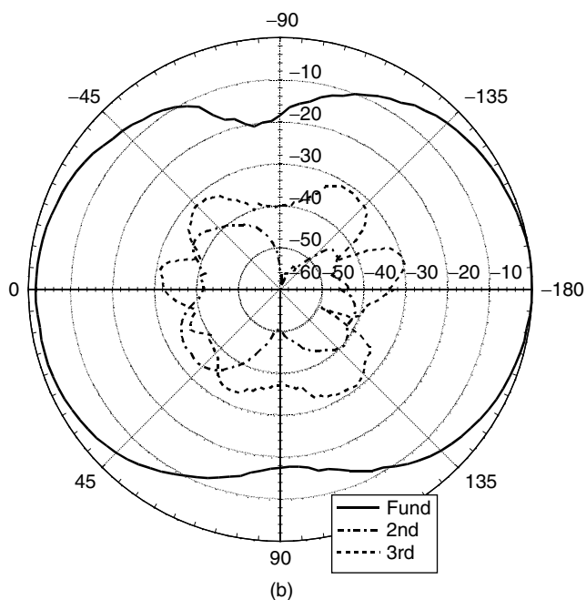
Figure 9.30. Measured data for slot-antenna based push-pull. In (a), a maximum PAE of 63% is achieved. In (b), harmonic suppression is demonstrated to be -30 dB below the fundamental in all planes. Note that the harmonics are calibrated to the fundamental power using the Friis transmission equation.
