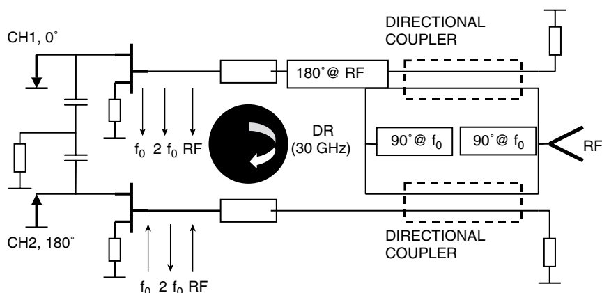
Figure 9.31. Architecture of 60 GHz second harmonic SOM.
