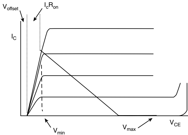
Figure 2.12. Schematic I - V curve of HBT for power amplifier application.
