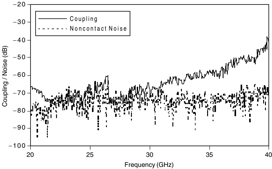
Figure 8.13. Measured crosstalk of the coupled lines shown in Figure 8.11(b), with the idling ports open-circuited.
