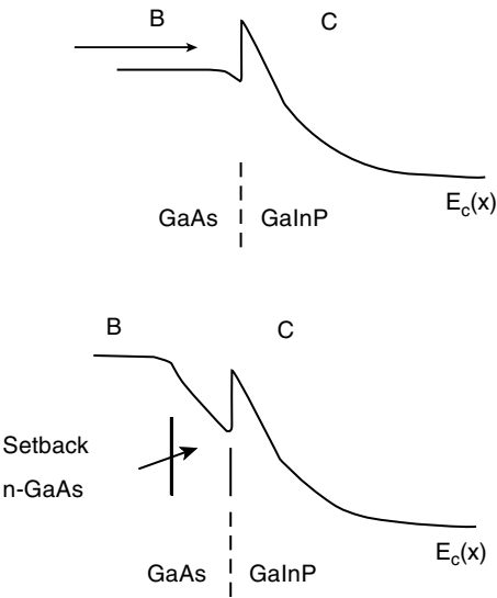
Figure 2.19. Schematic diagram of conduction band near BC junction, indicating the potential barrier formed as a result of \Delta E_c (with and without a setback layer of GaAs).
