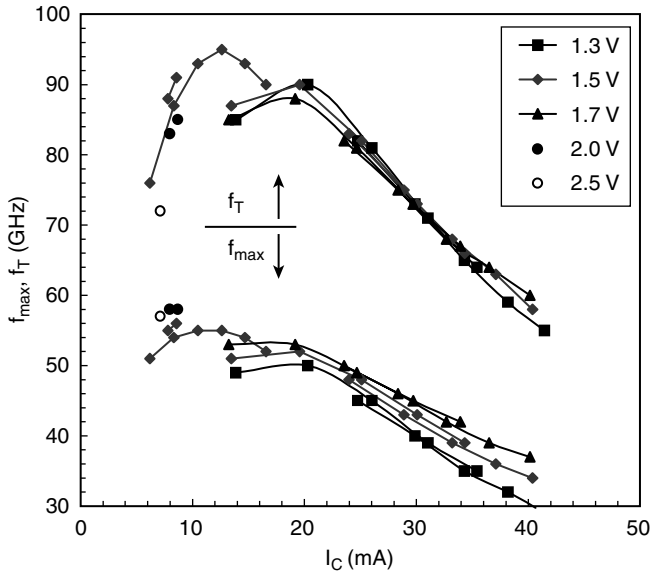
Figure 3.8. Dependence of f_T and f_{\text{max}} on dc bias I_C and V_{\text{CE}} for a 2 \times 10 \mu\text{m}^2 HBT. Four identical HBTs were measured, two at low current densities and two at high current densities.
