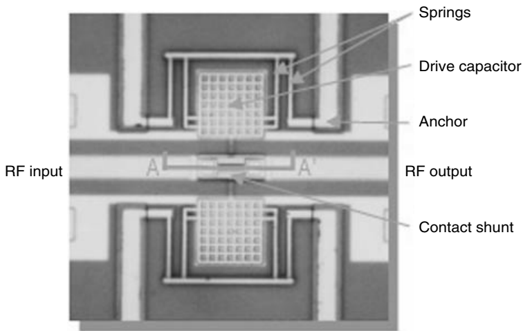
Figure 10.3. Rockwell Science Center's microrelay [4].
