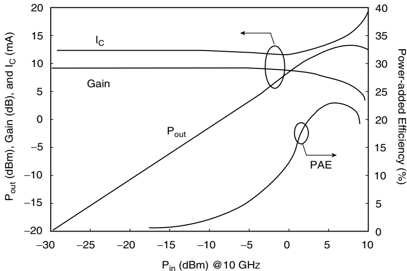
Figure 3.12. Power characteristics of 5 \times 10 \mu\text{m}^2 HBT from Wafer R under constant V_{EB} bias with V_{EC} = 4.0 V. Maximum P_{out} = 0.49 \text{ mW}/\mu\text{m}^2 and PAE = 24\% .
