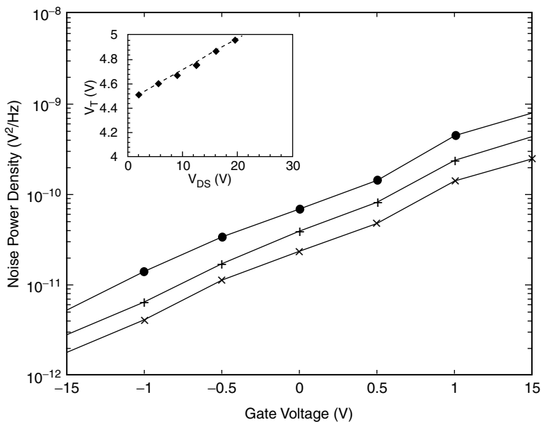
Figure 5.9. Noise power spectral density as a function of the gate bias in the linear regime of operation. The results are shown for three frequencies f = 0.1, 0.3 , and 0.6 kHz, from the upper to lower curve, respectively. Inset shows the threshold voltage dependence on V_{DS} . (After Balandin et al. [14]. Copyright © 1999 IEEE; reprinted with permission)
