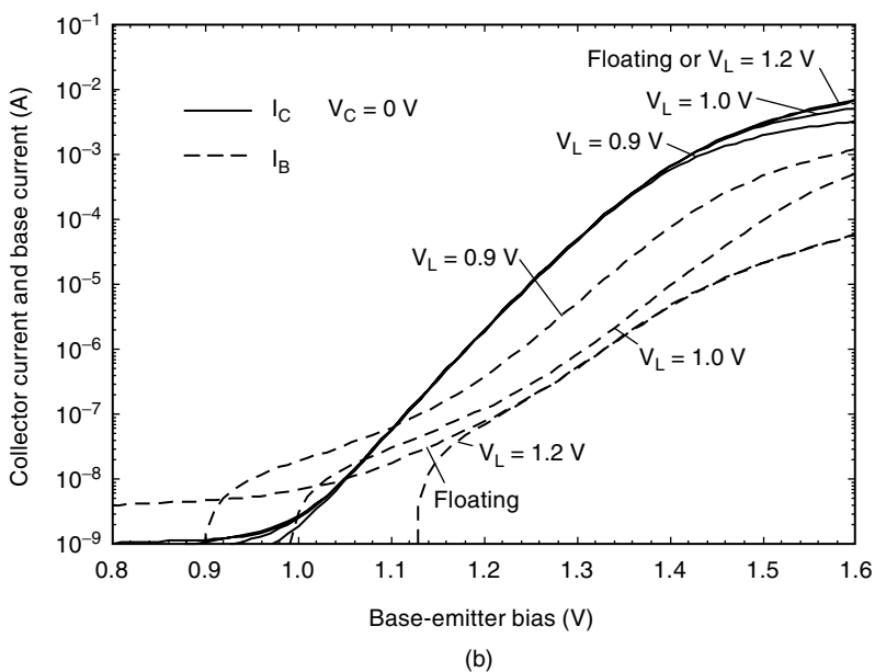
Figure 2.5. Representative Gummel plots measured for (a) Type-A HBTs and (b) type-B HBTs with various V_L bias voltages.
