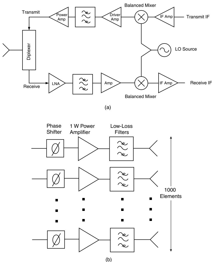
Figure 11.1. Typical millimeter-wave (a) transceiver front-end block diagram and (b) new generation K-band phased array for satellite communications.
