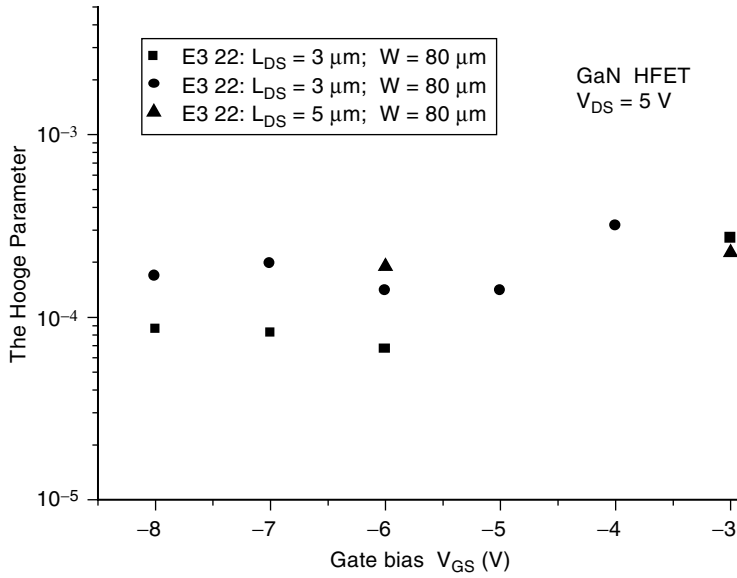
Figure 5.4. Hooe parameter \alpha_H as a function of the gate bias. The results are shown for three devices biased at V_{DS} = 5 V. The gate dimensions are 0.25\ \mu m by 80\ \mu m . (After Balandin et al. [14]. Copyright © 1999 IEEE; reprinted with permission)
