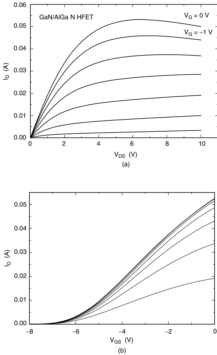
Figure 5.2. The dc current-voltage characteristics for GaN HFET (E432). The gate width W=80\text{ }\mu\text{m} , the gate length L_G=0.25\text{ }\mu\text{m} , and the drain-source separation distance L_{DS}=4\text{ }\mu\text{m} . (a) The gate bias V_{GS} is used as a parameter and it changes from 0 V (top curve) with a step of -1 V. (b) The drain bias V_{DS} varies from 0 V (bottom curve) with a step of +1 V. (After Balandin et al. [14]. Copyright © 1999 IEEE; reprinted with permission)
