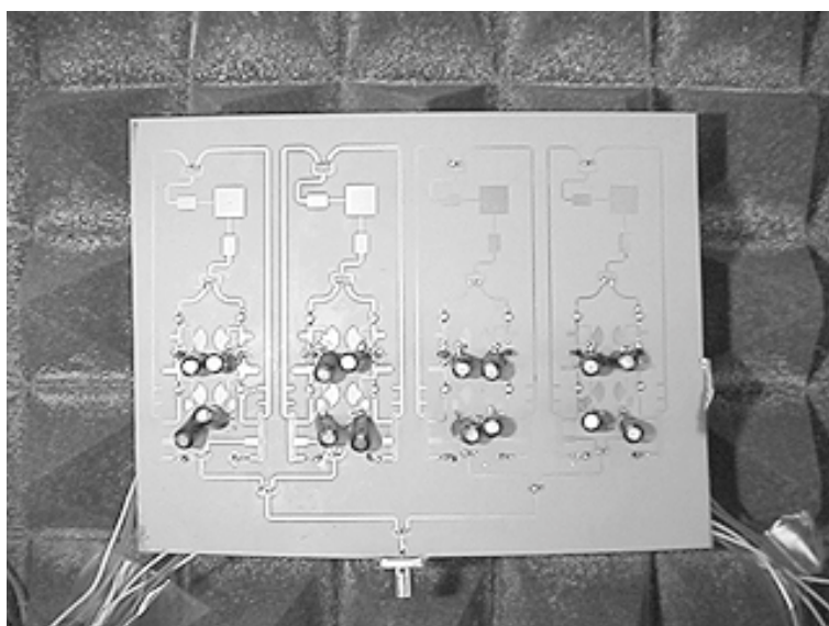
Figure 9.38. Details of active retrodirective array with conversion gain including (a) layout of active mixer and (b) photograph of prototype four-element array.
