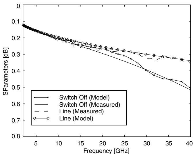
Figure 10.20. Comparison of the measured (—) and modeled (×) insertion loss of a FGCPW line with no switch and a FGCPW line with switch off.
