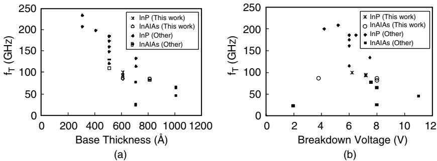
Figure 3.5. Published values of f_T versus (a) base thickness and (B) breakdown voltage \text{BV}_{CE0} for InP-based NPN SHBTs with InP and InAlAs emitters.
