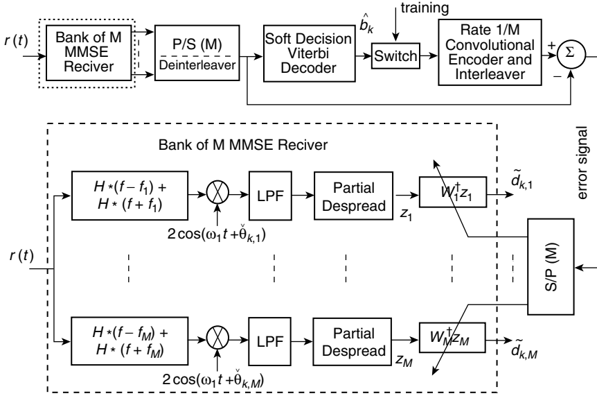
Figure 1.21. Receiver block diagram for user k [5].
