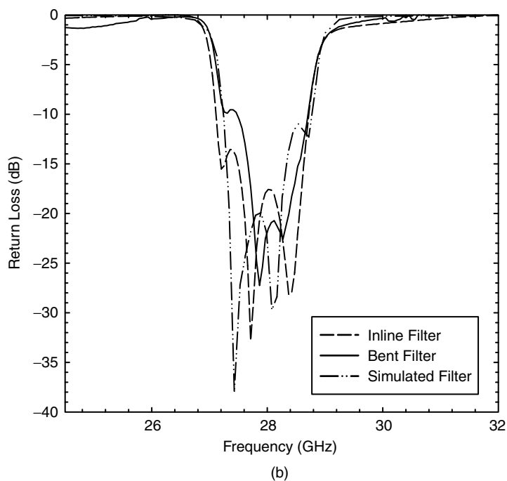
Figure 11.10. Comparison of the inline, bent, and simulated single four-pole filter response: (a) insertion loss and (b) return loss.
