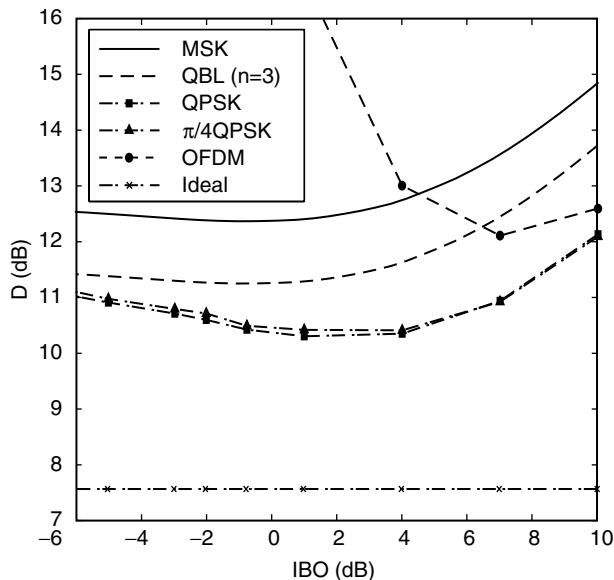
Figure 7.9. Figure of merit for various modulation schemes ( W'/R_b = 0.675 and \text{BER} = 10^{-3} ).
