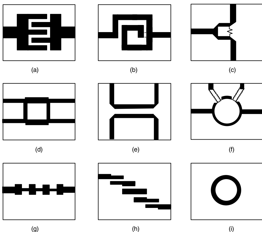
Figure 8.1. Examples of planar passive components based on microstrip line technology: (a) interdigitated capacitor, (b) spiral inductor, (c) Wilkinson power divider/combiner, (d) branch line coupler, (e) directional coupler, (f) rat-race ring coupler, (g) lowpass filter, (h) bandpass filter, and (i) ring resonator.
