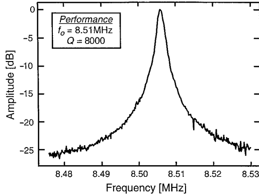
Figure 12.7. Frequency characteristic for an 8.5 MHz clamped–clamped beam polysilicon μmechanical resonator measured under 70 mtorr vacuum using a dc-bias voltage V_P = 10 V, a drive voltage of v_i = 3 mV, and a transresistance amplifier with a gain of 33 \text{ K}\Omega to yield an output voltage v_o . Amplitude = v_o/v_i . (From reference [18])
