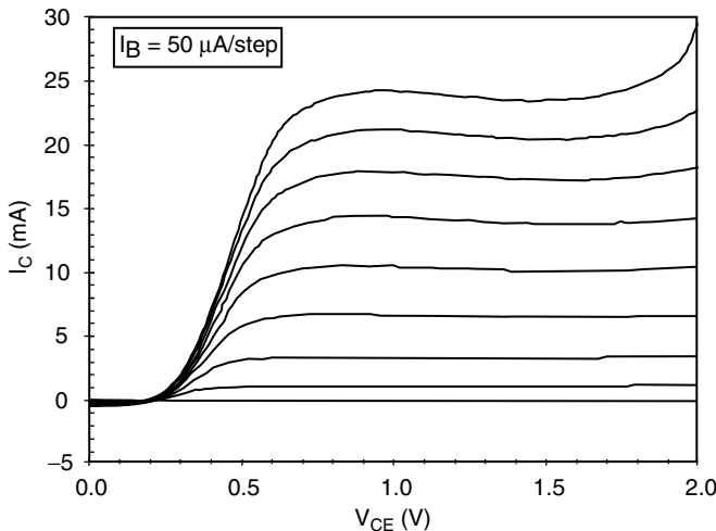
Figure 3.6. Common-emitter I_C – V_{CE} characteristics for 2 \times 10 \mu\text{m}^2 HBT from the reference Wafer A.
