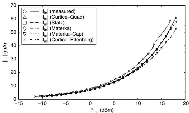
Figure 7.23. Measured and modeled fundamental drain current versus input power.
