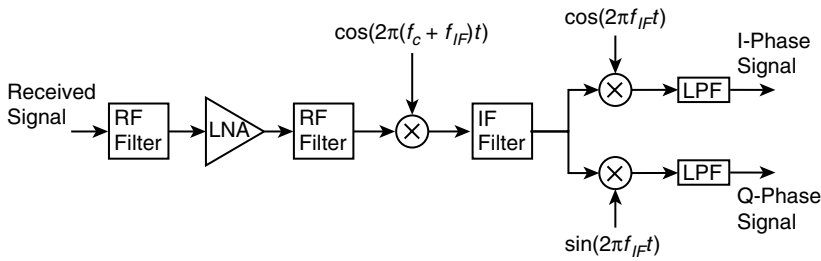
Figure 1.29. Superheterodyne receiver.
