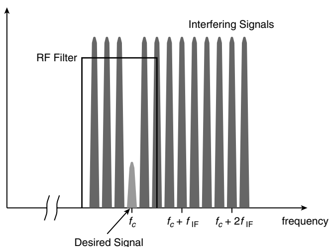
Figure 1.28. Received signal.
