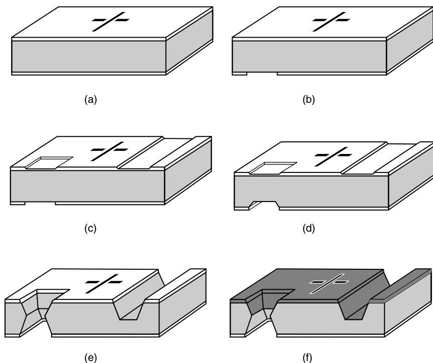
Figure 11.4. Fabrication of the ground plane wafer. (a) Alignment marks are deposited on a low-resistivity oxide wafer (oxide thickness = 1.2\text{ }\mu\text{m} ). (b) The back side is patterned and the oxide is etched in the pattern openings. (c) The front side of the wafer is patterned and 9000\text{ }\text{\AA} of oxide is etched. (d) The silicon is etched from the back of the wafer using the oxide as an etch mask. (e) Now 3000\text{ }\text{\AA} of oxide is etched from the entire sample, exposing the silicon on the front side. The sample is then etched until the ground plane is at the specified depth. (f) The oxide is stripped off the sample and the sample is metalized.
