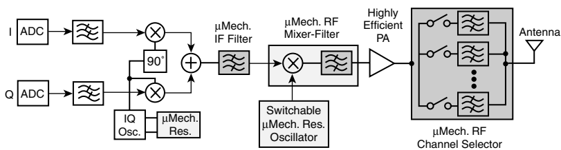
Figure 12.24. RF channel-select transmitter architecture, possible only if high-power \mu mechanical resonators can be achieved. Here, on-chip \mu mechanical blocks are shaded, and the PA is not necessarily implemented on-chip.
