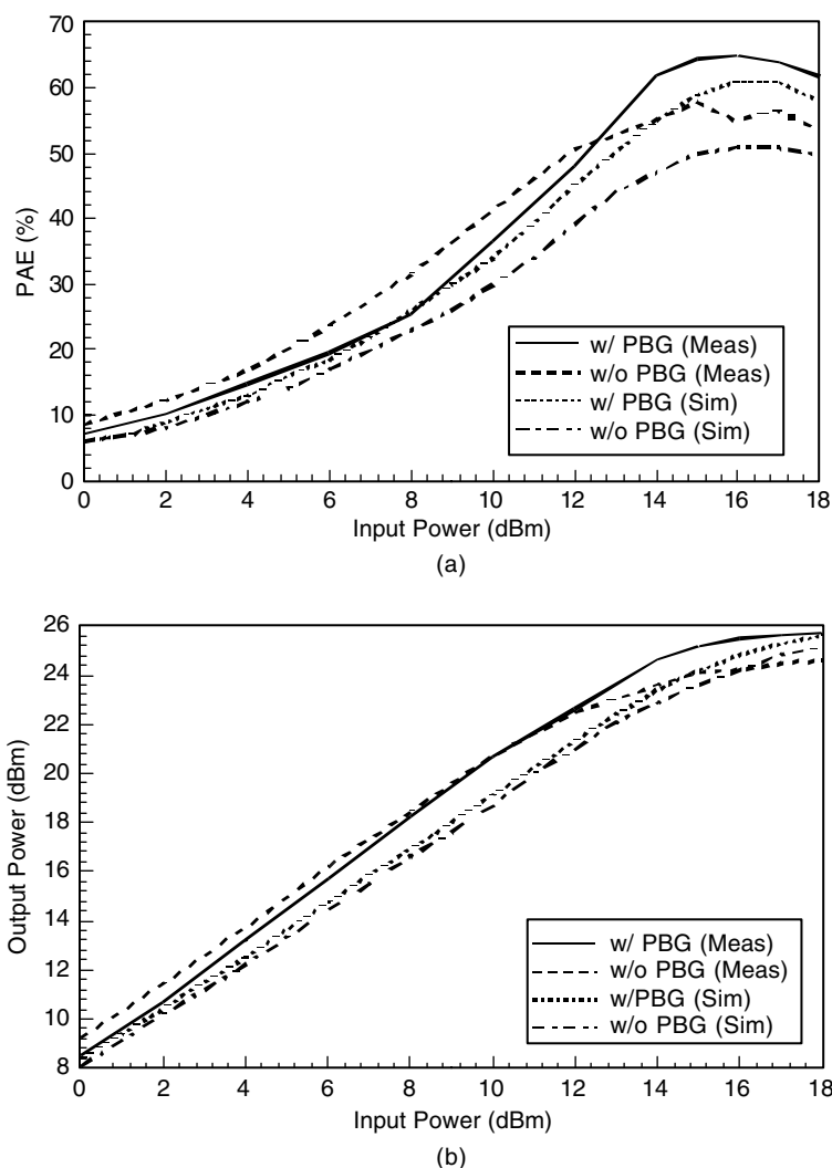
Figure 8.31. Simulation and measurement results of (a) PAE and (b) output power versus input power for the PBG and reference amplifier.
