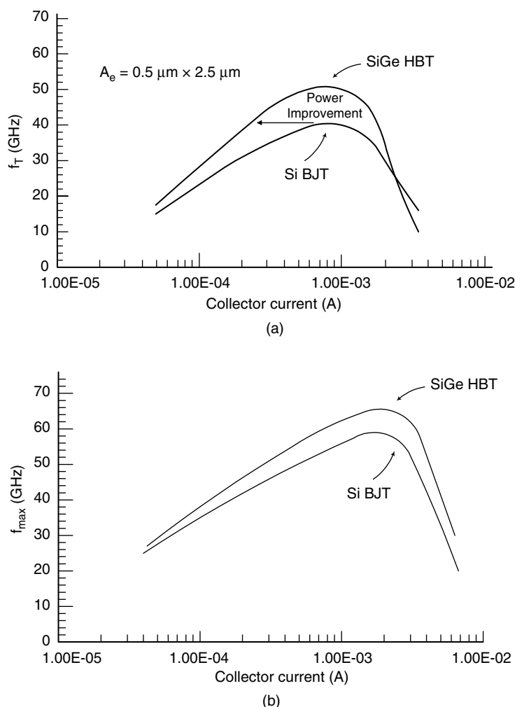
Figure 4.6. Comparison of epi-base Si/SiGe HBT and Si BJT with comparable base resistivity and geometry. (a) f_T versus collector current and (b) f_{max} versus collector current.
