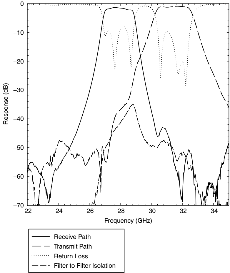
Figure 11.14. Summary of measured diplexer.
