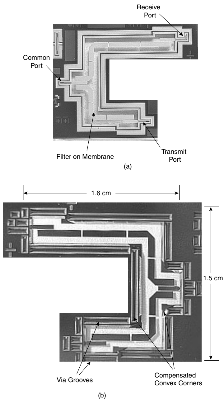
Figure 11.12. Fabricated K-band diplexer: (a) top view and (b) bottom view without the ground plane or shielding cavity.
