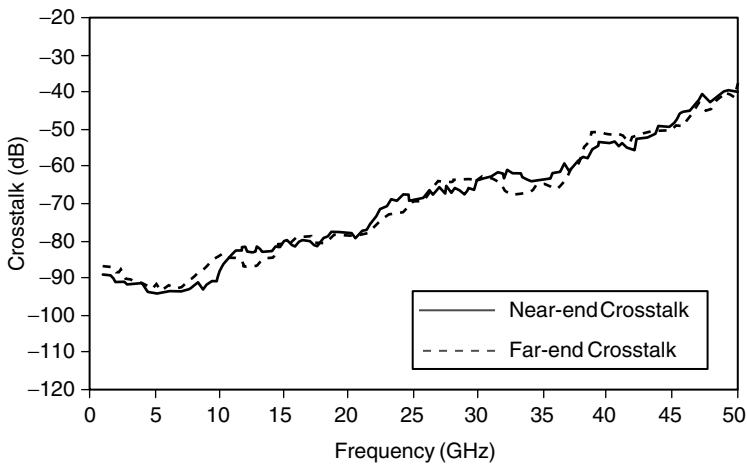
Figure 8.14. Measured crosstalk of an improved test structure of the coupled lines as shown in Figure 8.11(b), with the idling ports terminated by matched loads.
