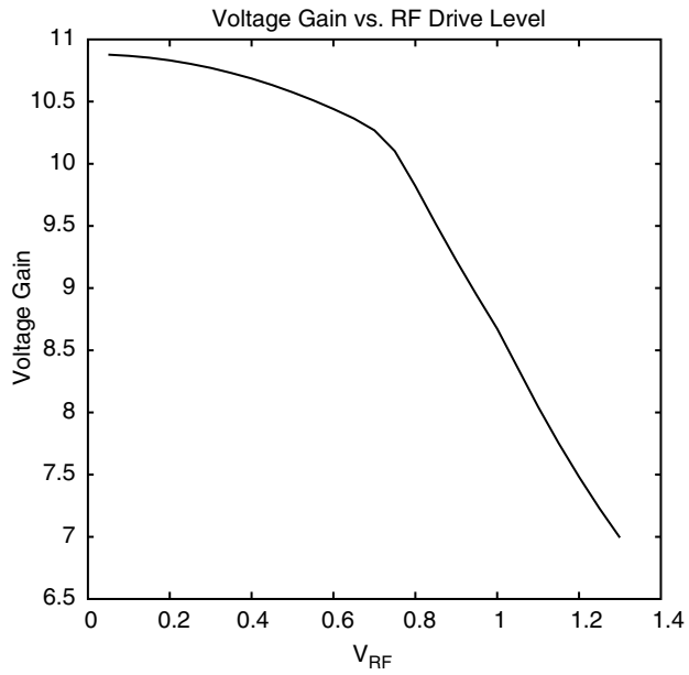
Figure 7.1. Voltage gain versus RF voltage drive level.
