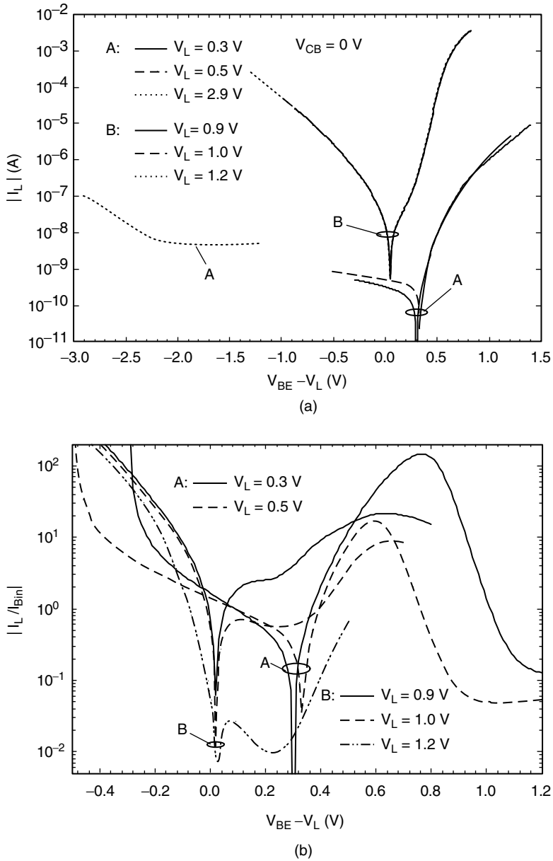
Figure 2.7. (a) Leakage current |I_L| and (b) the ratio |I_L/I_{Bin}| measured through the on-ledge Schottky potentiometer versus the offset voltage of V_{BE} - V_L .
