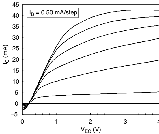
Figure 3.9. Forward I–V characteristics of 5 \times 10 \mu\text{m}^2 PNP HBTs from Wafer R with I_B = 0.5 \text{ mA/step} .
