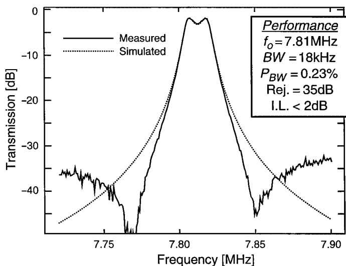
Figure 12.17. Measured spectrum for a terminated 7.81 MHz \mu mechanical filter with excessive input/output shunt capacitance. Here, Q_{\text{ftr}} = 435 . (From reference [18])
