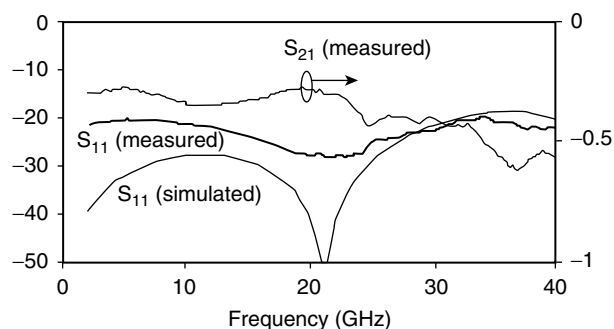
Figure 10.30. S-parameters for the four-switch network of Figure 10.27 with all switches off.
