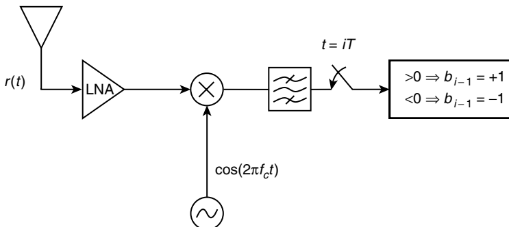
Figure 1.4. Receiver.
