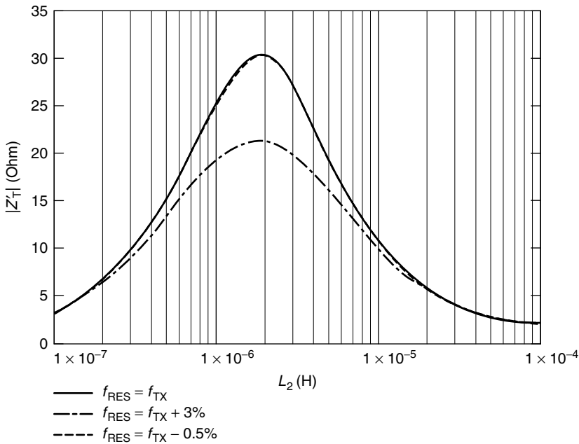
Figure 4.36 The value of Z'_T as a function of the transponder inductance L_2 at a constant resonant frequency f_{\text{RES}} of the transponder. The maximum value of Z'_T coincides with the maximum value of the Q factor in the transponder
