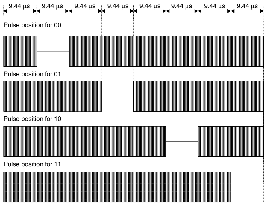
Figure 9.35 ‘1 of 4’ coding arises from the combination of eight time slots of 9.44\ \mu\text{s} length. The value of the digit to be transmitted in the value range 0–3 can be determined from the time position of a modulation pulse
