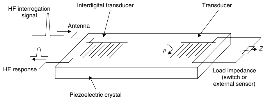
Figure 4.103 Principal layout of a passive surface wave transponder connected to an external sensor (reproduced by permission of Siemens AG, ZT KM, Munich)
