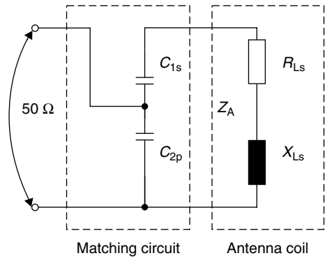
Figure 11.18 Simple matching circuit for an antenna coil
