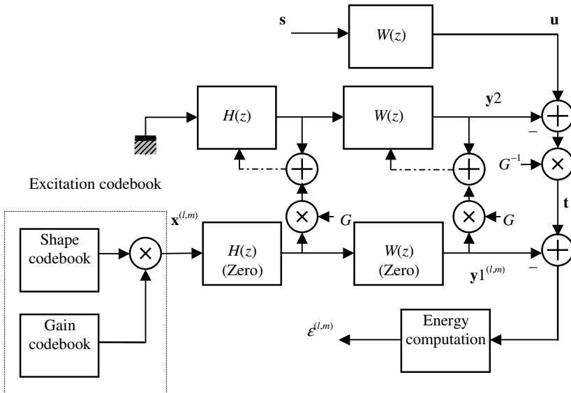
Figure 14.6 Another equivalent analysis-by-synthesis loop with reduced complexity.
