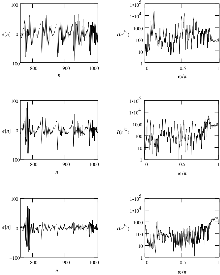
Figure 4.11 Plots of prediction error and periodograms for the voiced frame in Figure 4.6. Top: M = 3 . Middle: M = 10 . Bottom: M = 50 .
