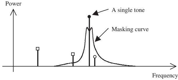
Figure 1.15 Example of the masking curve associated with a single tone. Based on the masking curve, examples of audible (□) and inaudible (○) tones are shown, which depend on whether the power is above or below the masking curve, respectively.
