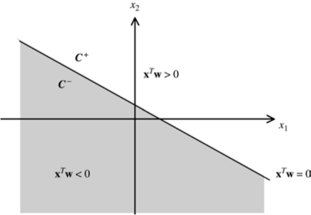
Figure D.2 Decision surface in a two-dimensional space.
