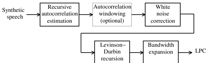
Figure 14.2 Procedure to obtain the LPCs for the synthesis filter.
