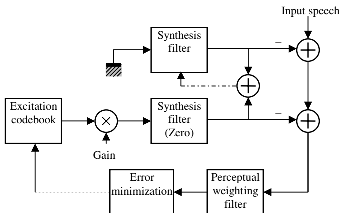
Figure 14.4 Analysis-by-synthesis loop of the LD-CELP encoder.
