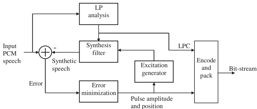
Figure 10.3 Encoder of a closed-loop multipulse coder.
