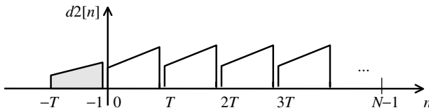
Figure 12.1 Extracting a codevector from the adaptive codebook when T < N : only the samples from -T to -1 are used and are periodically replicated to form the codevector.
