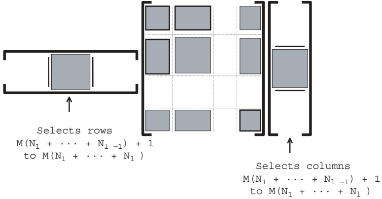
Figure 7.15 Illustration of the product \mathbf{S}_l^T \mathbf{Q} \mathbf{S}_l .
