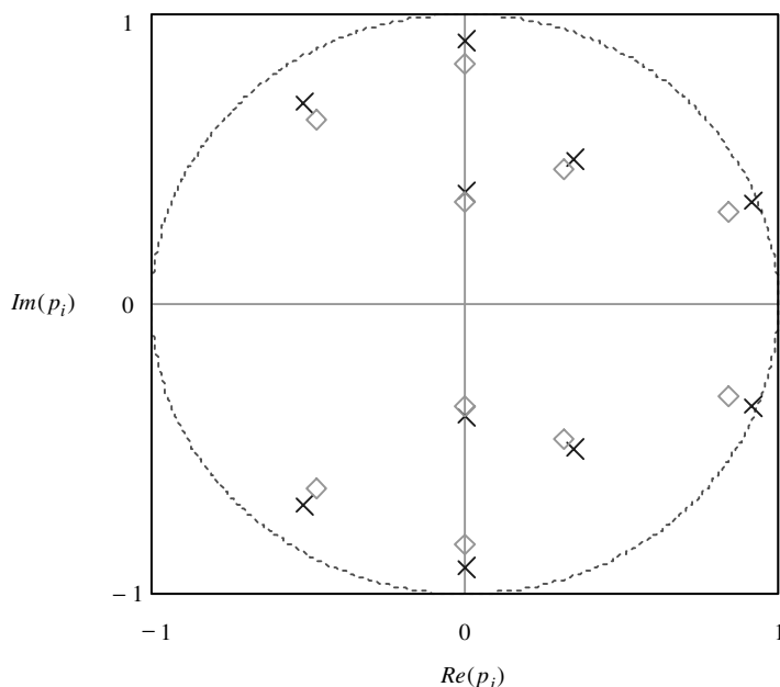
Figure 4.29 Plot of poles for the original (x) and bandwidth-expanded (◇) synthesis filters.
