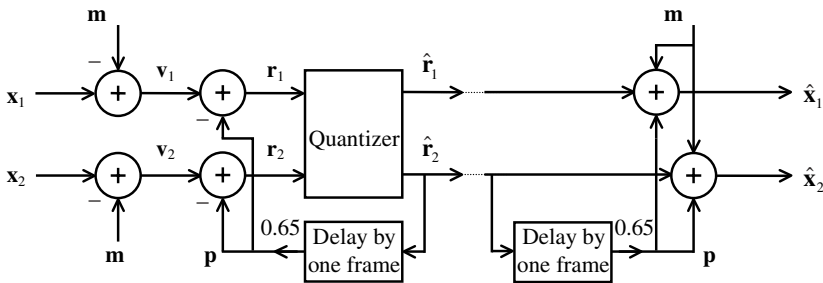
Figure 15.14 Illustration of LSF quantization for the GSM EFR coder.
