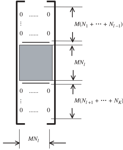
Figure 7.14 General form of the shifting matrix \mathbf{S}_l . The shaded area represents an M \cdot N_l \times M \cdot N_l identity matrix.
