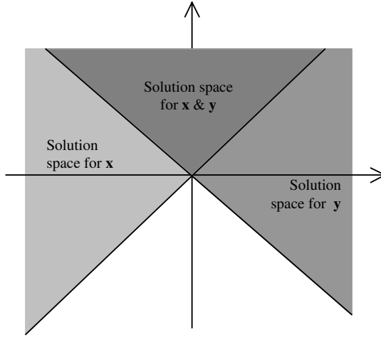
Figure D.5 Example of solution space for two patterns.
