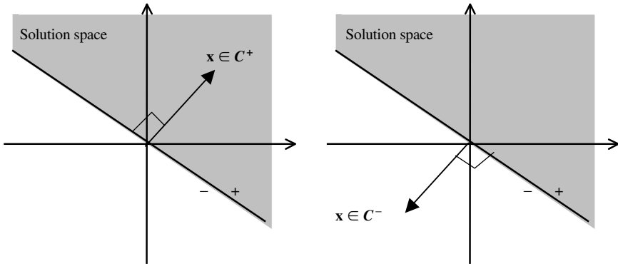
Figure D.4 Left: Solution space for \mathbf{x} \in C^+ . Right: Solution space for \mathbf{x} \in C^- .
