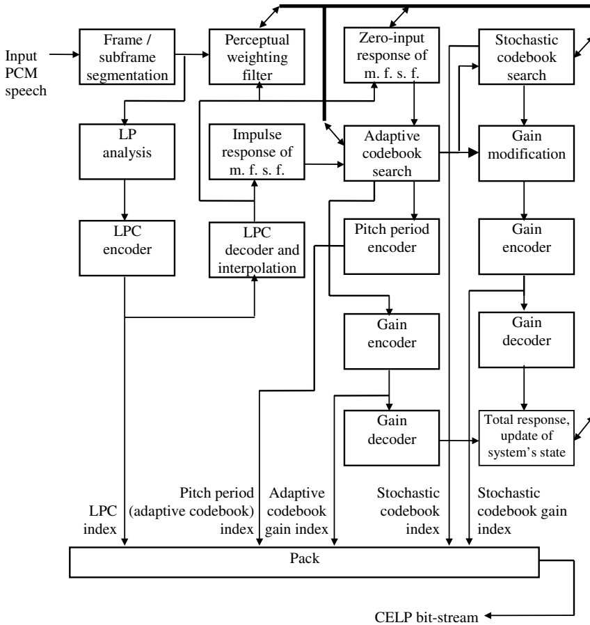
Figure 12.11 Block diagram of the FS1016 CELP encoder (m. f. s. f. means modified formant synthesis filter).
