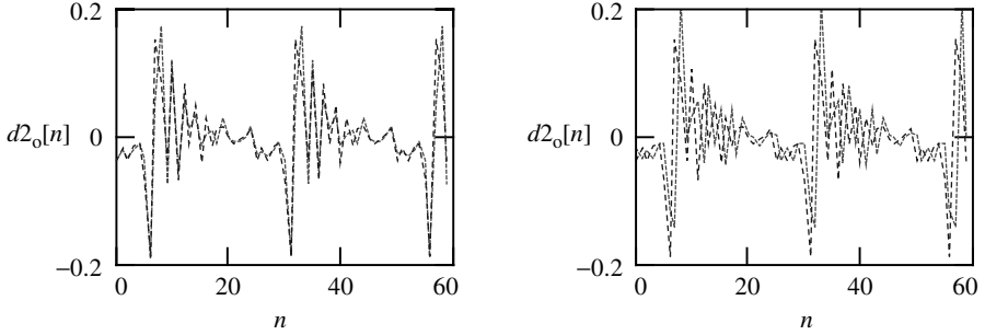
Figure 12.9 Adaptive codevector at t = 25 . The signal is derived from the same codebook samples as in Figure 12.3. Two fractional delay values are considered: \frac{1}{4} (left) and \frac{3}{4} (right). The original codevector with no fractional delay is plotted for comparison (dotted line).
