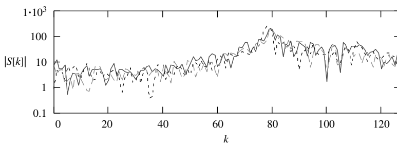
Figure 1.11 Comparison between the magnitude of the DFT for the three signal frames of Figure 1.10.
