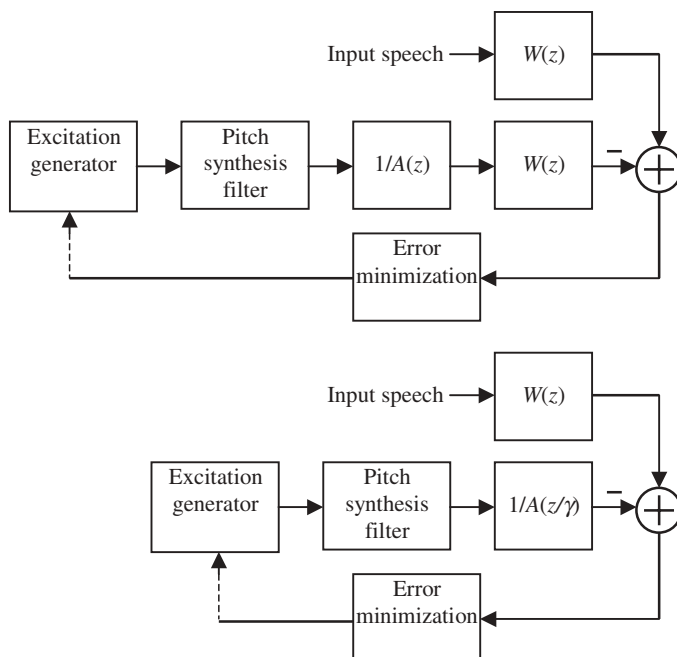
Figure 11.8 Equivalent realizations of the system in Figure 11.5. Top: By translating the perceptual weighting filter. Bottom: After merging the formant synthesis filter with the perceptual weighting filter.
