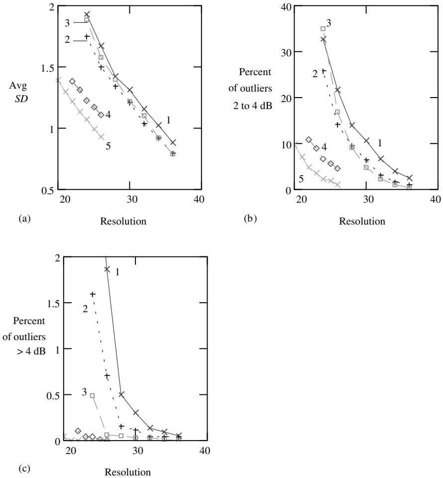
Figure 8.22 Plots of quantization performance for five different schemes: (a) average SD, (b) percentage of outliers having SD between 2 and 4 dB, and (c) percentage of outliers having SD > 4 dB. Data from Paliwal and Kleijn [1995], Tables 2, 3, 5, 8, and 9.
