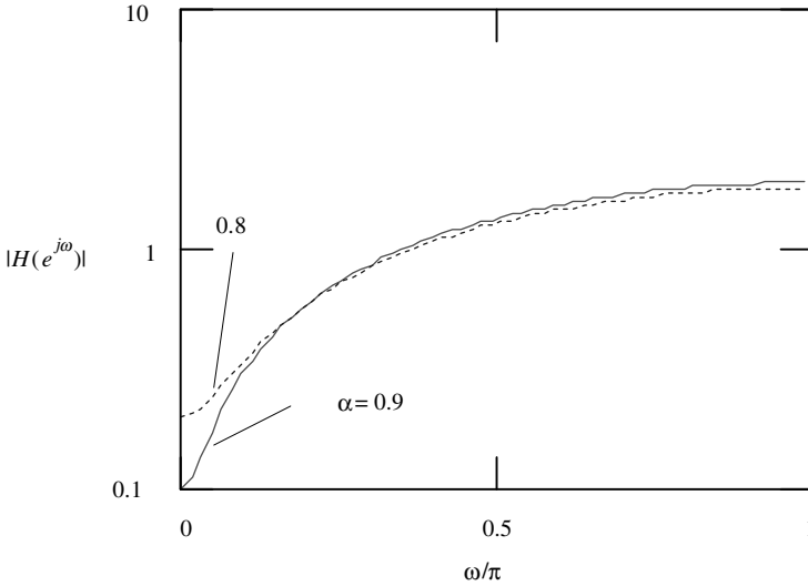
Figure 4.27 Magnitude plots of the transfer functions of the pre-emphasis filter.
