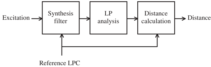
Figure 9.11 Setup of an experiment in LP analysis.
