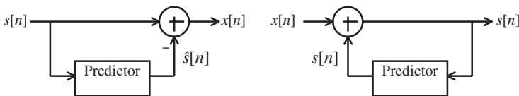
Figure 4.33 Block diagram of the AR analyzer filter ( left ) and synthesizer filter ( right ).
