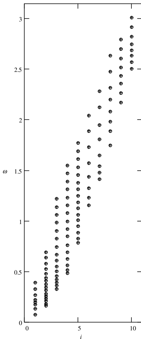
Figure 8.16 Plot of LSF quantization codewords for the FS1016 coder. Data from National Communications System [1992], Table 8.
