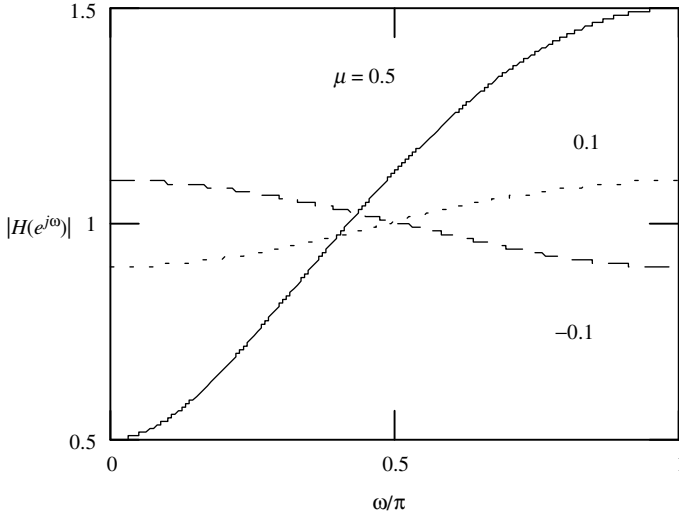
Figure 11.18 Plots of the magnitude of the system function H(z) = (1 - \mu z^{-1}) for three values of \mu .
