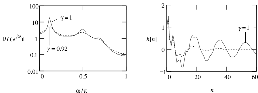
Figure 4.28 Magnitude of the transfer function ( left ) and impulse response ( right ) of the original (solid line) and bandwidth-expanded (dotted line) synthesis filters.
