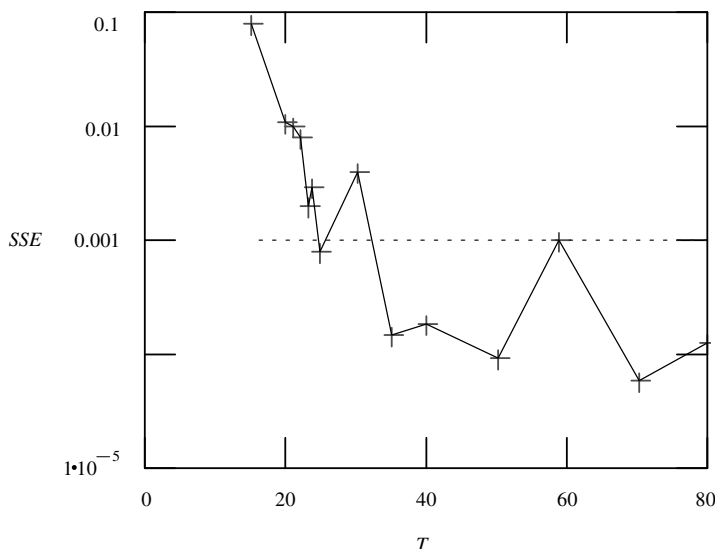
Figure 9.13 Sum of squared error (SSE) between the estimated and reference LPC as a function of the period of the excitation impulse train in a single experiment. The dotted line represents the SSE obtained from a single impulse input.
