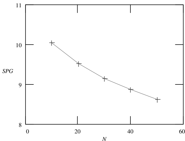
Figure 4.13 Segmental prediction gain (SPG) as a function of the frame's length ( N ) in an external prediction experiment.
