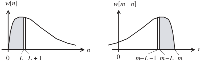
Figure 3.13 Chen window showing the nonrecursive and recursive portion ( left ), together with the time-reversed and -shifted version ( right ).
