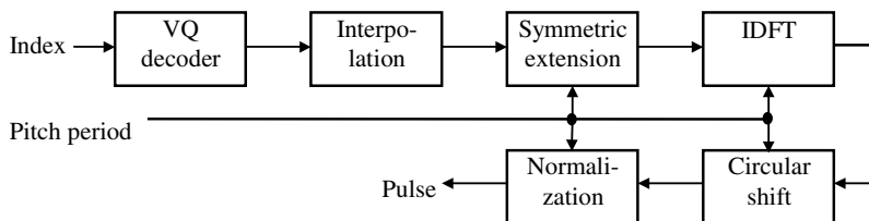
Figure 17.4 Block diagram of the excitation pulse generation procedure during decoding.
