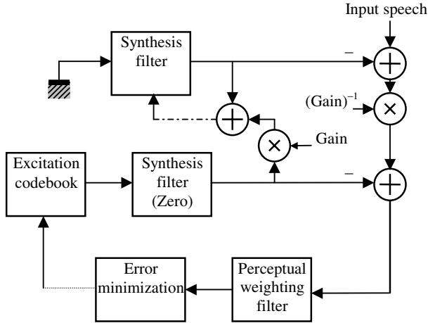
Figure 14.5 An equivalent analysis-by-synthesis loop.
