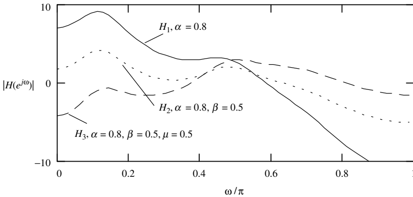
Figure 11.16 Some postfilter configurations and their magnitude responses.
