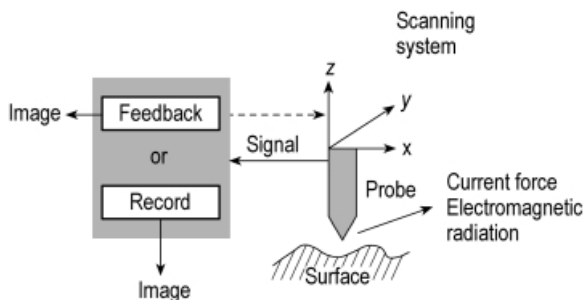
Fig. 5.1. General scheme of scanning probe microscopy.
