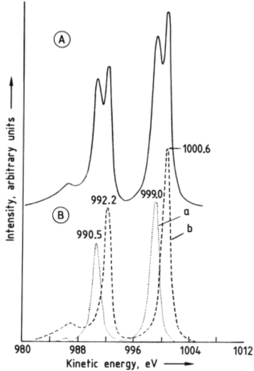
Fig. 2.8. Example of a chemical shift in the Sn 3d peak for a very thin layer of Sn oxide in Sn metal. (A) spectrum after linear background subtraction, (B) spectrum resolved into its respective components. (a) \text{Sn}^{n+} , (b) \text{Sn}^0 .
