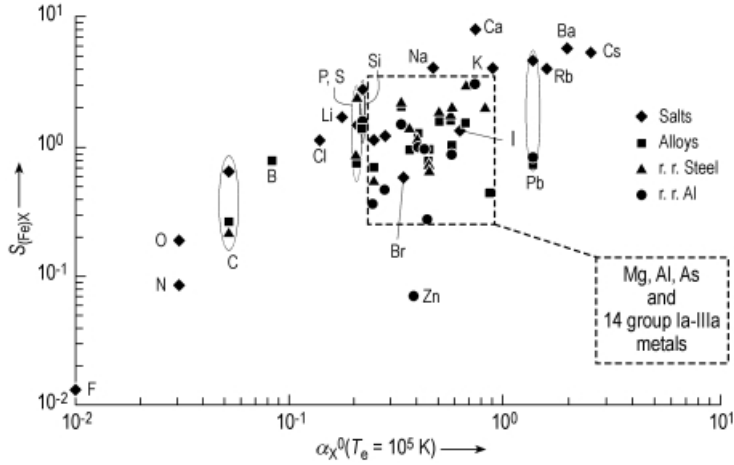
Fig. 3.36. Experimental, Fe-related HF-plasma SNMS sensitivity factors S_{(\text{Fe})X} with elements X ordered according to their post-ionization probabilities calculated according to [3.74]; from Ref. [3.71] (salts); [3.72] alloys, [3.73] round robins (r.r.).
