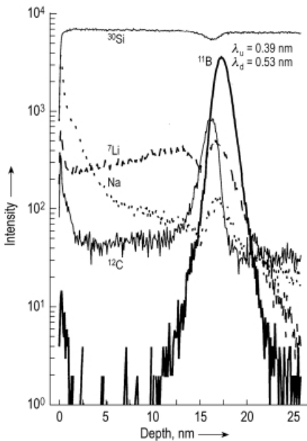
Fig. 3.17. Multi-element depth profile of a B layer in Si performed with 600-eV \text{SF}_5^+ sputtering [3.41].
