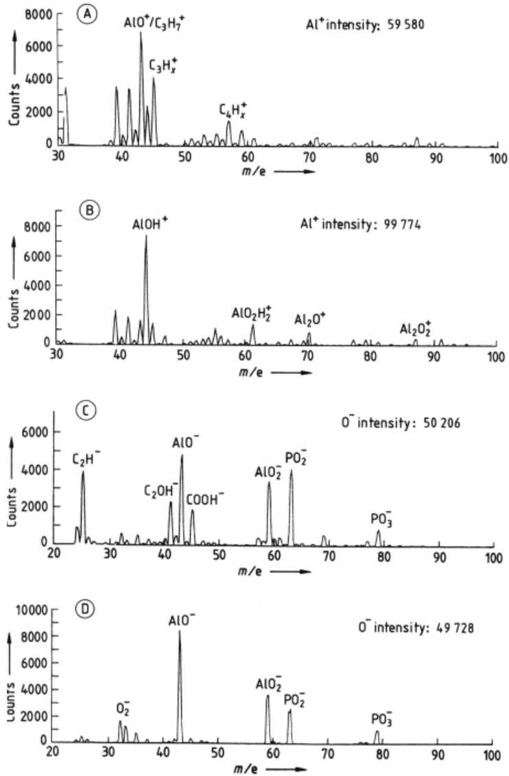
Fig. 3.8. SSIMS spectra from oxide films on aluminum after anodization in phosphoric acid for 3 or 5 s [3.18].
