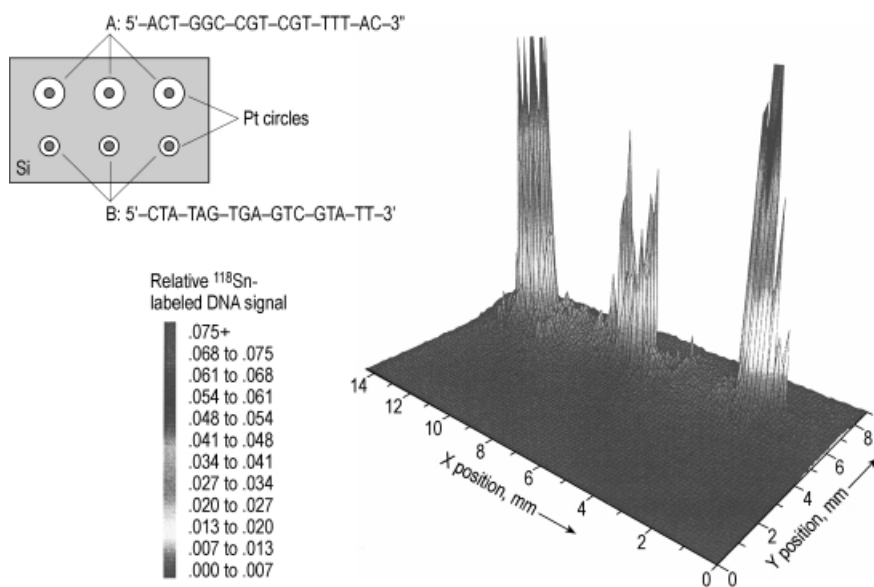
Fig. 3.46. ^{118}\text{Sn} image of Sn-labeled DNA hybridized to six oligonucleotide spots; three complimentary and three non-complementary.
