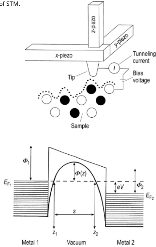
Fig. 5.12. Energy level diagram of a tunneling junction [5.34].
