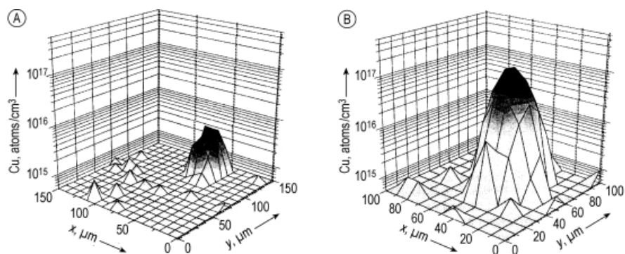
Fig. 3.45. R-laser-SNMS images of copper around (a) tellurium and (b) cadmium inclusions [3.116].
