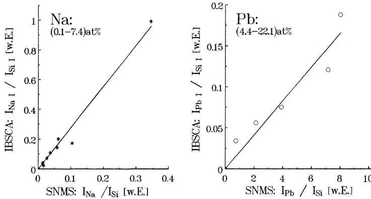
Fig. 4.49. Comparison of relative intensities measured with IBSCA and SNMS. Conditions: sputter equilibrium after bombardment with 5 keV \text{Ar}^+ ; the samples were oxitic glasses with different content of Na (0.1–7.4 at%) and Pb (4.4–22.1 at%).
