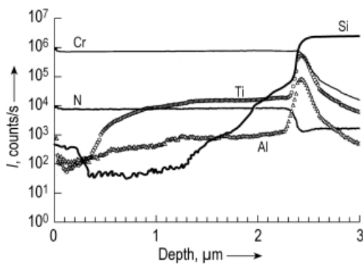
Fig. 3.27. Depth profile of CrN layer deposited on Si. Primary ions \text{O}_2^+ ; primary energy 5.5 keV; primary intensity 2 \mu\text{A} ; measuring time 1 h.
