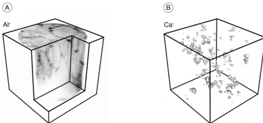
Fig. 3.29. 3D element distribution of powder metallurgically produced steel. Diameter of the cube 150 \mu\text{m} . Primary ions top 0.1 \mu\text{A Cs}^+ , bottom 2 \mu\text{A O}_2^+ ; depth top 1 \mu\text{m} , bottom 11 \mu\text{m} .
