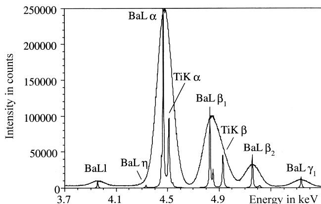
Fig. 4.25. A WDX spectrum of \text{BaTiO}_3 plotted against energy and compared with the corresponding EDX spectrum [4.91].
