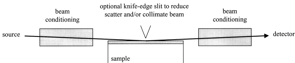
Fig. 4.33. Schematic diagram of the experimental arrangement for GXRR measurements. Beam-conditioning optics can include slits,
