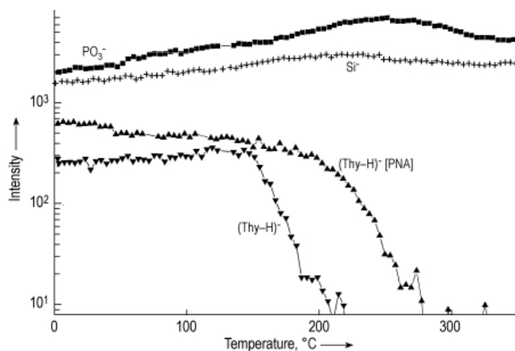
Fig. 3.13. TP SIMS measurements of an ODN ( c = 0.1 mm) and PNA ( c = 0.1 mm, curve labeled as PNA) TTTTCCTCTCTC-sequence [3.26].
