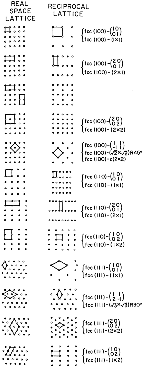
Fig. 2.48. Direct and reciprocal lattices of a series of commonly occurring two-dimensional superlattices. Open circles correspond to the ideal (1 \times 1) surface structure, whereas filled circles represent adatoms in the direct lattice and fractional-order spots in the reciprocal lattice [2.243].
