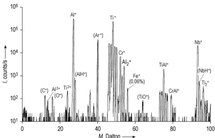
Fig. 3.35. HF-plasma SNMS survey spectrum of a powder metallurgically-produced TiAl alloy sample. In brackets:
