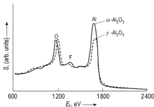
Fig. 3.56. LEIS obtained from different types of alumina with 3 keV He ions [3.142].
