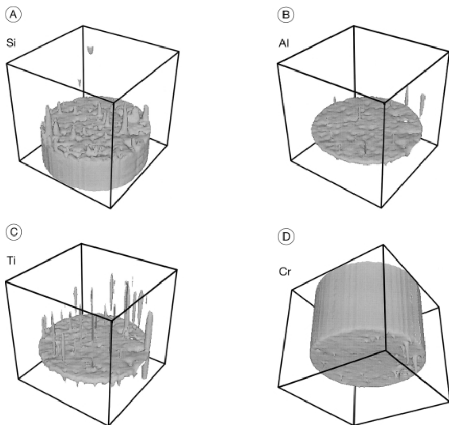
Fig. 3.28. 3D depth profile of the CrN layer on Si substrate, same measurement as Fig. 3.27. The thickness of the CrN layer is 2.3 \mu\text{m} , dia-
