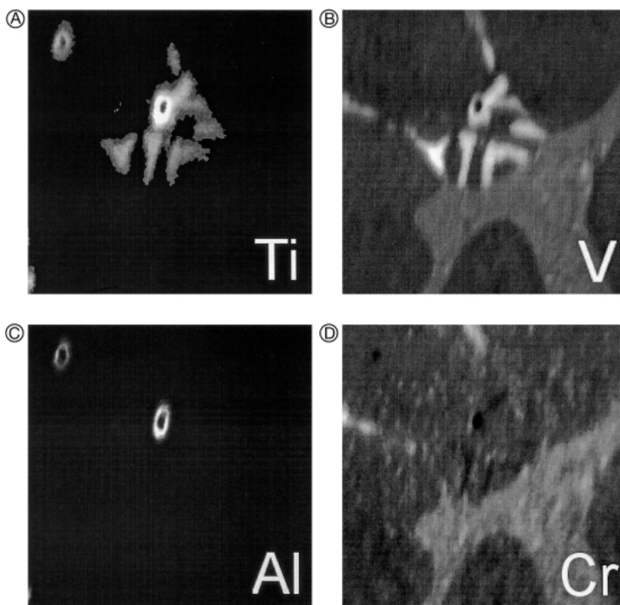
Fig. 3.23. Scanning SIMS image of the carbide structure of a high-speed steel [3.52]. In the V distribution different phases (MC and \text{M}_2\text{C} ) are visible. The Al distribution shows the shell structure of the NMI (non-metallic impurities) acting as condensation nucleus. Measurement time 10 min; image size 64 \times 64 \mu\text{m} ; primary ions \text{O}_2^+ ; primary energy 5.5 keV.
