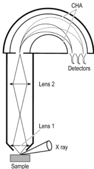
Fig. 2.6. Typical configuration of an XPS spectrometer.
