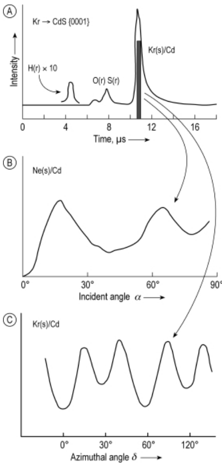
Fig. 3.62. Examples of TOF-SARS spectra for Kr scattering from CdS – time-of-flight spectrum, scans for the angle of incidence \alpha , and the azimuthal angle \delta [3.149].
