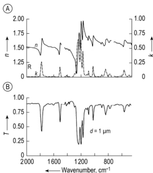
Fig. 4.64. (a) Bulk spectrum of polycarbonate n and k ; (b) with n , k calculated transmission spectrum for a thickness of 1 \mu\text{m} .
