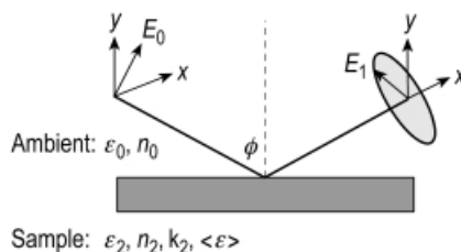
Fig. 4.61. Principle of measurement in ellipsometry.
