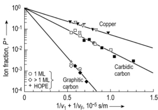
Fig. 3.53. Ion fraction of ^3\text{He} and ^4\text{He} ions (open and full symbols, respectively) in LEIS from Cu ( \nabla , \blacktriangledown ) and different types of C (carbodic carbon \square , \blacksquare ; graphitic carbon \circ , \diamond , + , \blacklozenge ) as a function of the sum of the reciprocal velocities of the incoming and the scattered ion [3.139].
