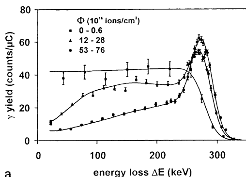
Fig. 3.68. (a) Dependence of measured \gamma yield on \Delta E for impact of (6.385 + \Delta E) MeV N^{15} ions on an SiO_2 -Si sample and for different fluence intervals. (b) Deconvoluted H concentration profiles corresponding to (a) [3.195].
