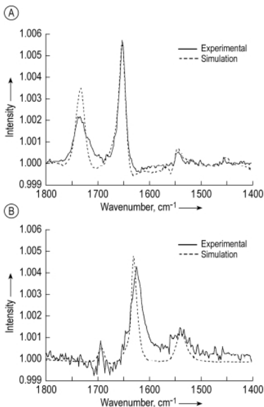
Fig. 4.53. Experimental and simulated PM (polarization modulated) IRRAS spectra of single monolayers of (A) PBG and (B) K(LK) 7 at the air–water interface. The surface pressure was 20 mN m −1 [4.281].
