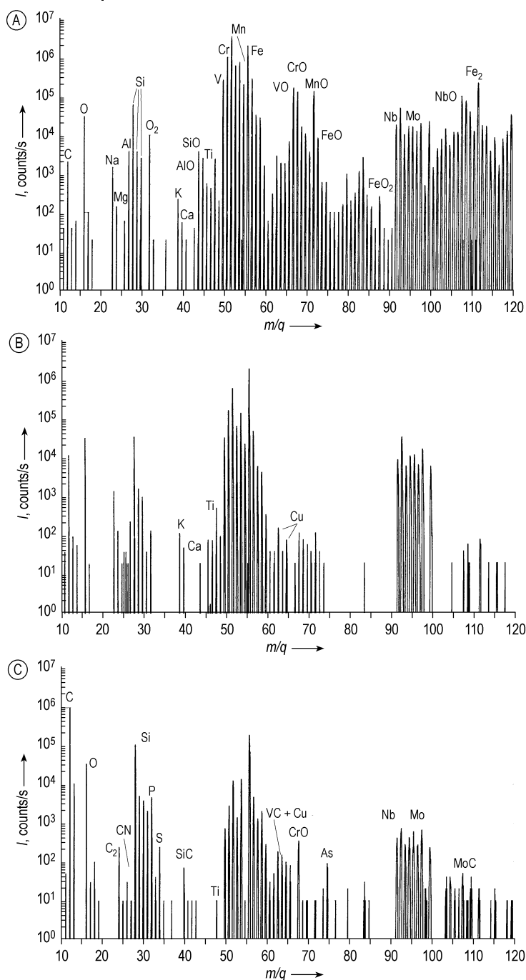
Fig. 3.21. SIMS spectra obtained from a high-speed steel. (A) primary ions O_2^+ ; no secondary ion energy limitation; electronegative elements are sensitive; many molecule ions are visible. (B) same conditions but 300 V offset was used; the molecule ion intensities are reduced significantly. (C) Primary ions Cs^+ ; 300 V offset was used; therefore electronegative elements are detected more sensitively.
