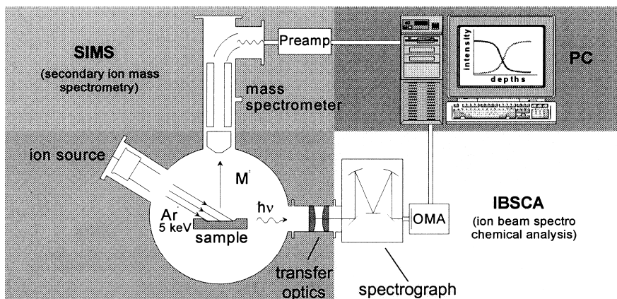
Fig. 4.46. Schematic diagram of IBSCA measurement equipment; this usually combined with a mass spectrometer (SIMS or SNMS).
