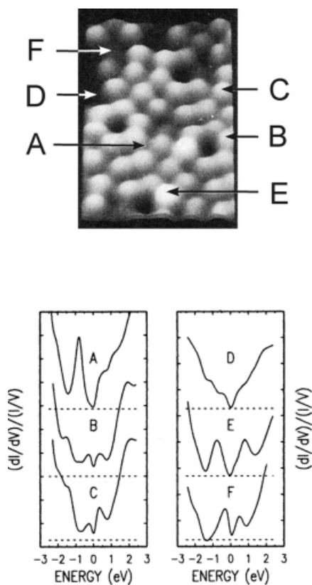
Fig. 5.16. Top: STM image of a region of an O 2 -exposed Si (111)-7 × 7 surface. The sites labeled with A, B, and C have not been changed by exposure to oxygen. D, E, and F correspond to oxygen-induced dark, bright, and perturbed (gray) sites, respectively. Bottom: Tunneling spectra corresponding to the different sites [5.41].
