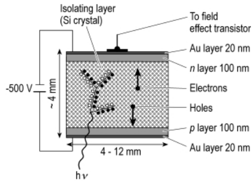
Fig. 4.7. A semiconductor detector operated as a pin diode with a reverse voltage or bias. An incident X-ray photon ultimately produces a series of electron-hole pairs. They are "swept out" by the bias field of -500\text{ V} – electrons in the direction of the n-layer; holes in the direction of the p-layer. Thus, a small charge pulse is produced after [4.21].
