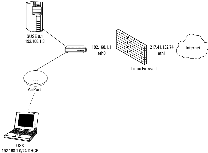
Figure 23-2: Network using a netfilter firewall
