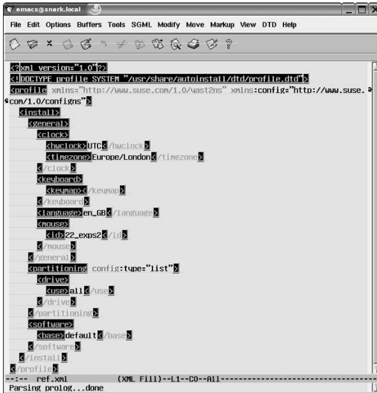
Figure 9-36: Editing the control file with emacs
