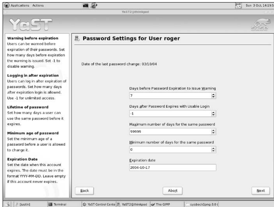
Figure 9-25: Editing password settings
