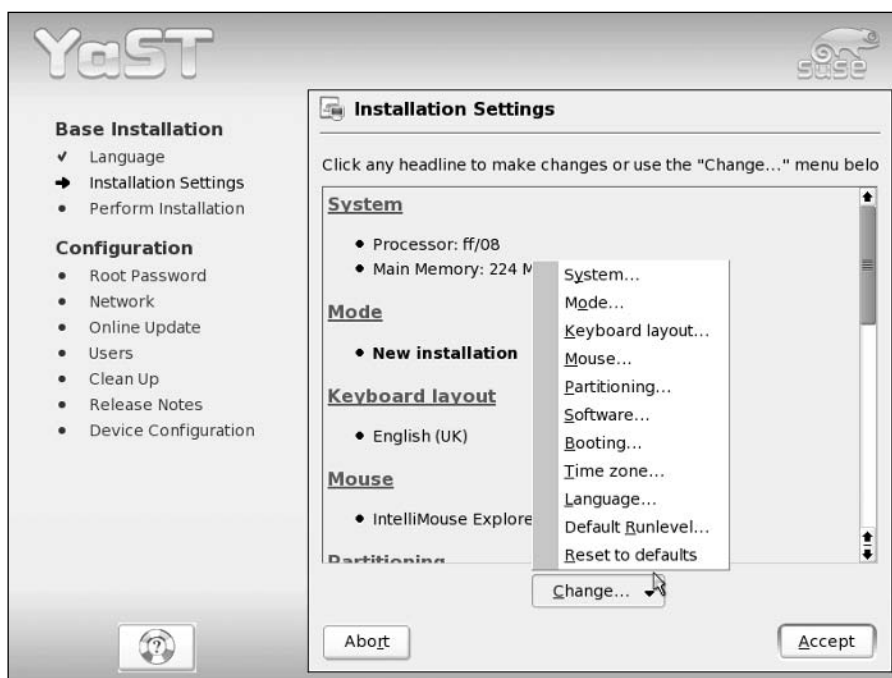
Figure 1-6: Installation customization
