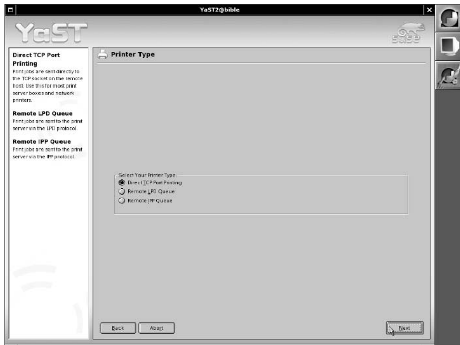
Figure 9-10: Printing protocol
