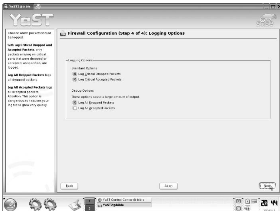
Figure 23-7: Enabling logging
