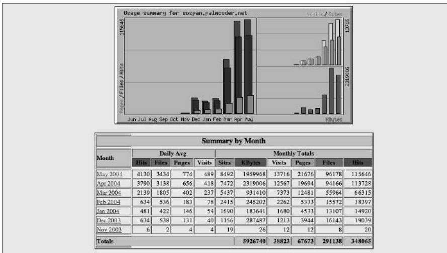
Figure 7-1: Webalizer output
