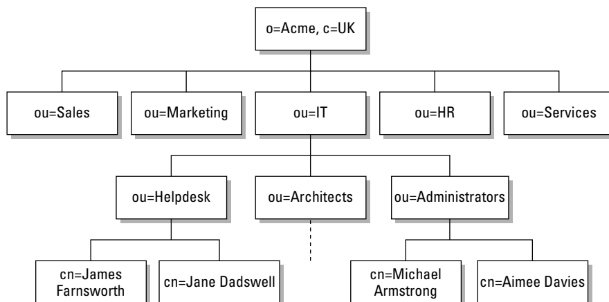
Figure 24-2: Acme organization in LDAP
