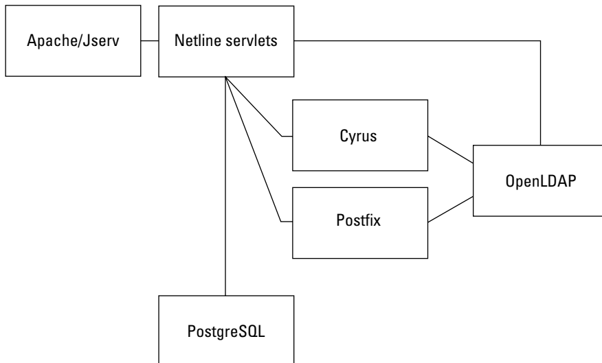
Figure 29-12: Conceptual overview of SLOX components
