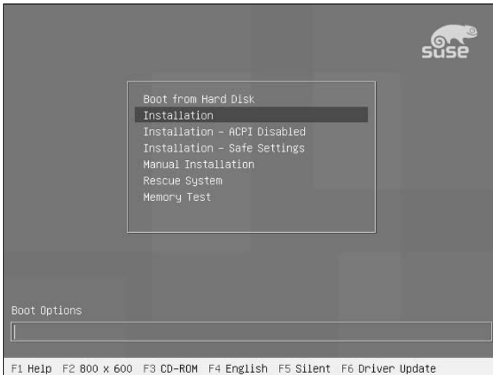
Figure 1-2: Boot options
