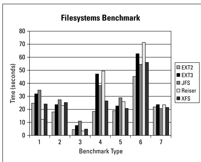
Figure 3-2: Benchmark results
