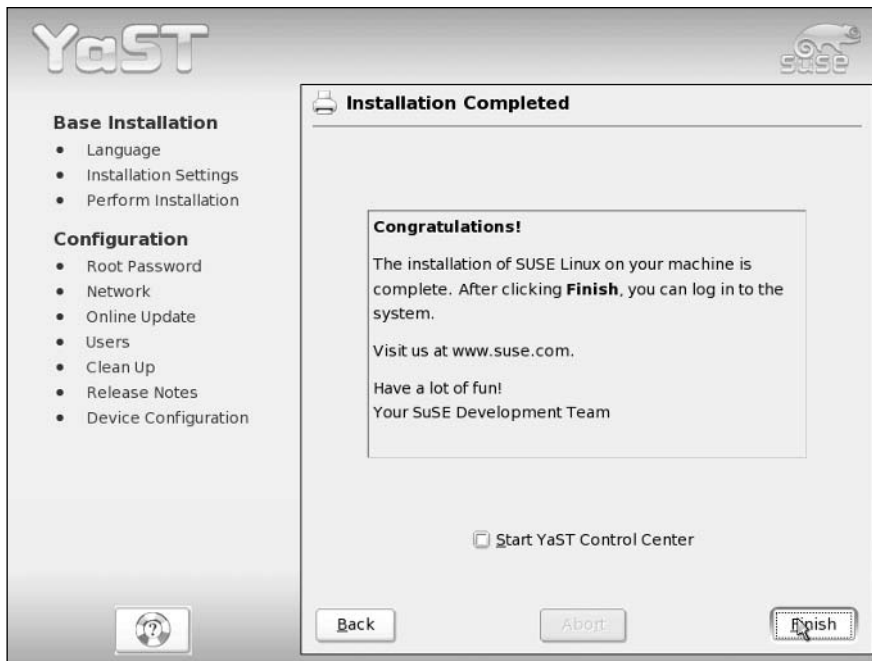
Figure 1-37: Installation completed
