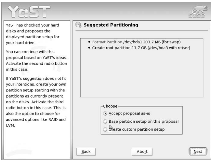
Figure 1-7: Partitioning
