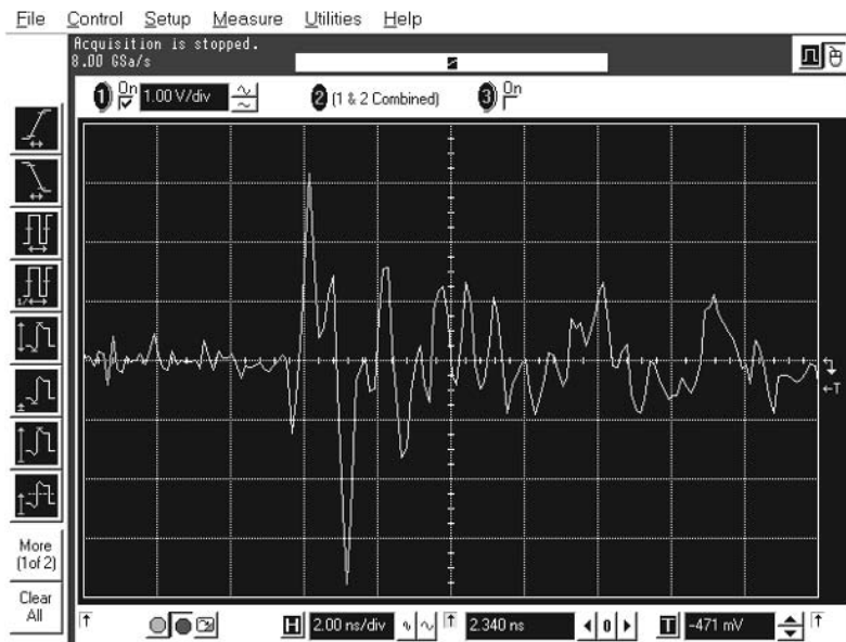
Figure 9.38 Loop output from board with original configuration. (Photograph courtesy of Doug Smith.)
