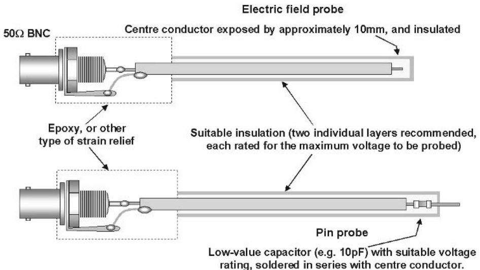
Figure 5.23 Various construction details of an electric field probe. (Artwork courtesy of EMC Compliance Journal [3].)
