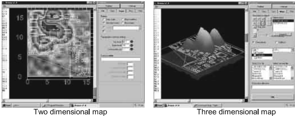
Figure 9.49 Typical plots from top side of PCB scanner. (Plots courtesy of Detectus AB.)
