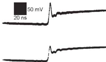
Figure A.25 Data from 1.0- \mu F electrolytic capacitor.
