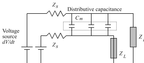
Figure 2.10 Electric field coupling.
