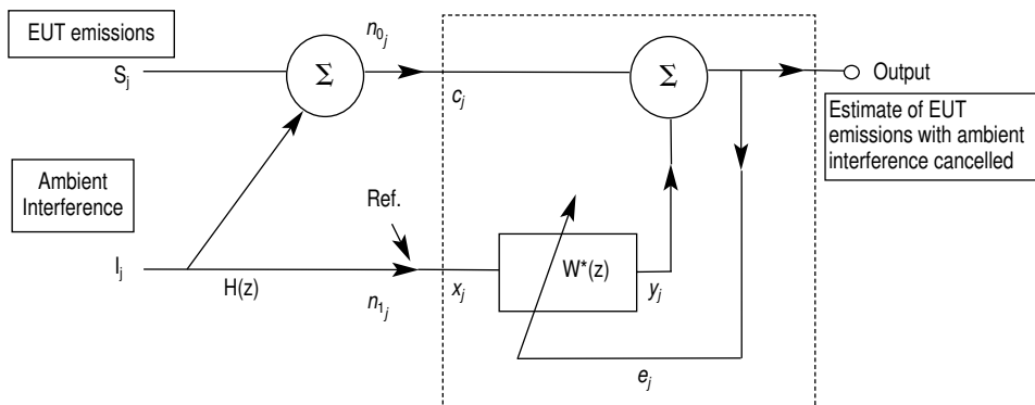
Figure 3.12 Block diagram of a basic cancellation system.
