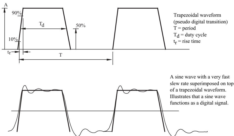
Figure 1.1 Sine wave appearing as a digital transition.
