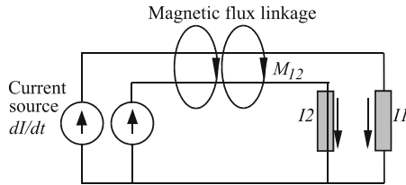
Figure 2.8 Magnetic field coupling.
