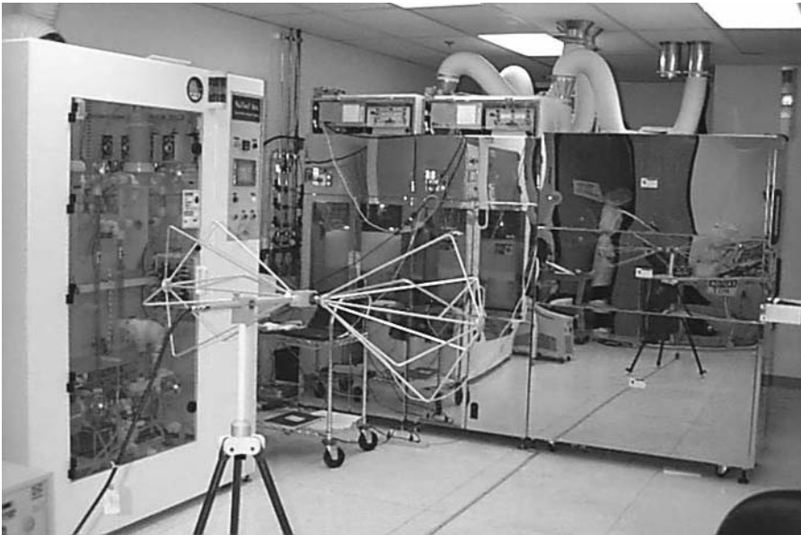
Figure 7.4 Sample in situ test of an industrial product.
