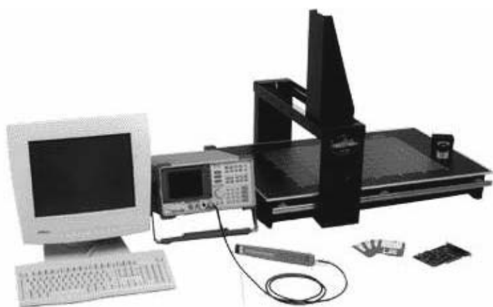
Figure 9.48 EMC scanner for top-sided electromagnetic field measurements. (Photograph courtesy of Detectus AB.)
