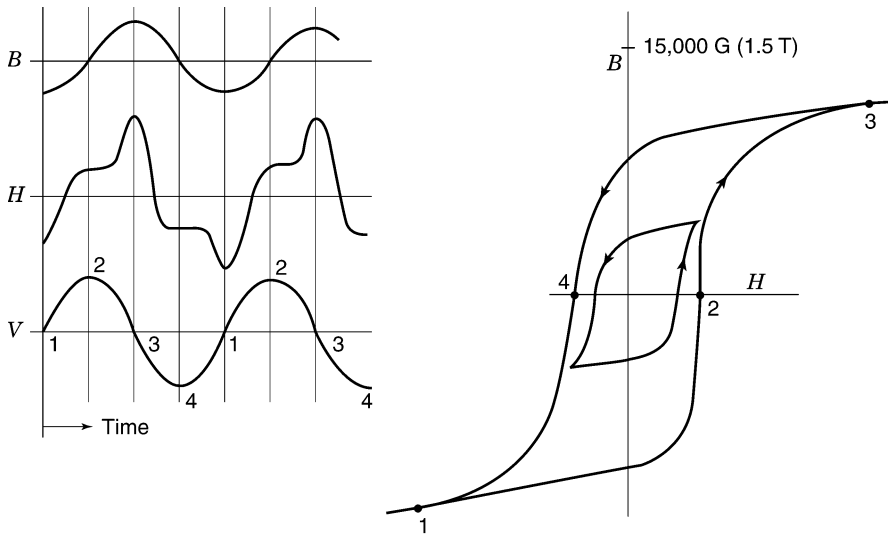
The B field is sinusoidal when the applied voltage is sinusoidal.
