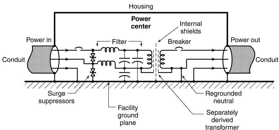
FIGURE 7.3 Power center.
