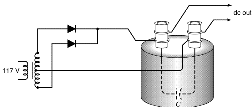
FIGURE 5.6 Four-terminal capacitor.
