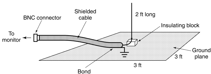
FIGURE 6.10 Simple antenna for field measurement.
