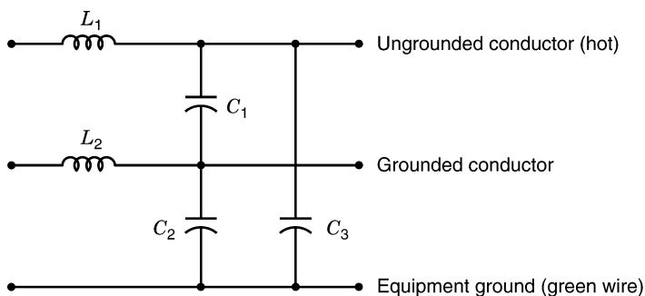
FIGURE 5.11 Simple line filter.
