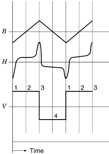
The H field when the applied voltage is a square wave. The B field is triangular.
