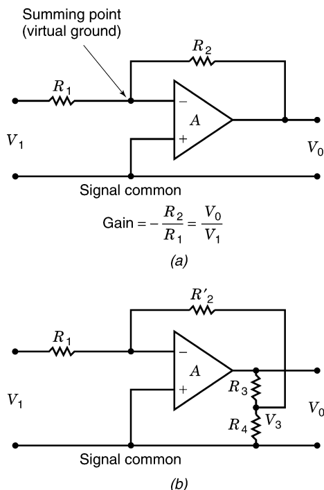
FIGURE 5.7 Operational feedback.
