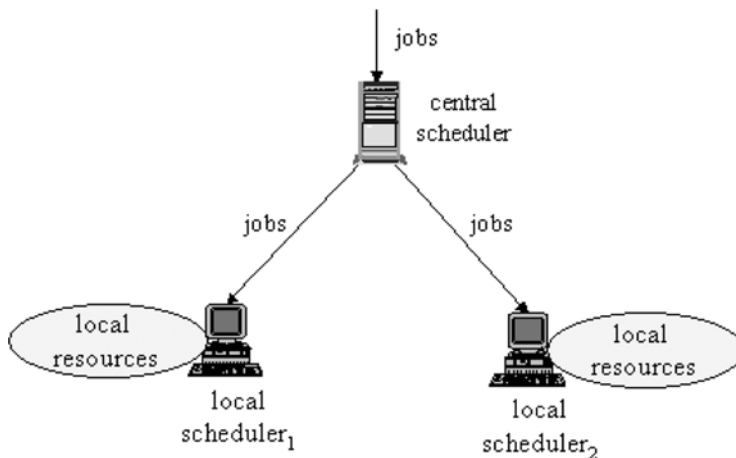
Figure 6.5 Hierarchical scheduling
