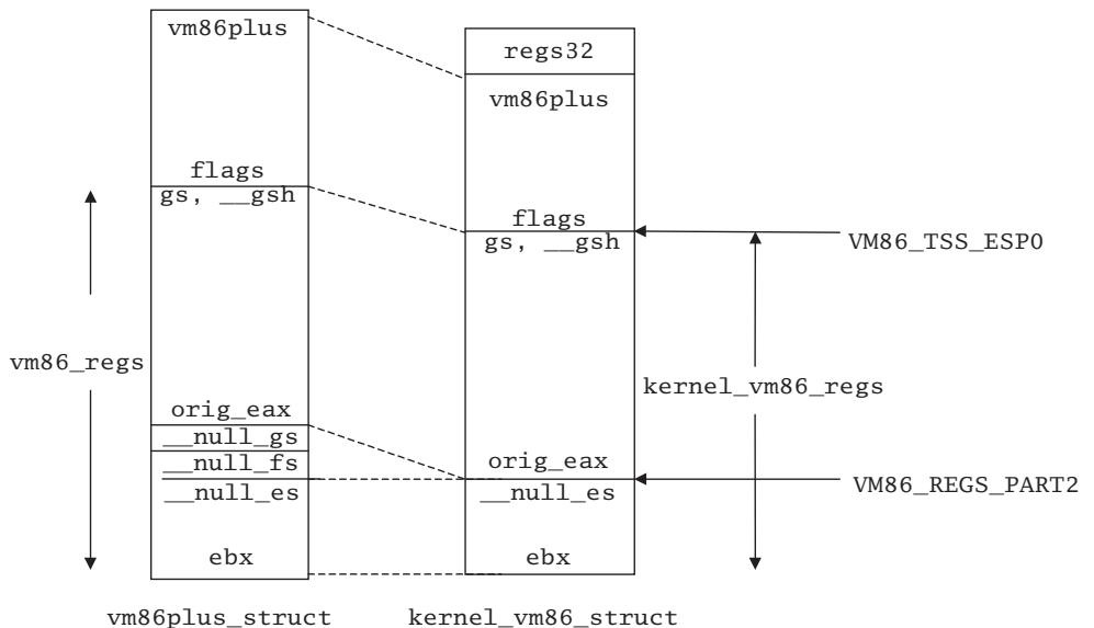
Figure 24.8 User-supplied information copied to the stack
