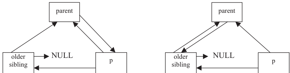
Figure 3.4 Removing a youngest child from the family tree
