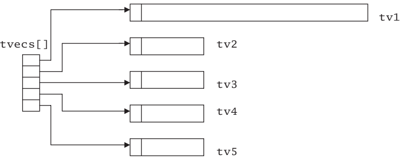
Figure 15.27 Timer lists
