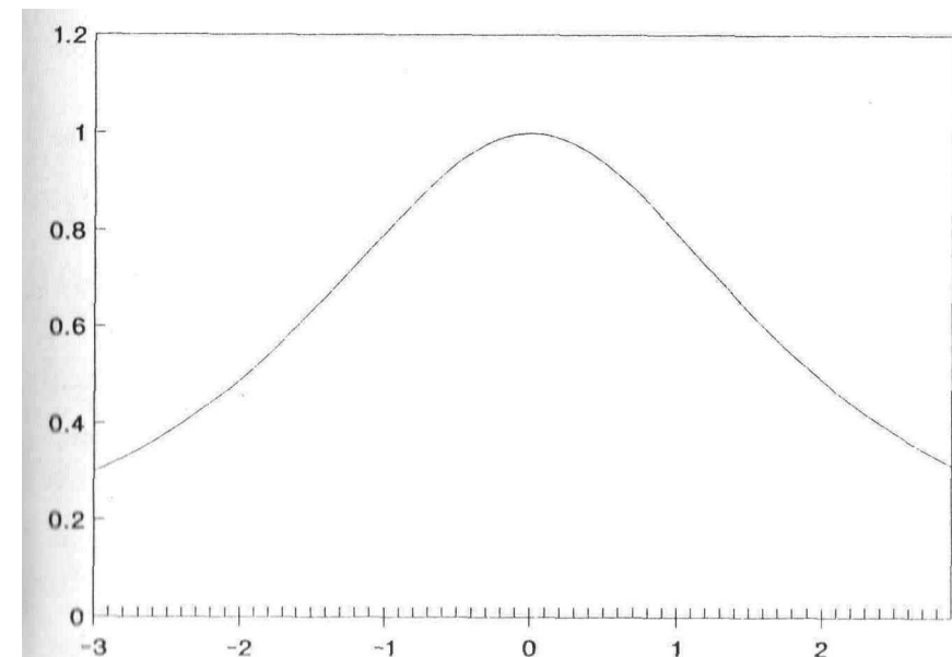
Figure 4-6 LOC = 0 SCALE = .5 SKEW = 0 KURT = 2.
