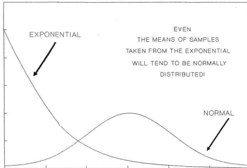
Figure 3-6 The Exponential Distribution and the Normal.
