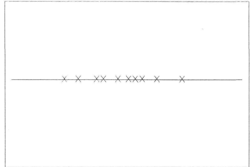
Figure B-9 Sequence of haphazard events in time.
