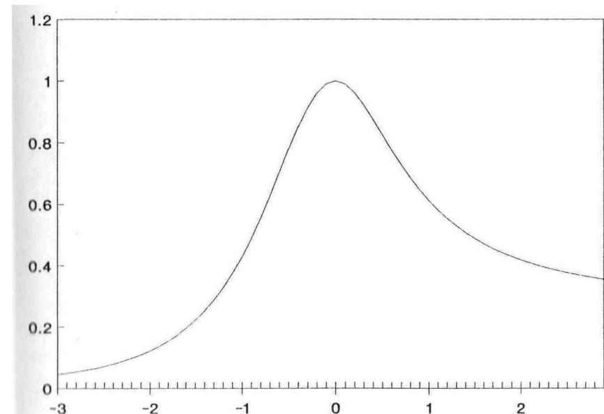
Figure 4-9 LOC = 0 SCALE = 1 SKEW = +0.5 KURT = 2.
