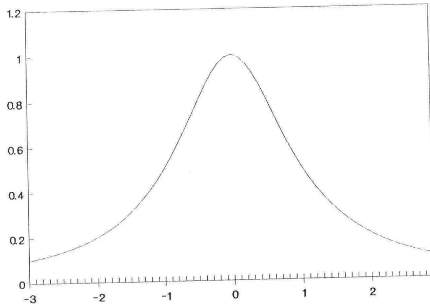
Figure 4-2 LOC = 0 SCALE = 1 SKEW = 0 KURT = 2.
