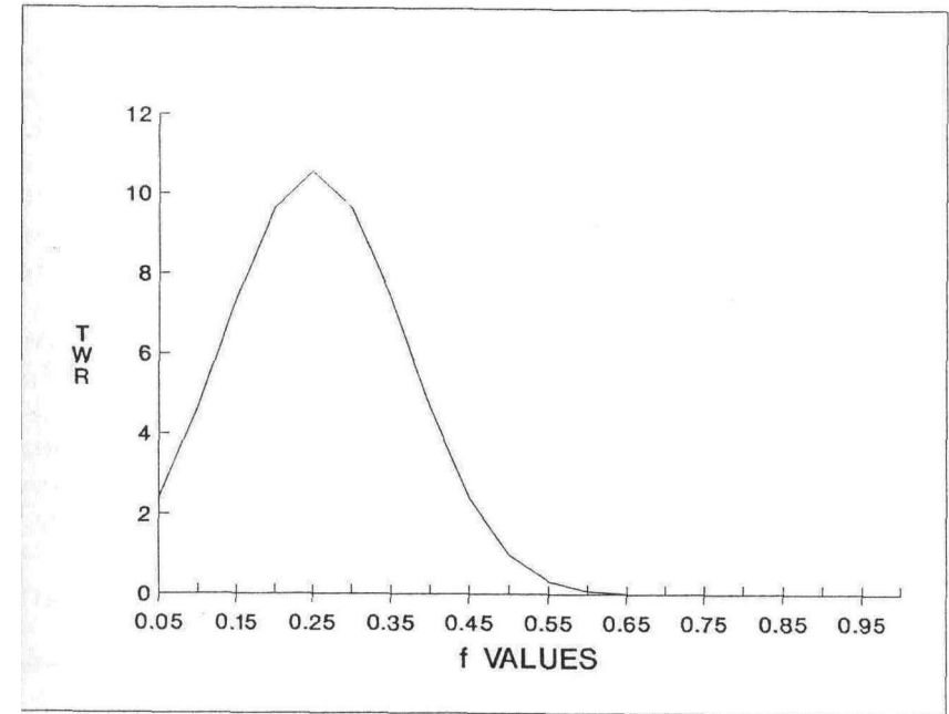
Figure 1-1 20 sequences of +2, -1.
