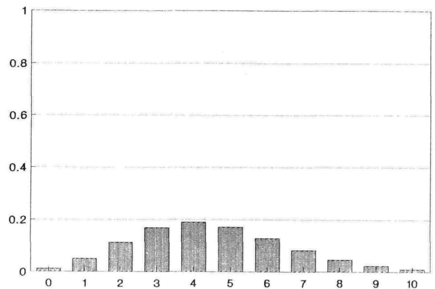
Figure B-12 Probability density functions for the Poisson Distribution ( L = 4.5 ).
