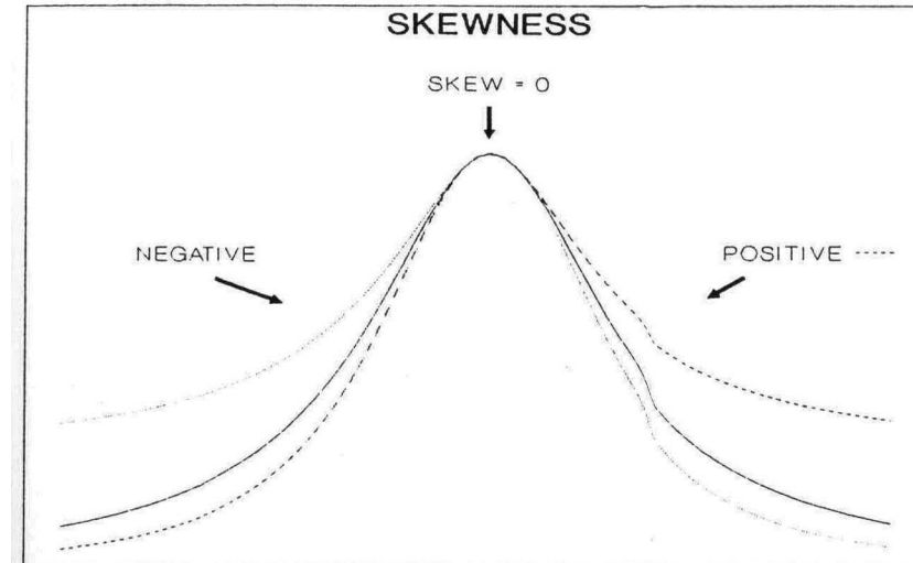
Figure 3-2 Skewness.
