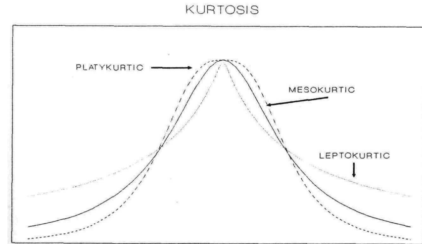
Figure 3-4 Kurtosis.
