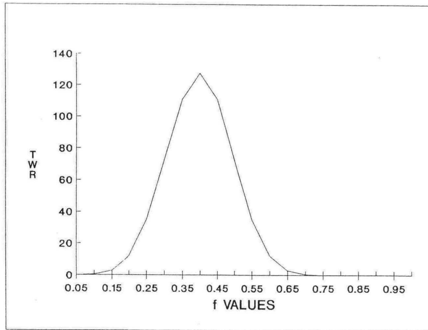
Figure 1-6 20 sequences of +5, -1.
