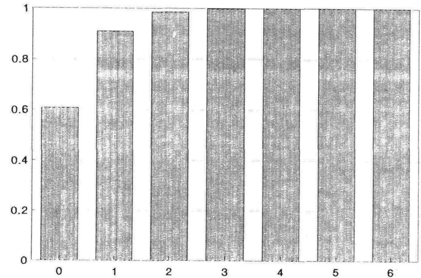
Figure B-11 Cumulative probability functions for the Poisson Distribution ( L = .5 ).
