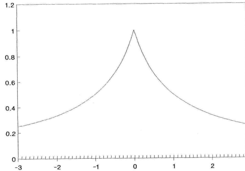
Figure 4-5 LOC = 0 SCALE = 1 SKEW = 0 KURT = 1.
