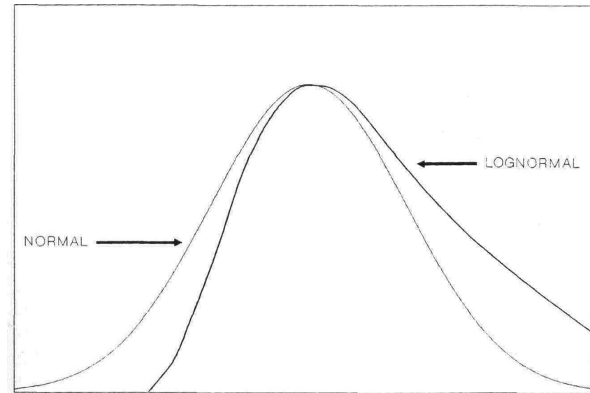
Figure 3-15 The Normal and Lognormal distributions.
