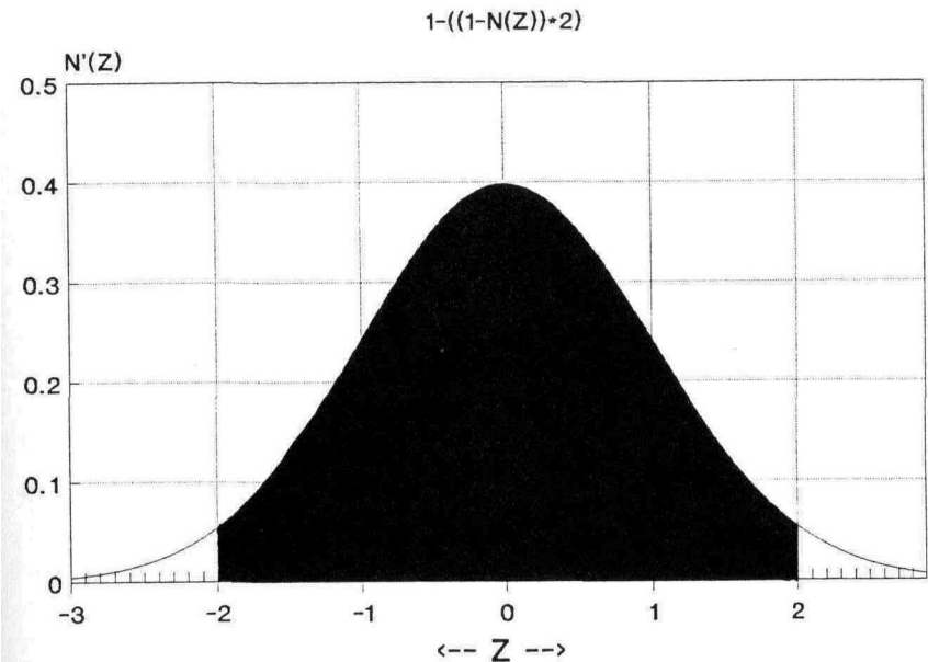
Figure 3-10 A two-tailed probability of an event being + \text{ or } - 2 sigma.
