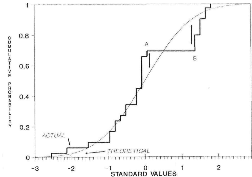
Figure 4-1 The K-S test.
