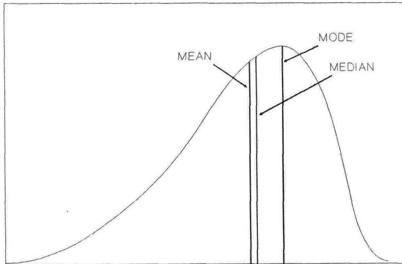
Figure 3-3 Skewness alters location.
