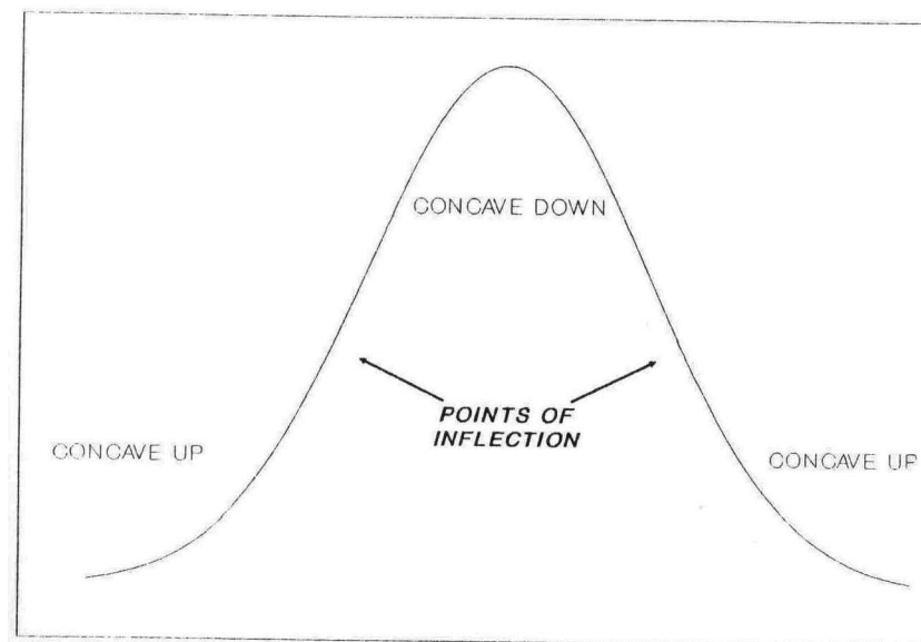
Figure 4—11 Points of inflection on a bell-shaped distribution.
