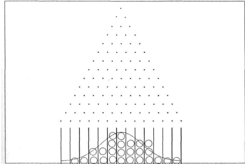
Figure 3-5 Galton's board.
