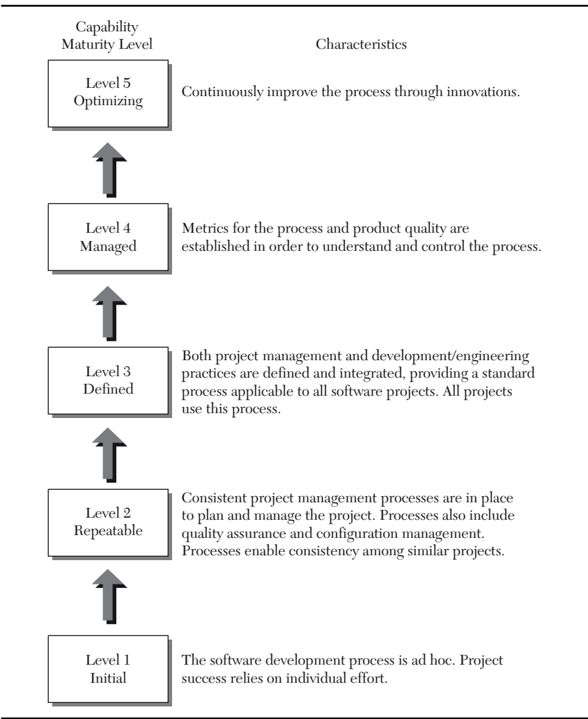
EXHIBIT 14.2 Software engineering institute capability maturity model overview
