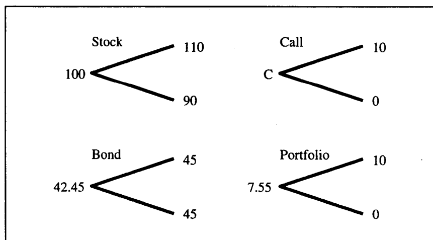
FIGURE 4.1 One-Period Payoffs
