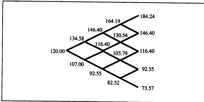
Stock Price Lattice for Problem 18
