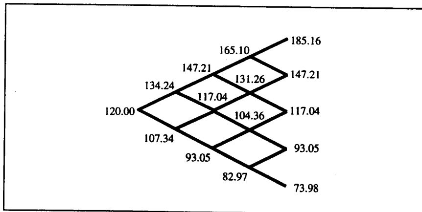
Adjusted Stock Price Lattice for Problem 19
