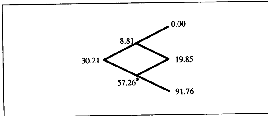
American Put Price Lattice for Problem 7
