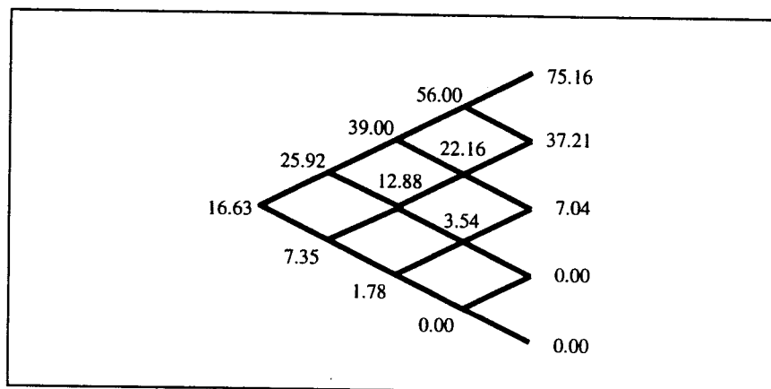
Call Price Lattice for Problem 19
