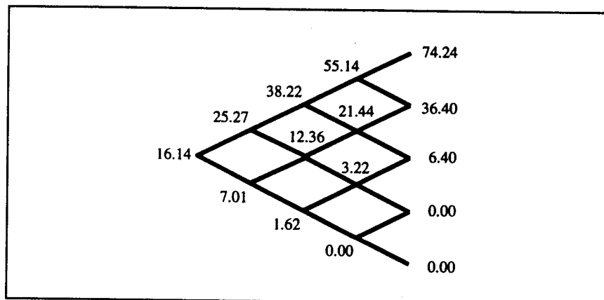
Call Price Lattice for Problem 18
