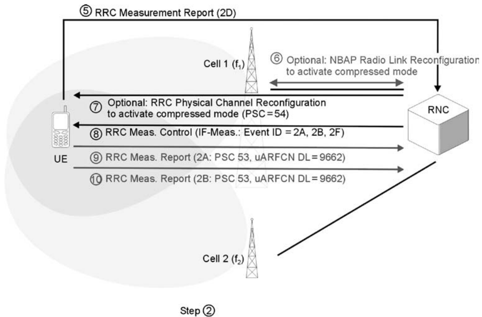
Figure 2.34 Inter-frequency handover step 2
