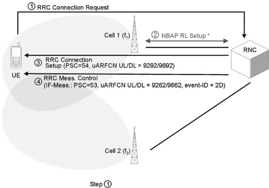
Figure 2.33 Inter-frequency handover step 1
