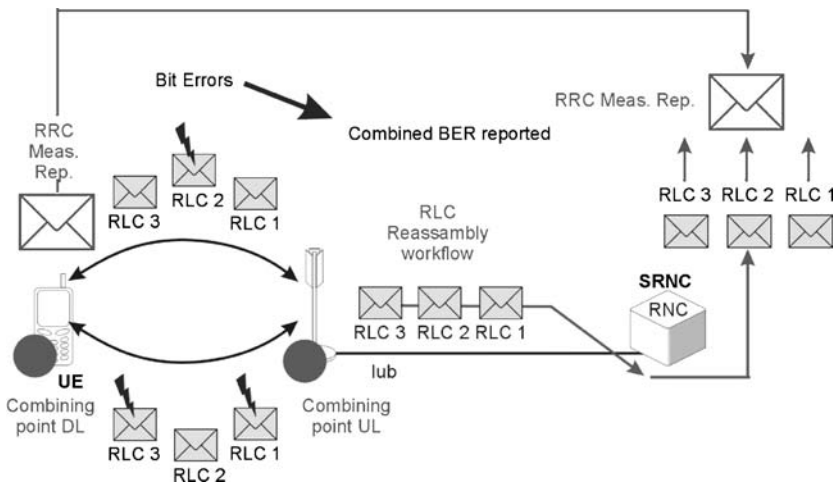
Figure 1.30 UE in CELL_DCH – two radio links in active set – softer handover
