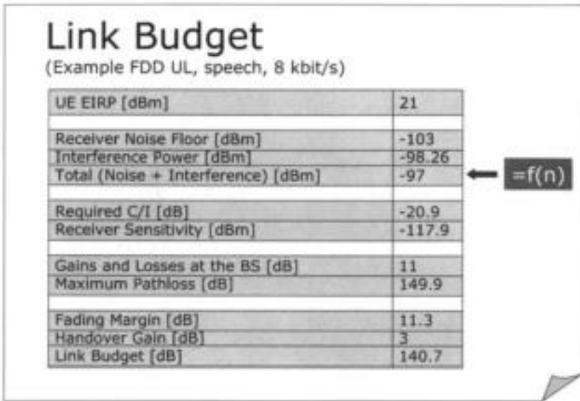
Figure 9.3: Sample link budget calculation
