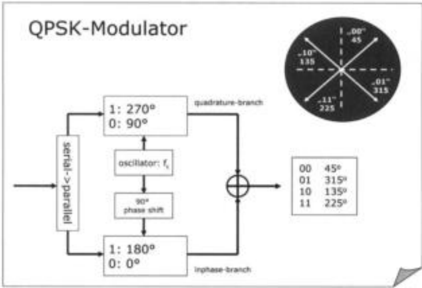
Figure 1.2: QPSK modulation
