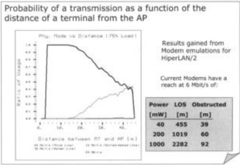
Figure 11.17: Range of HiperLAN/2 at 6 Mbit/s
