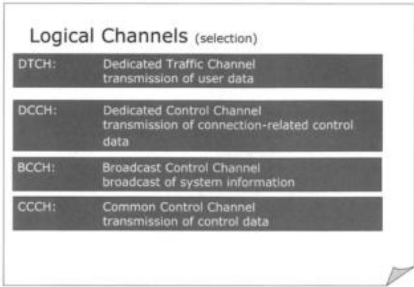
Figure 5.15: Logical channels
