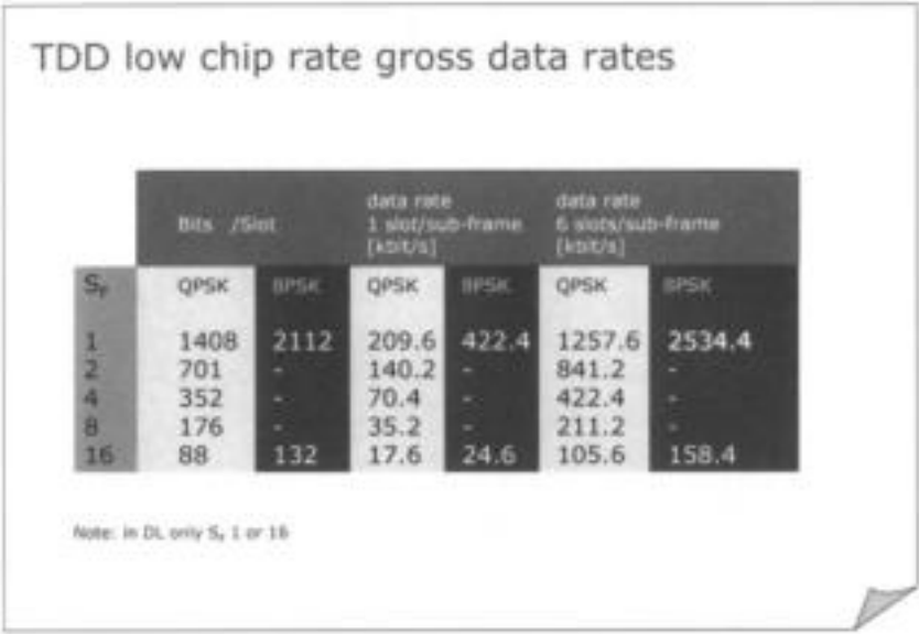
Figure 8.19: Configurations and transmission rates of DPCH in low chip rate TDD mode
