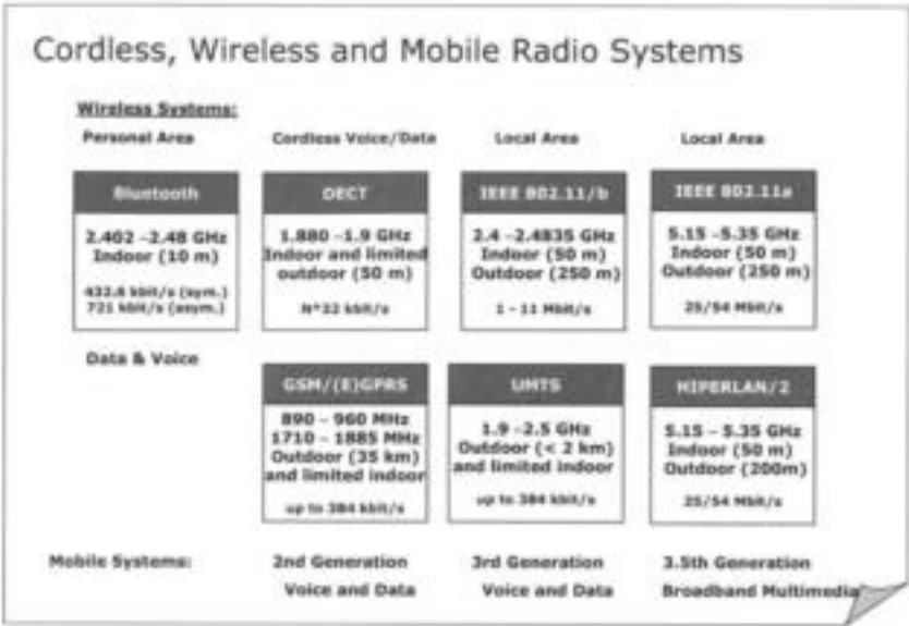
Figure 11.1: Cordless, wireless and mobile radio systems
