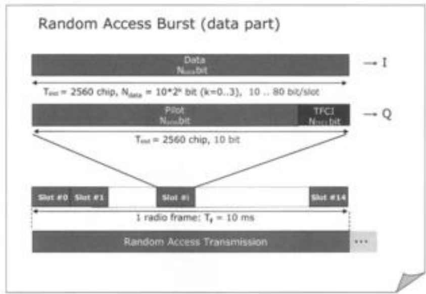
Figure 8.13: Time and burst structure with data transmission over a PRACH
