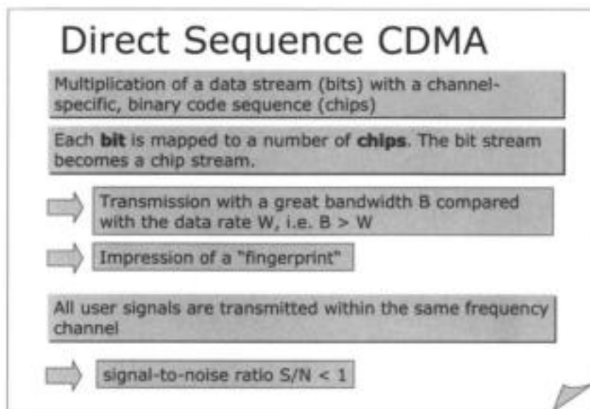
Figure 6.7: Direct-sequence CDMA
