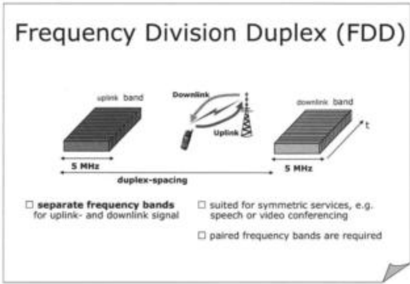
Figure 6.3: Frequency-division duplex
