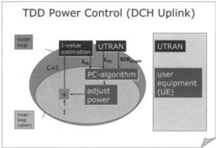
Figure 7.9: Power control on the uplink in TDD mode
