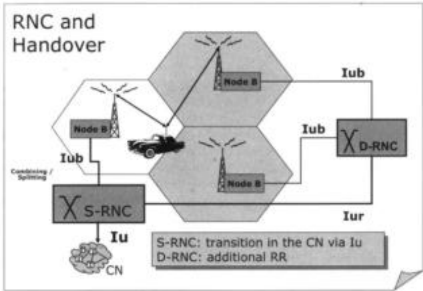
Figure 4.14: The role of RNC in a handover
