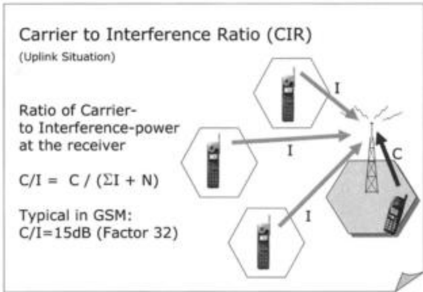
Figure 2.5: Signal-to-interference ratio
