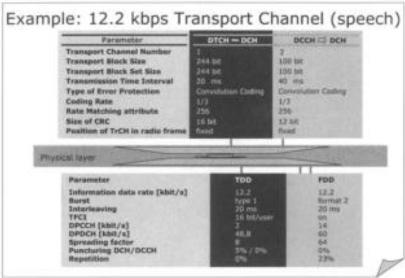
Figure 8.21: Mapping of 12.2 kbit/s reference channels to physical channels in FDD and TDD mode
