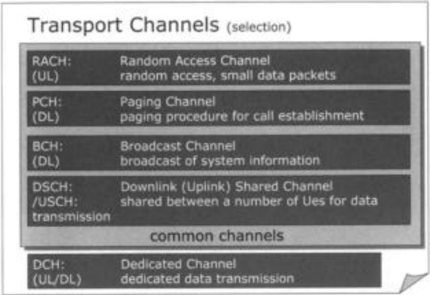
Figure 5.10: Transport channels
