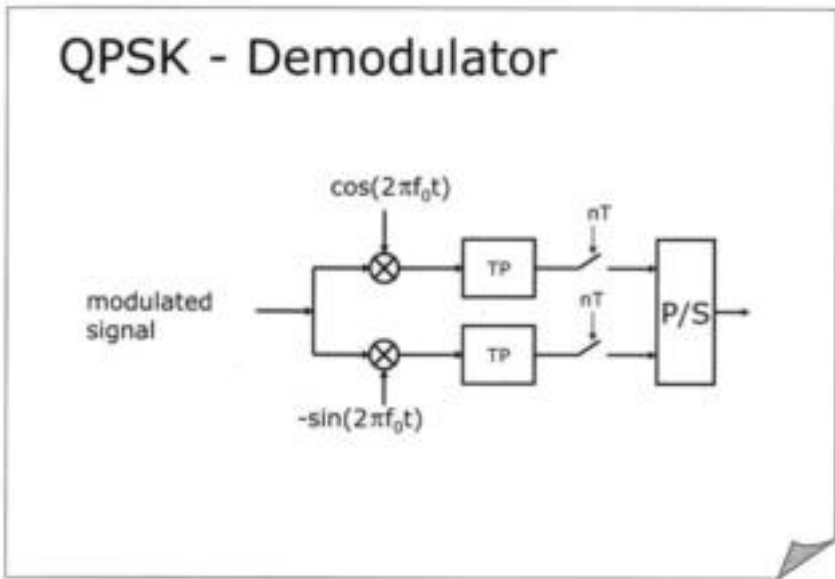
Figure 1.3: QPSK demodulator
