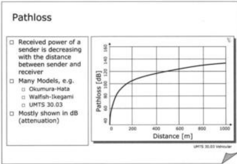
Figure 2.4: Propagation attenuation
