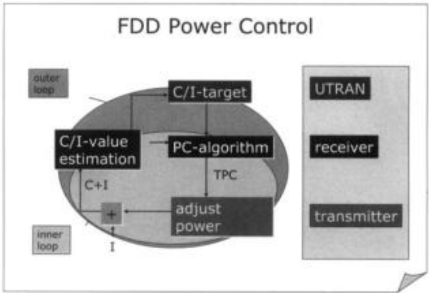
Figure 7.8: Power control in FDD mode
