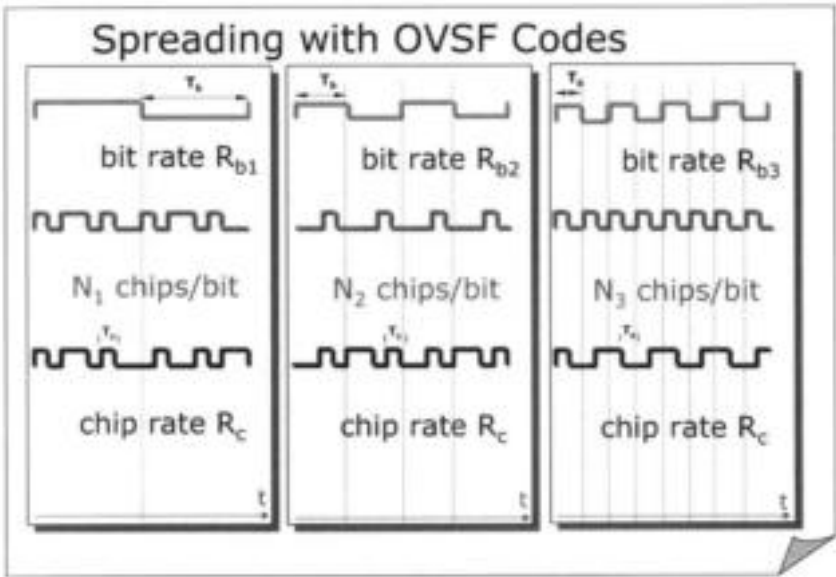
Figure 6.15: Implementation of variable bit rates using OVFS codes
