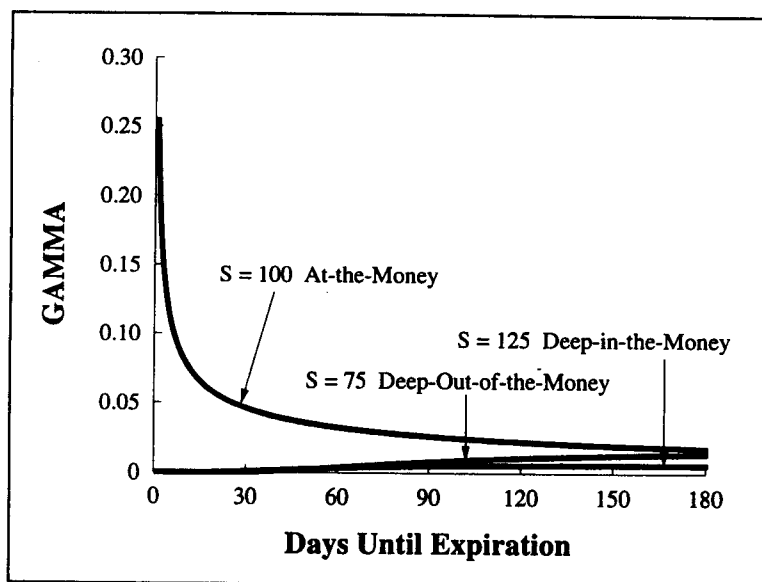
FIGURE 5.14 GAMMA as a Function of the Time until Expiration X = \$100 ; \sigma = 0.3 ; r = 0.08 ; T - t = 180 days
