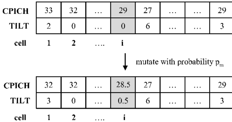
Figure 14.17 Mutation operator, practical implementation [34]. (Reproduced by permission of © 2004 IEEE).
