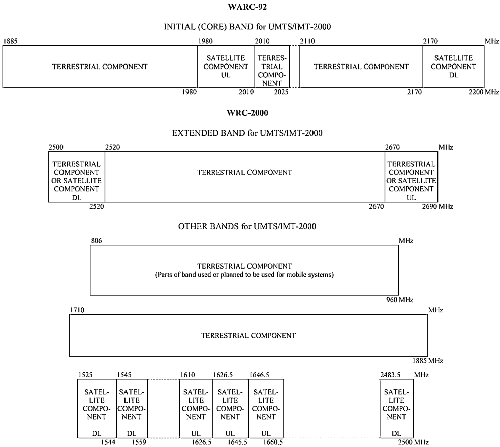
Figure 3.1 Frequency bands identified for UMTS/IMT-2000 by WARC-92 and WRC-2000.
