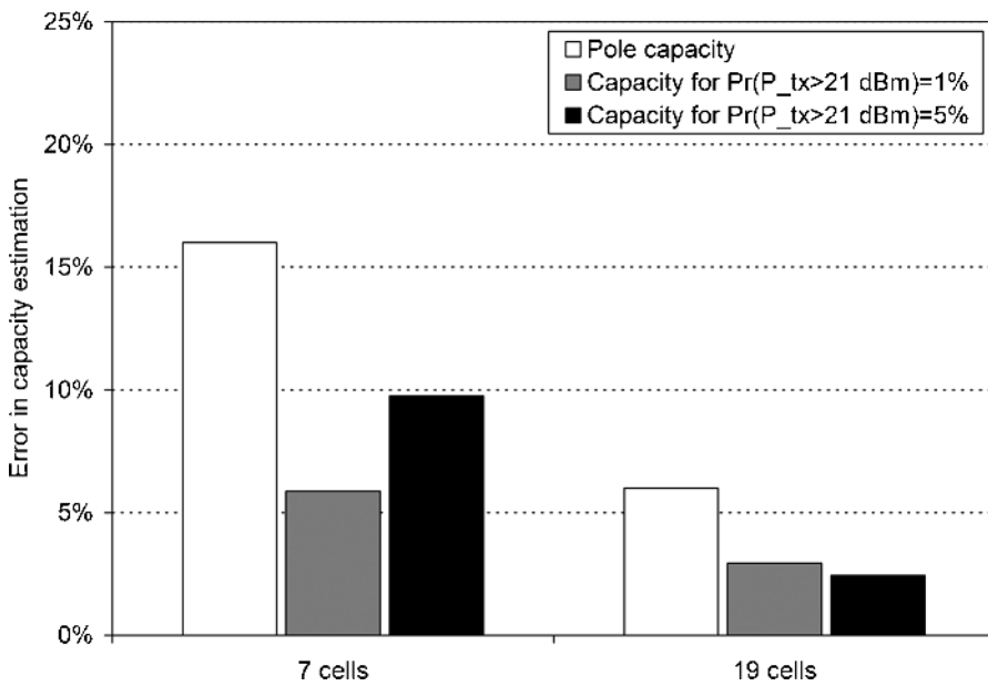
Figure 9.16 Error in capacity estimation for different number of cells assumed in simulations in the uplink.
