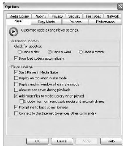
Figure 4-12: Player tab.
