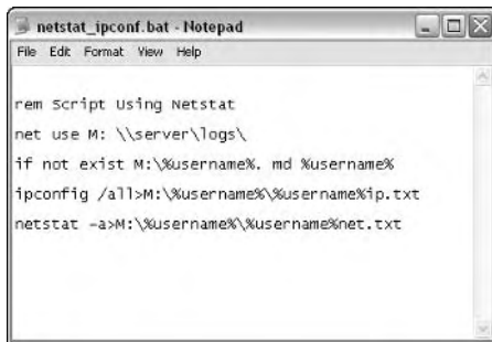
Figure 21-15: ipconfig and netstat scripts.
