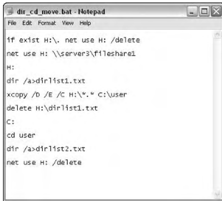
Figure 21-13: Using the dir , cd , and delete commands.
