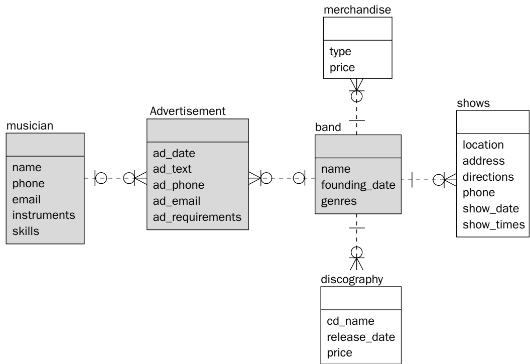
Figure 9-29: A basic data warehouse ERD business rules database model.
