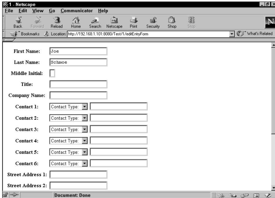
Figure 7-11: editEntryForm.html form
