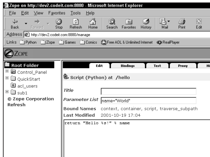
Figure 15-3: Passing parameters
