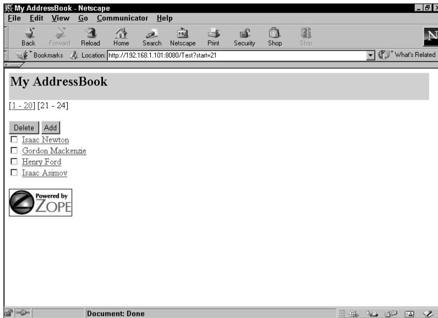
Figure 8-4: Batch Navigation 2
