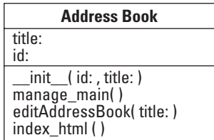
Figure 7-4: AddressBook UML diagram
