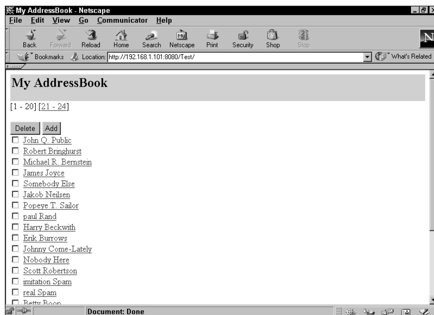
Figure 8-3: Batch Navigation 1
