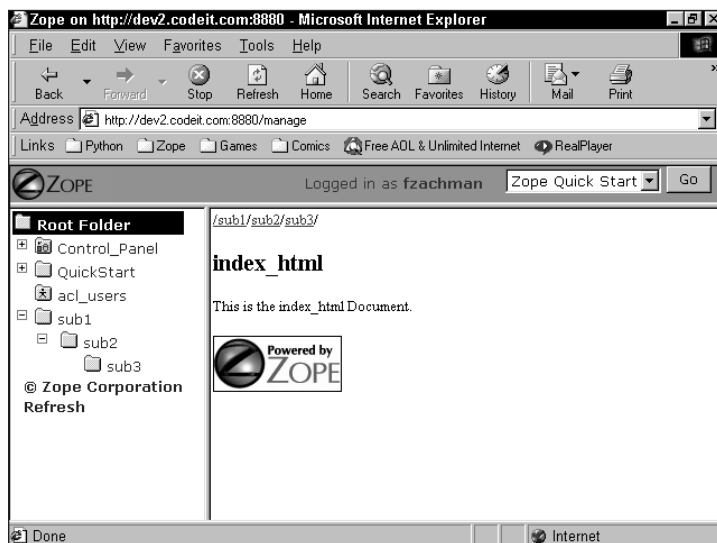
Figure 15-5: Breadcrumbs
