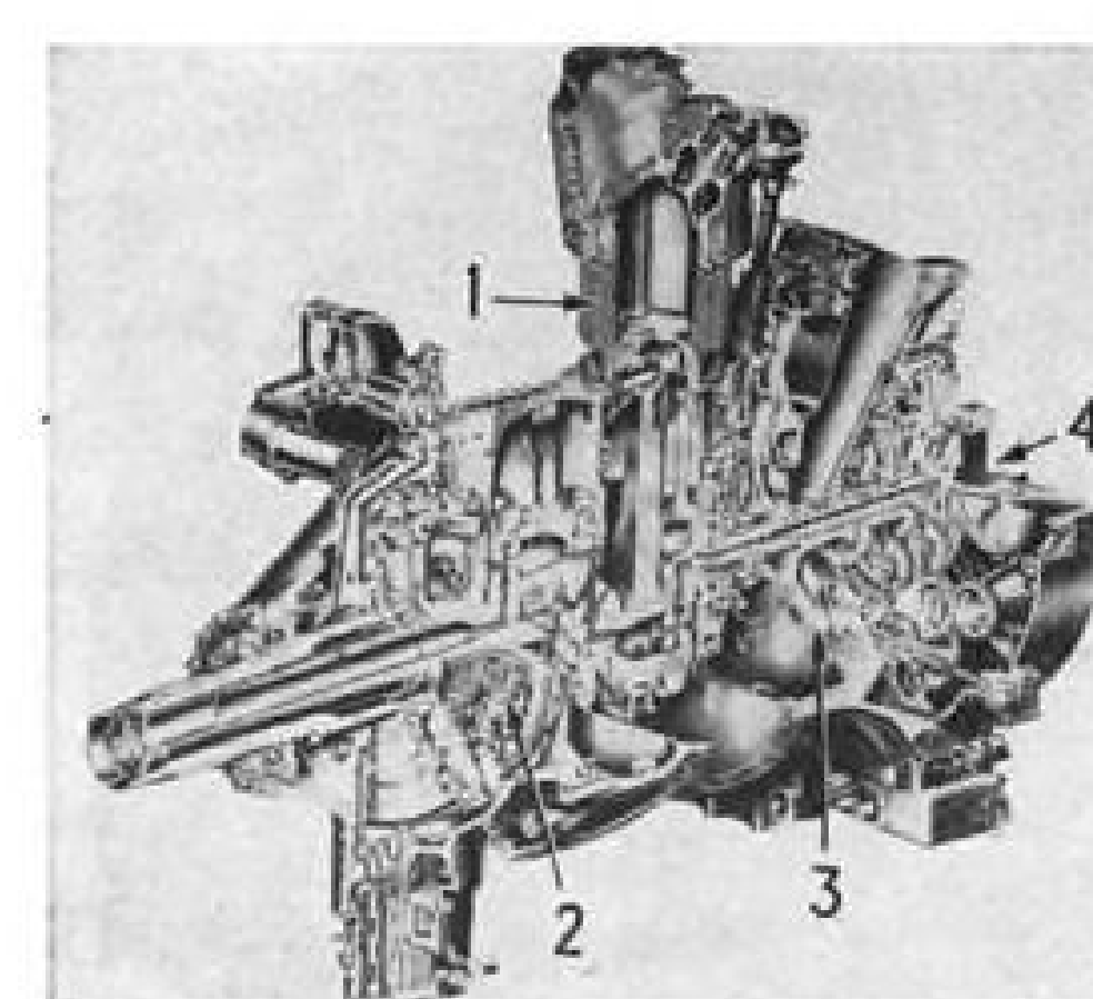
1941—This is cutaway view of the 2200-hp. R-3350-23, power plant. Disclosed here are: 1, Aluminum-finned cylinder barrel; 2, second order balancer; 3, supercharger impeller, 13-in. single speed installation, complemented by a turbosupercharger; and 4, simplified rear section. Evidenced is compactness of design features.
