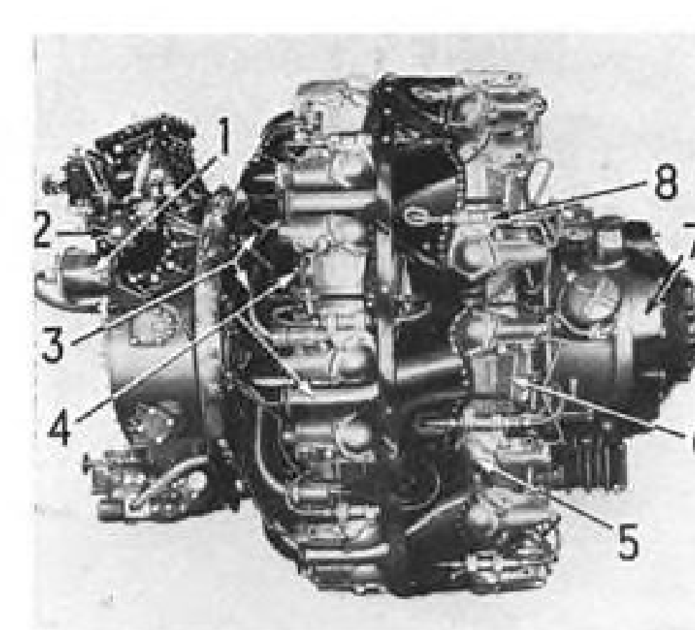
1945—Cyclone 18BD, 2500-hp. engine using 100/130 fuel: 1, Low tension generator; 2, fuel injection; 3, Y-type intake pipes; 4, all rear exhaust; 5, smaller rocker box covers with close-spaced studs for effective oil seal; 6, forged aluminum head; 7, 16:7 reduction gear; and 8, low-tension ignition with high tension coils at heads.
