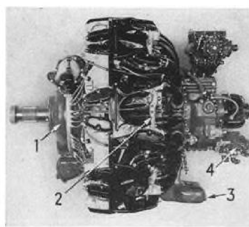
1939—R3350-4, -5 delivered 2000-hp., also used 100 octane fuel. Changes indicated are: 1, Shorter nose section housing improved gear system with 16:7 gear ratio; 2, cylinder head suspension brackets; 3, rear sump; and 4, oil pump. Two-speed supercharger impeller, also a 12-in. unit, was fitted with a double clutch.
