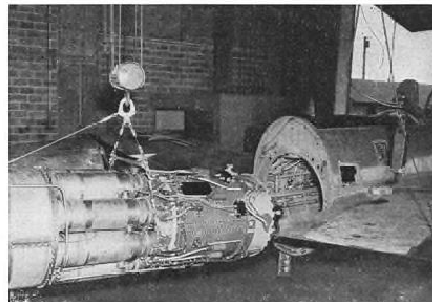
THIS quick method to accomplish removal of entire power plant.
