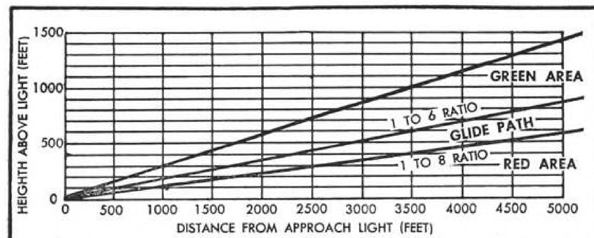
Chart of lighted glide path: on correct approach, pilot sees both red and green lights.
