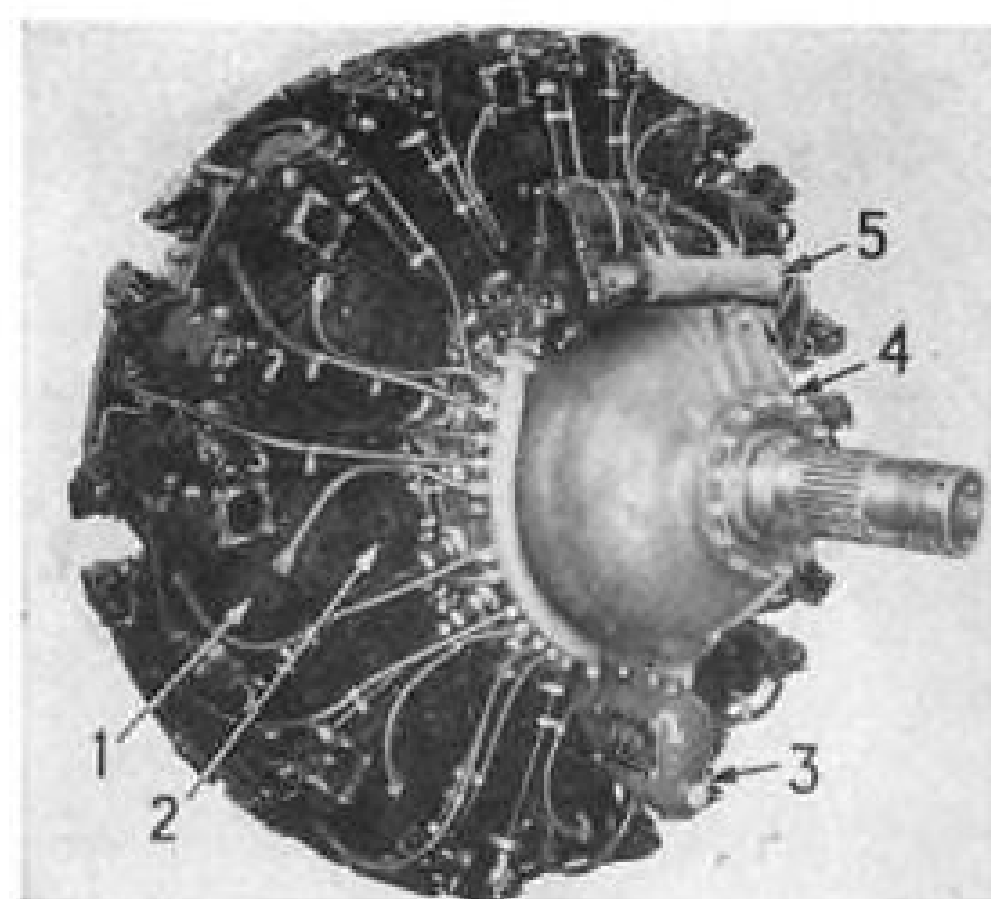
1937—R3350-1, -2, -3 delivered 1700 hp. for takeoff, used 100 octane fuel. Engine had: 1, Cast aluminum cylinder head; 2, steel barrel fins; 3, sump only (no pump); 4, 2:1 reduction gear; and 5, non-supercharged ignition. Crankcase suspension was used, and 12-in. supercharger impeller (single or two speed) was employed.
