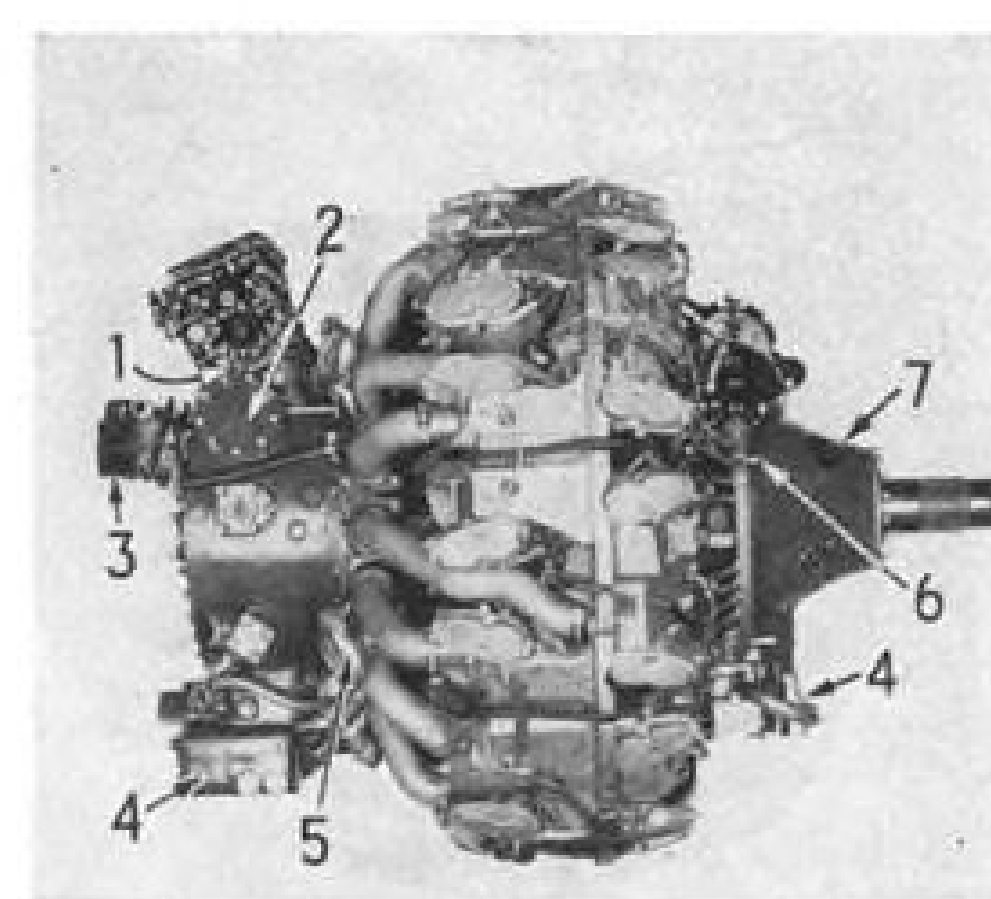
1941—R3350-23 (used in B-29) was 2200-hp. plant using 100 octane fuel. Features: 1, Carburetor adapter eliminated; 2, fuel injection added here later; 3, supercharged magneto; 4, sump and pump combined; 5, crankcase Lord mount; 6, supercharged ignition; and 7, 20:7 reduction gear. Other details are shown in the cutaway view.
