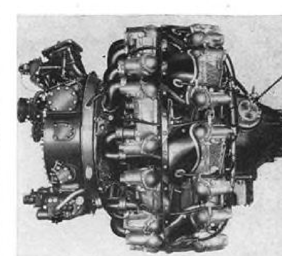
1947—R3350-26W (C18CA) is 2700-hp. (dry) engine using 115/145 fuel. It weighs 2848 lb. as against smaller power, 2884-lb. C18BD; has lightweight high-tension ignition system (arrow) for lower altitude operation than C18BD; water injection; fuel injection at impeller; MAP regulator for altitude changes; and 16:7 reduction gear.
