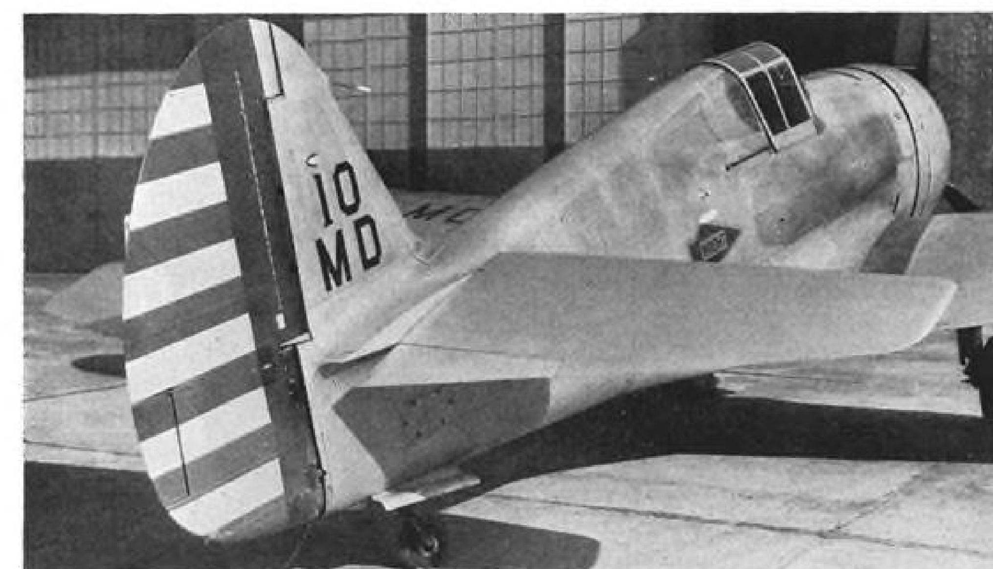
This all-movable horizontal tail installation on the Curtiss XP-42 was employed in NACA research studies on longitudinal control devices for use at very high speed conditions.
