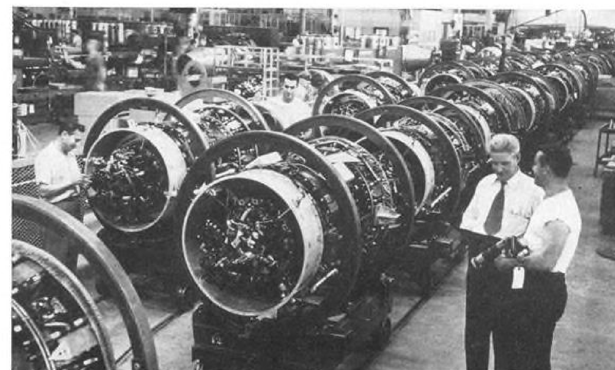
FINAL ASSEMBLY station just before routing jets to test cells for "green" run.
