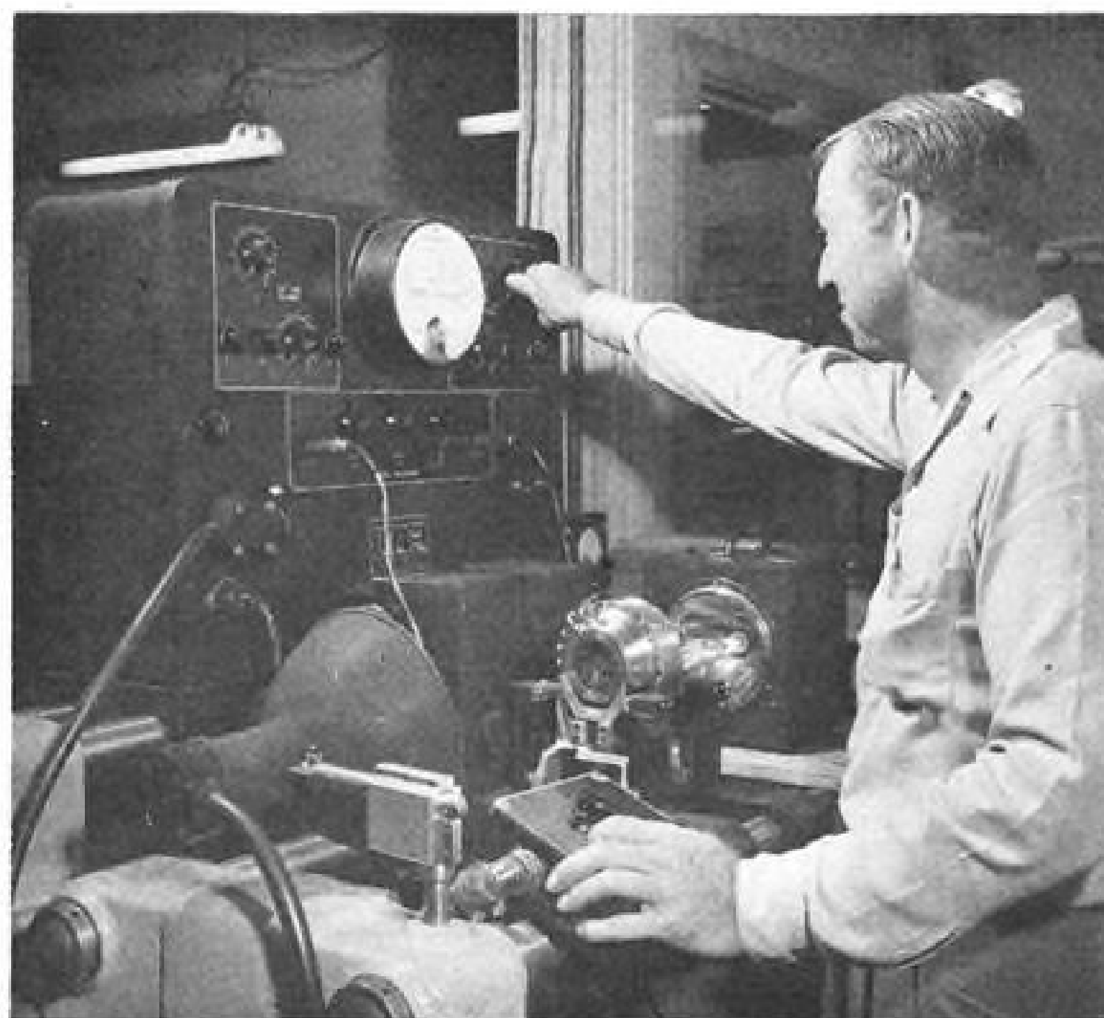
DYNAMIC BALANCING of air bearing gyro components is carried out in the dust-free rooms of North American's precision machine shop.
