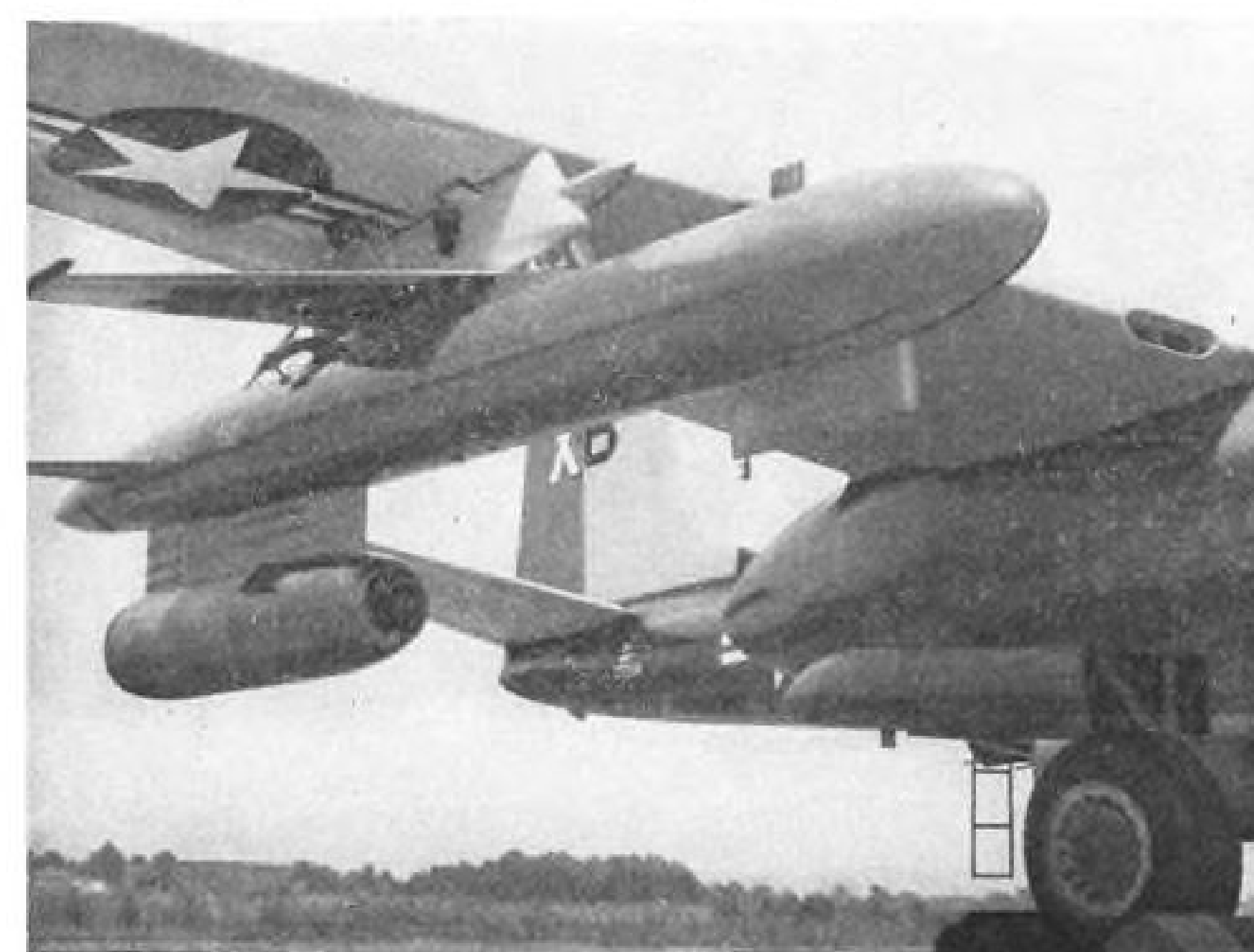
GAME BIRD —Martin's KDM-1 radio-controlled target missile Plover under wing of Navy JD-1.
