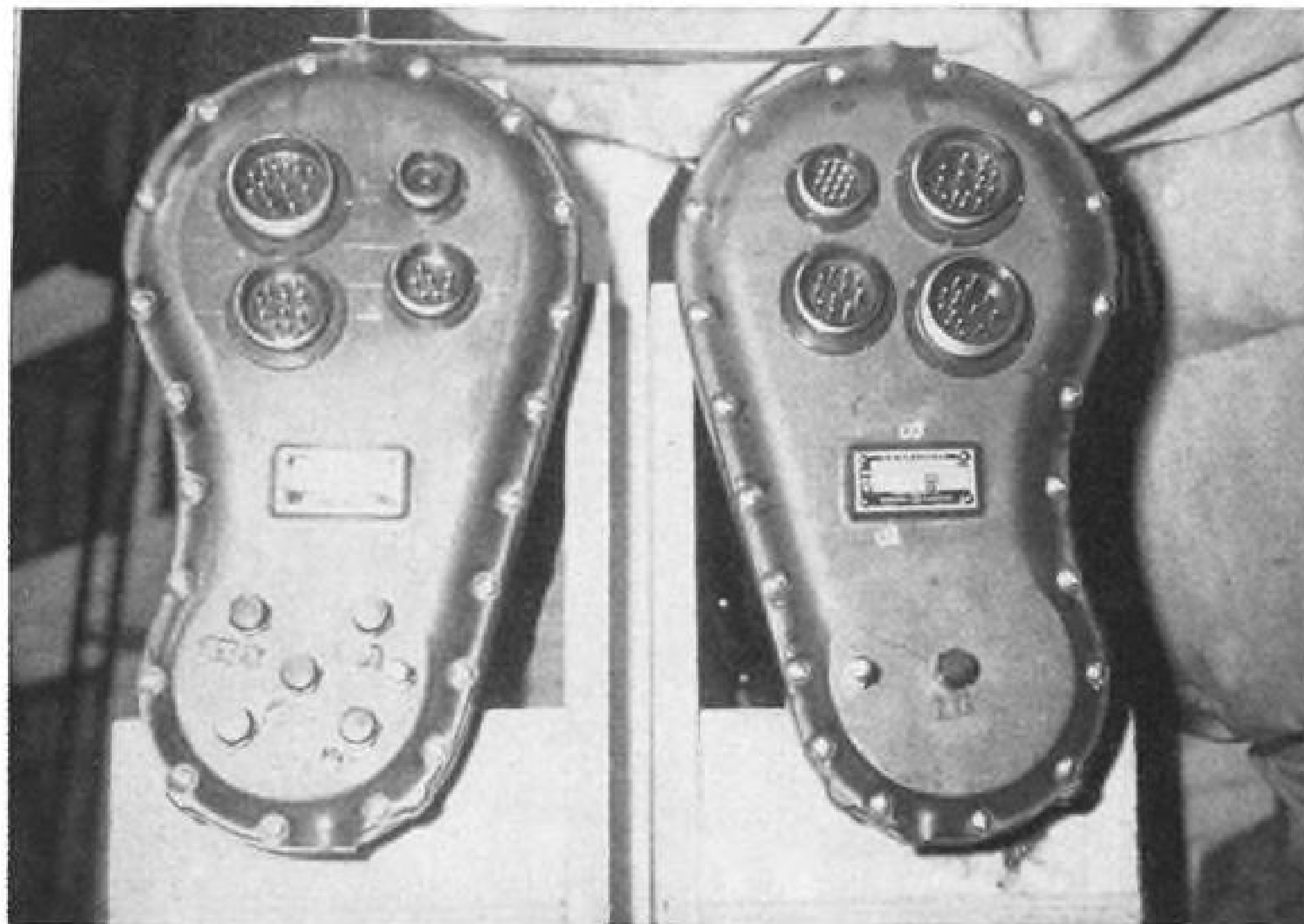
"BRAIN BOXES" on -17 jet control maximum permissible limits of temperature, fuel flow and acceleration that can be handled without damage to engine or aircraft structure.
