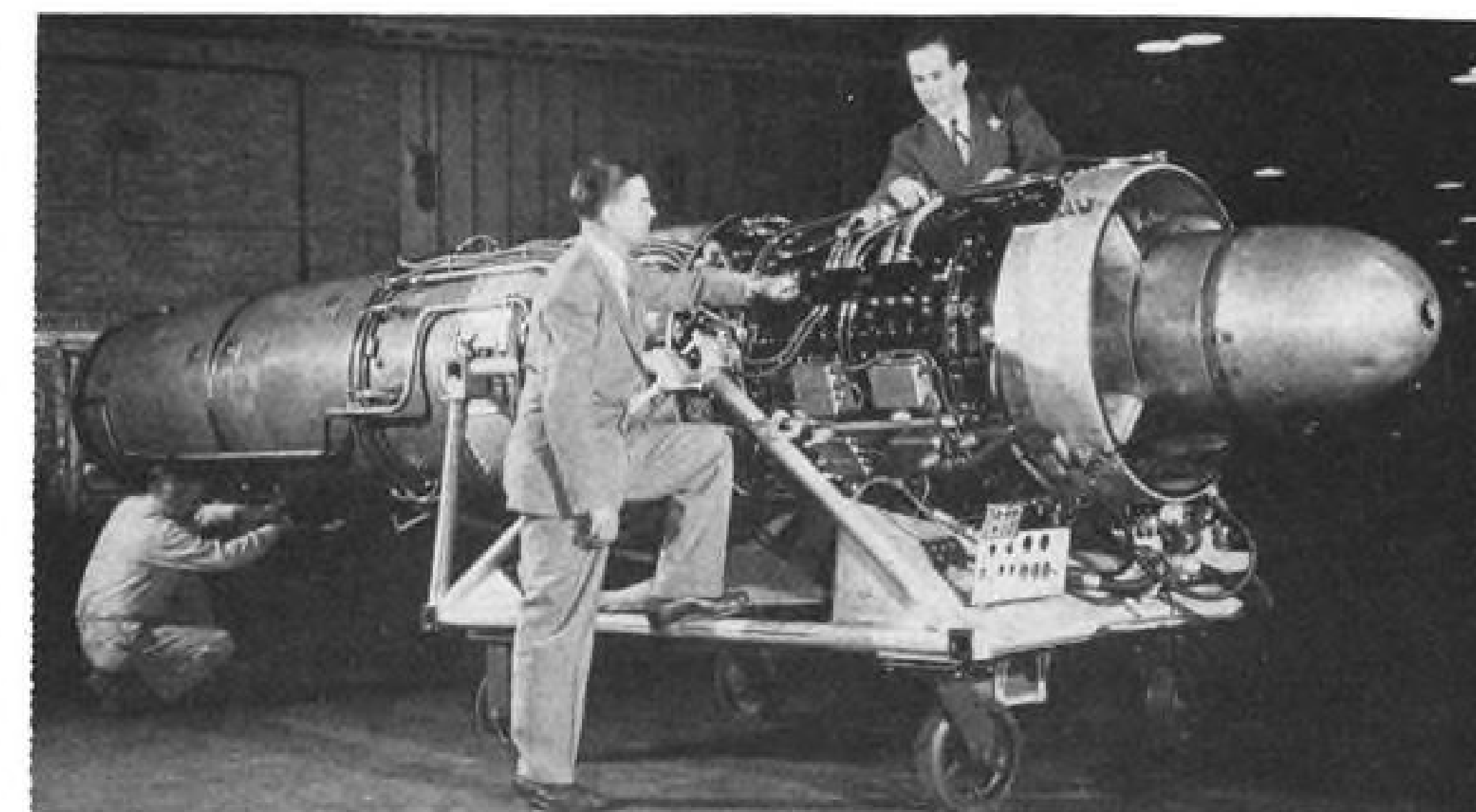
J-47-GE-17 has afterburner, deicing, electronic controls, and fewer strategic materials.
