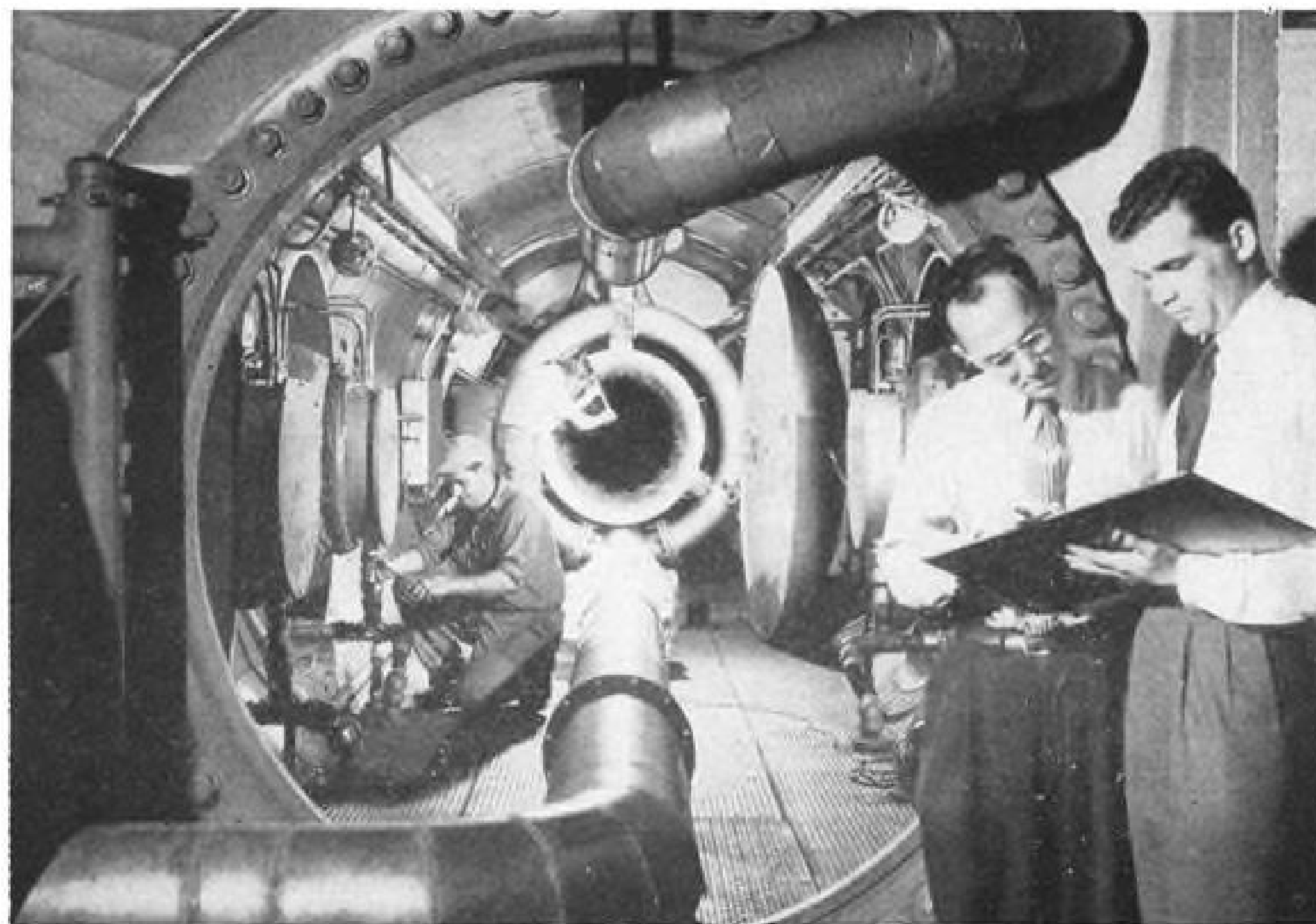
TEST CHAMBER for experimental compressor (blacked out, in rear center). Steel chamber has 10-ft. diameter, is about 40 ft. long. Facility has run about 300 hr. to date.
