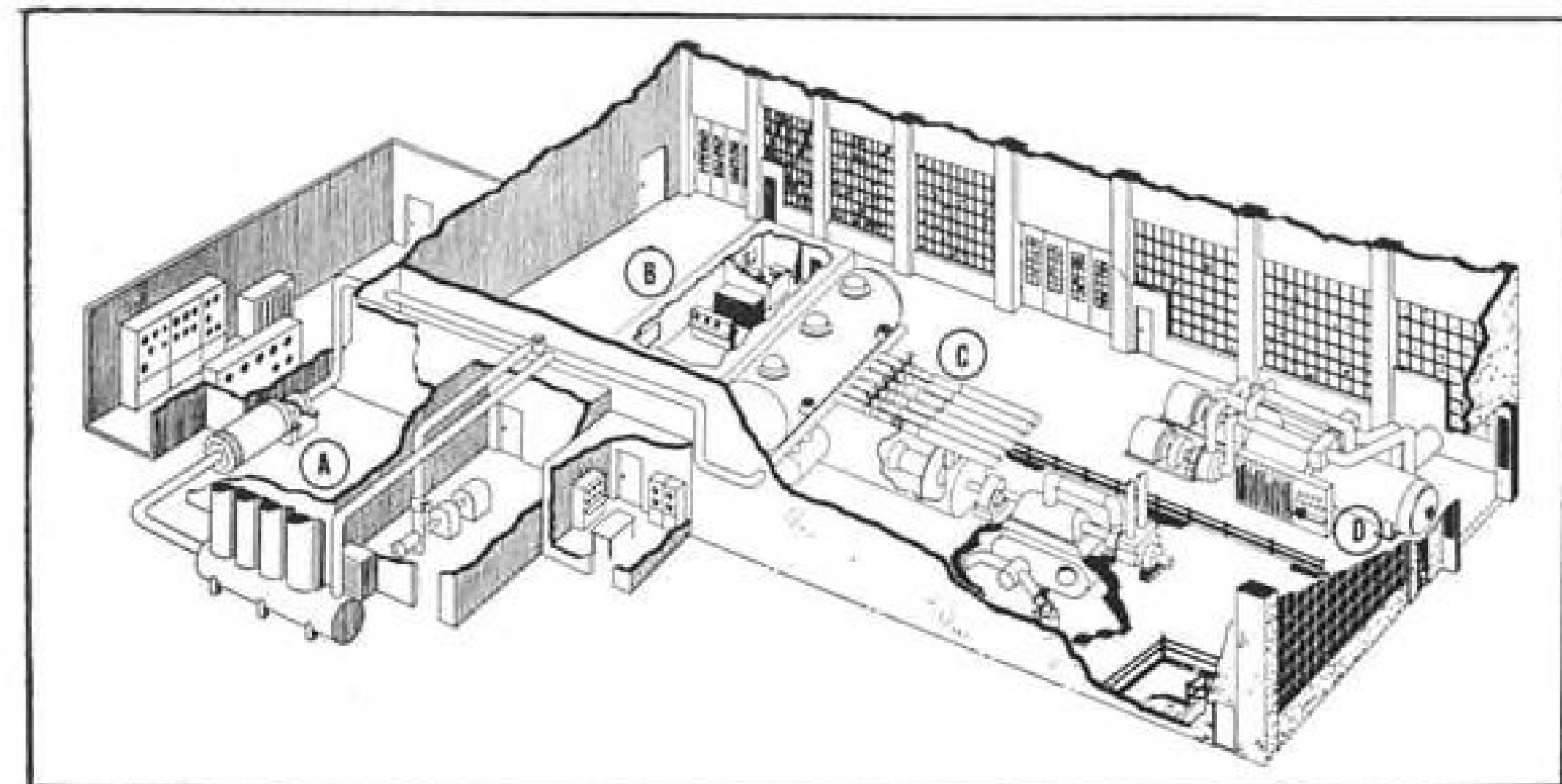
NEW LAB for jet components: A, combustion test stand; B, main control room; C, full-scale compressor stand; D, scale-model stand. Facility will simulate 70,000-ft. height.
