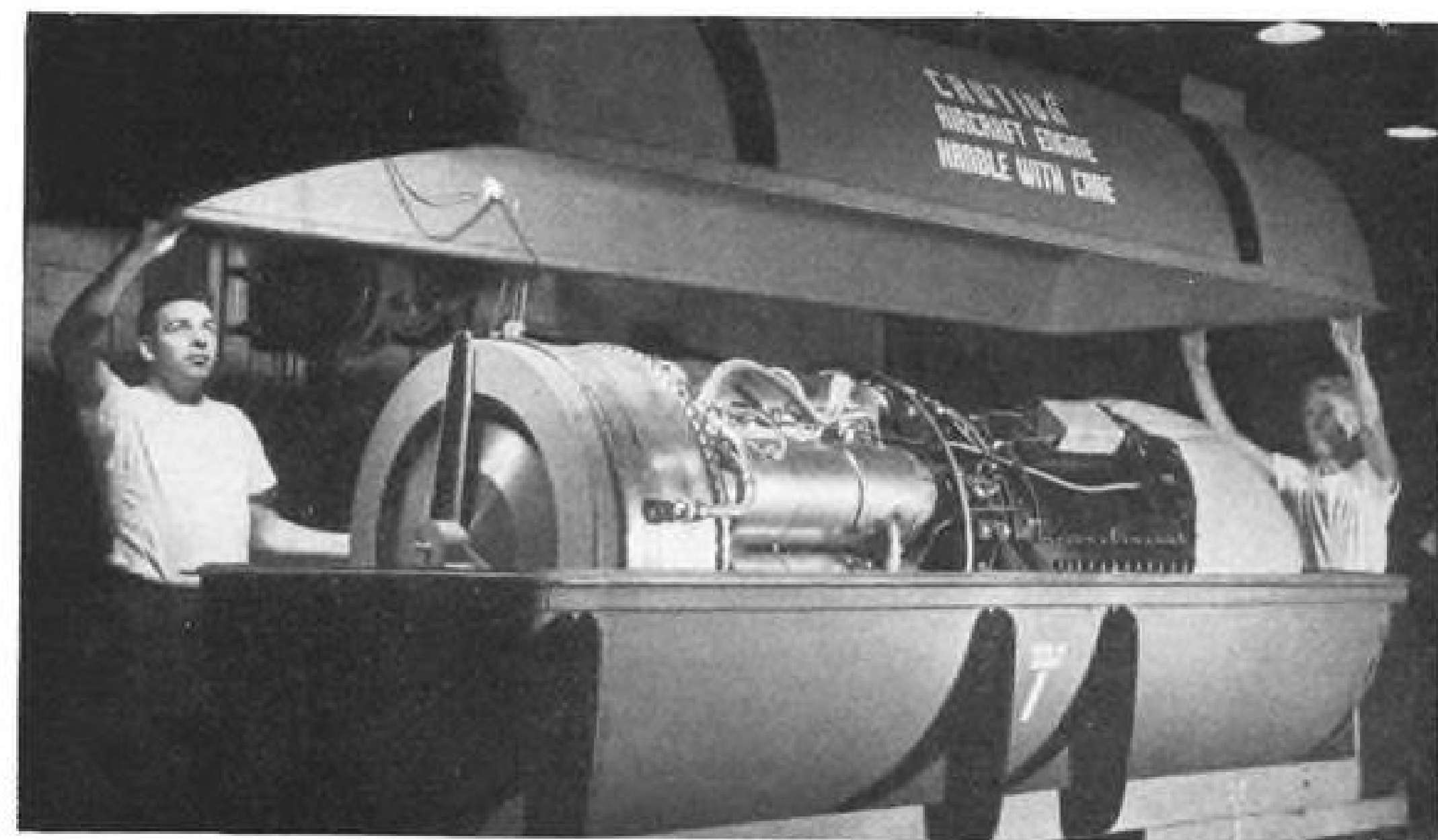
SHIPPING CAN firmly cradles J-47. Unit is non-sinkable, filled with dehydrated air.
