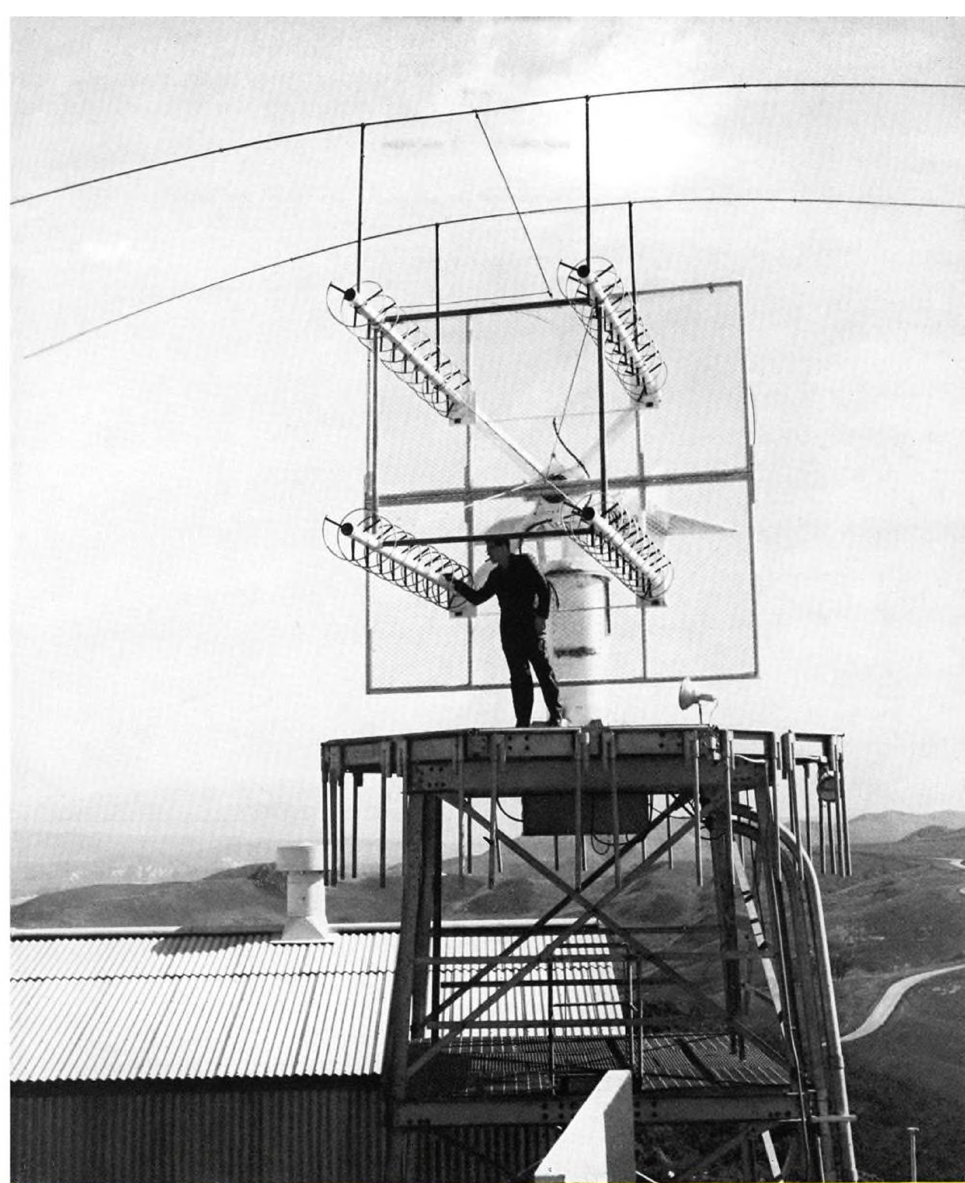
Project Mercury Telemetry Tracking Antenna at Point Arguello, Calif.
