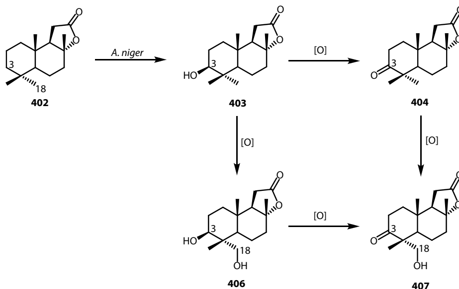
FIGURE 15.116 Biotransformation of (+)-sclareolide ( 402 ) by Aspergillus niger .
