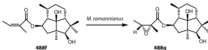
FIGURE 15.144 Biotransformation of 5 \beta ,6 \beta -dihydroxypresilphiperfolane 2 \beta -angelate ( 488f ) by Mucor ramannianus .
