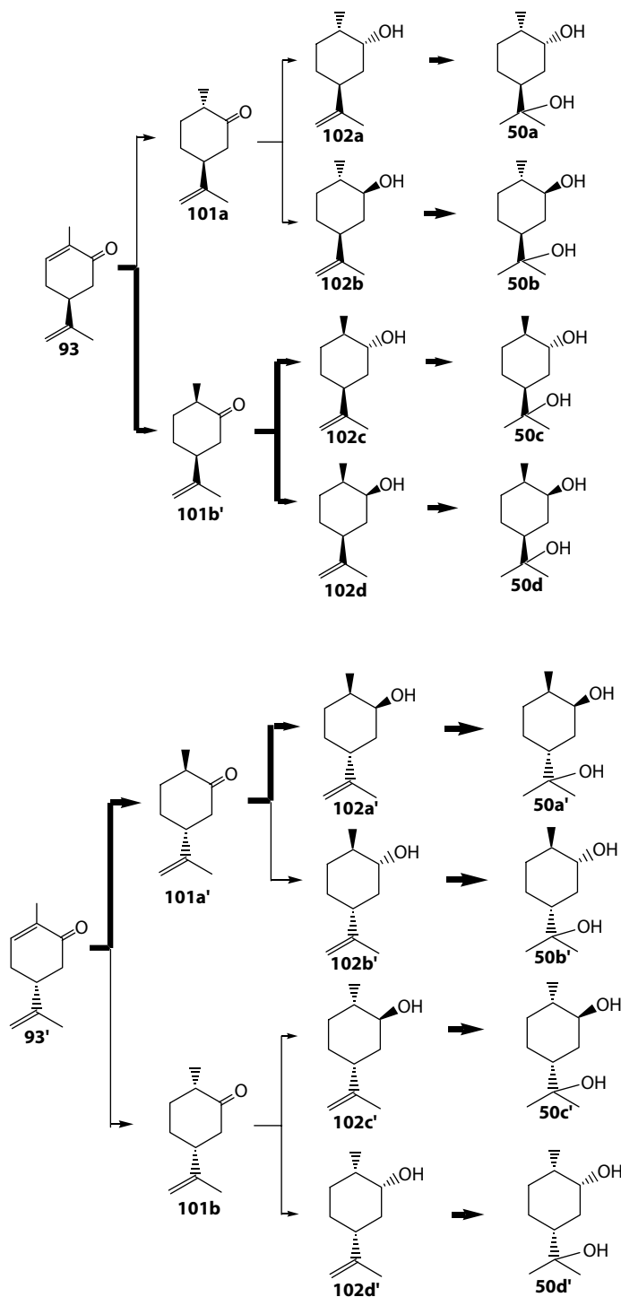
FIGURE 14.99 Formation of eight kinds of 8-hydroxydihydrocarveols ( 50a – 50d , 50a' – 50d' ), dihydrocarvones ( 101a – 101b and 101a' – 101b' ), and dihydrocarveols ( 102a – 102d and 102a' – 102d' ) from (+)- ( 93 ) and (–)-carvone ( 93' ) by Euglena gracilis Z. (Modified from Noma, Y. et al., 1993. Proc. 37th TEAC , pp. 23–25.)
