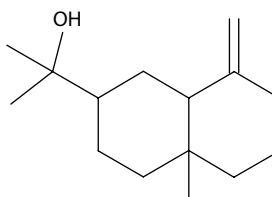
\beta -Eudesmol ( 34 )
