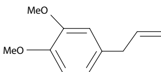
Methyl eugenol ( 27 )
