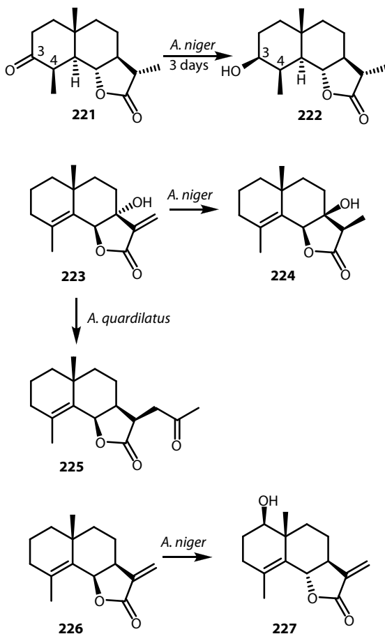
FIGURE 15.67 Biotransformation of C4-epimer ( 221 ) of 214 , 7 \alpha -hydroxyfrullanolide ( 223 ), and frullanolide ( 226 ) by Aspergillus niger and Aspergillus quadricolatus .
