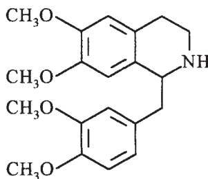
tetrahydropapaverine
