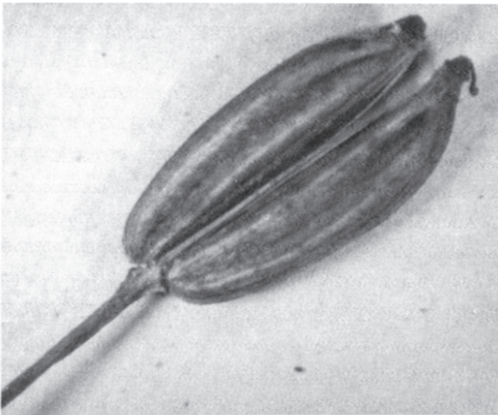
Figure 22 Schizocarp
