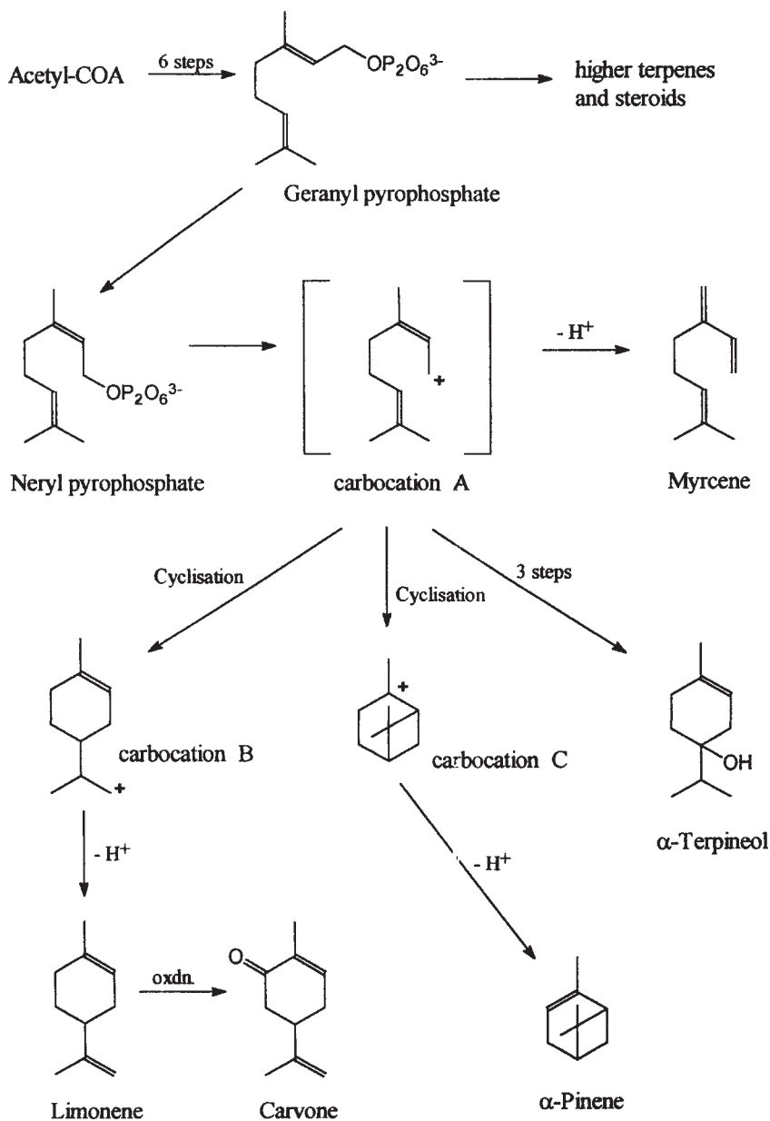
Figure 6 Biogenetic relationship of Carum terpenoid constituents
