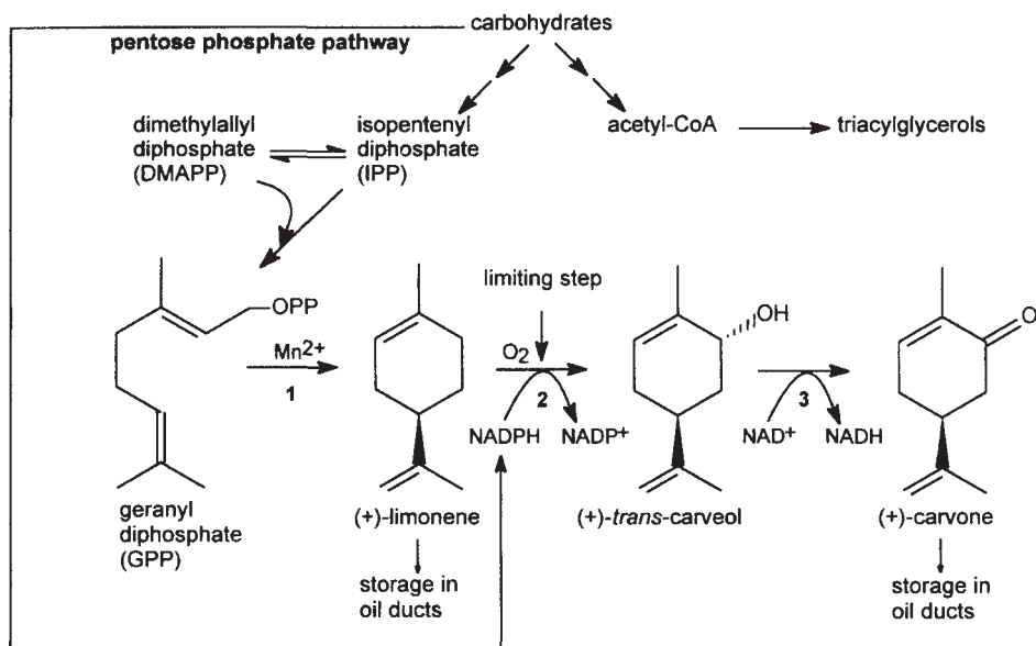
Figure 4 Biosynthetic pathway of limonene and carvone in caraway. Enzymes involved in the final three steps are: (1) (+)-limonene synthase, (2) (+)-limonene hydroxylase and (3) (+)-trans-carveol dehydrogenase
