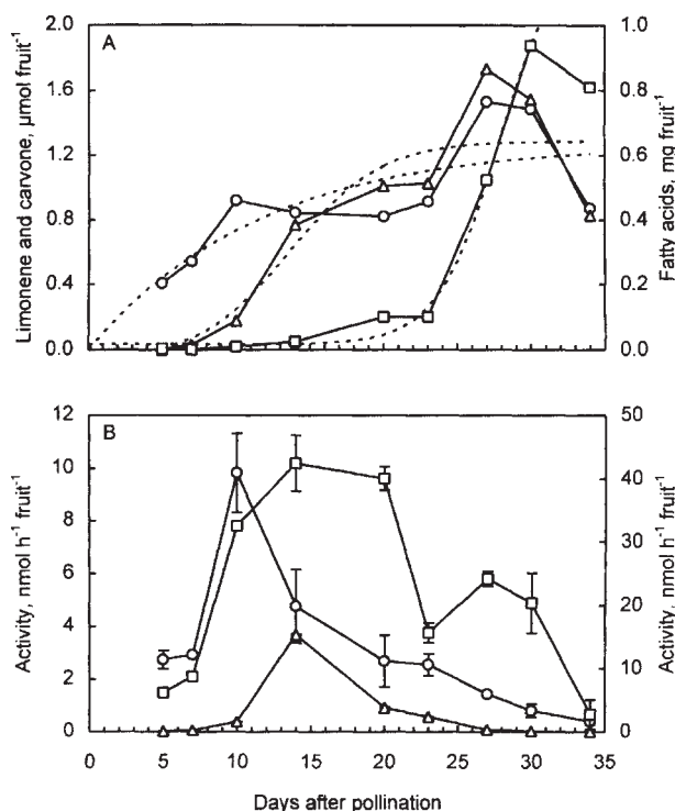
Figure 5 Developmental changes in the contents of limonene (o), carvone ( \Delta ) and fatty acids (seed oil) (e) in caraway fruits (A) and activities of limonene synthase (o), limonene-6-hydroxylase ( \Delta ) (both on the left y-axis) and trans -carveol dehydrogenase (e) (right y-axis) (B). Dotted lines in A represent fitted values
