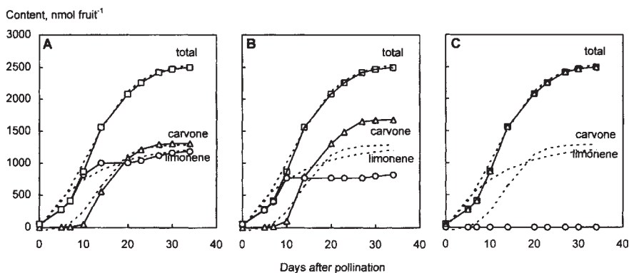
Figure 7 Developmental changes in limonene, carvone and total essential oil contents determined by gas chromatography (broken lines; data from Figure 5A) and calculated using a regression model with the enzyme activities from Figure 5B: (o) limonene, ( \Delta ) carvone and ( \square ) total essential oil. The activity of limonene-6-hydroxylase was corrected to account for the loss of activity during extraction. Towards maturation an increasing substrate competition was assumed to occur. (A) model describing the present situation, (B) using doubled limonene hydroxylase activity and (C) using a limonene-6-hydroxylase activity continuously at the maximum level of 14 DAP (Figure 6)
