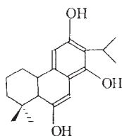
Figures 37–54 Abietane type diterpenoids.
