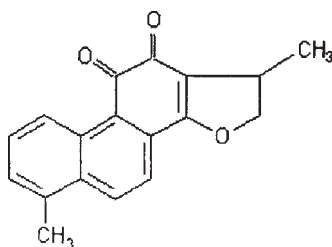
Figure 12 15, 16-dihydroxytanshinone I.
