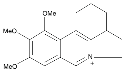
22 roserine
