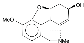
Galanthamine
