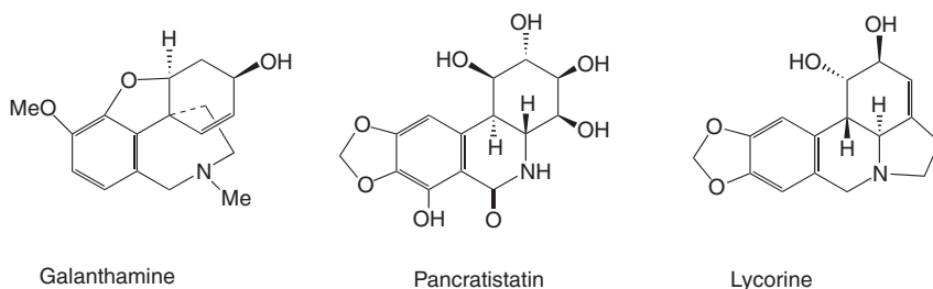
Figure 11.1 Chemical structures of Amaryllidaceae alkaloids with important biological activities.
