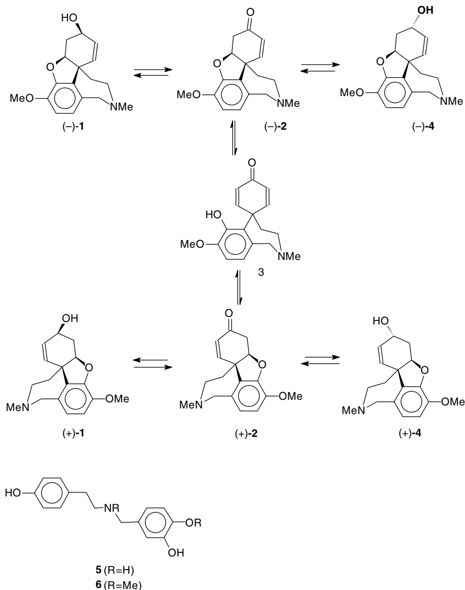
Figure 12.1 (Above) The equilibrium process between narwedine hydroxydienone ( 3 ) and its enantiomers ( 2 ) and oxidative/reductive interconversion between ( 2 ) and galanthamine ( 1 ) and epi -galanthamine ( 4 ) enantiomers. (Below) Norbelladine ( 5 ) and N,O -dimethylnorbelladine ( 6 ).
