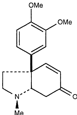
Figure 6.1 Sceletium type alkaloid mesembrenone ( 82 ) isolated from N. pallidulus .
