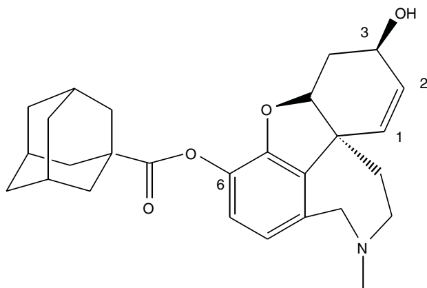
Adamantyl-ester galanthamine, 2
