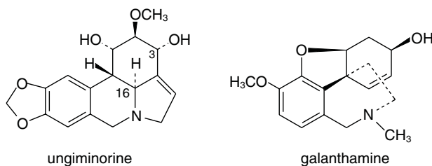
Figure 15.5 Structure of ungimnorine and galanthamine.
