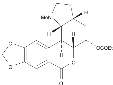
38 poetinatine
