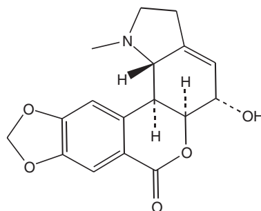
Hippeastrine 8
