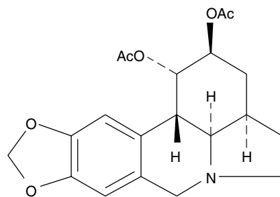
17 nartazine
