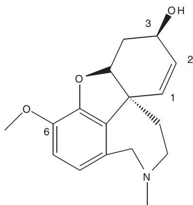
Galanthamine, 1
