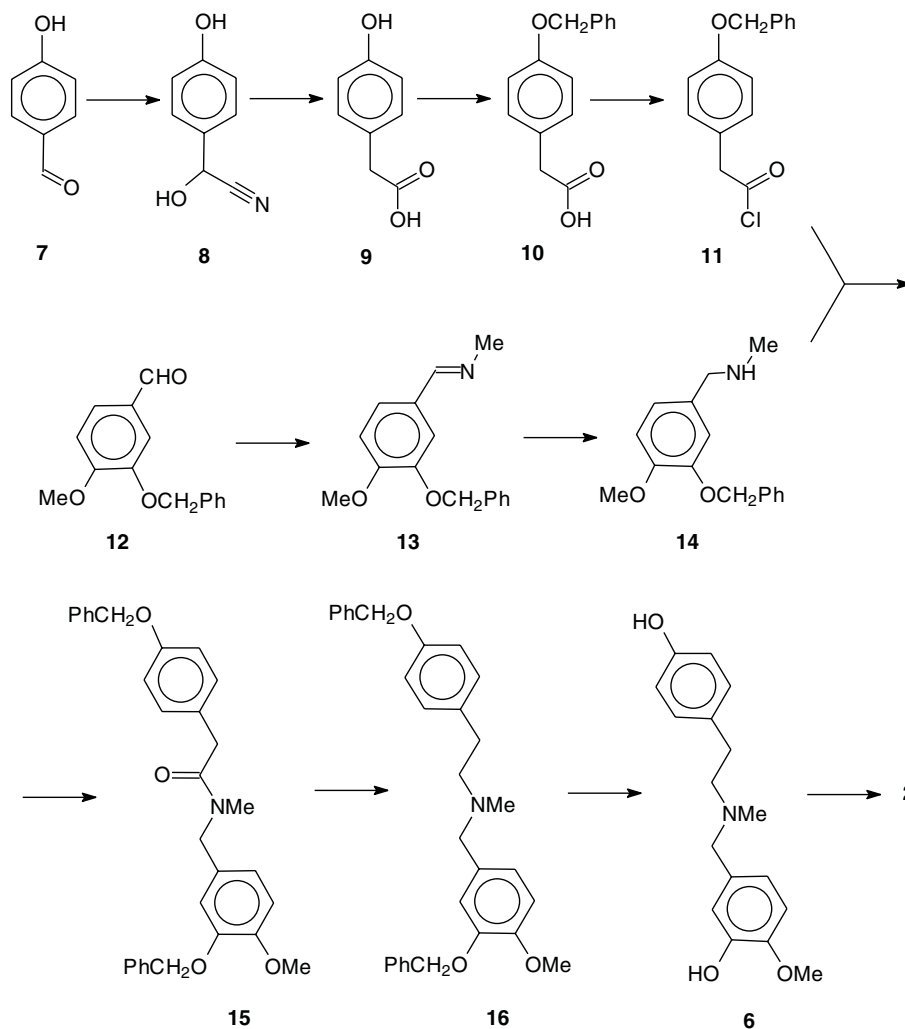
Figure 12.2 Synthesis of narwedine ( 2 ) via N,O -dimethylnorbelladine ( 6 ) (Barton and Kirby, 1960, 1962).
