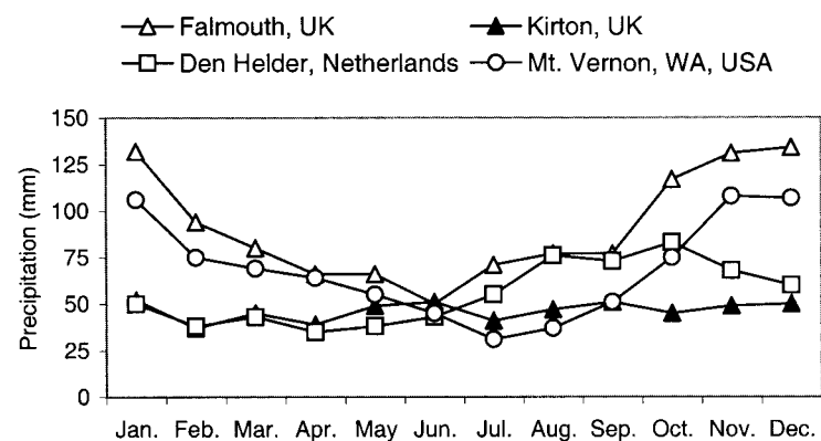
Figure 4.1 Mean monthly weather data for Falmouth (south-west England), Kirton (eastern England), Den Helder (the Netherlands) and Mt Vernon (Washington State). Data are long-term means, for at least 30 years to 1999, from Washington Post historical weather data and Horticulture Research International.
