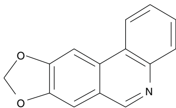
65 trisphaeridine
