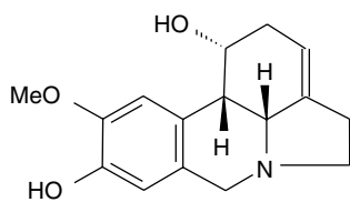
Fortucine
