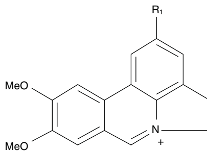
20 vasconine
