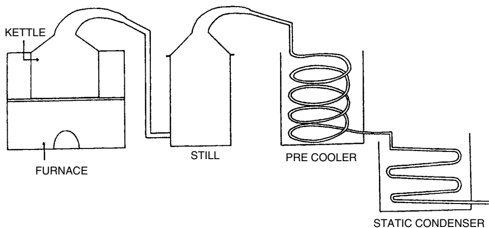
Figure 5.8 Diagram of a traditional cinnamon leaf oil distillation unit.
