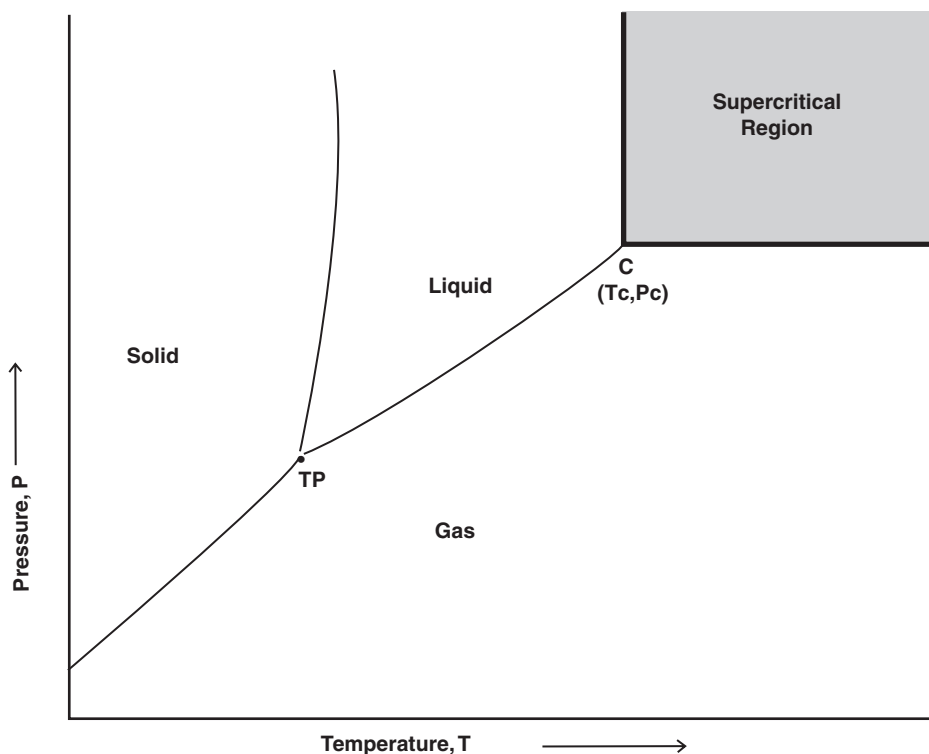
Figure 11.12 Phase diagram.
