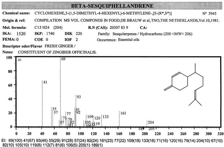
Figure 3.8 Mass spectra of \beta -bisabolene and \beta -sesquiphellandrene.
