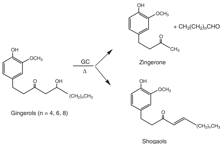
Scheme 3.1 Thermal degradation of gingerols during gas chromatography. (adapted from Connell (1970))
