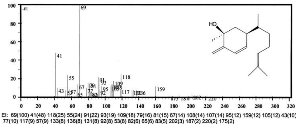
Figure 3.13 Mass spectra of trans - and cis -β-sesquiphellandrols.
