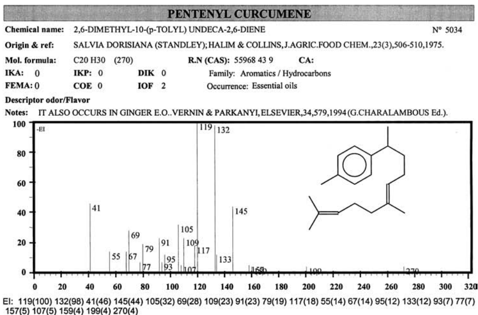
Figure 3.10 Mass spectra of ar-curcumenyl and pentenyl curcumenyl.
