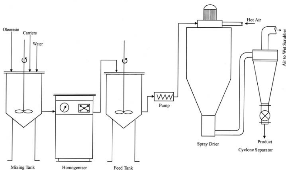
Figure 11.16 Microencapsulation/spray drying.
