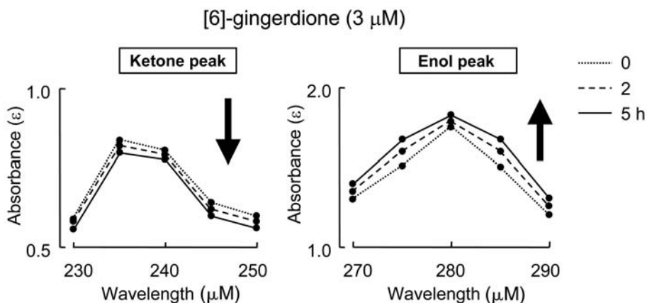
Figure 13.4 UV absorption spectrum for (6)-gingerdione ( 3\text{ }\mu\text{M} ) just after preparation (0 hour) and after incubation for 2 and 5 hours at 27^\circ\text{C} . (From Kimura et al., 1989c.)
