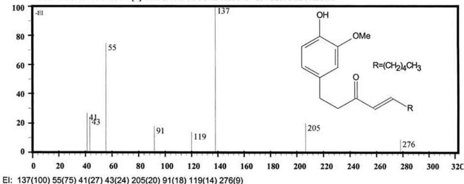
Figure 3.16 Mass spectra of zingerone.
