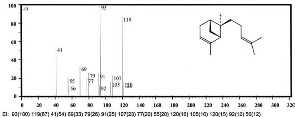
Figure 3.9 Mass spectra of \alpha -zingiberene and \alpha -bergamotene.
