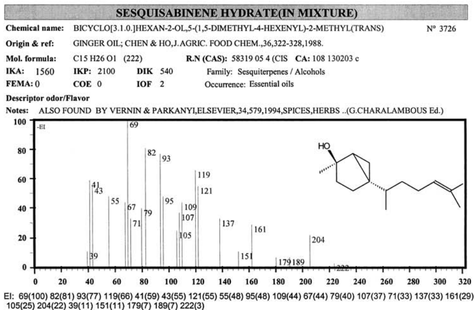
Figure 3.12 Mass spectra of 10-epi- \gamma -eudesmol and sesquisabinene hydrate.
