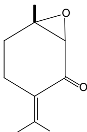
piperitenone oxide
