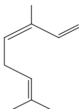
(E)-β-ocimene
