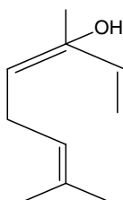
linalool
