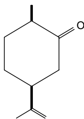
cis-dihydrocarvone
