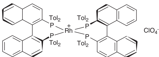
FIGURE 10.14 Rhodium ( S )-Tol-BINAP complex, the key catalyst in the Takasago process.
