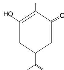
6-hydroxycarvone
