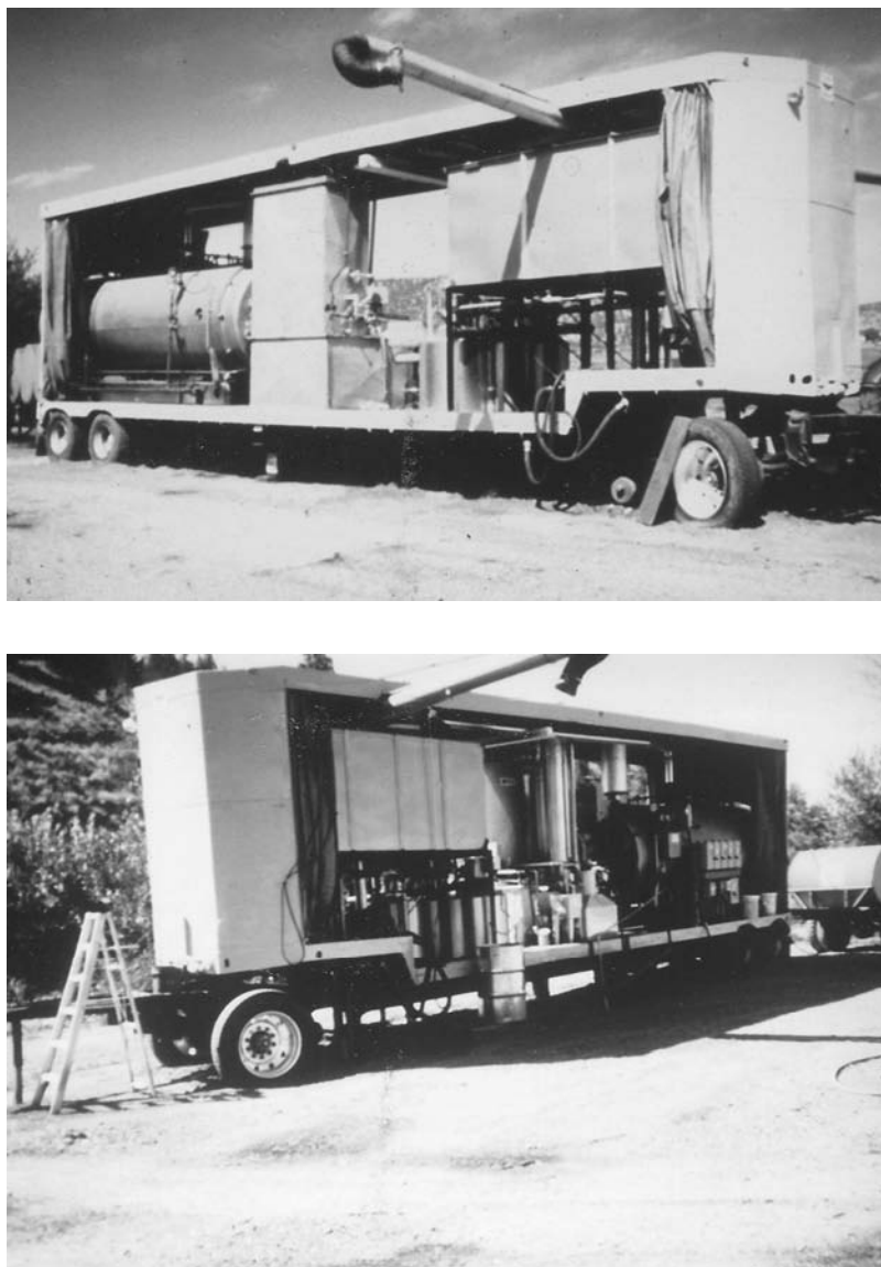
FIGURE 6.6 Example of mobile distillery designed by Newhouse Manufacturing, Inc.
