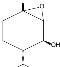
1,2-epoxymenthol
