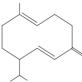
germacrene D
