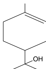
α-terpineol
