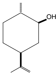
dihydrocarveol
