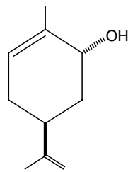
trans-carveol
