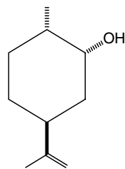
neodihydrocarveol
