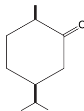
cis -carvomenthone
