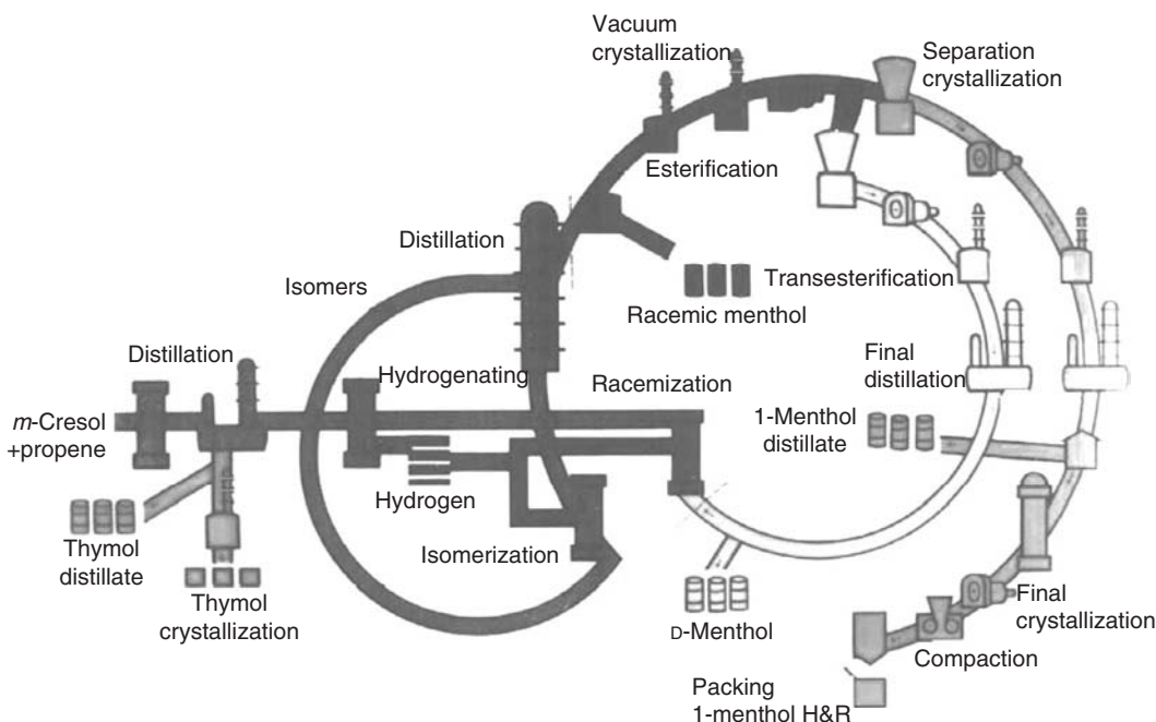
FIGURE 10.10 Flow scheme of the Haarmann and Reimer menthol process.
