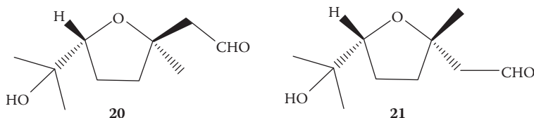
FIGURE 8.7 Structure of 20 = trans-7-hydroxy-3,7-dimethyl-3,6-oxyoctanal, 21 = cis-7-hydroxy-3,7-dimethyl-3,6-oxyoctanal.
