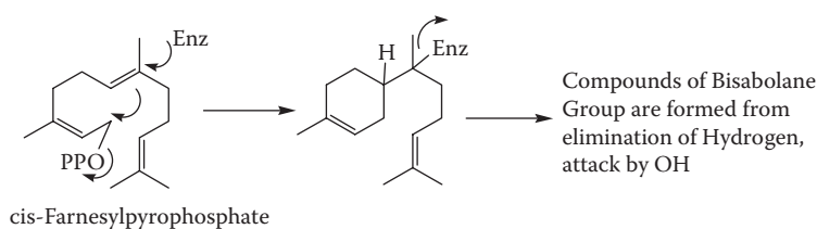
SCHEME 2.9 Cyclization of cis -FPP to monocyclic bisabolane compounds.
