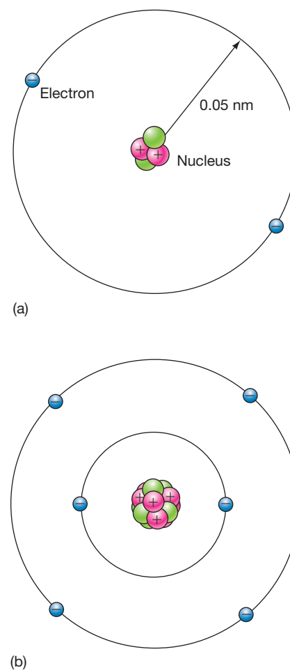
▲ FIGURE 2.21 Helium and Carbon (a) A helium atom in its ground state has two electrons within the lowest-energy orbital around a nucleus containing two protons and two neutrons. (b) A carbon atom in its ground state has six electrons orbiting around a six-proton, six-neutron nucleus—two of the electrons in an inner orbital and the other four at a greater distance from the center.
