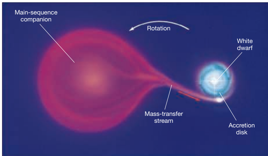
◀ FIGURE 12.14 Close Binary System If a white dwarf in a binary system is close enough to its companion, its gravitational field can tear matter from the companion's surface. Notice that the matter does not fall directly onto the white dwarf's surface. Instead, it forms an accretion disk of gas spiraling down onto the dwarf.
