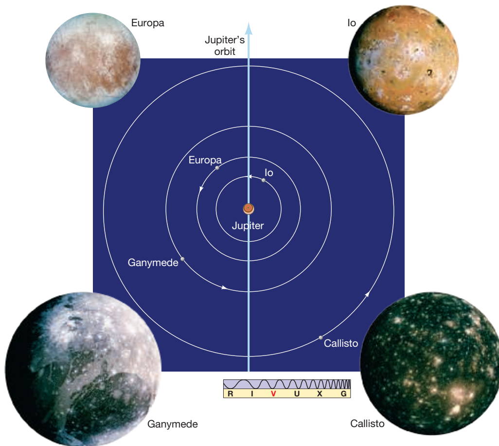
◀ FIGURE 8.2 Galilean Moons INTERACTIVE The orbits of the four Galilean moons of Jupiter, drawn to scale, as seen from above the planet's north pole. The four insets show actual images of those moons, taken by the Galileo spacecraft and scaled here as they would appear from a distance of about 1 million kilometers. (NASA)
