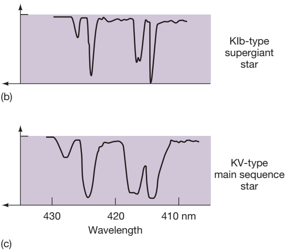
FIGURE 10.17 Luminosity Classes (a) Approximate locations of the standard stellar luminosity classes in the H–R diagram. The widths of absorption lines also provide information on the density of a star’s atmosphere. The denser atmosphere of a main-sequence K-type star has broader lines (c) than a giant star of the same spectral class (b).
