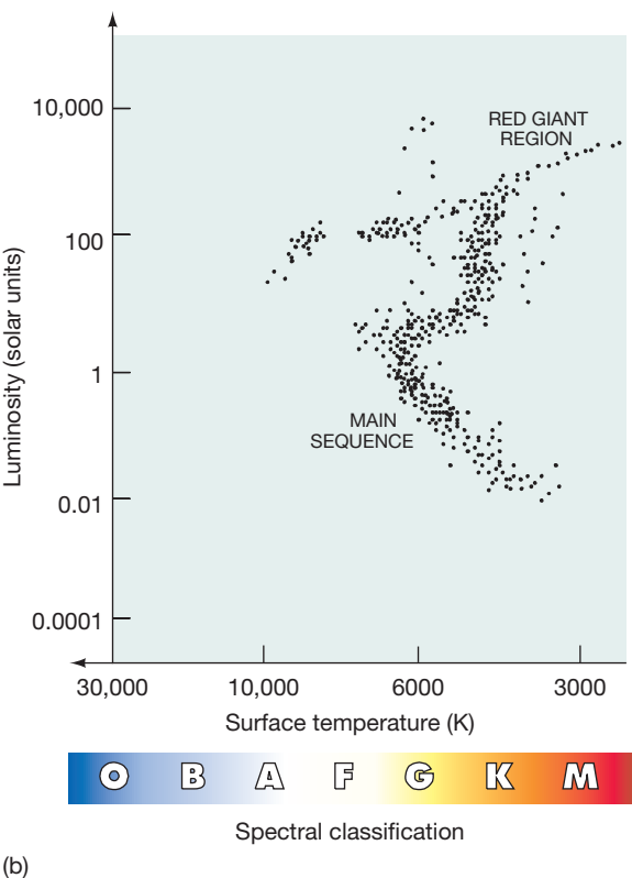
▲ FIGURE 11.30 Globular Cluster (a) The globular cluster Omega Centauri is approximately 5000 pc from Earth and some 40 pc in diameter. (b) An H–R diagram for some of its stars. (P. Seitzer)
