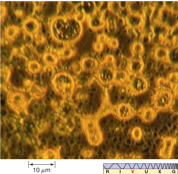
◀ FIGURE 18.6 Interstellar Globules These oily, hollow droplets rich in organic molecules were made by exposing a freezing mixture of primordial matter to harsh ultraviolet radiation. When immersed in water, the larger ones display cell-like membrane structure. Although they are not alive, they bolster the idea that life on Earth could have come from space. (NASA)
