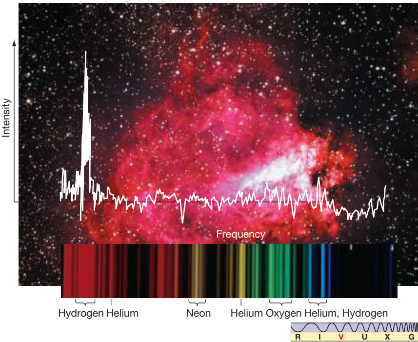
▼ FIGURE 11.10 Nebular Spectrum The visible spectrum of the hot gases in a nearby star-forming region known as the Omega Nebula (M17). Shining by the light of several very hot stars, the nebula produces a complex spectrum of bright and dark lines (bottom), also shown here as an intensity trace from red to blue (center). (ESO)
