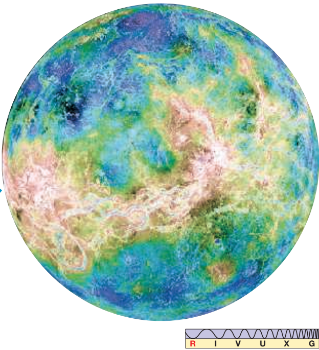
► FIGURE 6.14 Venus Magellan Map A planetwide mosaic of Venus made from Magellan images, colored in roughly the same way as Figure 6.13 to represent altitude: blue is lowest, white highest. (NASA)
