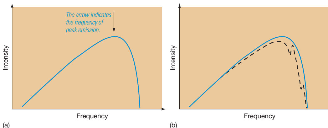
◀ FIGURE 2.10 Blackbody Curves, Ideal vs.
