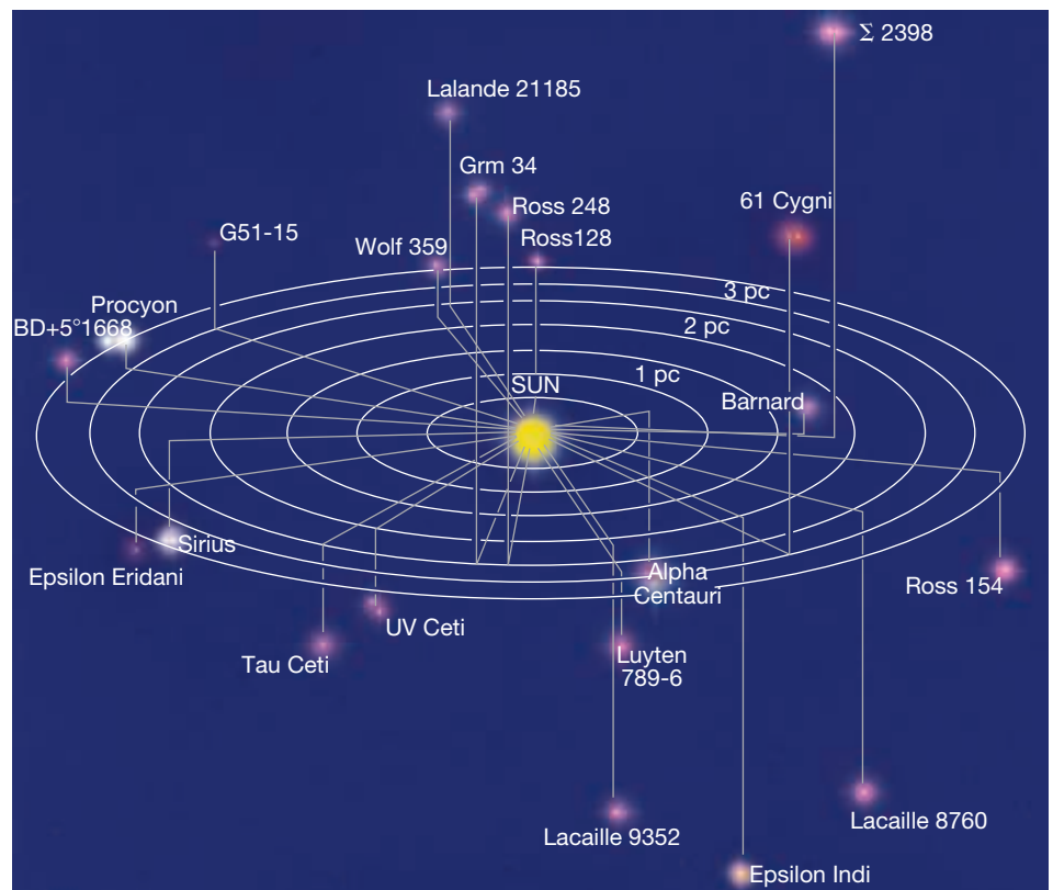
▼ FIGURE 10.2 Sun's Neighborhood A plot of the 30 closest stars to the Sun, projected so as to reveal their three-dimensional relationships. All lie within 4 pc (about 13 light-years) of Earth. The gridlines represent distances in the Galactic plane, and the vertical lines denote distances perpendicular to that plane.
