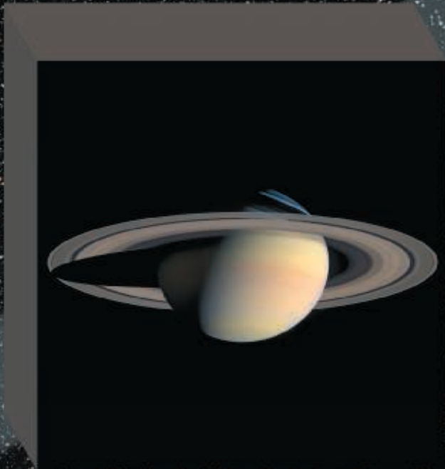
Saturn \sim 10^8 m
