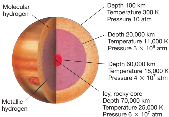
▲ FIGURE 7.19 Jupiter's Interior Jupiter's internal structure, as deduced from spacecraft measurements and theoretical modeling. Pressure and temperature increase with depth, and the atmosphere gradually liquefies over the outermost few thousand kilometers. Below 20,000 km, the hydrogen behaves like a liquid metal. At the center of the planet lies a rocky core (red region), itself larger than any of the terrestrial planets.
