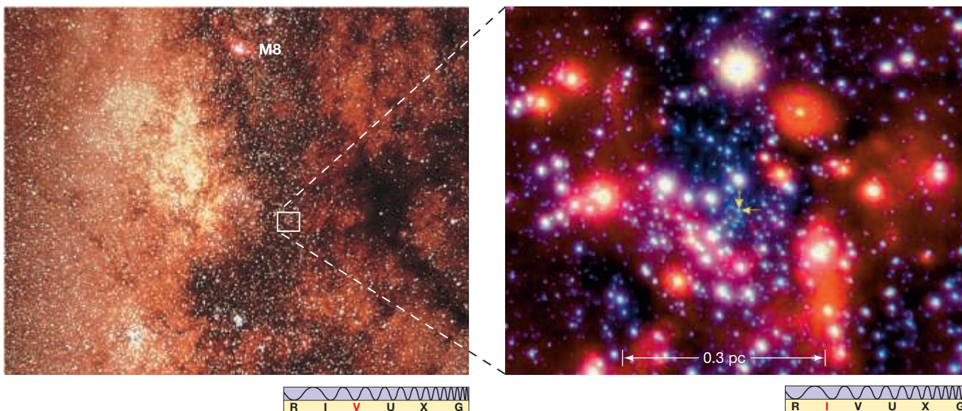
▼ FIGURE 14.22 Galactic Center INTERACTIVE Photograph of stellar and interstellar matter in the direction of the Galactic center. The field is roughly 20°, top to bottom, and is a continuation of the bottom part of Figure 11.5. The overlaid box indicates the location of the center of our Galaxy. The inset shows an adaptive-optics infrared view of the dense stellar cluster surrounding the Galactic center, whose very core is indicated by the twin arrows. (AURA; ESO)
