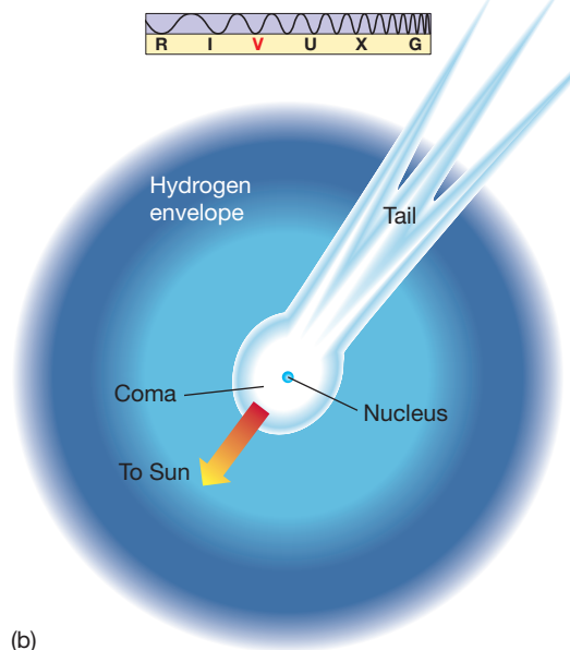
▲ FIGURE 4.9 Halley's Comet (a) Halley's Comet in 1986, about 1 month before it rounded the Sun. (b) Diagram of a typical comet, showing the nucleus, coma, hydrogen envelope, and tail, approximately to the same scale as in part (a). (c) The inset is Halley's nucleus, as seen by the European Giotto spacecraft, showing it to be very dark. The Sun is toward the left in this image. The brightest areas are jets of evaporated gas and dust spewing from the comet's nucleus. (NOAO ESA/Max Planck Institute)
