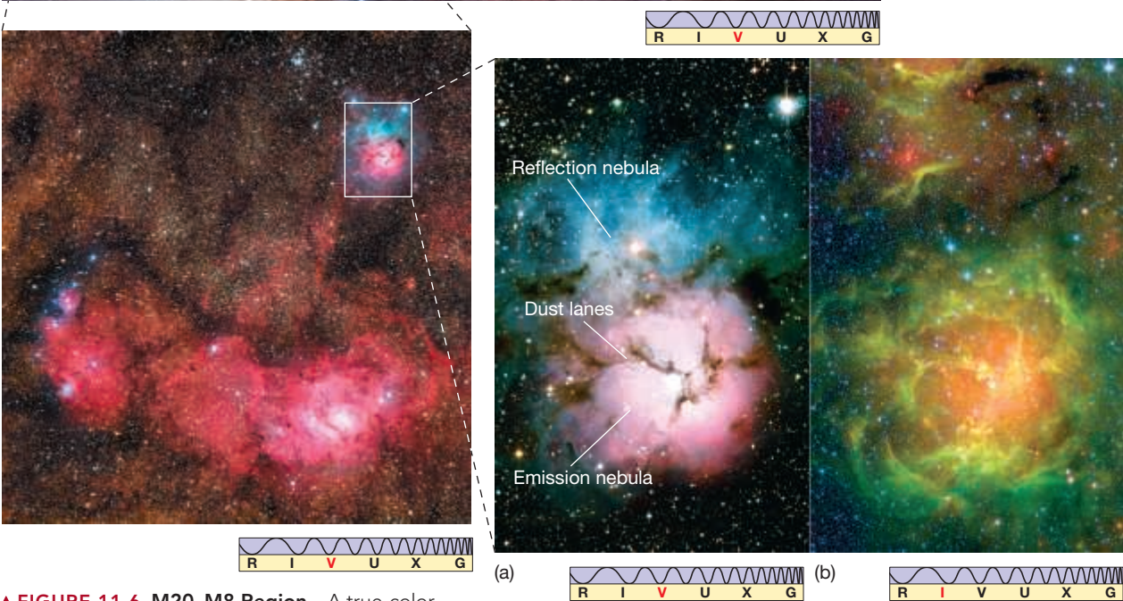
▲ FIGURE 11.6 M20–M8 Region A true-color enlargement of the bottom of Figure 11.5, showing M20 (top) and M8 (bottom) more clearly. ( R. Gendler )
