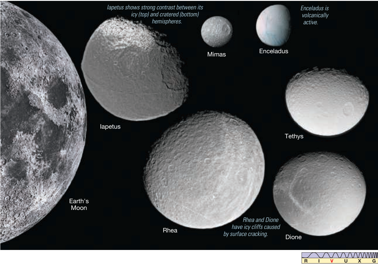
◀ FIGURE 8.15 Saturnian Moons Saturn’s six medium-sized satellites, to scale, as imaged by the Cassini spacecraft. All are heavily cratered and all are shown here in natural color. For scale, part of Earth’s Moon is shown at left. (UC/Lick Observatory; NASA)
