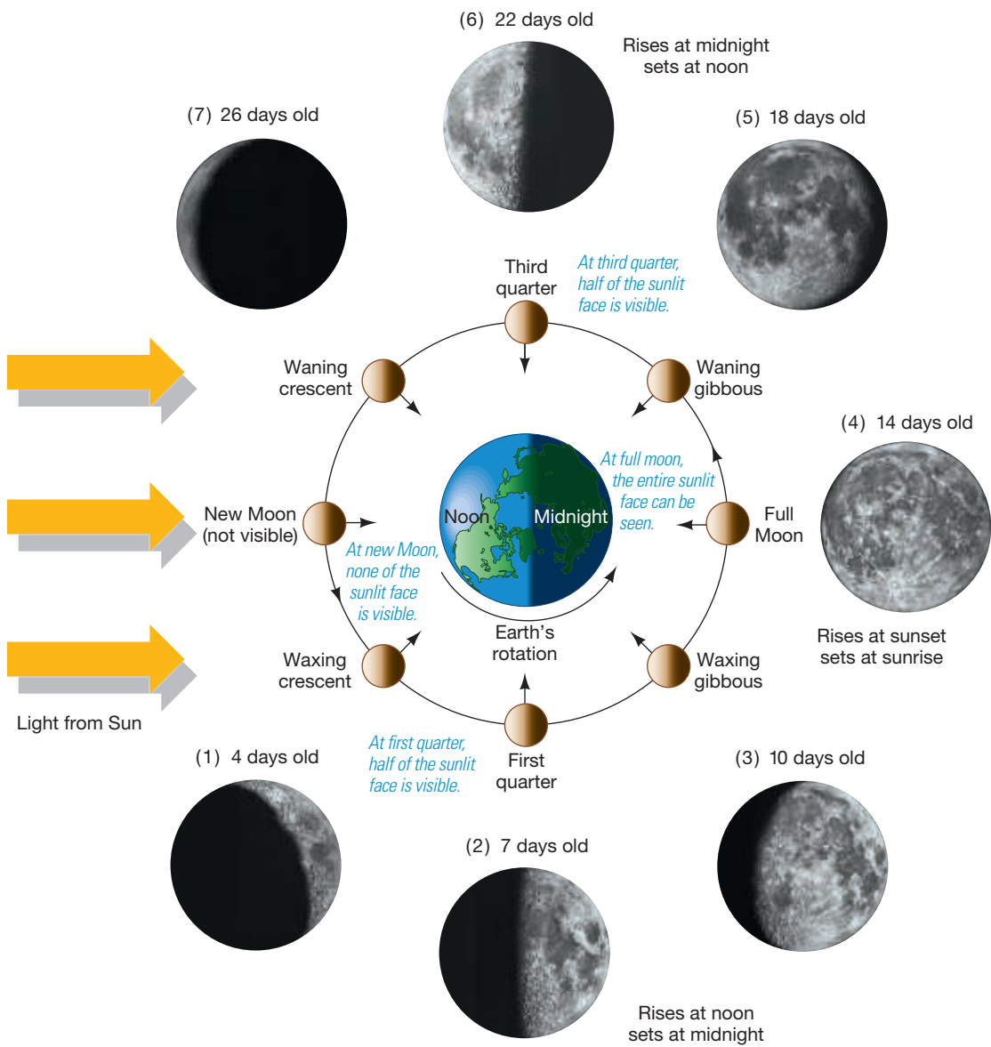
◀ FIGURE 0.13 Lunar Phases (a) Because the Moon orbits Earth, this top-down view shows how the visible fraction of the lunar sunlit face varies from night to night, although the Moon always keeps the same face toward our planet. (Note the location of the small, straight arrows that mark the same point on the lunar surface at each phase shown.) The complete cycle of lunar phases takes about 29 days to complete. Rising and setting times for some phases are also indicated. (b) A side view shows how the Moon's orbit is inclined at about 5^\circ to the ecliptic, so not all orbital configurations produce an eclipse. (Insets: UC/Lick Observatory)
