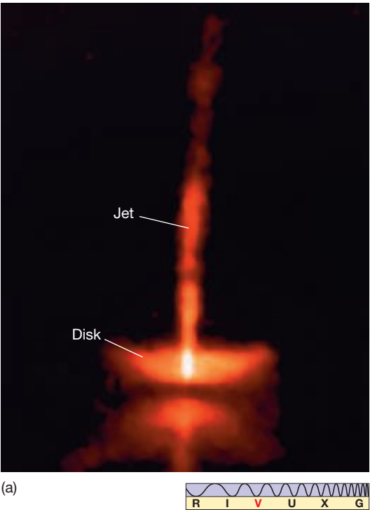
▼ FIGURE 11.24 Protostellar Outflow (a) This remarkable image (at right) shows two jets emanating from the young star system HH30, the result of matter accreting onto an embryonic star near the center. (b) The view below of the Orion molecular cloud shows the outflow from a newborn star, still surrounded by nebular gas. The inset shows a pair of jets called HH1/HH2, formed when matter falling onto another protostar (still obscured by the dusty cloud fragment from which it formed) creates a pair of high-speed jets of gas perpendicular to the flattened protostellar disk. The jets are nearly 1 light-year across. Several more Herbig-Haro objects can be seen at top right—one of them resembling a "waterfall." (AURA; NASA)
