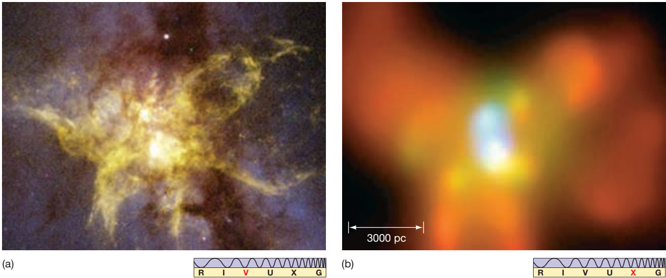
► FIGURE 16.17 Binary Black Hole Hole These (a) optical ( Hubble ) and (b) X-ray ( Chandra ) images of the starburst galaxy NGC 6420 show two supermassive black holes (the blue-white objects near the center of the X-ray image) orbiting about 1 kpc apart. Theoretical estimates imply that they will merge in about 400 million years, releasing an intense burst of gravitational radiation. ∞ (Discovery 13-1) (NASA)
