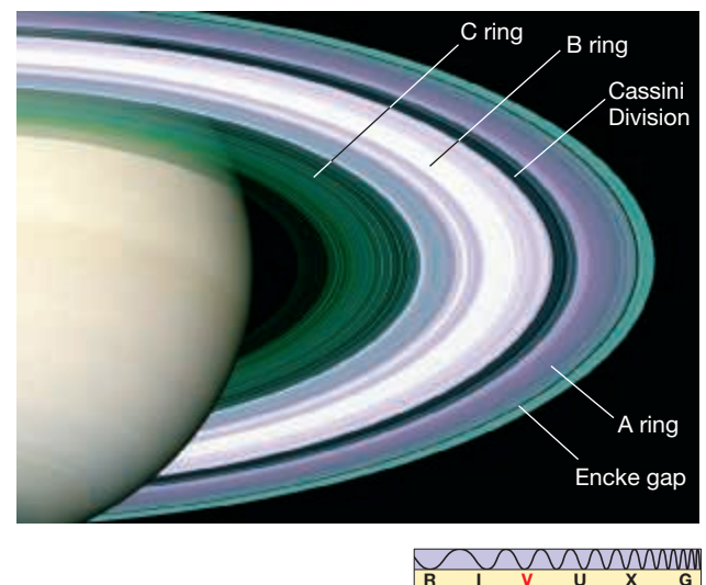
▲ FIGURE 8.19 Saturn's Rings Saturn as observed by the Cassini spacecraft in 2005. The main ring features are marked and are shown here in false color in order to enhance contrast. (NASA/ESA)
