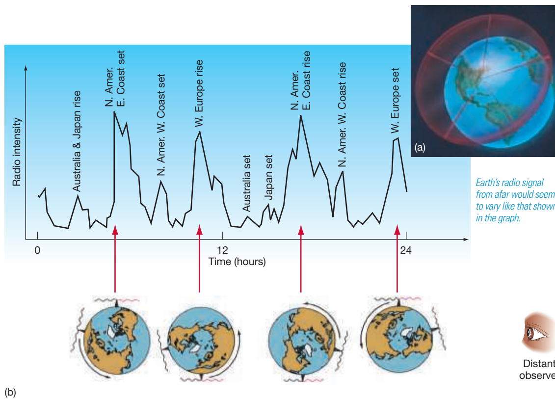
FIGURE 18.15 Earth's Radio Leakage Radio radiation leaks from Earth into space because of the daily activities of our technological civilization. (a) Most radio and television transmitters broadcast their energy parallel to Earth's surface, sending a great "sheet" of electromagnetic radiation into interstellar space. (b) Because the great majority of transmitters are clustered in the eastern United States and western Europe, a distant observer would detect blasts of radiation from Earth as our planet rotates each day.
