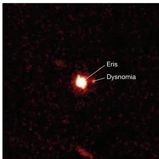
◀ FIGURE 8.35 Kuiper Belt Object (a) The trans-Neptunian object Eris and its small moon Dysnomia (named after the Greek goddess of discord and her daughter of chaos and lawlessness) were imaged in the infrared at the Keck Observatory in Hawaii. (b) An artist's conception of the Eris system, with Dysnomia at the top and the distant Sun at right. (Keck)
