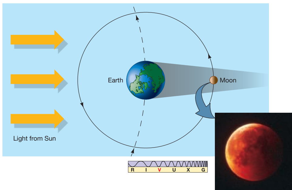
▲ FIGURE 0.14 Lunar Eclipse INTERACTIVE When the Moon passes through Earth's shadow, we see a darkened, copper-colored Moon, as shown by the partial eclipse in the inset photograph. The red coloration is caused by sunlight deflected by Earth's atmosphere onto the Moon's surface. (Inset: G. Schneider)
