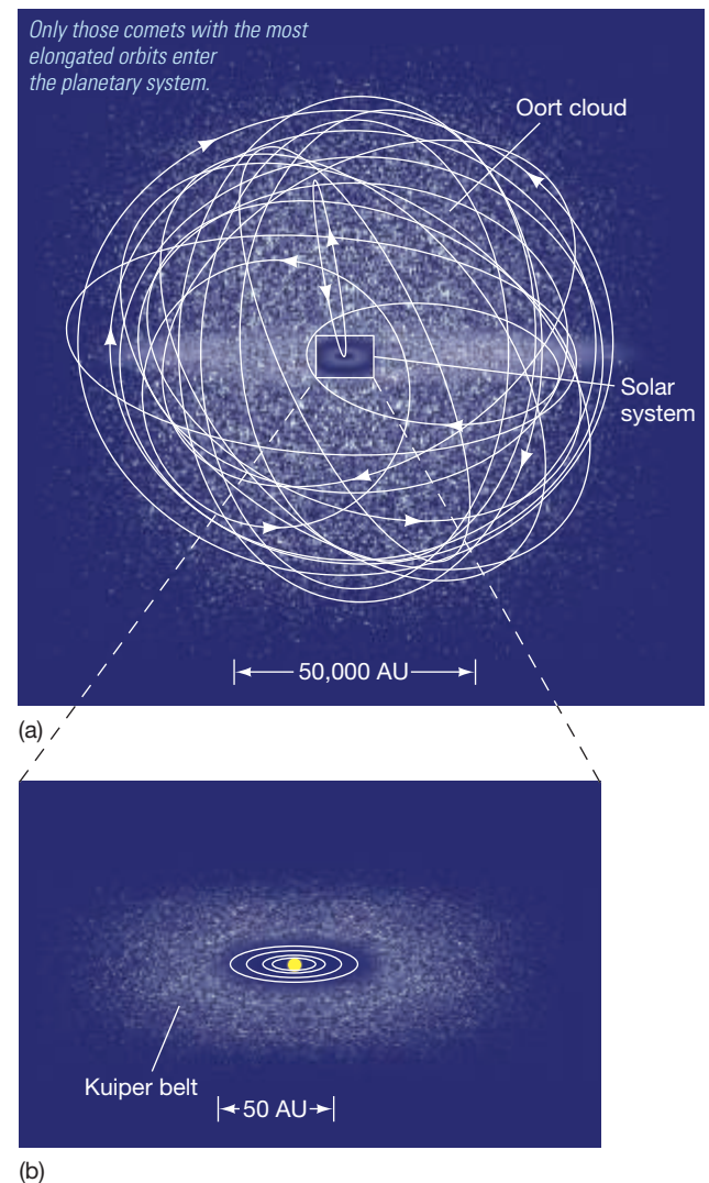
▲ FIGURE 4.15 Comet Reservoirs (a) Diagram of the Oort cloud, showing a few cometary orbits. The solar system is smaller than the overlaid box at the center of the figure. (b) The Kuiper belt, the source of short-period comets, whose orbits hug the ecliptic plane.
