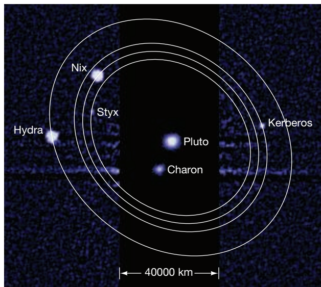
▲ FIGURE 8.30 Pluto Charon System Pluto, Charon, and four smaller moons can be seen in this 2012 Hubble Space Telescope image. The vertical black stripe in the middle of the frame is there because Pluto and Charon were imaged with a much shorter exposure than the other much fainter moons. The orbits of the outer moons are marked. (NASA)
