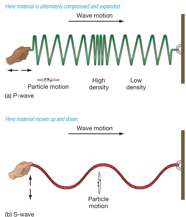
▲ FIGURE 5.8 P- and S-waves (a) Pressure (P) waves traveling through Earth's interior cause material to vibrate in a direction parallel to the direction of motion of the wave. (b) Shear (S) waves produce motion perpendicular to the direction in which the wave travels, pushing material from side to side.
