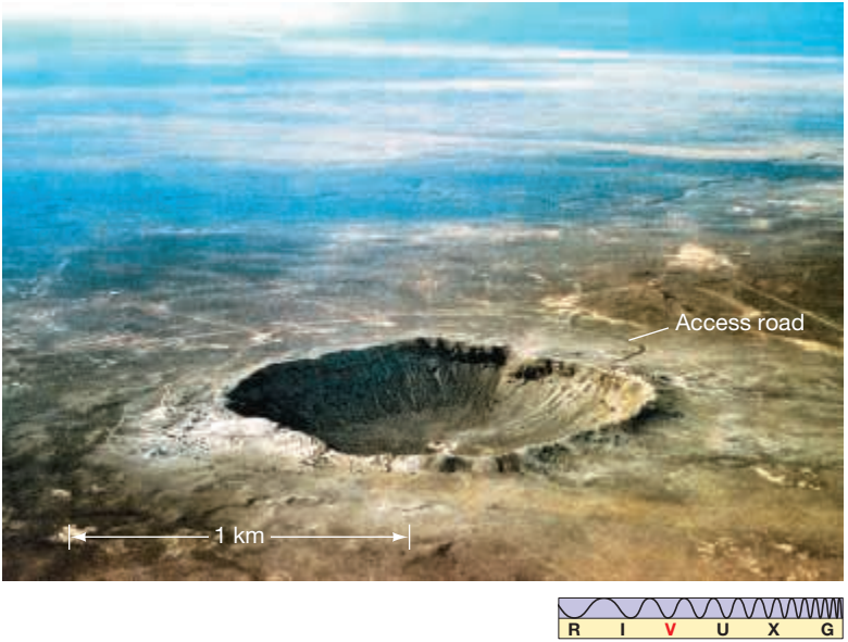
► FIGURE 4.19 Barringer Crater The Barringer Meteor Crater, near Winslow, Arizona, 1.2 km in diameter and 0.2 km deep, resulted from a meteorite impact about 25,000 years ago. The meteoroid was probably about 50 m across and likely weighed around 200,000 tons. (U.S. Geological Survey)
