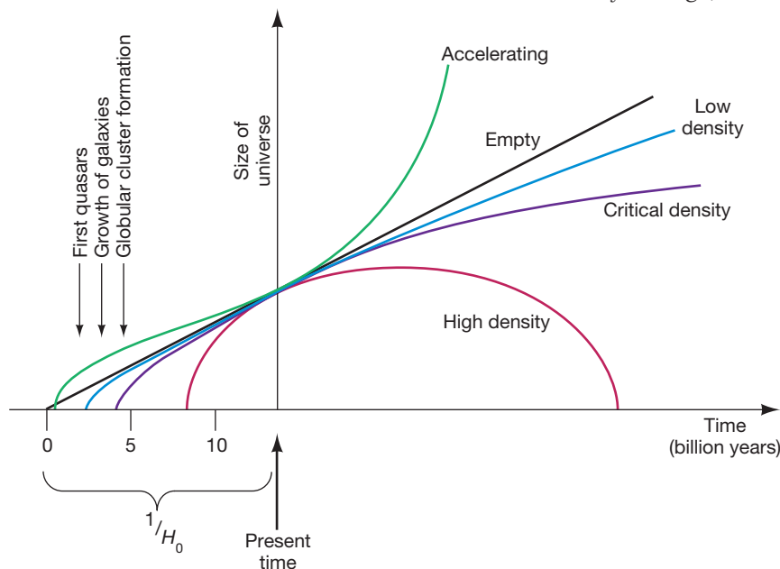
◀ FIGURE 17.12 Cosmic Age The age of a universe without dark energy (represented by all three lower curves colored red, purple, and blue) is always less than 1/H_0 and decreases for larger values of the present-day density. The existence of a repulsive cosmological constant (green curve) increases the age of the cosmos.
