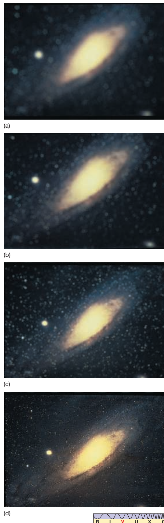
► FIGURE 3.12 Resolution Detail becomes clearer in the Andromeda galaxy as the angular resolution is improved some 600 times, from (a) 10', to (b) 1', (c) 5", and (d) 1". (Adapted from AURA)
