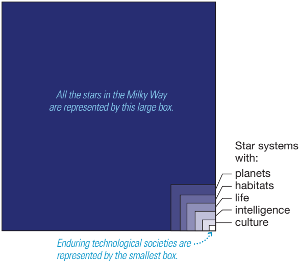
▲ FIGURE 18.10 Drake Equation Of all the star systems in our Milky Way Galaxy, progressively fewer and fewer have each of the qualities typical of a long-lasting technological society.
