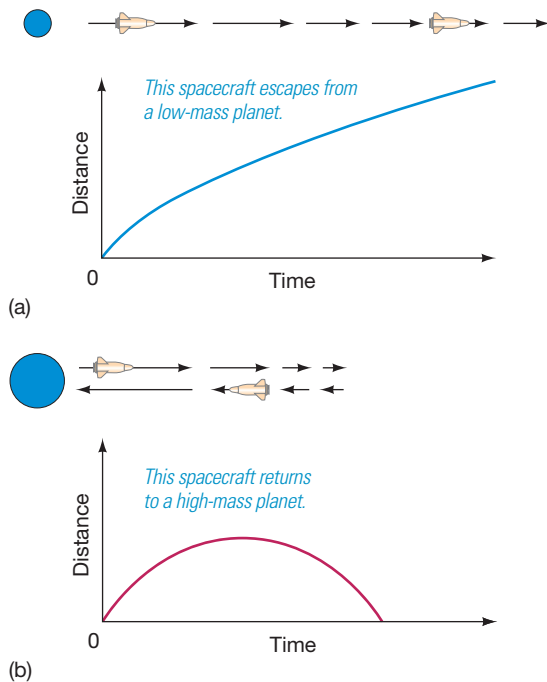
▲ FIGURE 17.5 Escape Speed (a) A spacecraft (arrow) leaving a planet (blue ball) with a speed greater than the planet's escape speed follows an unbound trajectory and escapes. (b) If the launch speed is less than the escape speed, the ship eventually drops back to the planet. Its distance, as graphed, first rises and then falls.
