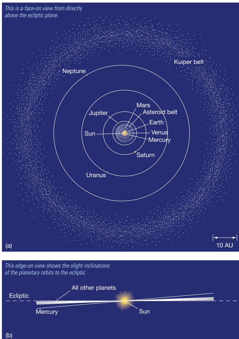
▲ FIGURE 4.1 Solar System Major bodies of the solar system include the Sun, planets, and asteroids. Except for Mercury, the orbits of the planets are almost circular (a) and lie nearly in the same plane (b). The entire solar system, including the Kuiper belt, spans nearly 100 AU.
