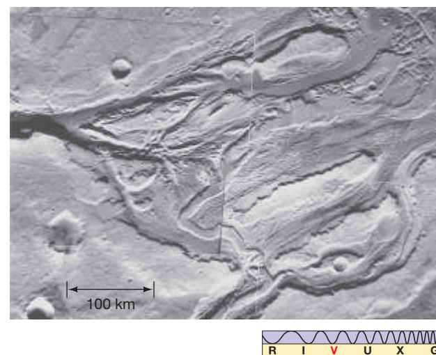
▲ FIGURE 6.24 Martian Outflow This outflow channel near the Martian equator bears witness to a catastrophic flood that occurred about 3 billion years ago. (NASA)
