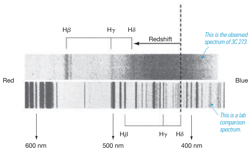
► FIGURE 15.28 Quasar Spectrum Optical spectrum of the distant quasar 3C 273. (This is a negative, as the lines are actually in emission.) Notice the redshift of the three hydrogen spectral lines marked as H\beta , H\gamma , and H\delta . (Sec. 2.6) The widths of these lines imply rapid internal motion within the quasar. (Adapted from Palomar/Caltech)
