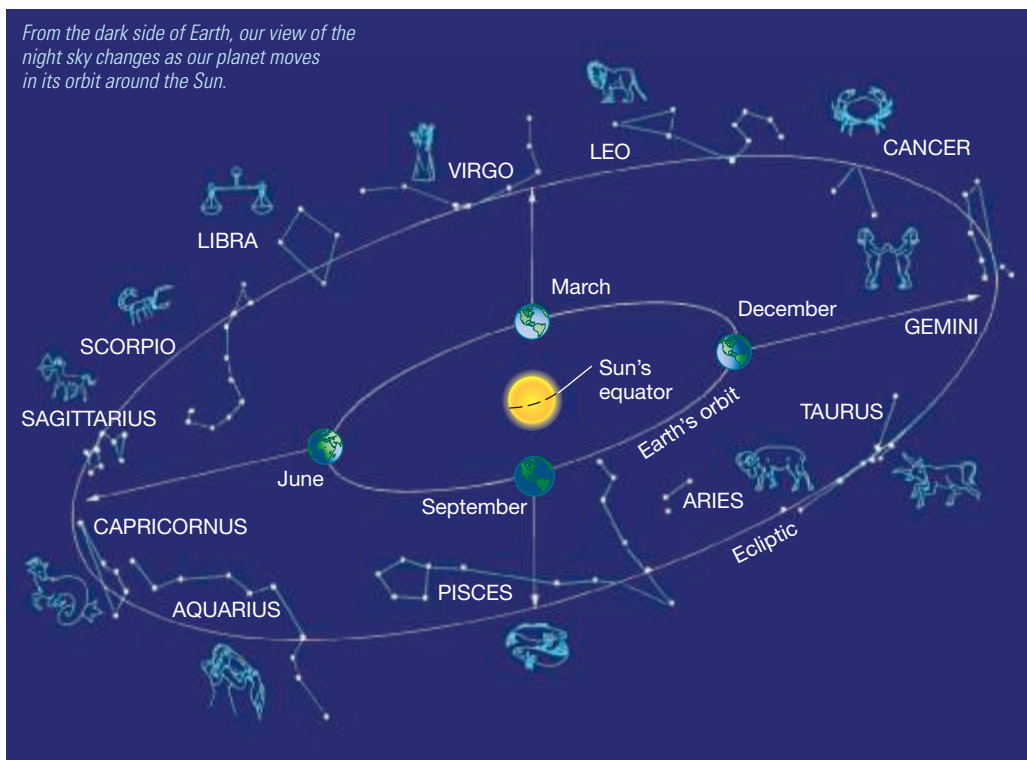
► FIGURE 0.8 The Zodiac INTERACTIVE The night side of Earth faces a different set of constellations at different times of the year. The 12 constellations named here make up the astrological zodiac. The arrows indicate the most prominent zodiacal constellations in the night sky at various times of year. For example, in June, when the Sun is “in” Gemini, Sagittarius and Capricornus are visible at night.
