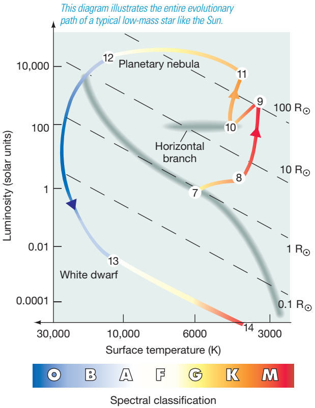
► FIGURE 12.10 White Dwarf on H-R Diagram INTERACTIVE A star’s passage from the horizontal branch (stage 10) to the white dwarf stage (stage 13) creates an evolutionary path that cuts across the H–R diagram.
