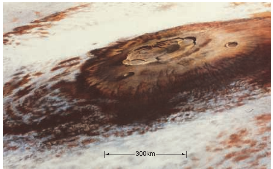
▲ FIGURE 6.22 Martian Volcano Olympus Mons, the largest volcano (now dormant) known on Mars or anywhere else in the solar system, is nearly three times taller than Mount Everest on Earth, measuring about 700 km across its base and rising 25 km high at its peak. By comparison, the largest volcano on Earth, Hawaii’s Mauna Loa, measures a mere 120 km across and peaks just 9 km above the Pacific Ocean floor. (NASA)
