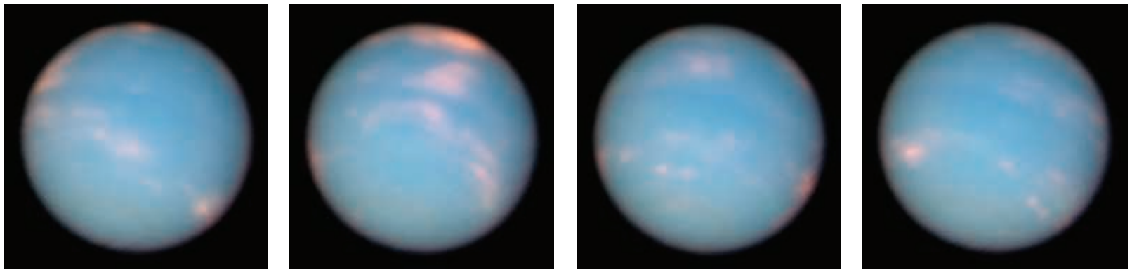
▲ FIGURE 7.18 Neptune's Dark Spot (a) These 2011 Hubble Space Telescope views of Neptune were taken at roughly 4-hour intervals, offering a full view of the planet. The cloud features (mostly methane ice crystals) are tinted pink here because they were imaged in the infrared, but they are white in visible light. (b) Close-up views, taken by Voyager 2 of the Great Dark Spot of Neptune, show a large storm system in the planet's atmosphere, possibly similar in structure to Jupiter's Great Red Spot. The entire dark spot is roughly the size of Earth. (NASA)
