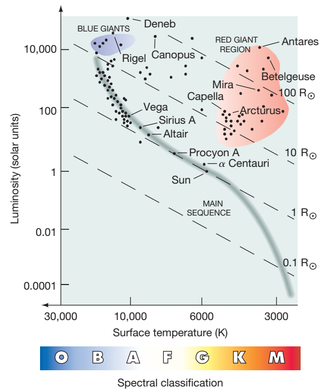
▲ FIGURE 10.14 H–R Diagram of Brightest Stars INTERACTIVE An H–R diagram for the 100 brightest stars in the sky is biased in favor of the most luminous stars—which appear toward the upper left—because we can see them more easily than we can the faintest stars. (Compare with Figure 10.13, which shows only the closest stars.)
