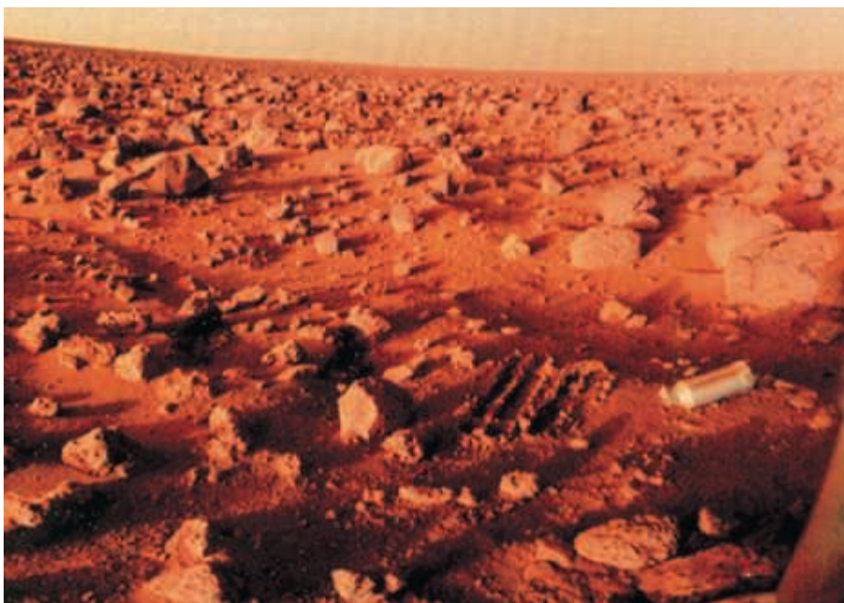
▲ FIGURE 6.30 Viking View This is the view from the Viking 2 spacecraft, now parked on Mars's northern Utopian plains. The fine-grained soil and the reddish rock-strewn terrain stretching toward the horizon contain substantial amounts of iron ore. The sky is pale pink, the result of airborne dust. The discarded canister in the foreground is about 20 cm long; the 0.5-m scars in the dirt were made by the robot's shovel. (NASA)
