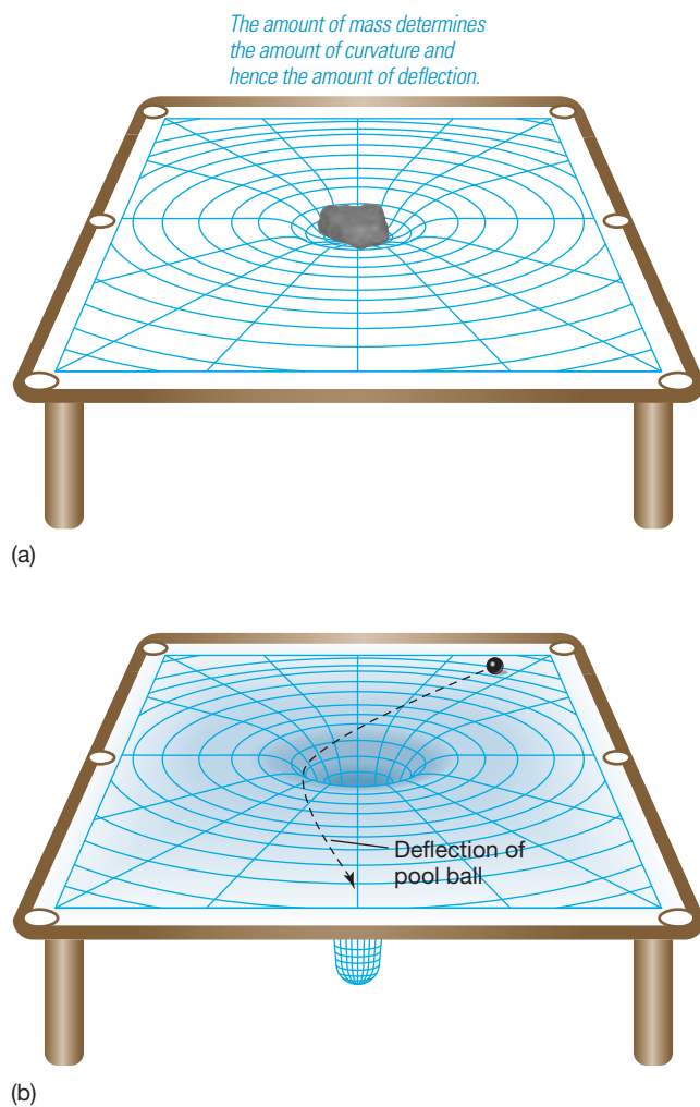
◀ FIGURE 13.18 Curved Space INTERACTIVE (a) A pool table made of a thin rubber sheet sags when a weight is placed on it. Likewise, space is bent, or warped, in the vicinity of any massive object. (b) A ball shown rolling across the table is deflected by the curvature of the surface, in much the same way that a planet's curved orbit is determined by the curvature of spacetime produced by the Sun.
