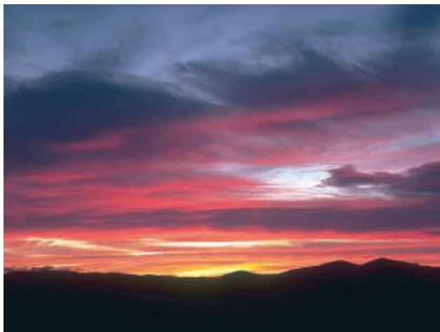
◀ FIGURE 11.3 Reddening in Earth's Atmosphere Sunlight is reddened as it passes through Earth's atmosphere at the end of a hot summer day. Airborne dust particles and water molecules scatter the Sun's blue light, leaving only its dimmed, red light—a spectacular sunset. (Joyce Photographics)
