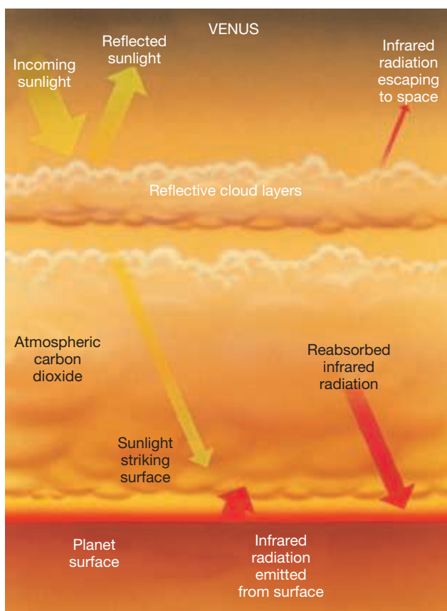
◀ FIGURE 6.34 Venus's Atmosphere Venus's atmosphere is much deeper and denser than Earth's, so a much smaller fraction of the infrared radiation leaving the planet's surface escapes into space. The result is a much stronger greenhouse effect and a correspondingly hotter planet.
