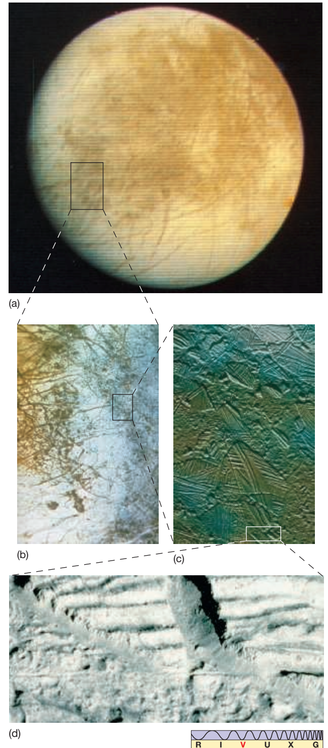
▲ FIGURE 8.5 Europa (a) A Voyager 1 mosaic of Europa. (b) Its icy surface is only lightly cratered, indicating that some ongoing process must be obliterating impact craters soon after they form. (c) This image from the Galileo spacecraft shows a smooth yet tangled surface, called Conamara Chaos, resembling the huge ice floes that cover Earth's polar regions. (d) This detailed Galileo image shows "pulled apart" terrain that suggests liquid water upwelling from the interior and freezing, filling in the gaps between separating surface ice sheets. (NASA)
