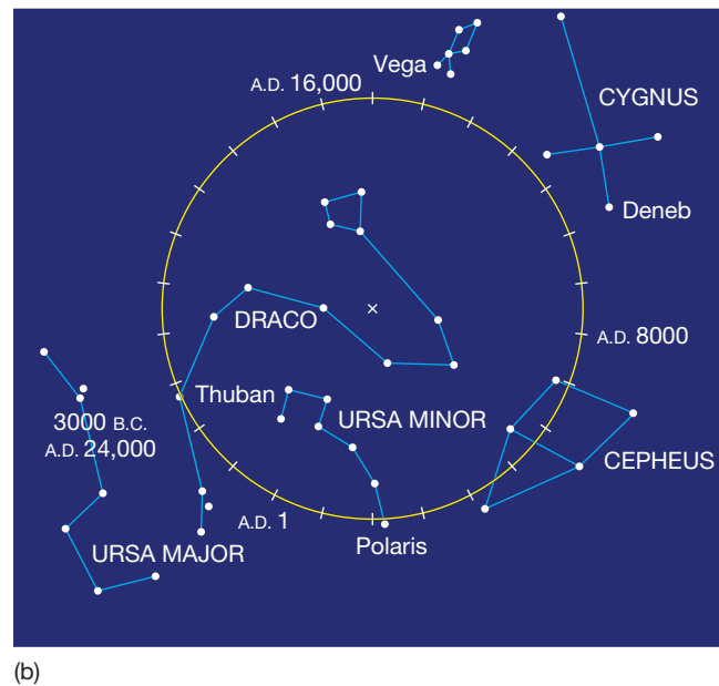
▲ FIGURE 0.12 Precession INTERACTIVE (a) Earth's axis currently points nearly toward the star Polaris. Some 12,000 years from now, Earth's axis will point toward a star called Vega, which will then be the "North Star." Five thousand years ago, the North Star was a star named Thuban in the constellation Draco. (b) The yellow circle shows the precessional path of the north celestial pole among some prominent northern stars and depicts the direction toward which Earth's pole points on the sky. Each tick mark represents 1000 years.
