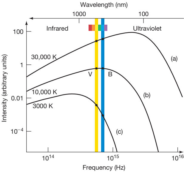
▲ FIGURE 10.8 Blackbody Curves Star (a) is very hot—30,000 K—so its B (blue) intensity is greater than its V (visual) intensity. Star (b) has roughly equal B and V readings and so appears white. Its temperature is about 10,000 K. Star (c) is red; its V intensity greatly exceeds the B value, and its temperature is 3000 K.
