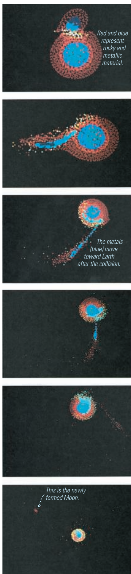
◀ FIGURE 5.26 Moon Formation This sequence shows a simulated collision between Earth and an object the size of Mars. (The sequence proceeds from top to bottom and zooms out dramatically in the later frames.) Note how most of the impactor's metallic core becomes part of Earth, leaving the Moon composed primarily of rocky material. ( W. Benz )
