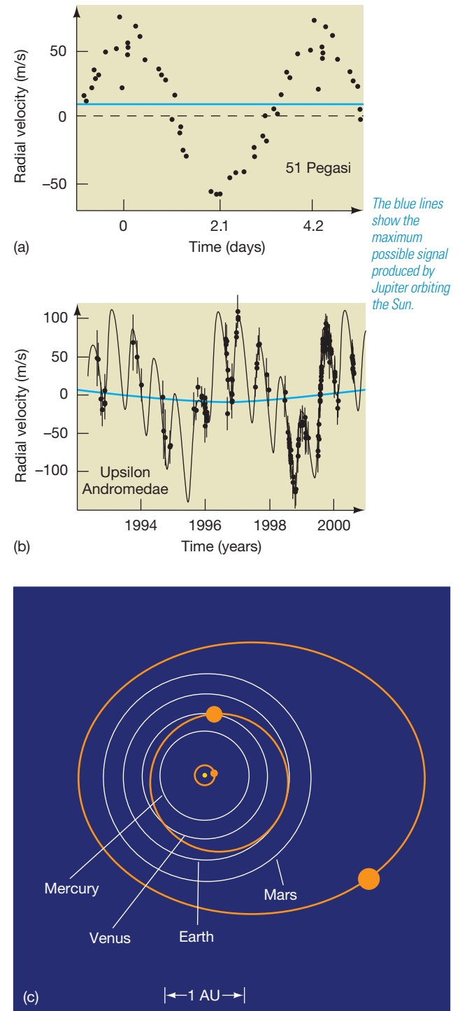
► FIGURE 4.32 Planets Revealed INTERACTIVE (a) Discovery data of the Doppler shift of the star 51 Pegasi reveal a clear periodic signal indicating the presence of a planetary companion of mass at least half the mass of Jupiter. (b) Radial velocity data for Upsilon Andromedae are more complex, but are well fit (solid line) by a three-planet system orbiting the star. (c) A sketch of the inferred orbits of the three planets in the Upsilon Andromedae system (in orange) with the orbits of the terrestrial planets superimposed for comparison (in white).
