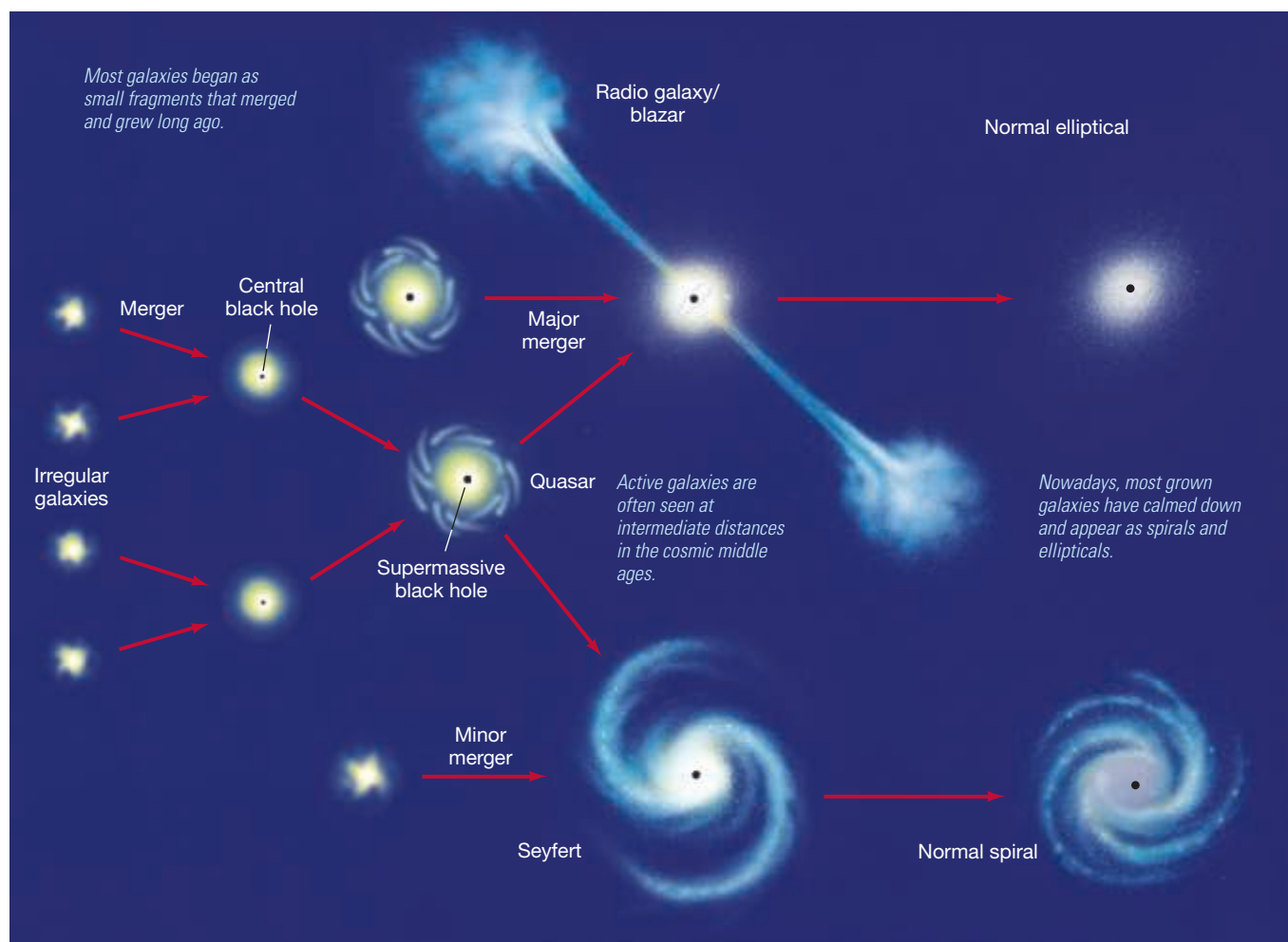
▲ FIGURE 16.19 Galaxy Evolution Most evolutionary sequences for galaxies began with galaxy mergers that led to highly luminous quasars, after which they decreased in violence through the radio and Seyfert galaxies, eventually resulting in normal ellipticals and spirals. The central black holes that powered the early activity remain at later times, but many of them have run out of fuel.
