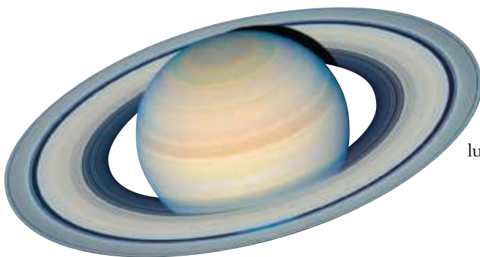
◀ FIGURE 7.2 Saturn Saturn as seen by the Hubble Space Telescope in 2003 when the planet was at its maximum tilt (27°) toward Earth in its 30-year orbit about the Sun. The colors in this photo are natural—that is, as we would see it if we had telescopic vision. (See also the full-page opening photo on page 200.) (NASA)
