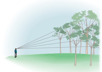
▲ FIGURE 17.2 Olbers's Paradox If the universe were homogeneous, isotropic, infinite in extent, and unchanging, then any line of sight from Earth should eventually meet a star and the entire night sky should be bright. This obvious contradiction of the facts is known as Olbers's paradox.
