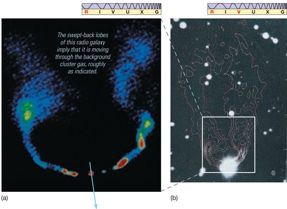
► FIGURE 16.4 Head-Tail Radio Galaxy (a) Radiograph, in false color, of the head-tail radio galaxy NGC 1265. (b) The same radio data, in contour form, superimposed on the optical image of the galaxy. (NRAO; Palomar/Caltech)
