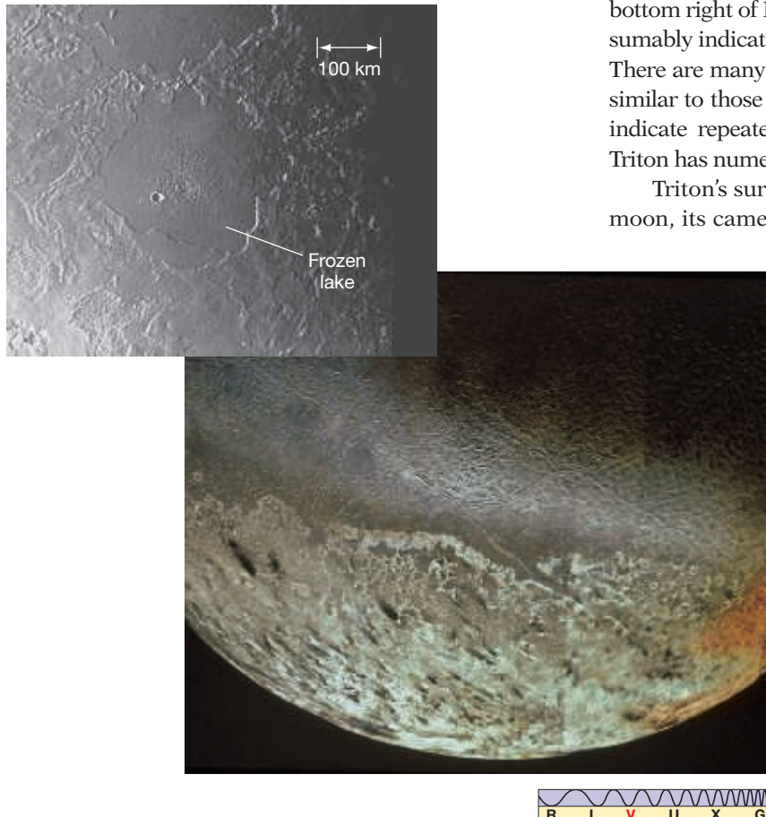
◀ FIGURE 8.14 Triton The south polar region of Triton, showing a variety of terrains ranging from deep ridges and gashes to what appear to be frozen water lakes, all indicative of past surface activity. The pinkish region at the lower right is nitrogen frost, forming the moon's polar cap. The roughly circular lakelike feature shown in the inset may have been caused by the eruption of an ice volcano. (NASA)
