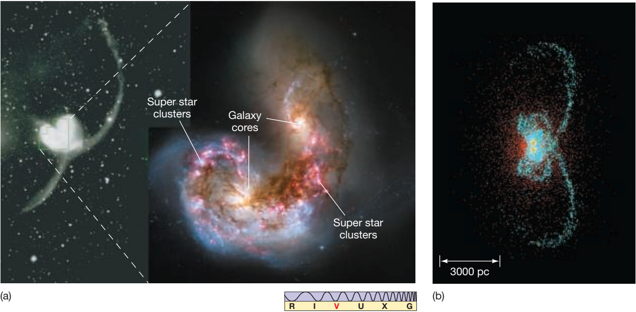
► FIGURE 16.8 Galaxy Collision (a) The long tidal “tails” (black-and-white image at left) mark the final plunge of the “Antennae” galaxies a few tens of millions of years ago. Strings of young, bright “super star clusters” (magnified color image at center) were caused by violent shock waves produced in the gas disks of the two colliding galaxies. (b) A computer simulation of the encounter shows many of the same features as the real object at left. (AURA; NASA; J. Barnes)
