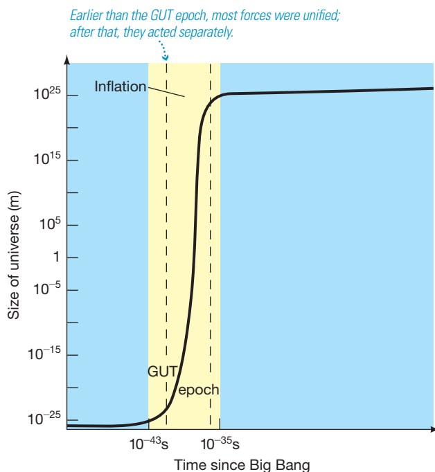
▲ FIGURE 17.21 Cosmic Inflation During the period of inflation, the universe expanded enormously in a very short time. Afterward, it resumed its earlier “normal” expansion rate, except that the size of the cosmos had become about 10^{50} times bigger than it was before inflation.
