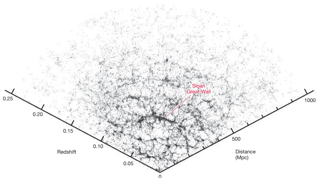
▲ FIGURE 17.1 Galaxy Survey This map of the universe is drawn using data from the Sloan Digital Sky Survey. ∞ (Discovery 16-1) It shows the locations of 66,976 galaxies lying within 12 degrees of the celestial equator and extending to a distance of almost 1000 Mpc (or a redshift of about 0.25). The largest known structure in the universe, the Sloan Great Wall, stretches nearly 300 Mpc across the center of the frame. (SDSS Collaboration)
