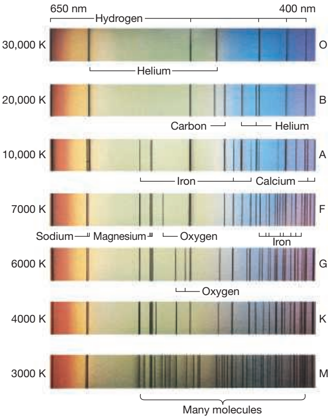
▲ FIGURE 10.9 Stellar Spectra Comparison of spectra observed for seven different stars having a range of surface temperatures. The spectra of the hottest stars, at the top, show lines of helium and multiply ionized heavy elements. In the coolest stars, at the bottom, helium lines are absent, but lines of neutral atoms and molecules are plentiful. At intermediate temperatures, hydrogen lines are strongest.
