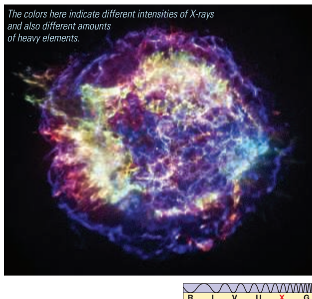
◀ FIGURE 3.28 X-Ray Image A false-color Chandra X-ray image of the supernova remnant Cassiopeia A, a debris field of scattered, hot gases that were once part of a massive star. Roughly 10,000 light-years from Earth and barely visible in the optical part of the spectrum, Cas A is awash in brilliantly glowing X-rays spread across some 10 light-years. (CXC/SAO)
