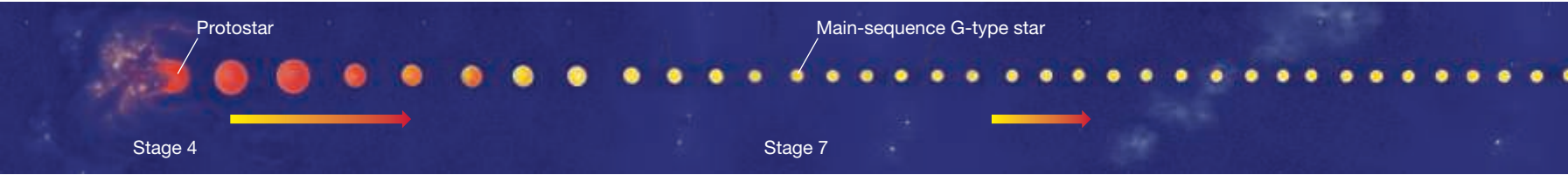
▼ FIGURE 12.8 G-type Star Evolution INTERACTIVE Artist’s conception of the relative sizes and changing colors of a normal G-type star (such as our Sun) during its formative stages, on the main sequence, and while passing through the red giant and white dwarf stages. At maximum swelling, the red giant is approximately 70 times the size of its main-sequence parent; the core of the giant is about 1/15 the main-sequence size and would be barely discernible if this figure were drawn to scale. The duration of time spent in the various stages—protostar, main-sequence star, red giant, and white dwarf—is roughly proportional to the lengths shown in this imaginary trek through space.
