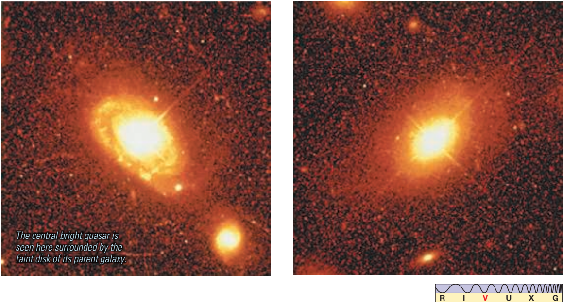
► FIGURE 16.18 Quasar Host Galaxies These long-exposure images of distant quasars show the young host galaxies in which the quasars reside, lending support to the idea that quasars represent an early, very luminous phase of galactic evolution. The quasar at the left is the best example, having the catalog name PG0052 + 251 and residing roughly 690 Mpc from Earth. (NASA)
