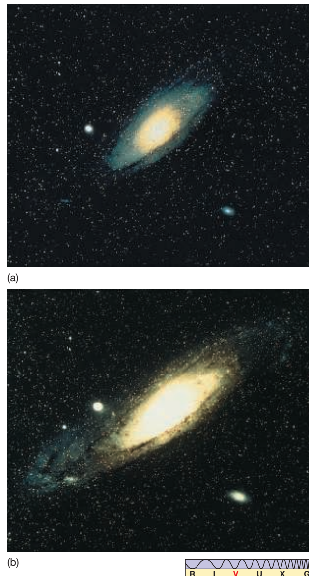
► FIGURE 3.9 Sensitivity Telescope size affects the image of a cosmic source, in this case the Andromeda galaxy. Both of these photographs had the same exposure time, but image (b) was taken with a telescope twice the size of that used to make image (a). Fainter detail can be seen as the diameter of the telescope mirror increases because larger telescopes are able to collect more photons per unit time. (Adapted from AURA)
