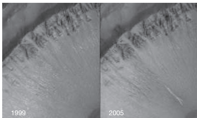
◀ FIGURE 6.29 Running Water on Mars? (a) This high-resolution Mars Global Surveyor view of a crater wall near the Mariner Valley shows evidence of "gullies" apparently formed by running water in the relatively recent past. (b) Comparison of two images taken 6 years apart of another Martian impact crater shows that something—the white streak (lower right), possibly water—flowed across the surface. (NASA)
