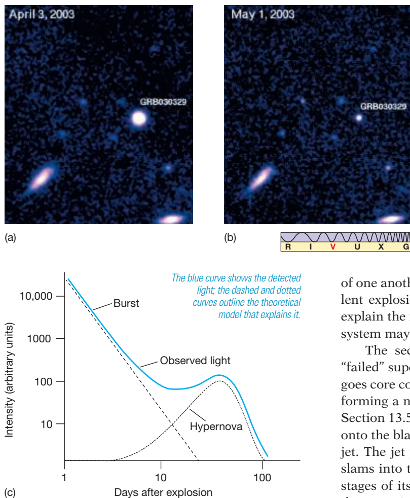
◀ FIGURE 13.13 Hypernova? The gamma-ray burst GRB 030329 may prove crucial to theorists' understanding of the physical processes underlying these violent phenomena. First detected by the High Energy Transient Explorer 2 satellite and subsequently observed at radio, optical, and X-ray wavelengths, the burst counterpart has all the hallmarks of a high-mass supernova, lending strong support to the hypernova model. Here, the counterpart is shown (a) near the moment of the burst and (b) fading a month later. (c) This graph shows details of the emitted radiation from another, but similar, gamma-ray burst. (ESO)
