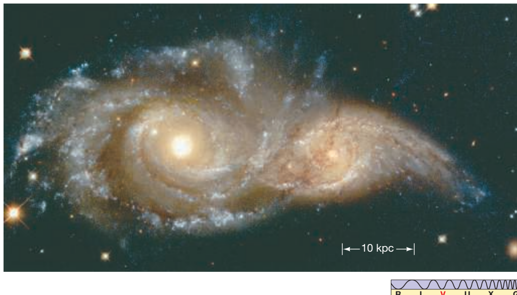
◀ FIGURE 16.6 Galaxy Encounter This encounter between two spiral galaxies, NGC 2207 (left) and IC 2163 (right), has already led to bursts of star formation in each. Eventually the two will merge, but not for a billion years or so. (NASA)
