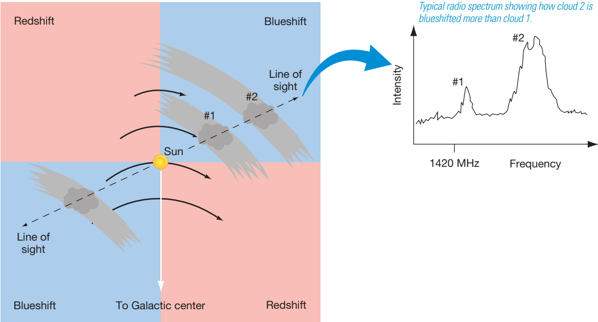
▼ FIGURE 14.14 Gas in the Galactic Disk Because the disk of our Galaxy is rotating differentially (inside faster than the outside), signals from different clumps of hydrogen matter along any line of sight are Doppler shifted by different amounts. Repeated observations in many different directions allow astronomers to map out the distribution of gas in our Galaxy.
