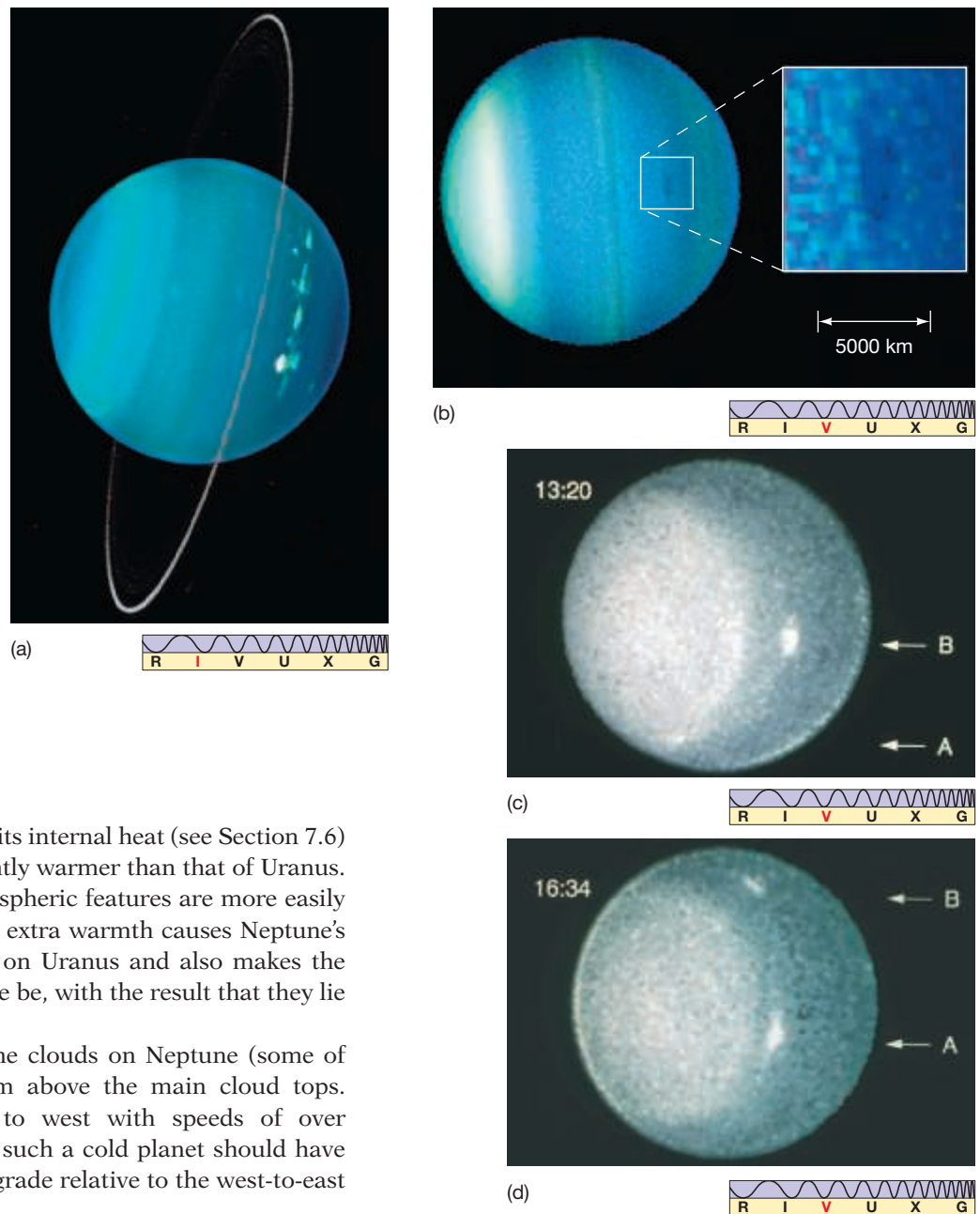
▲ FIGURE 7.17 Uranus's Atmosphere (a) This infrared image of Uranus was captured in 2004 by an adaptive optics system on an exceptionally clear night at the Keck Observatory in Hawaii. It shows unprecedented atmospheric detail, as well as a very thin ring. (b) The Hubble Space Telescope took this image of a rare dark spot on Uranus in 2006. (c, d) These computer-enhanced HST images, taken roughly 4 hours apart, show the motion of a pair of bright clouds (labeled A and B) in Uranus's southern hemisphere, allowing astronomers to track the planet's rotation. (L. Sromovsky and P. Fry; NASA)
