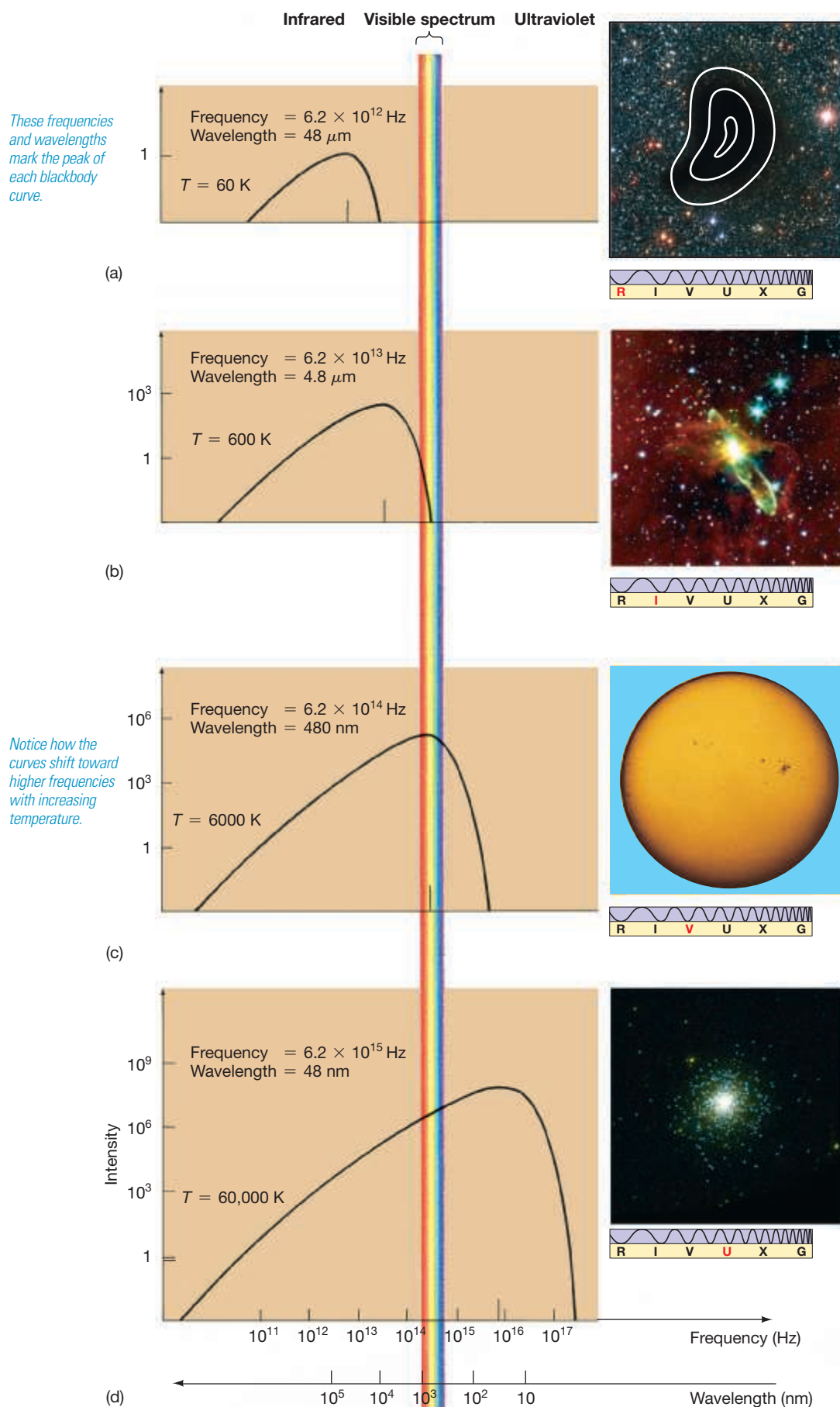
FIGURE 2.11 Blackbody Curves INTERACTIVE Comparison of blackbody curves for four cosmic objects. (a) A cool, dark galactic cloud called Barnard 68. At a temperature of 60 K, it emits mostly radio radiation, shown here as overlaid contours. (b) A dim, young star (shown white in the inset photograph) called Herbig-Haro 46. The star's atmosphere, at 600 K, radiates mainly in the infrared. (c) The Sun's surface, at approximately 6000 K, is brightest in the visible region of the electromagnetic spectrum. (d) Some very hot, bright stars in a cluster called Messier 2, as observed by an orbiting space telescope above Earth's atmosphere. At a temperature of 60,000 K, these stars radiate strongly in the ultraviolet. (ESO; AURA; NASA; Kennedy Space Center)
