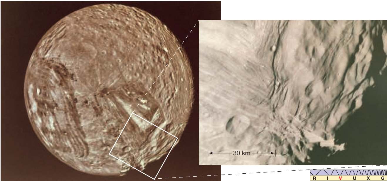
► FIGURE 8.18 Miranda The asteroid-sized innermost moon of Uranus, photographed by Voyager 2 . Miranda has a fractured surface suggestive of a violent past, but the cause of the grooves and cracks is unknown. (NASA)
