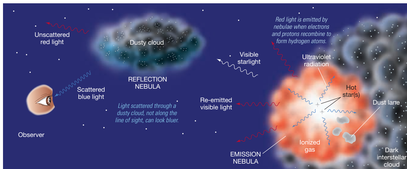
▼ FIGURE 11.8 Nebular Structure An emission nebula results when ultraviolet radiation from one or more hot stars ionizes part of an interstellar cloud. If starlight happens to encounter another dusty cloud, some of the radiation, particularly at the shorter wavelength blue end of the spectrum, may be scattered back toward Earth, forming a reflection nebula.
