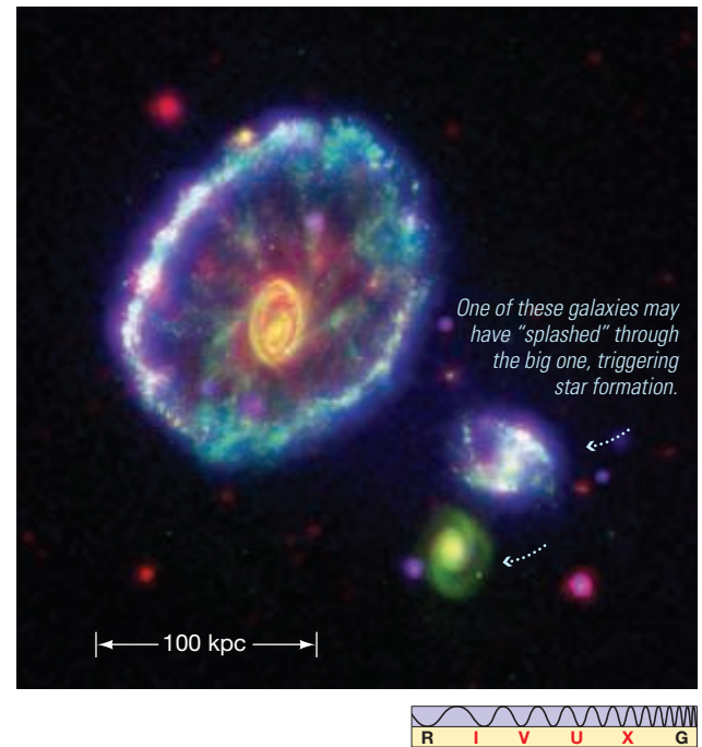
▲ FIGURE 16.5 Cosmic Splash The Cartwheel Galaxy (left) may have resulted from a collision (possibly with one of the smaller galaxies at right) that has led to an expanding ring of star formation moving outward through the galactic disk. This is a false color composite image combining four spectral bands: infrared in red (from Spitzer ), optical in green (from Hubble ), ultraviolet in blue (from Galex ), and X-ray in purple (from Chandra ). (NASA)
