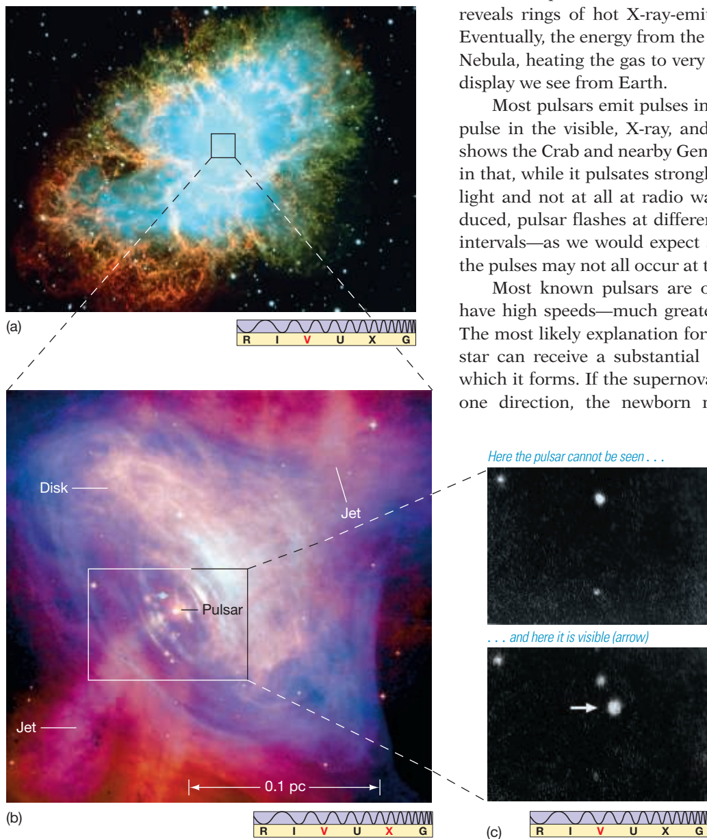
◀ FIGURE 13.4 Crab Pulsar In the core of the Crab Nebula (a), the Crab pulsar (c) blinks on and off about 30 times each second. In the top frame, the pulsar is off; in the bottom frame, it is on (arrow). (b) This Chandra X-ray image of the Crab, superimposed on a Hubble optical image, shows the central pulsar, as well as rings of hot X-ray-emitting gas in the equatorial plane, driven outward by the pulsar wind. Also visible in the image is a jet of hot gas escaping perpendicular to the equatorial plane. (ESO; NASA; UC/Lick Observatory)
