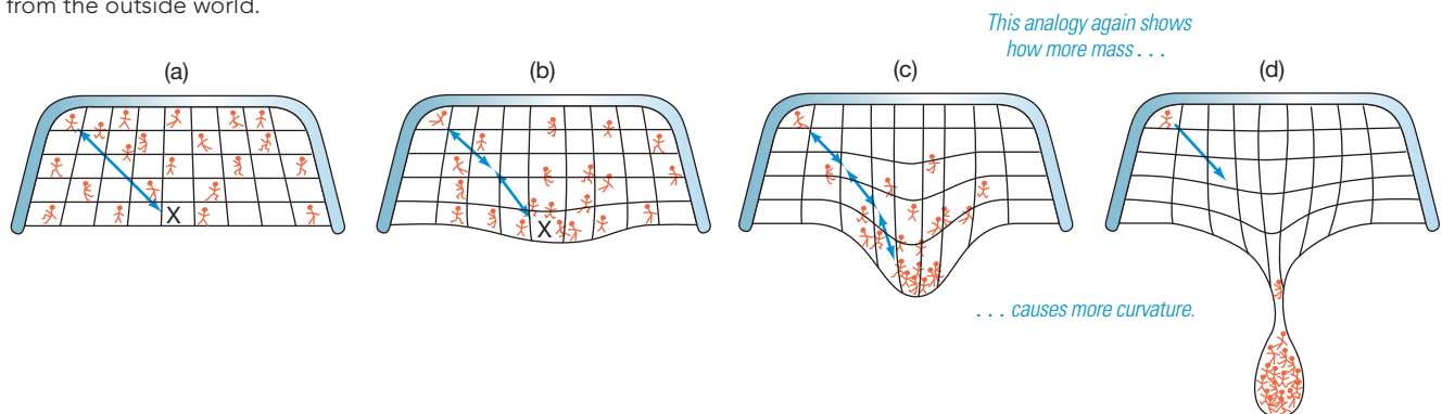
▼ FIGURE 13.19 Space Warping Mass causes a rubber sheet (or space) to be curved. As people assemble at a fixed spot on the sheet (marked by an “x”), the curvature grows larger, as shown in (a)–(c). The blue arrows represent some directions in which information can be sent from place to place. (d) The people are eventually sealed inside the bubble, forever trapped and cut off from the outside world.
